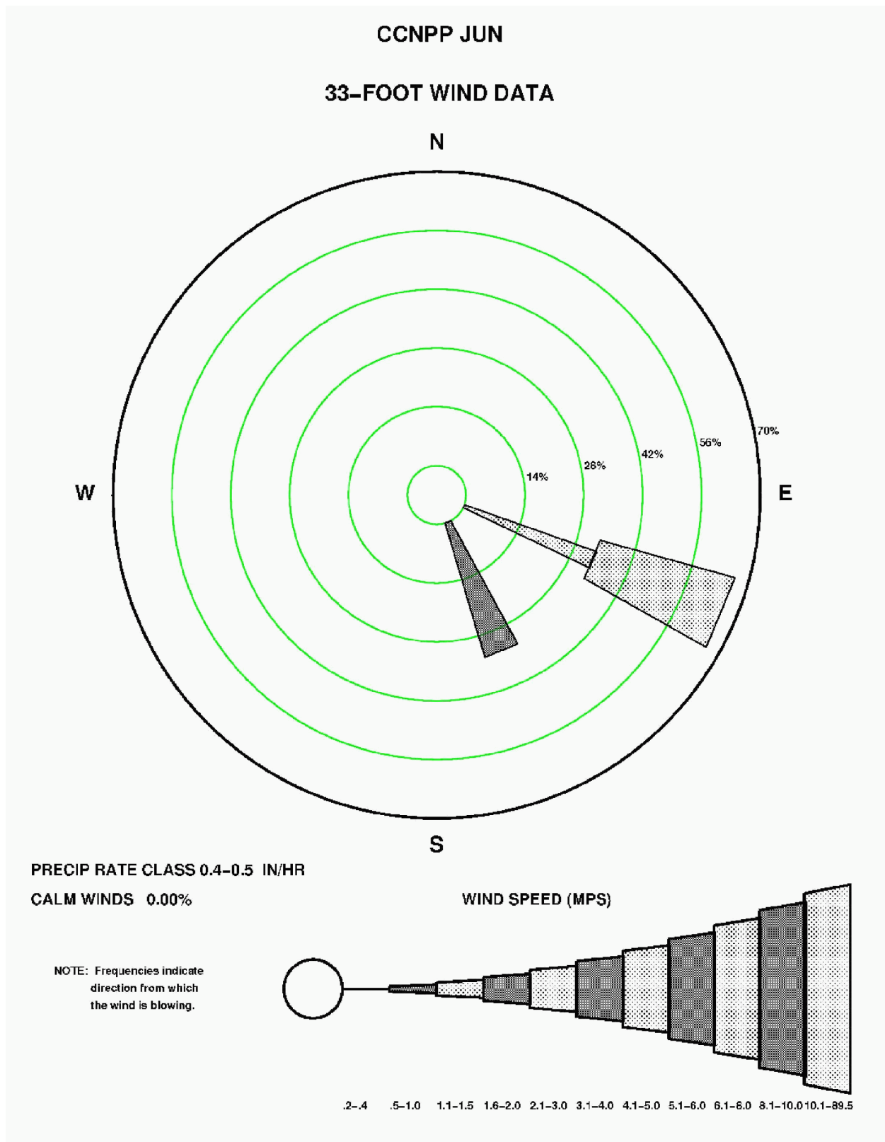
Figure 2.3-81—{CCNPP 33' (10 m) June Precipitation Wind Rose for Rate Class 0.4-0.5 in/hr}
