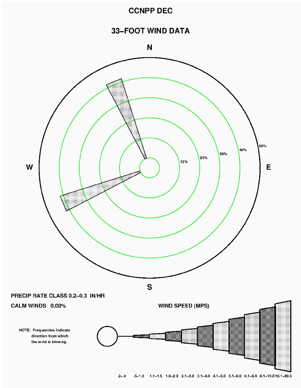
Figure 2.3-126—{CCNPP 33' (10 m) December Precipitation Wind Rose for Rate Class 0.2-0.3 in/hr}
