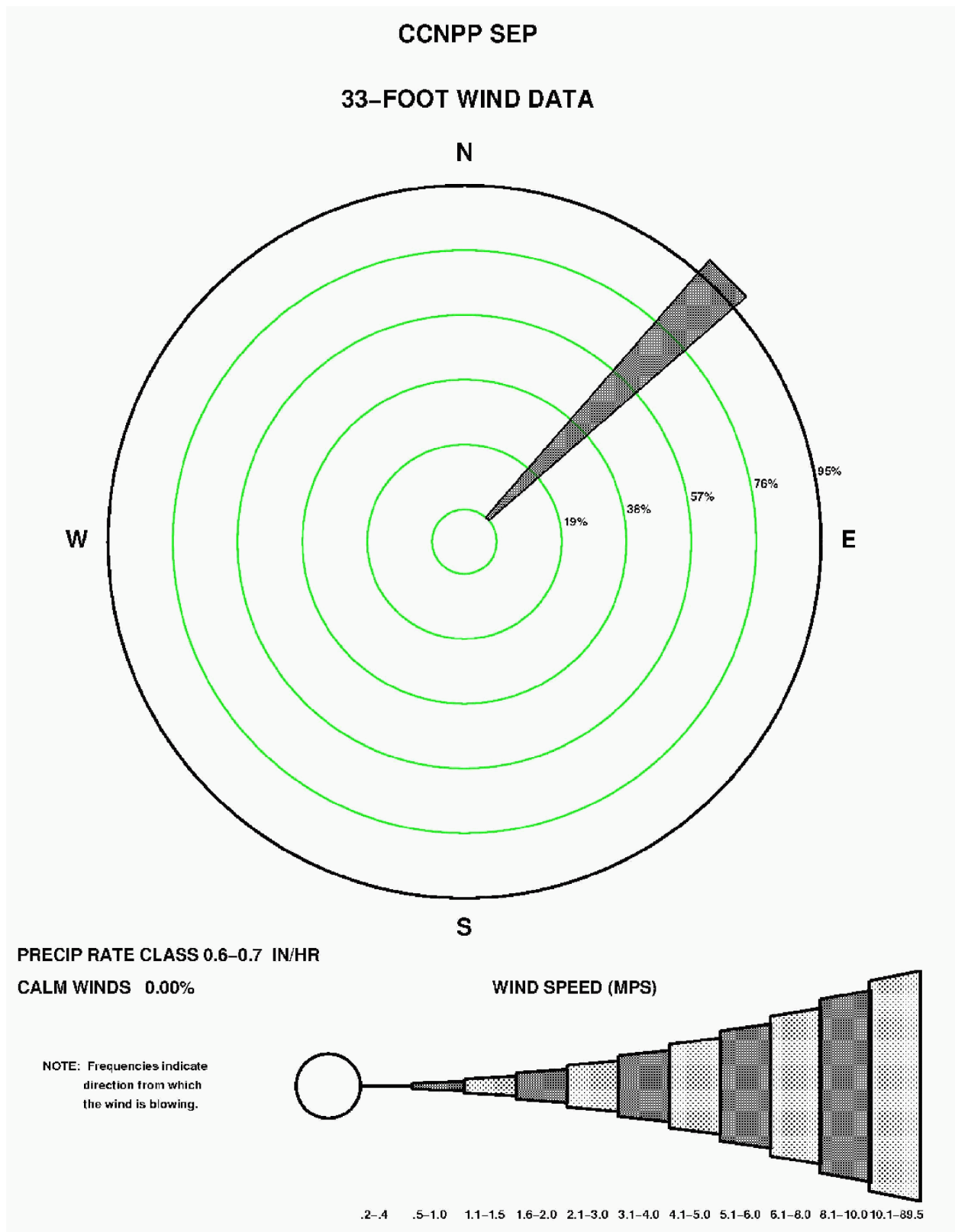
Figure 2.3-108—{CCNPP 33' (10 m) September Precipitation Wind Rose for Rate Class 0.6-0.7 in/hr}
