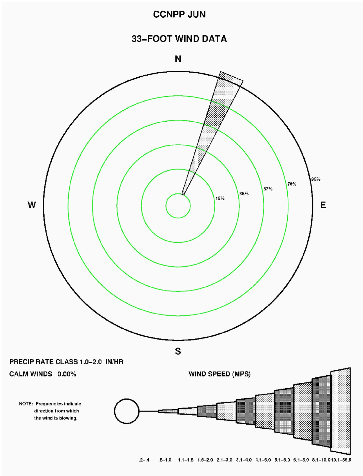
Figure 2.3-83—{CCNPP 33' (10 m) June Precipitation Wind Rose for Rate Class 1.0-2.0 in/hr}
