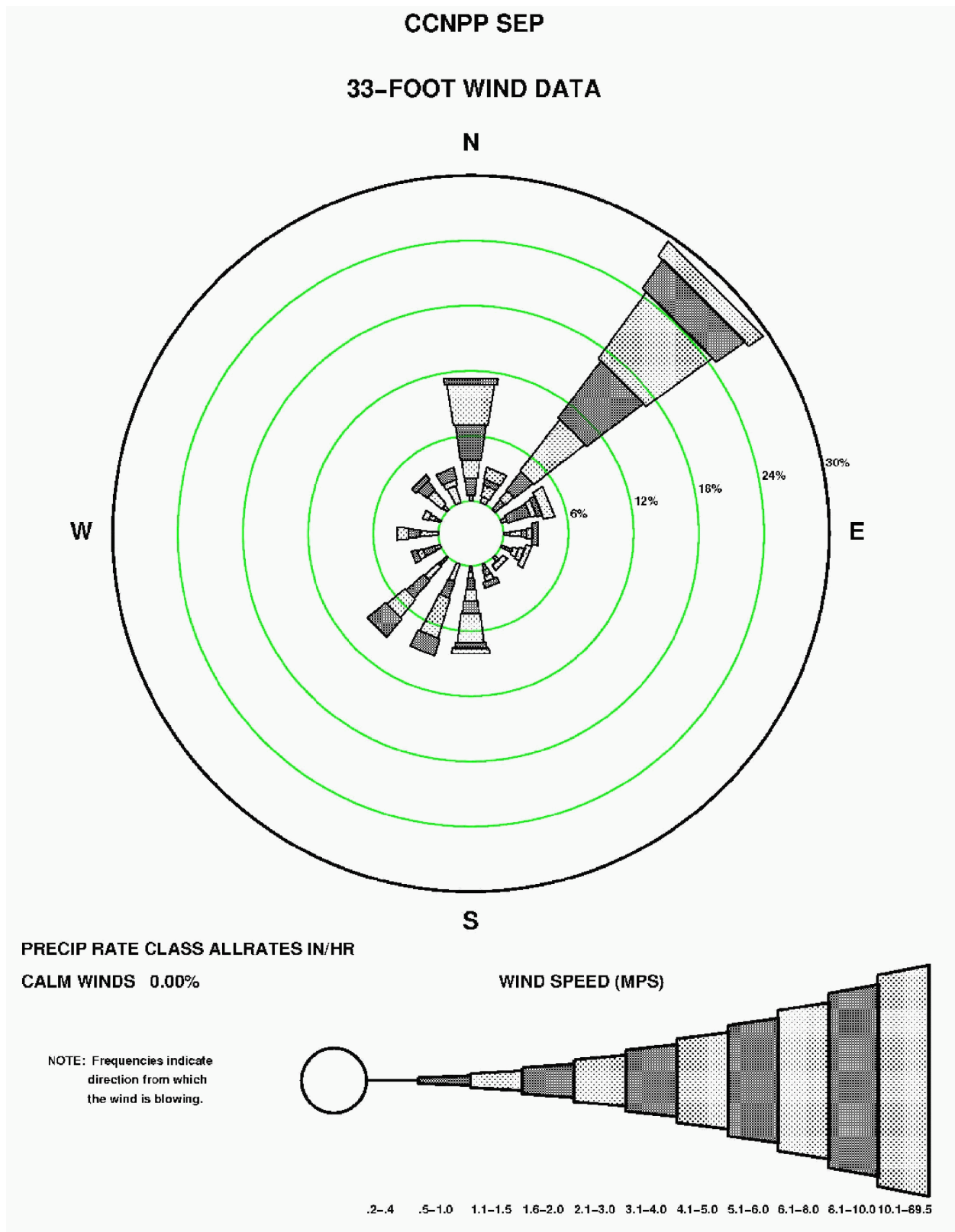
Figure 2.3-110—{CCNPP 33' (10 m) September Precipitation Wind Rose for All Rate classes}
