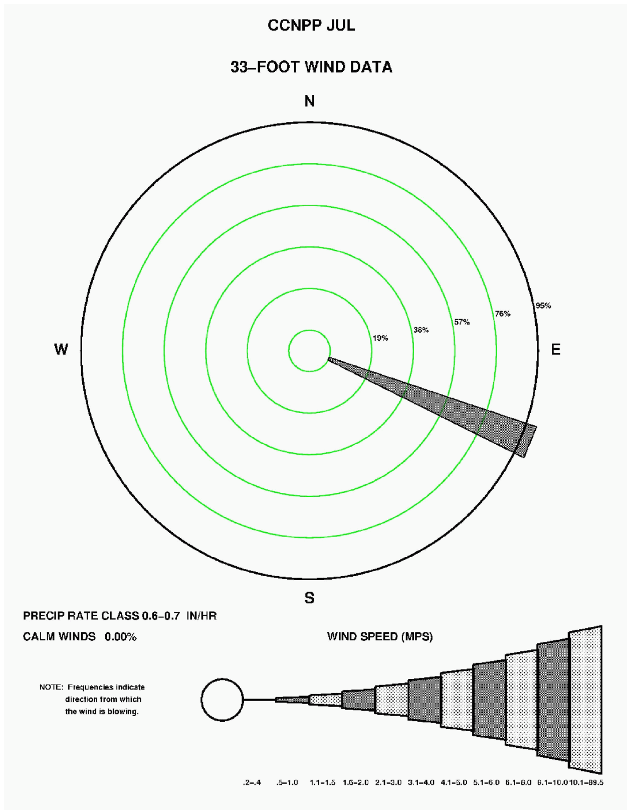
Figure 2.3-91—{CCNPP 33' (10 m) July Precipitation Wind Rose for Rate Class 0.6-0.7 in/hr}
