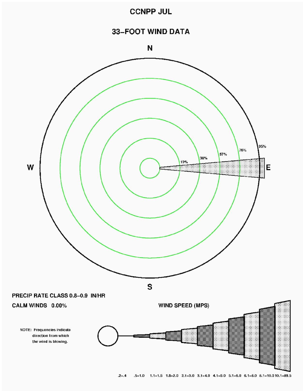
Figure 2.3-92—{CCNPP 33' (10 m) July Precipitation Wind Rose for Rate Class 0.8-0.9 in/hr}
