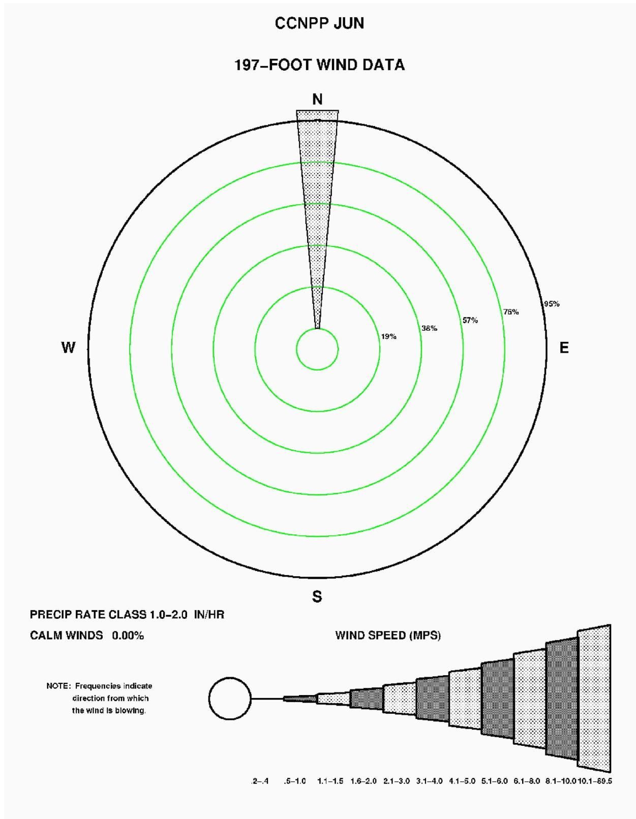
Figure 2.3-167—{CCNPP 197' (60 m) June Precipitation Wind Rose for Rate Class 1.0-2.0 in/hr}
