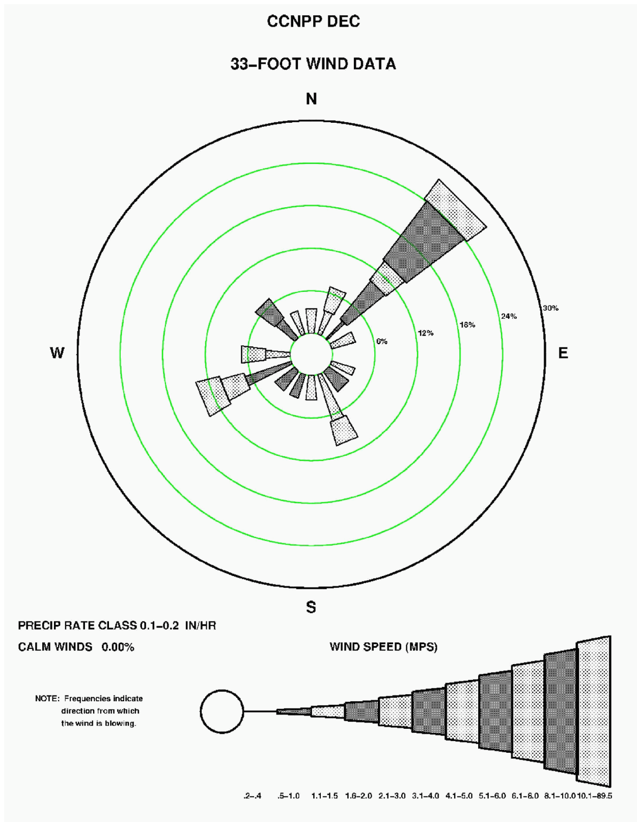
Figure 2.3-125—{CCNPP 33' (10 m) December Precipitation Wind Rose for Rate Class 0.1-0.2 in/hr}
