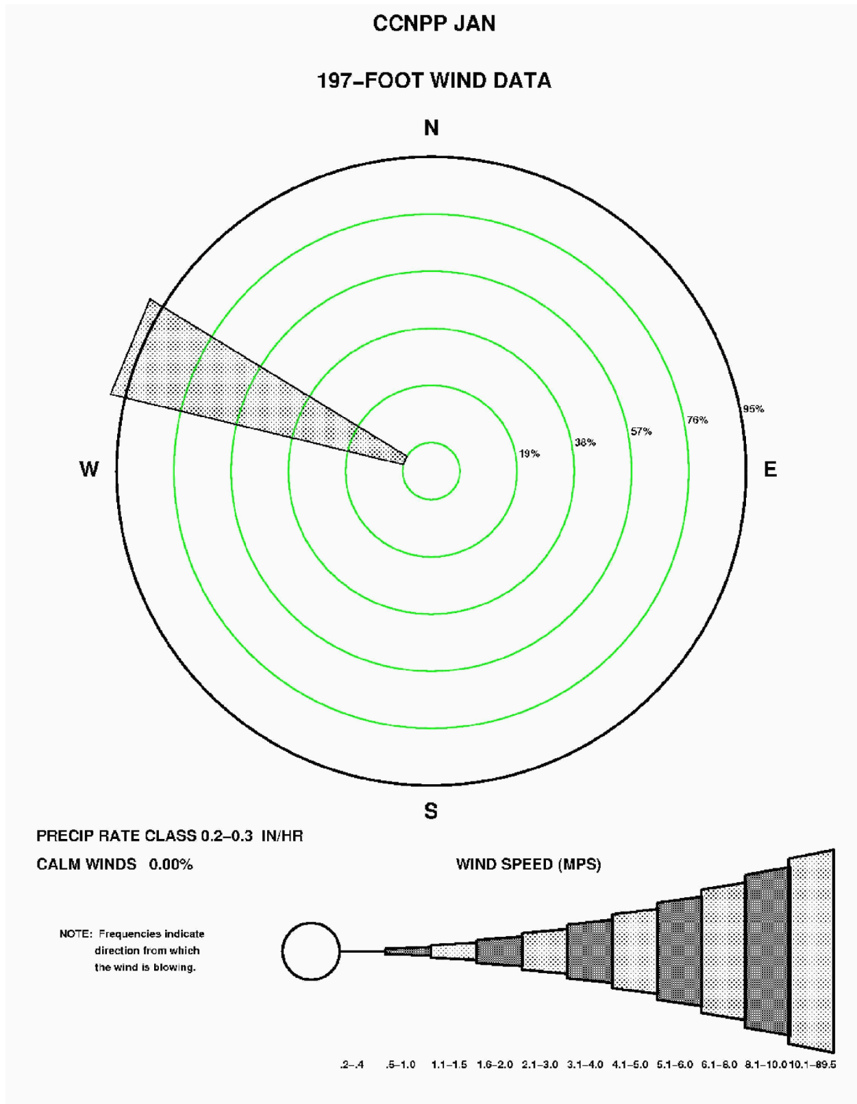
Figure 2.3-131—{CCNPP 197' (60 m) January Precipitation Wind Rose for Rate Class 0.2-0.3 in/hr}
