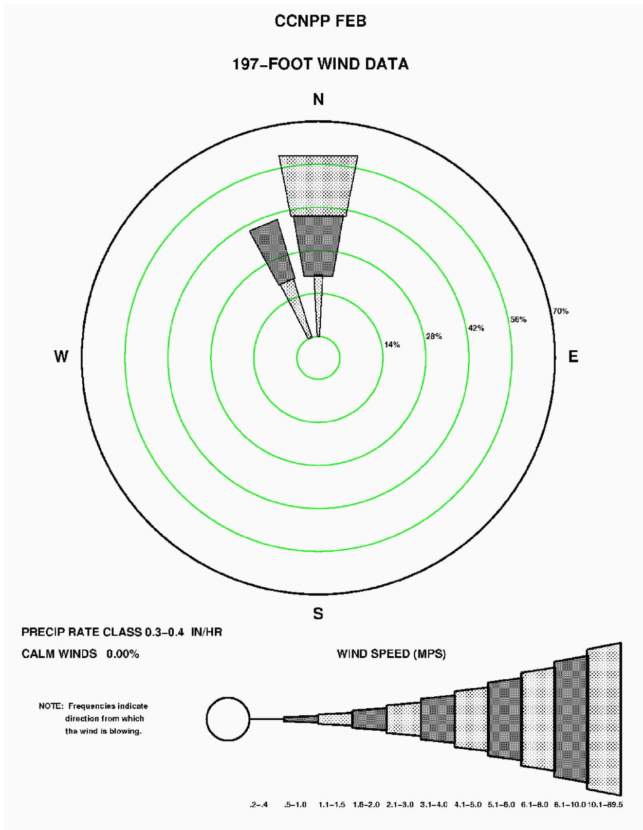
Figure 2.3-138—{CCNPP 197' (60 m) February Precipitation Wind Rose for Rate Class 0.3-0.4 in/hr}
