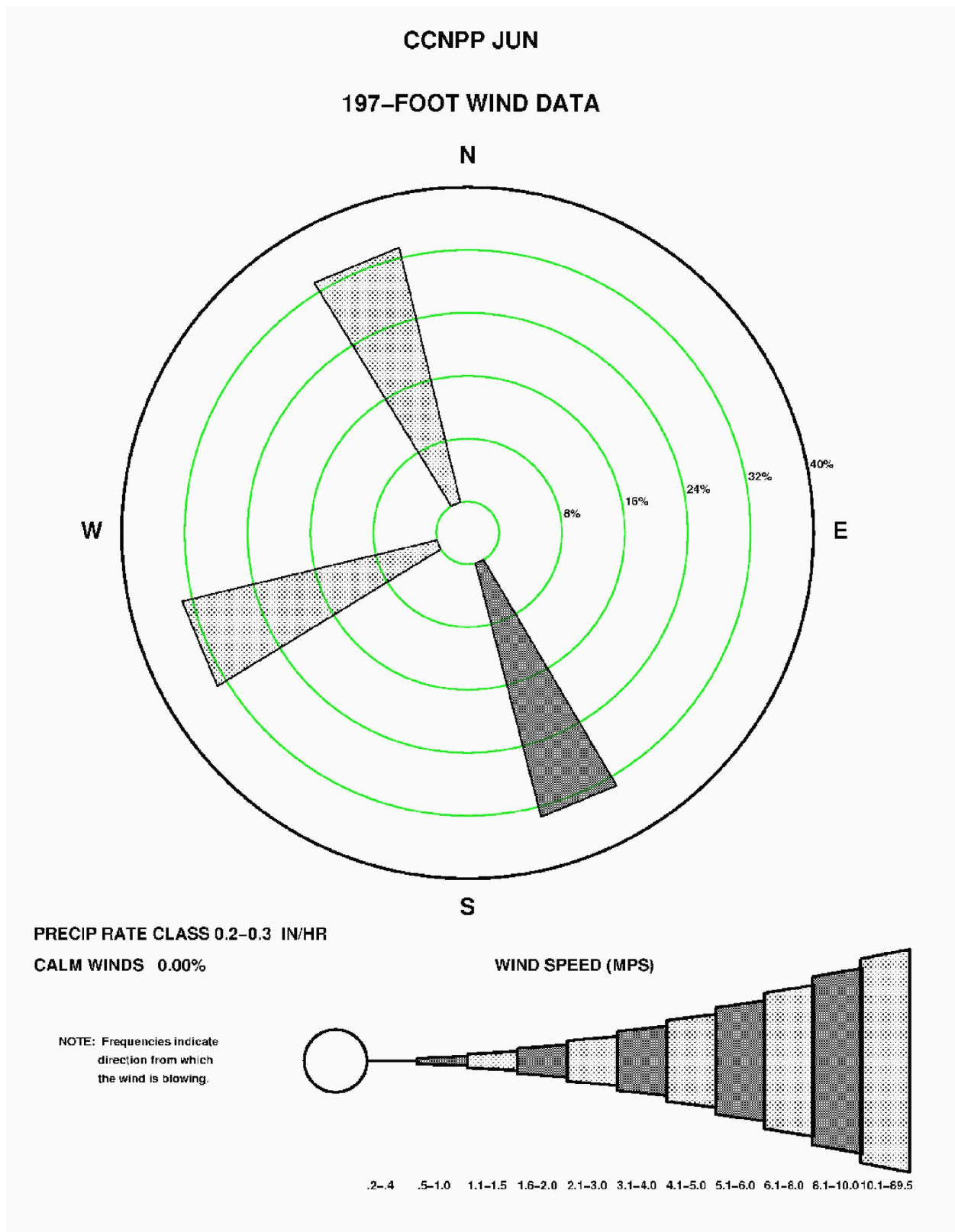
Figure 2.3-163—{CCNPP 197' (60 m) June Precipitation Wind Rose for Rate Class 0.2-0.3 in/hr}
