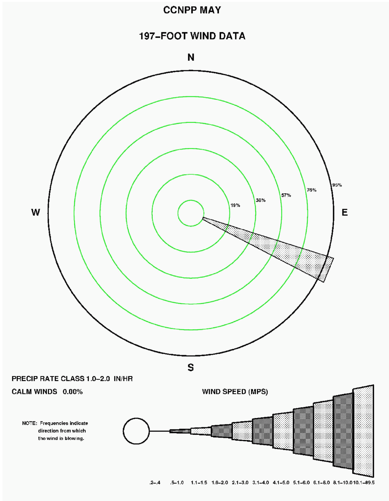
Figure 2.3-159—{CCNPP 197' (60 m) May Precipitation Wind Rose for Rate Class 1.0-2.0 in/hr}
