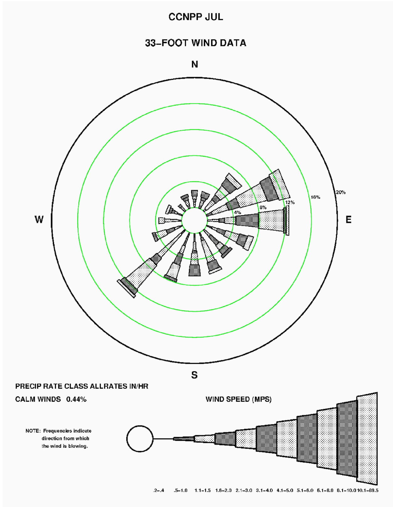
Figure 2.3-93—{CCNPP 33' (10 m) July Precipitation Wind Rose for All Rate classes}
