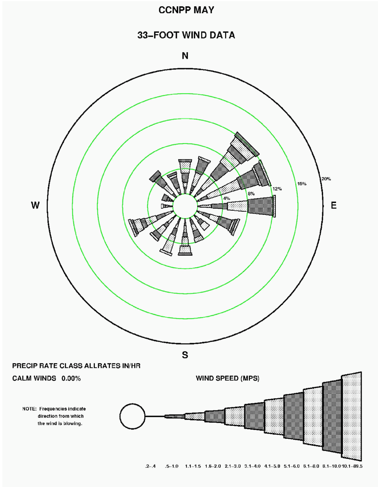
Figure 2.3-76—{CCNPP 33' (10 m) May Precipitation Wind Rose for All Rate classes}
