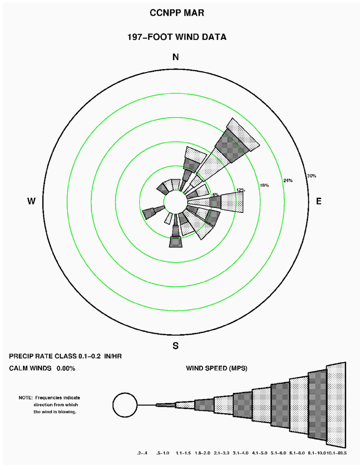
Figure 2.3-141—{CCNPP 197' (60 m) March Precipitation Wind Rose for Rate Class 0.1-0.2 in/hr}
