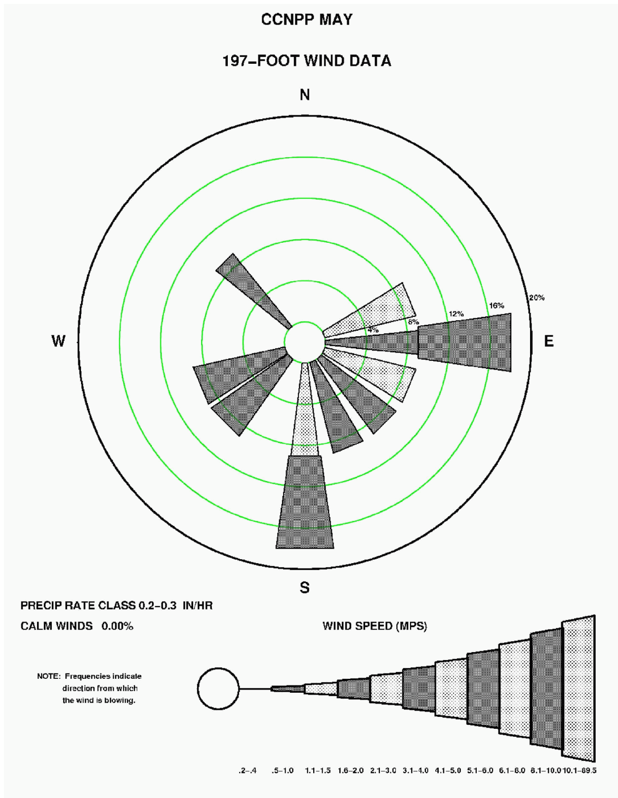
Figure 2.3-155—{CCNPP 197' (60 m) May Precipitation Wind Rose for Rate Class 0.2-0.3 in/hr}
