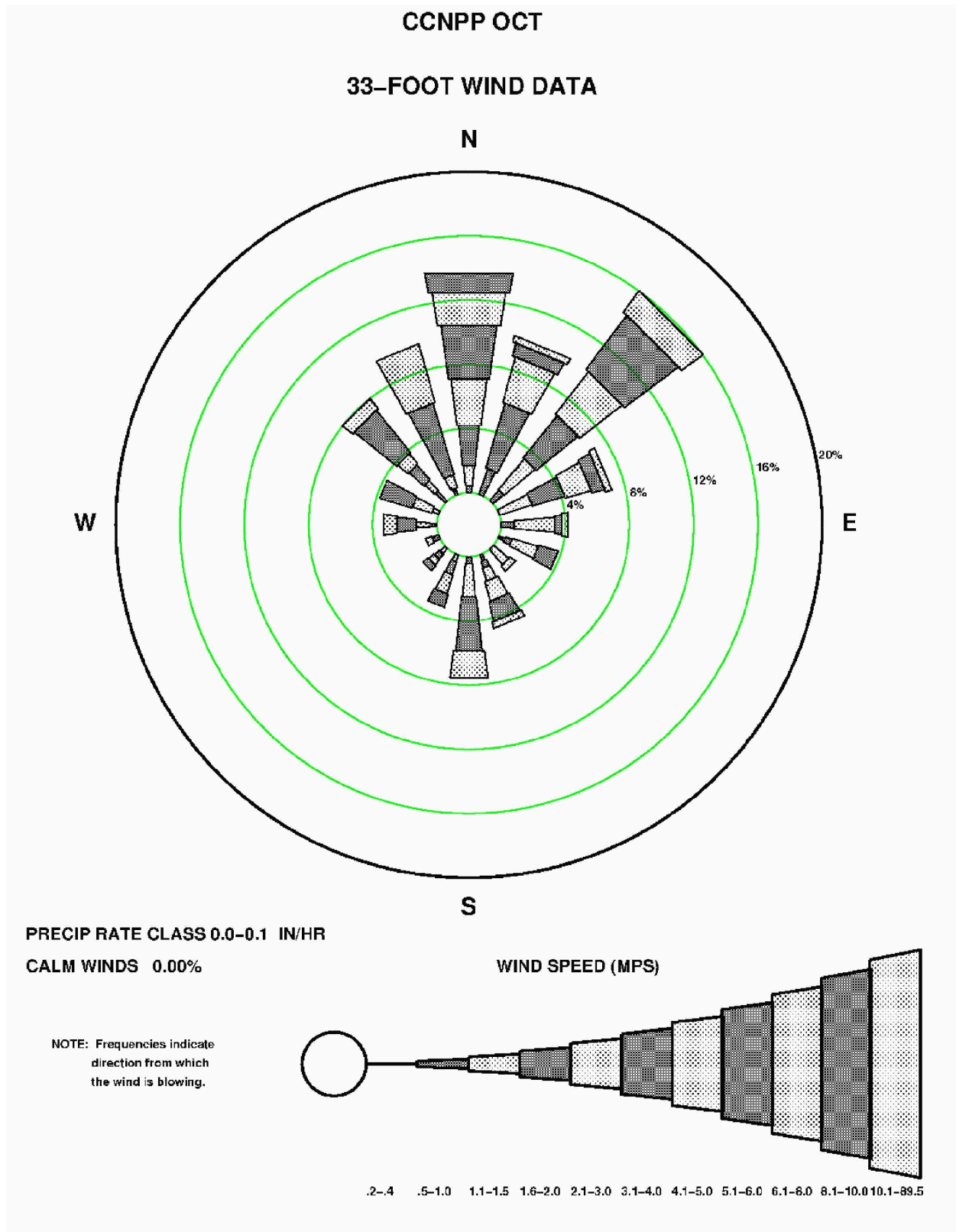
Figure 2.3-111—{CCNPP 33' (10m) October Precipitation Wind Rose for Rate Class 0.0-0.1 in/hr}
