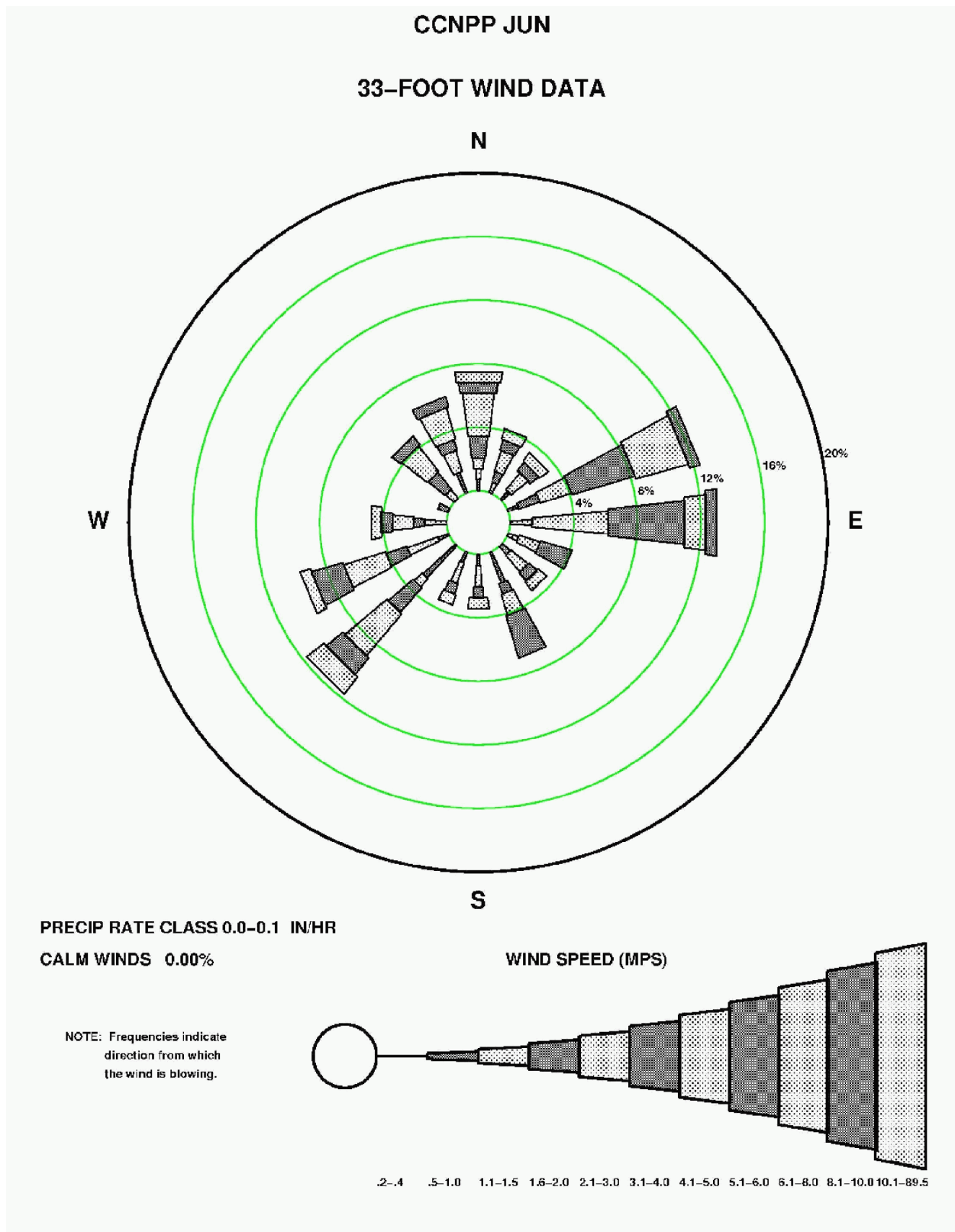
Figure 2.3-77—{CCNPP 33' (10 m) June Precipitation Wind Rose for Rate Class 0.0-0.1 in/hr}
