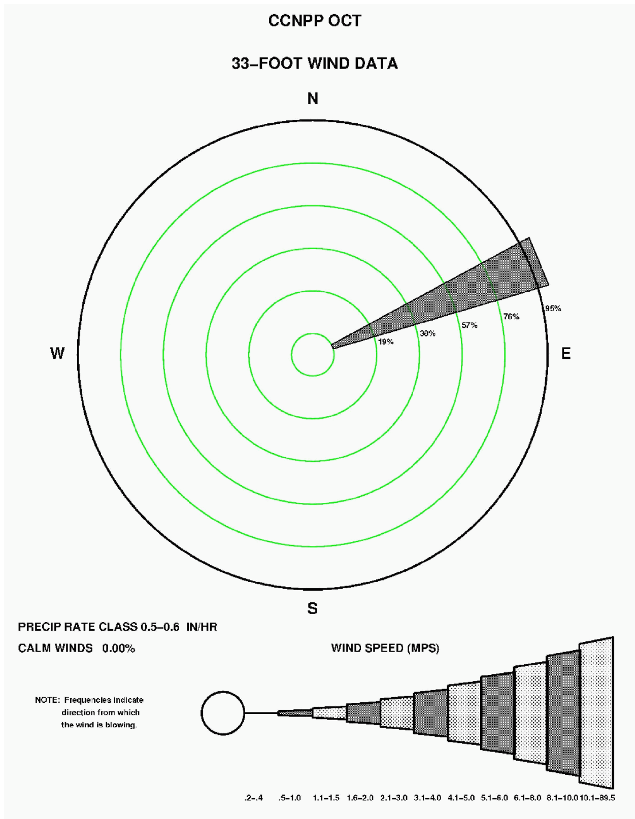
Figure 2.3-116—{CCNPP 33' (10 m) October Precipitation Wind Rose for Rate Class 0.5-0.6 in/hr}
