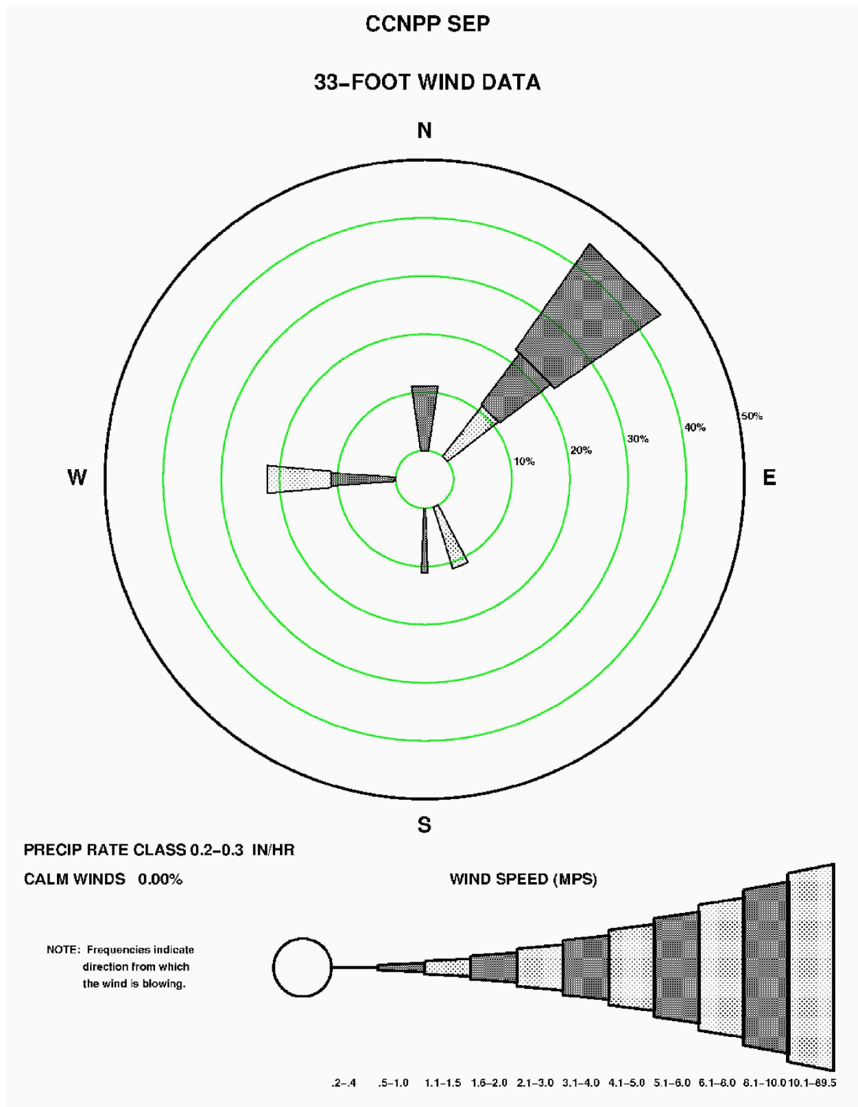
Figure 2.3-104—{CCNPP 33' (10 m) September Precipitation Wind Rose for Rate Class 0.2-0.3 in/hr}
