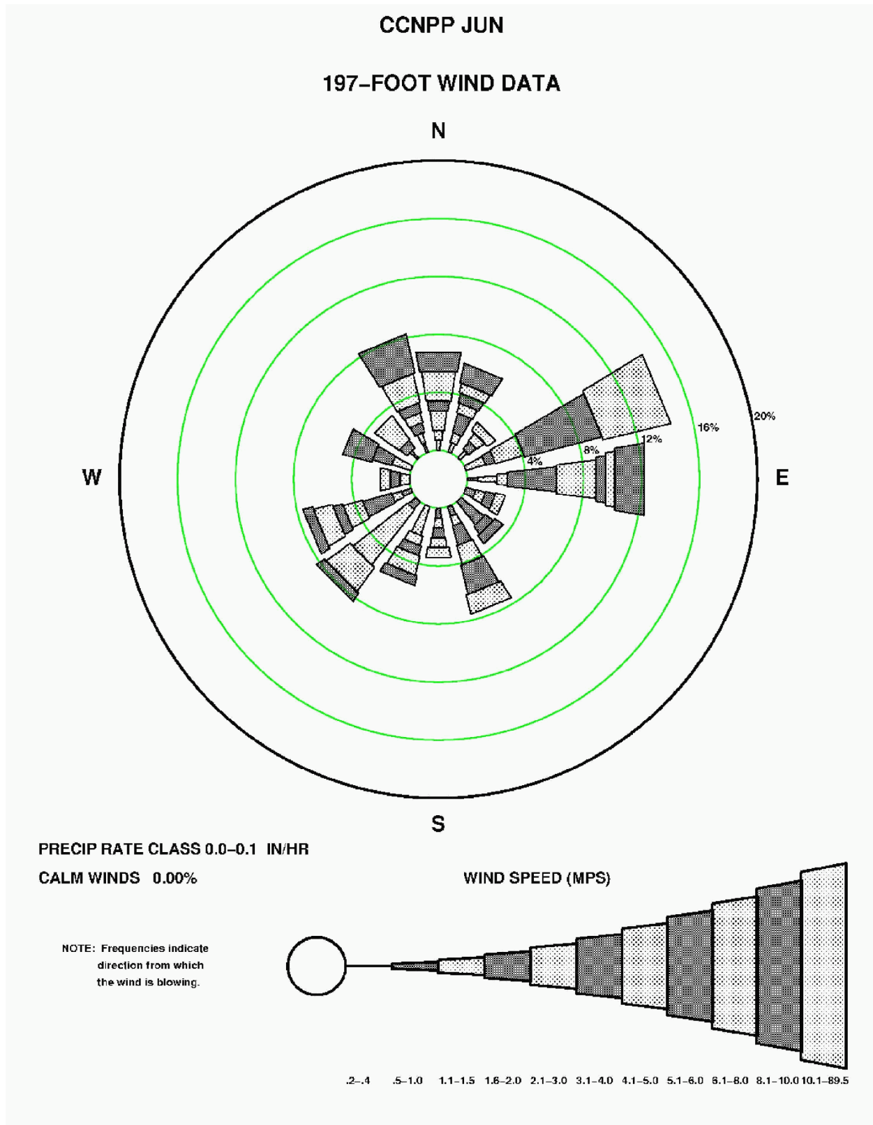
Figure 2.3-161—{CCNPP 197' (60 m) June Precipitation Wind Rose for Rate Class 0.0-0.1 in/hr}
