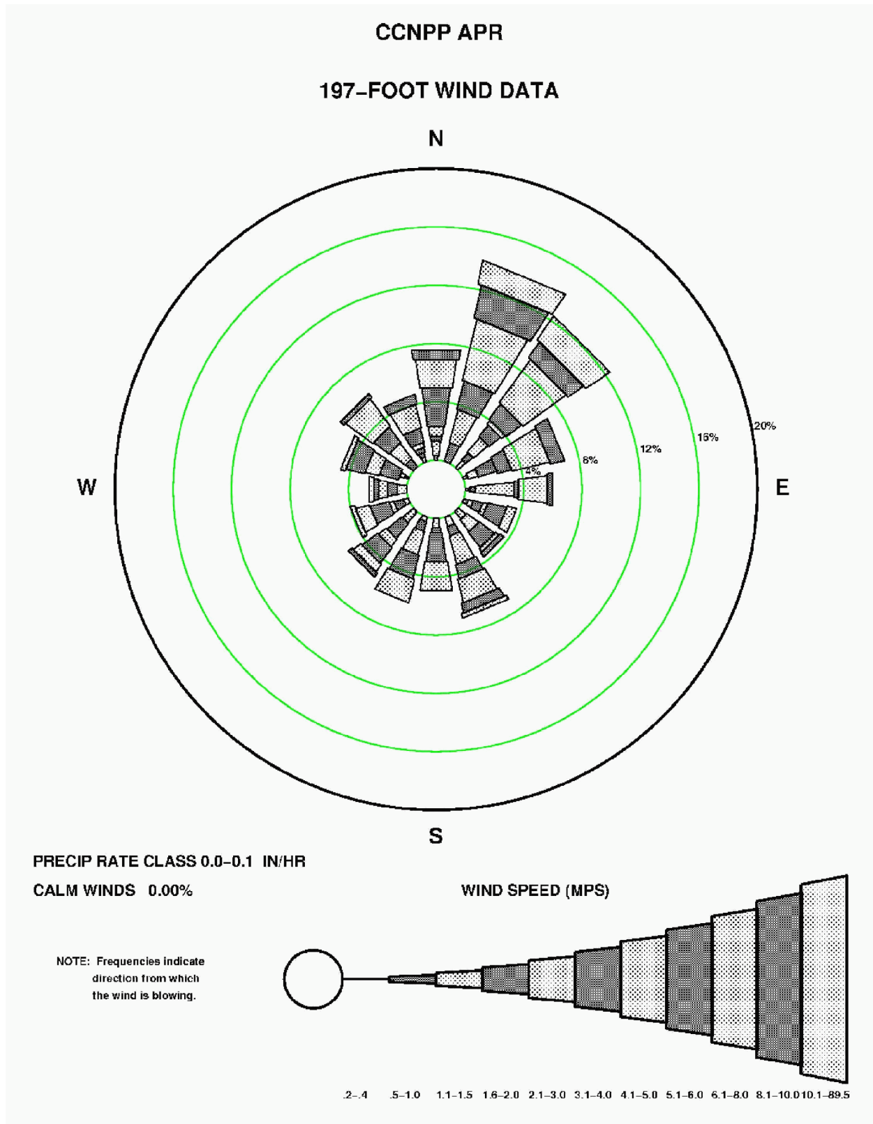
Figure 2.3-146—{CCNPP 197' (60 m) April Precipitation Wind Rose for Rate Class 0.0-0.1 in/hr}
