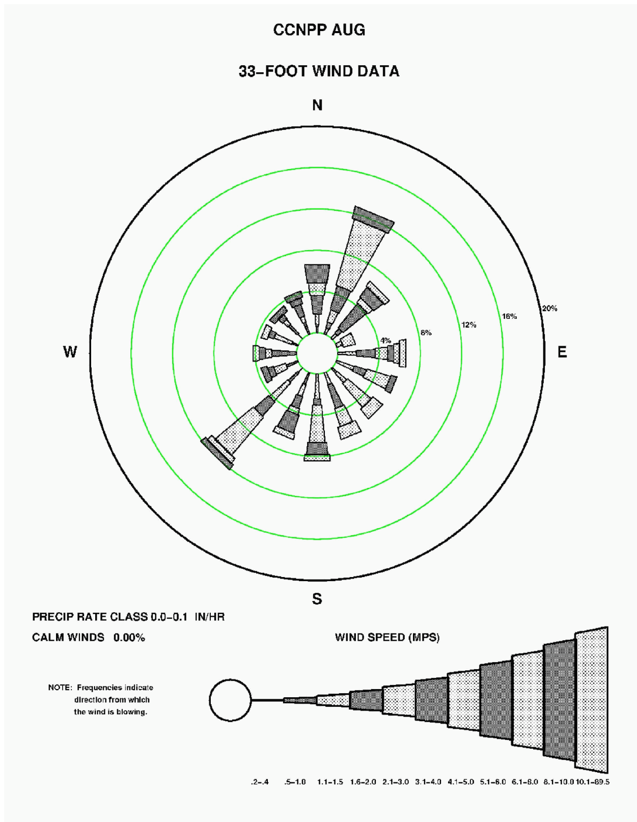
Figure 2.3-94—{CCNPP 33' (10 m) August Precipitation Wind Rose for Rate Class 0.0-0.1 in/hr}
