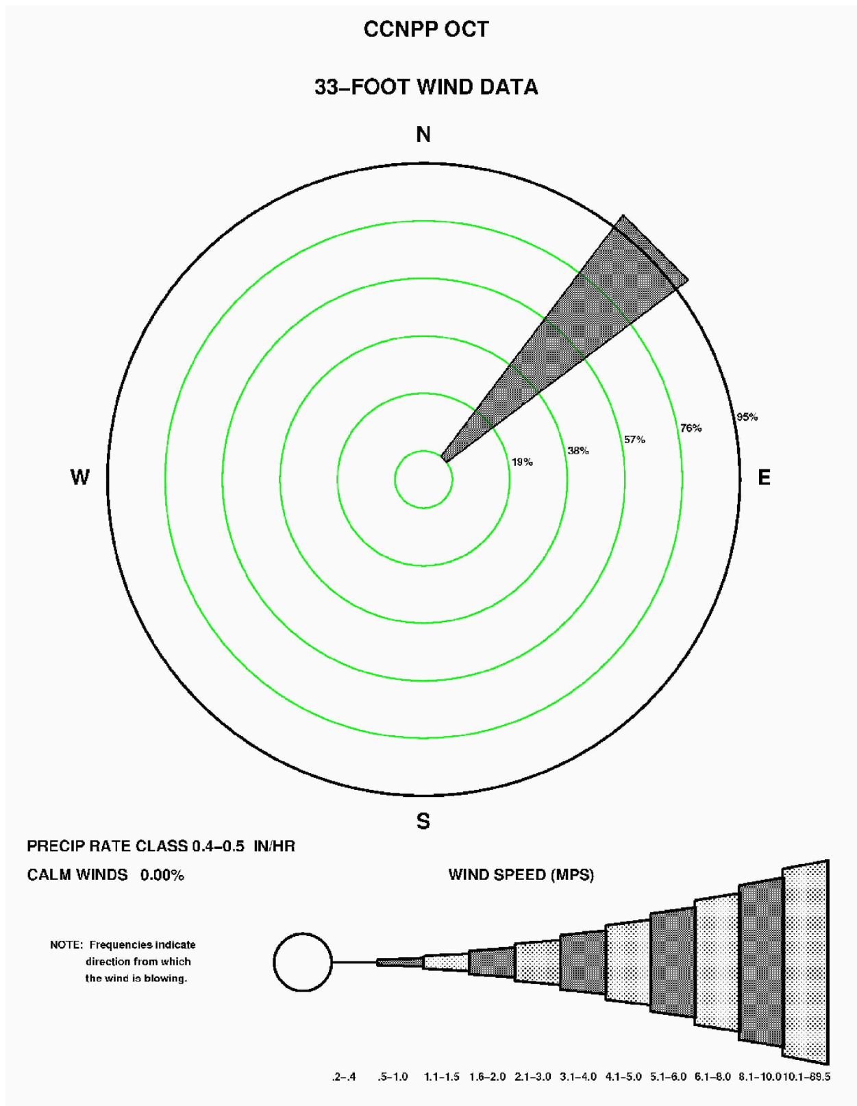
Figure 2.3-115—{CCNPP 33' (10 m) October Precipitation Wind Rose for Rate Class 0.4-0.5 in/hr}
