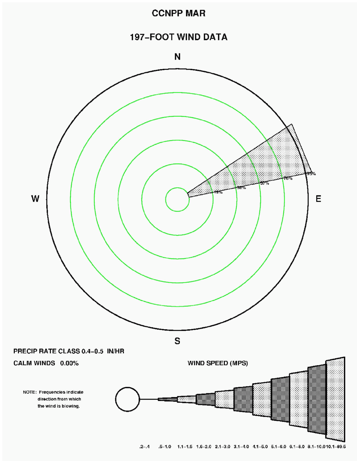
Figure 2.3-144—{CCNPP 197' (60 m) March Precipitation Wind Rose for Rate Class 0.4-0.5 in/hr}
