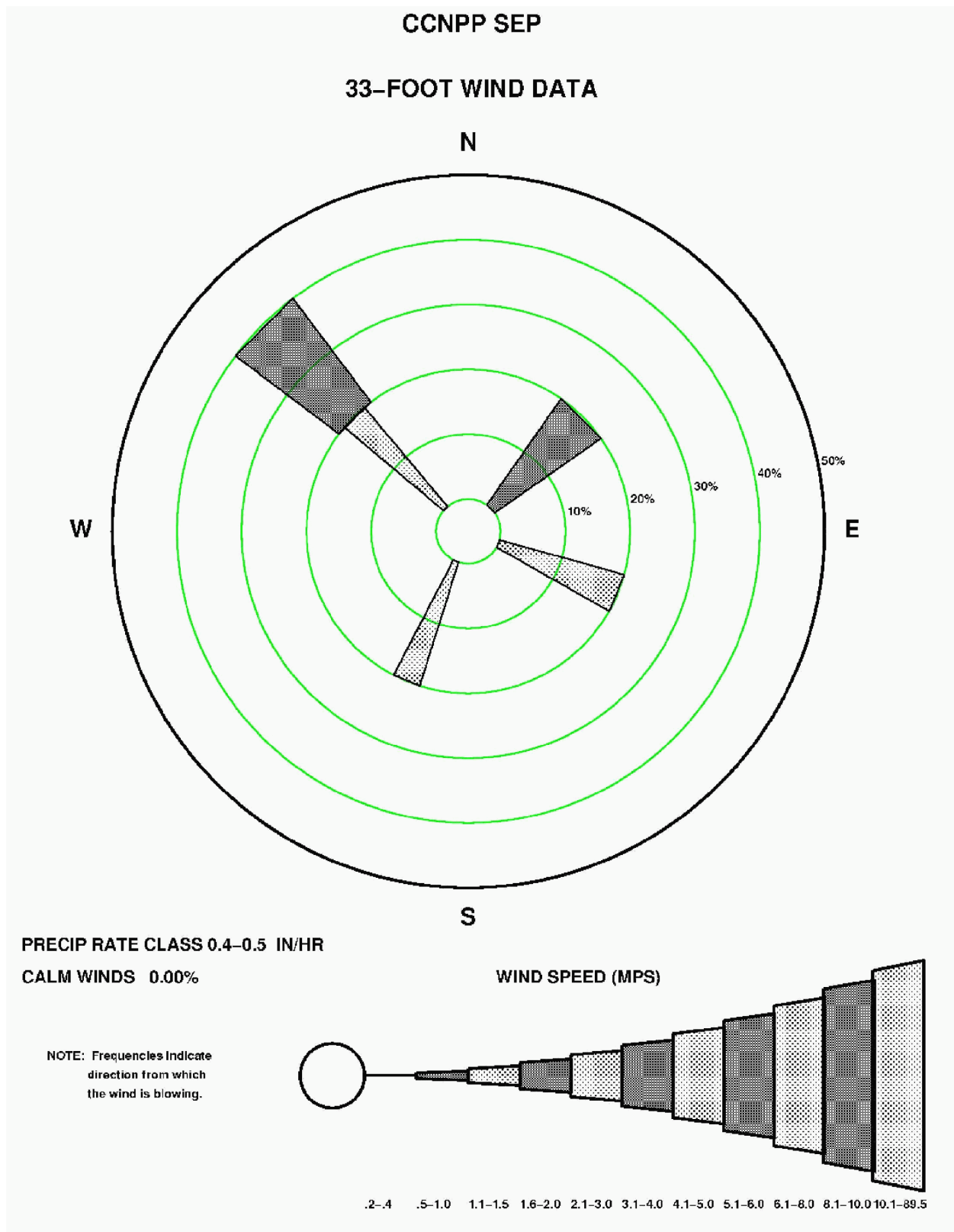
Figure 2.3-106—{CCNPP 33' (10 m) September Precipitation Wind Rose for Rate Class 0.4-0.5 in/hr}
