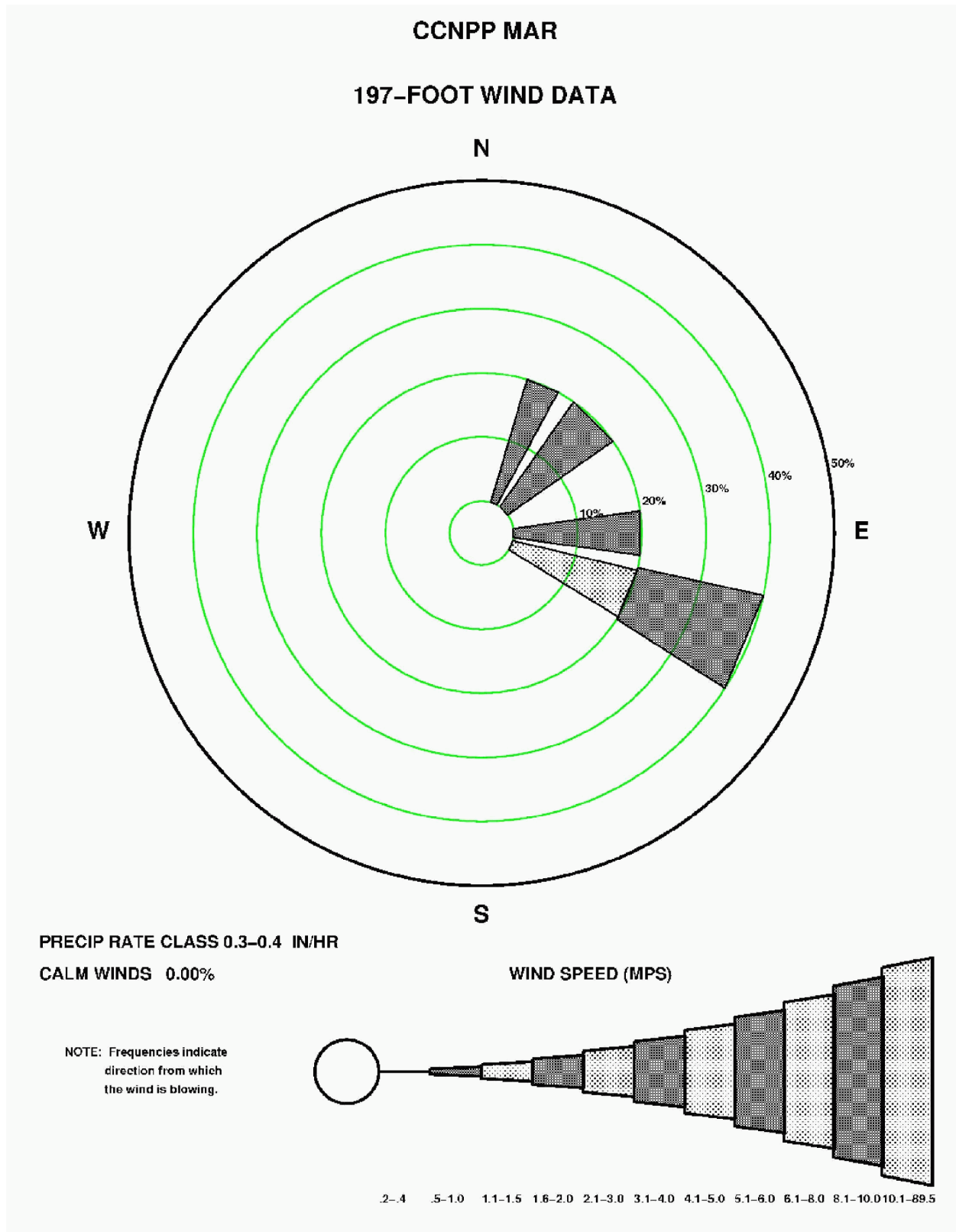
Figure 2.3-143—{CCNPP 197' (60 m) March Precipitation Wind Rose for Rate Class 0.3-0.4 in/hr}
