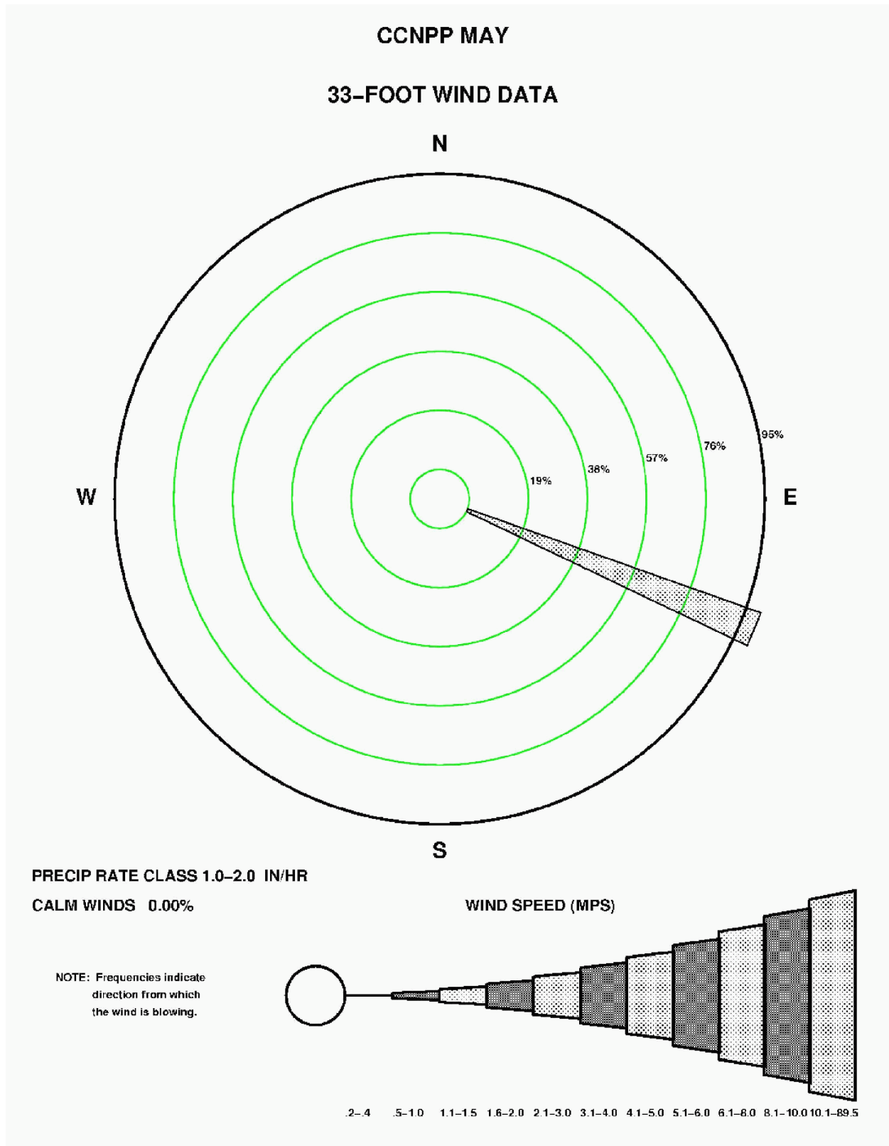
Figure 2.3-75—{CCNPP 33' (10 m) May Precipitation Wind Rose for Rate Class 1.0-2.0 in/hr}
