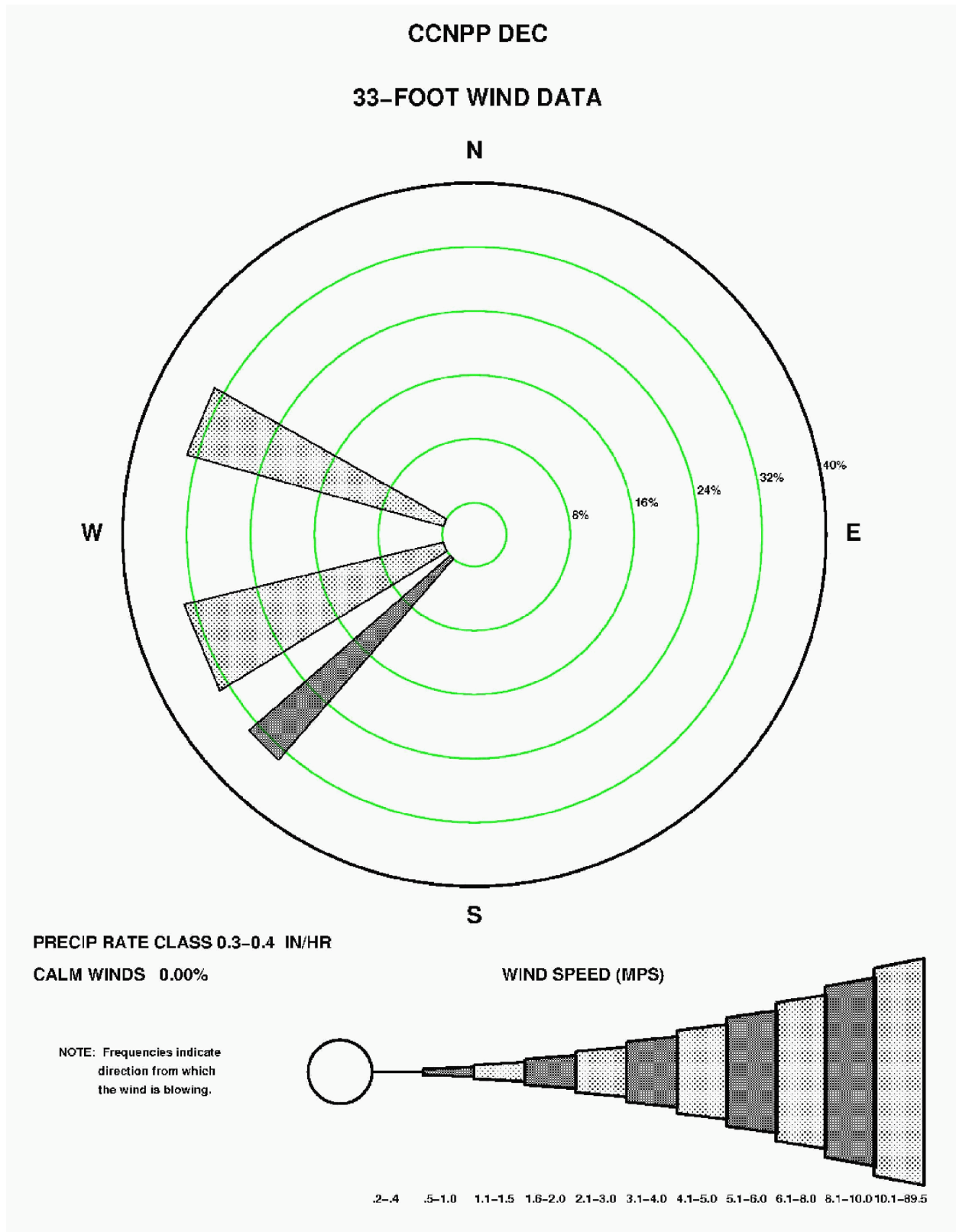
Figure 2.3-127—{CCNPP 33' (10 m) December Precipitation Wind Rose for Rate Class 0.3-0.4 in/hr}
