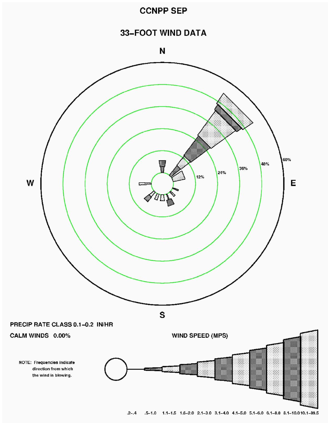
Figure 2.3-103—{CCNPP 33' (10 m) September Precipitation Wind Rose for Rate Class 0.1-0.2 in/hr}
