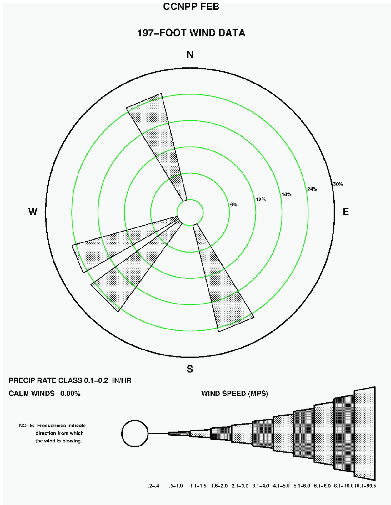
Figure 2.3-136—{CCNPP 197' (60 m) February Precipitation Wind Rose for Rate Class 0.1-0.2 in/hr}
