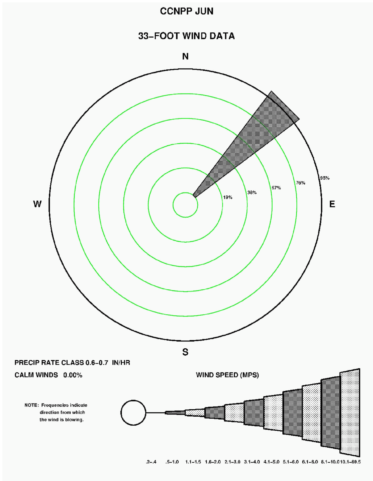
Figure 2.3-82—{CCNPP 33' (10 m) June Precipitation Wind Rose for Rate Class 0.6-0.7 in/hr}
