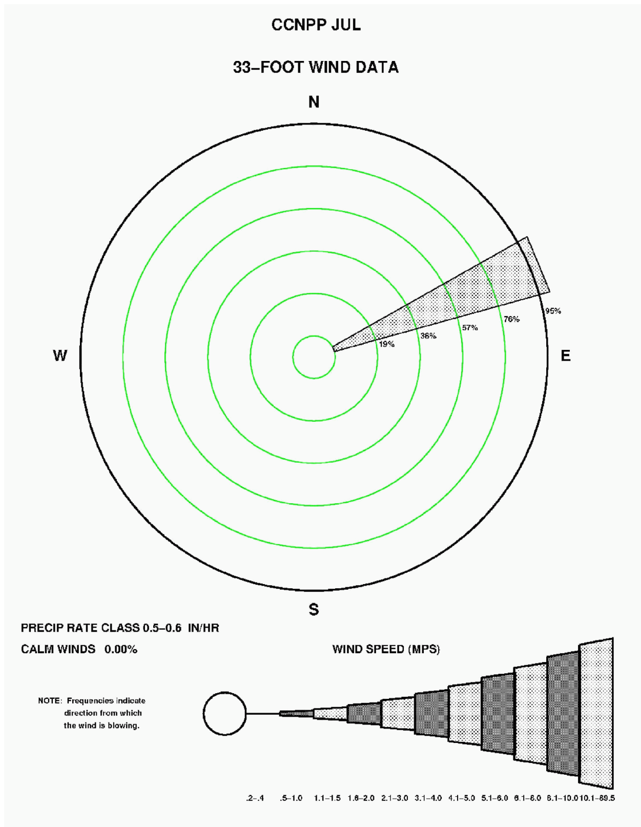
Figure 2.3-90—{CCNPP 33' (10 m) July Precipitation Wind Rose for Rate Class 0.5-0.6 in/hr}
