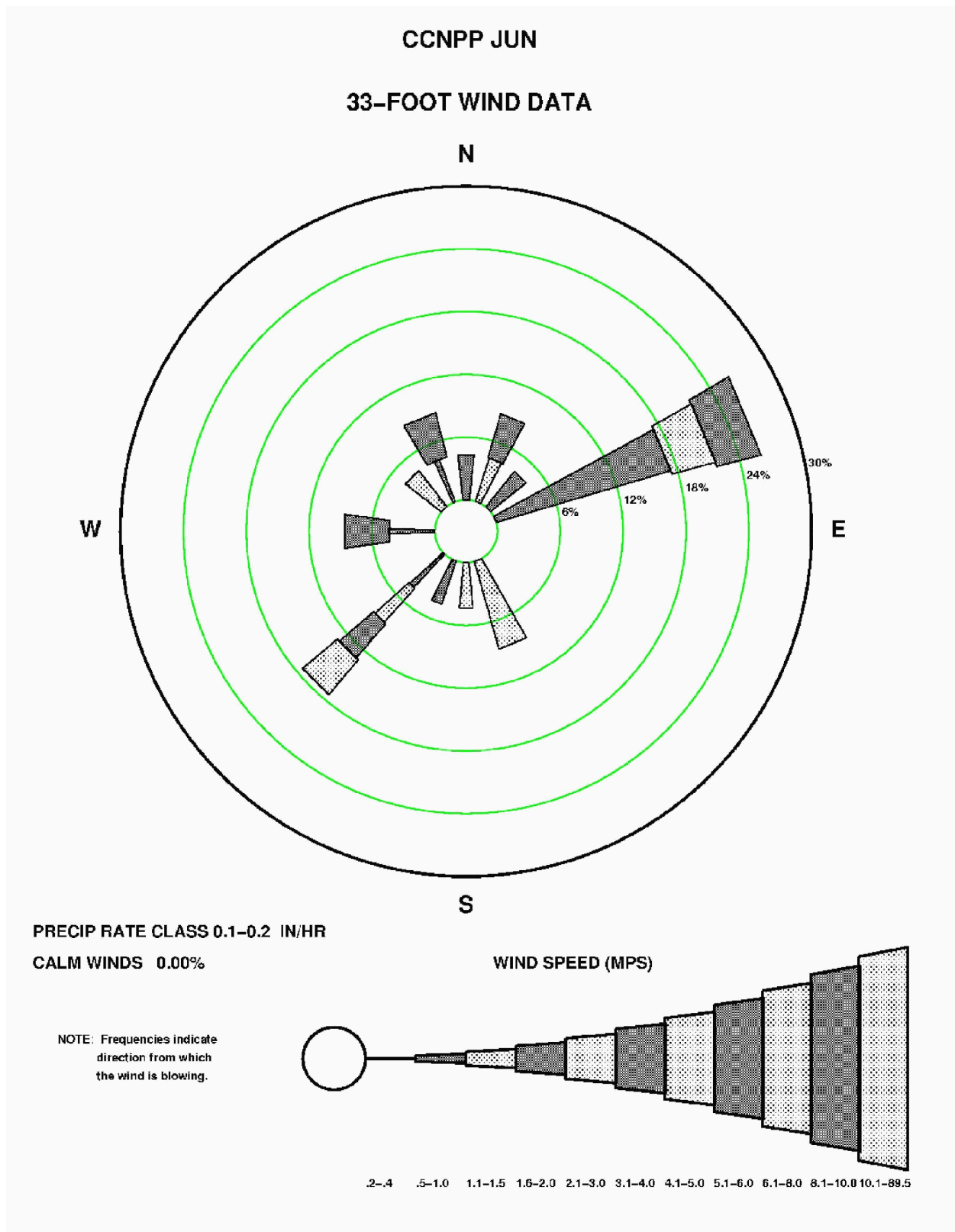
Figure 2.3-78—{CCNPP 33' (10 m) June Precipitation Wind Rose for Rate Class 0.1-0.2 in/hr}
