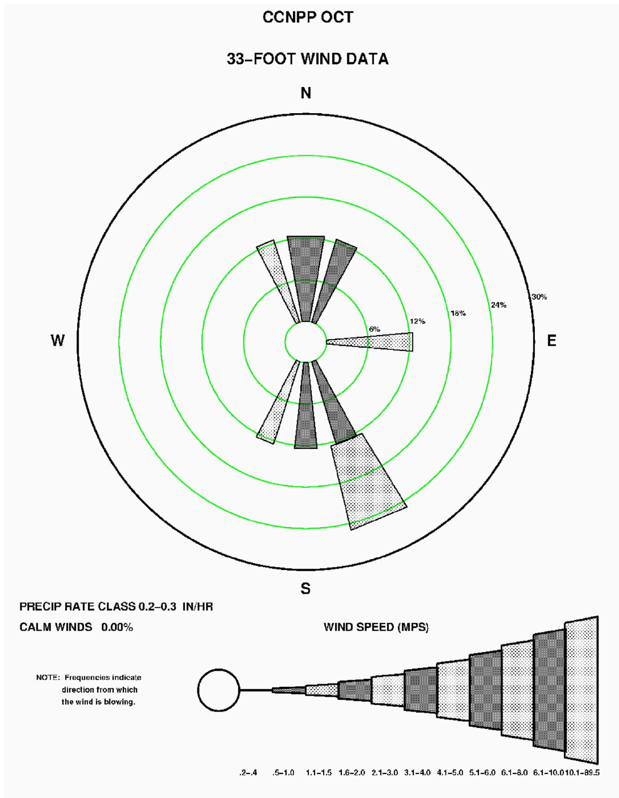
Figure 2.3-113—{CCNPP 33' (10 m) October Precipitation Wind Rose for Rate Class 0.2-0.3 in/hr}
