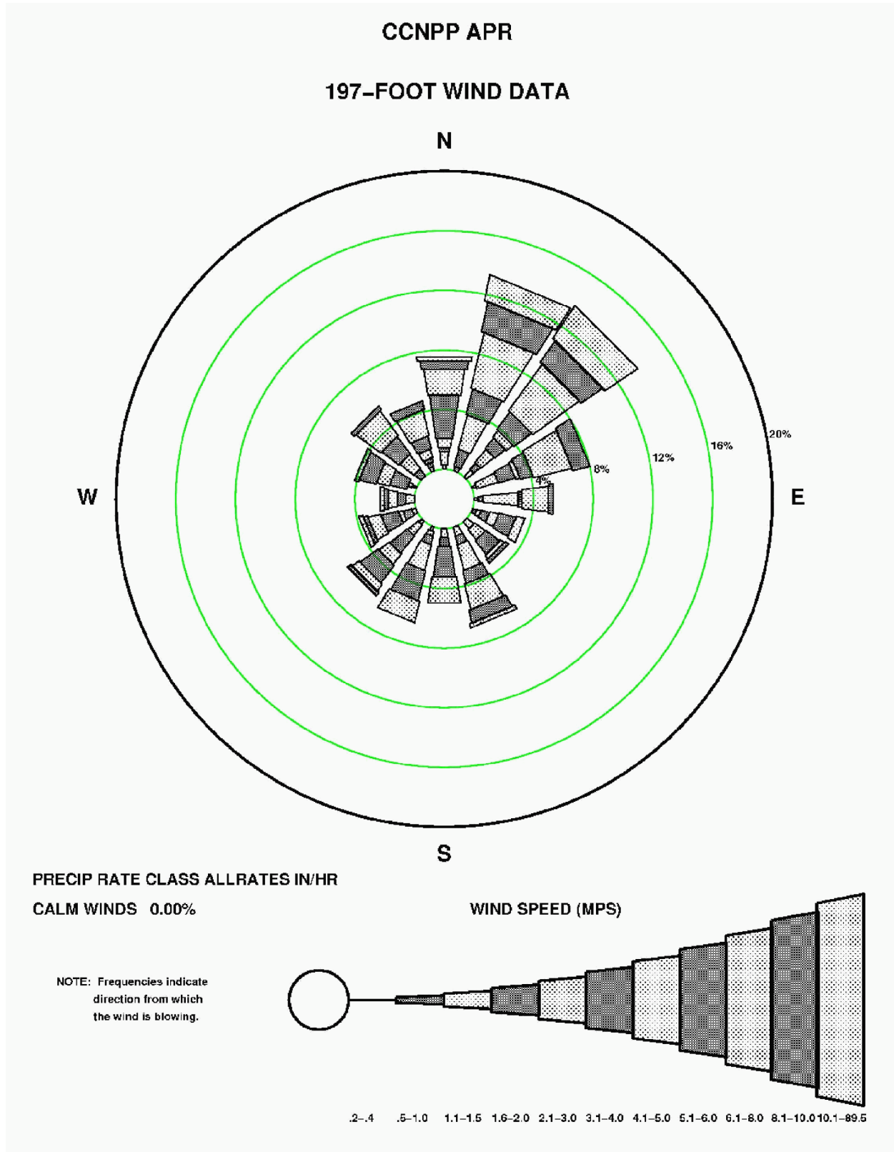
Figure 2.3-152—{CCNPP 197' (60 m) April Precipitation Wind Rose for All Rate classes}
