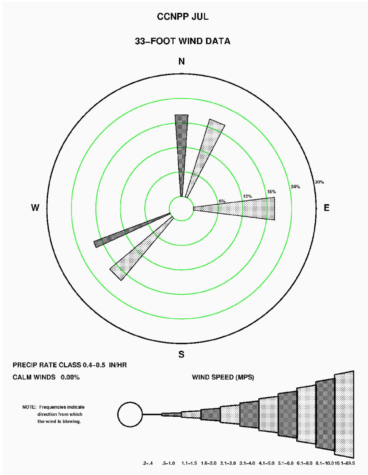
Figure 2.3-89—{CCNPP 33' (10 m) July Precipitation Wind Rose for Rate Class 0.4-0.5 in/hr}
