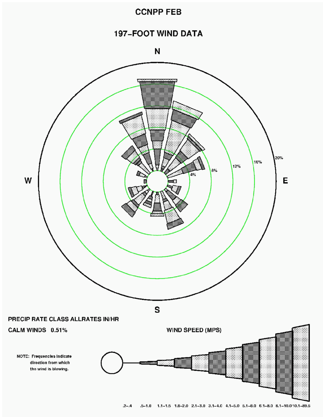
Figure 2.3-139—{CCNPP 197' (60 m) February Precipitation Wind Rose for All Rate classes}
