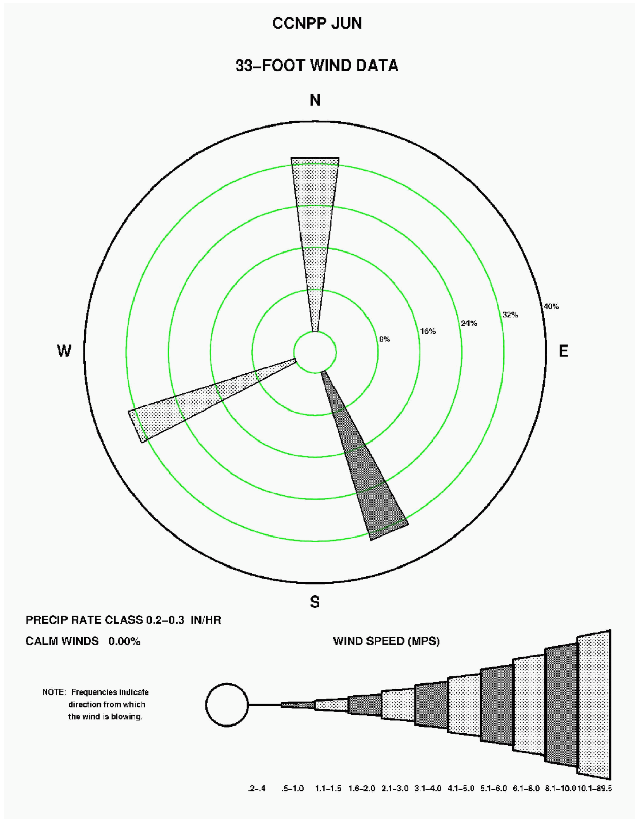
Figure 2.3-79—{CCNPP 33' (10 m) June Precipitation Wind Rose for Rate Class 0.2-0.3 in/hr}
