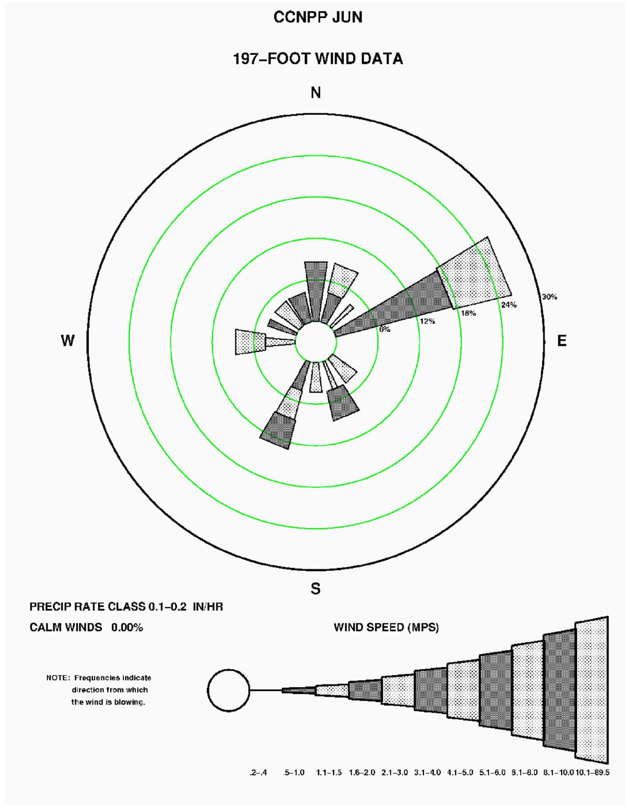
Figure 2.3-162—{CCNPP 197' (60 m) June Precipitation Wind Rose for Rate Class 0.1-0.2 in/hr}
