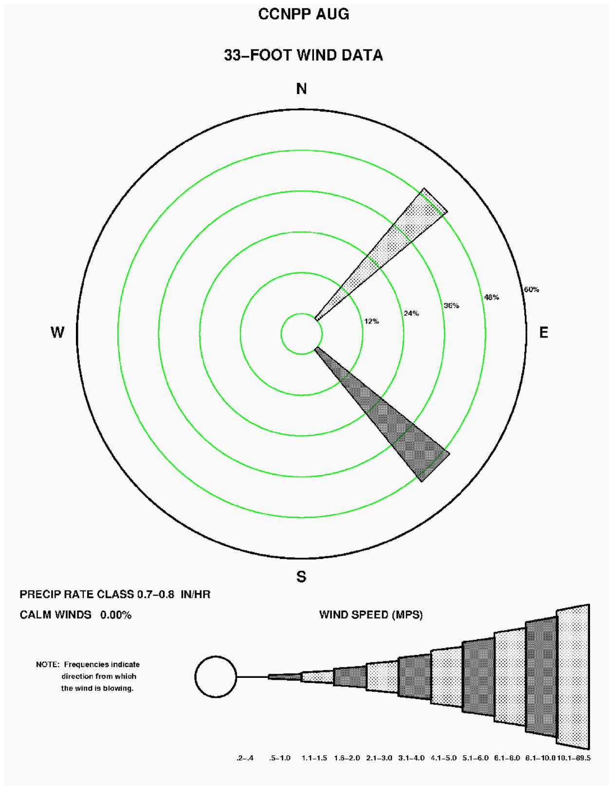
Figure 2.3-100—{CCNPP 33' (10 m) August Precipitation Wind Rose for Rate Class 0.7-0.8 in/hr}
