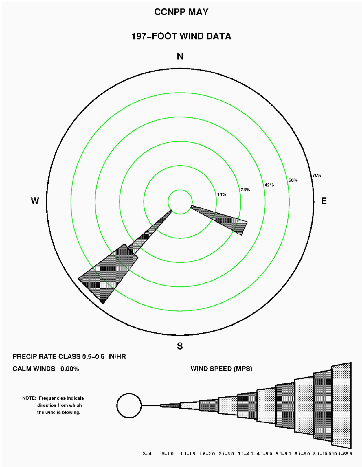
Figure 2.3-157—{CCNPP 197' (60 m) May Precipitation Wind Rose for Rate Class 0.5-0.6 in/hr}
