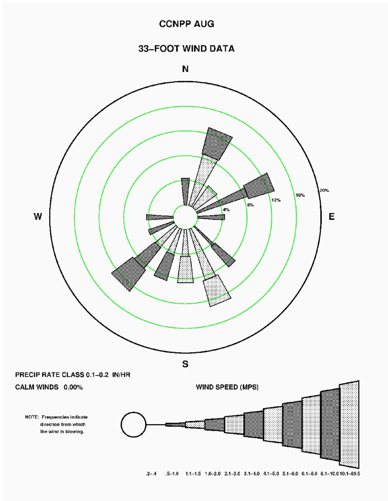
Figure 2.3-95—{CCNPP 33' (10 m) August Precipitation Wind Rose for Rate Class 0.1-0.2 in/hr}
