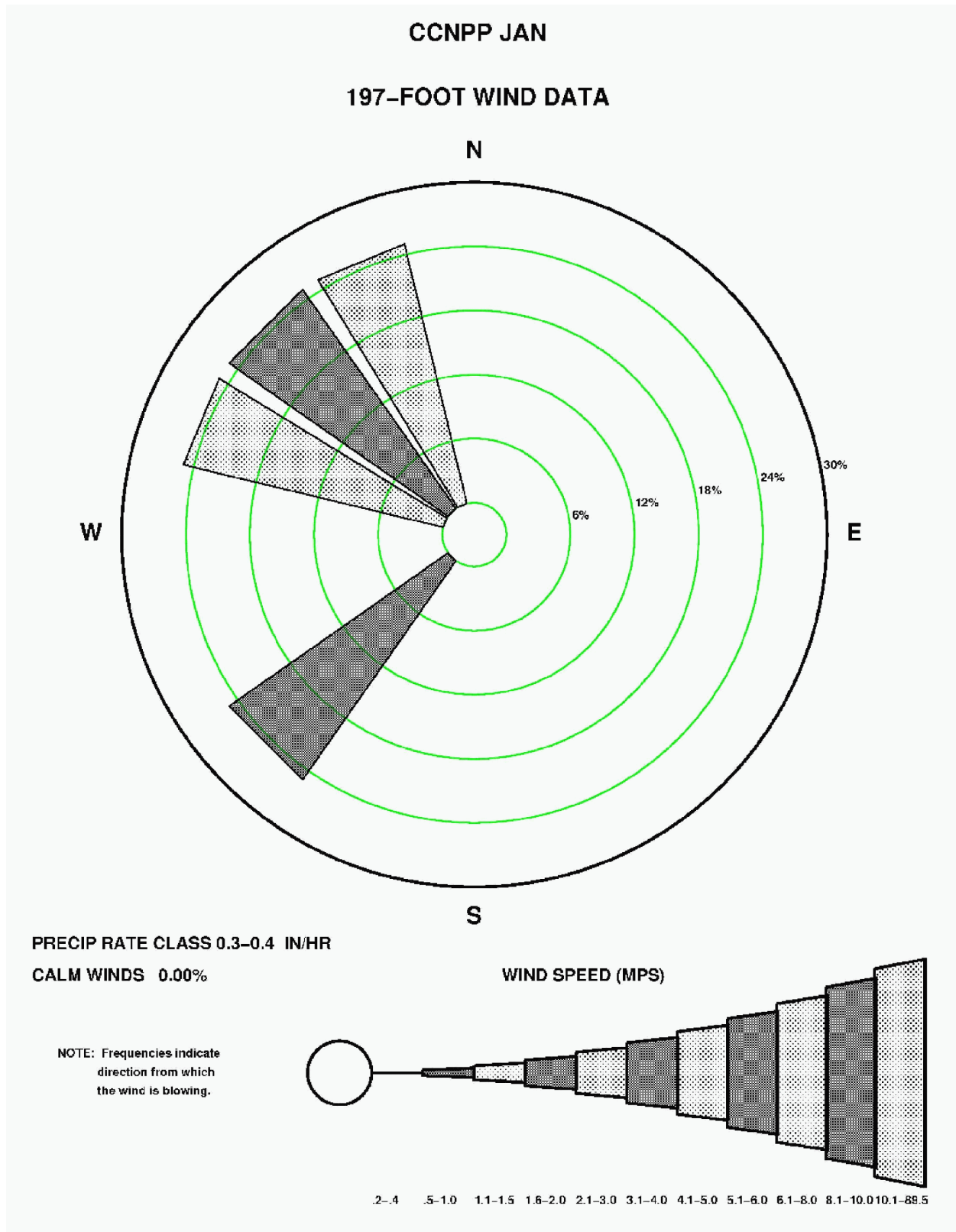
Figure 2.3-132—{CCNPP 197' (60 m) January Precipitation Wind Rose for Rate Class 0.3-0.4 in/hr}
