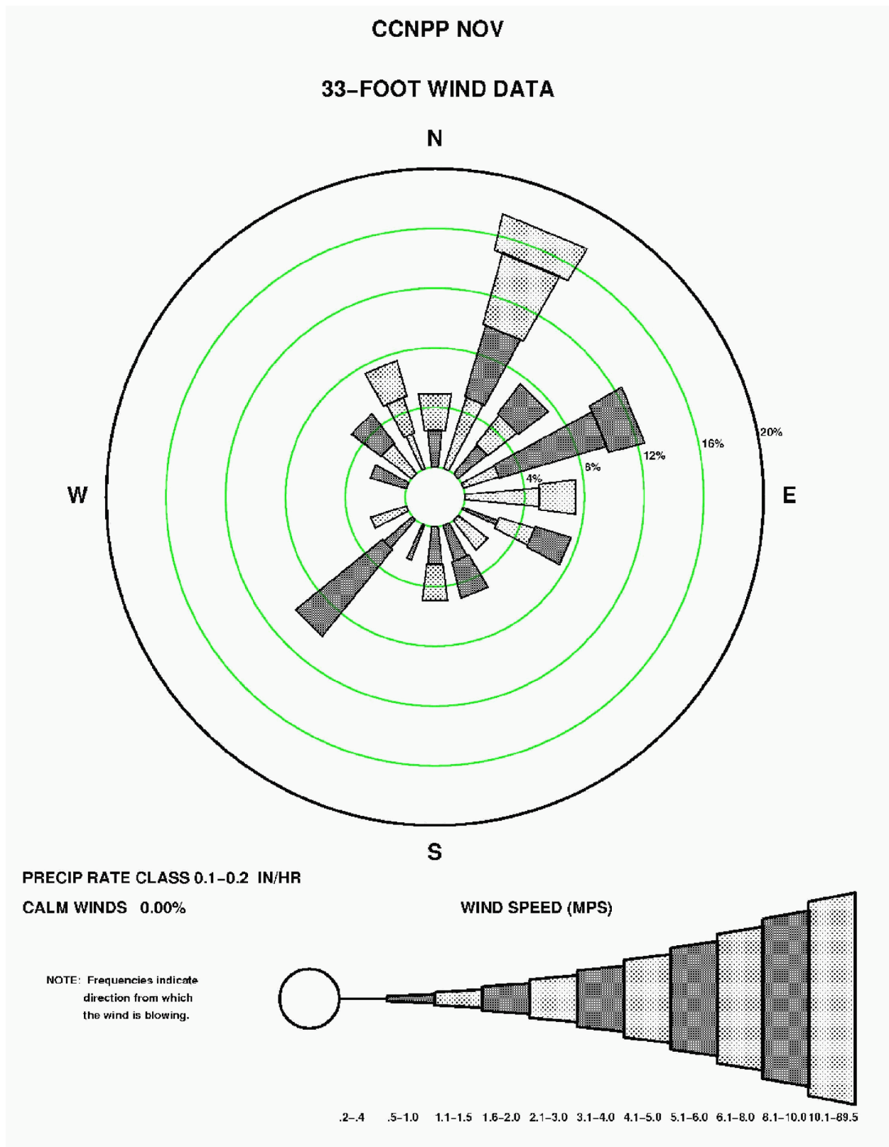
Figure 2.3-119—{CCNPP 33' (10 m) November Precipitation Wind Rose for Rate Class 0.1-0.2 in/hr}
