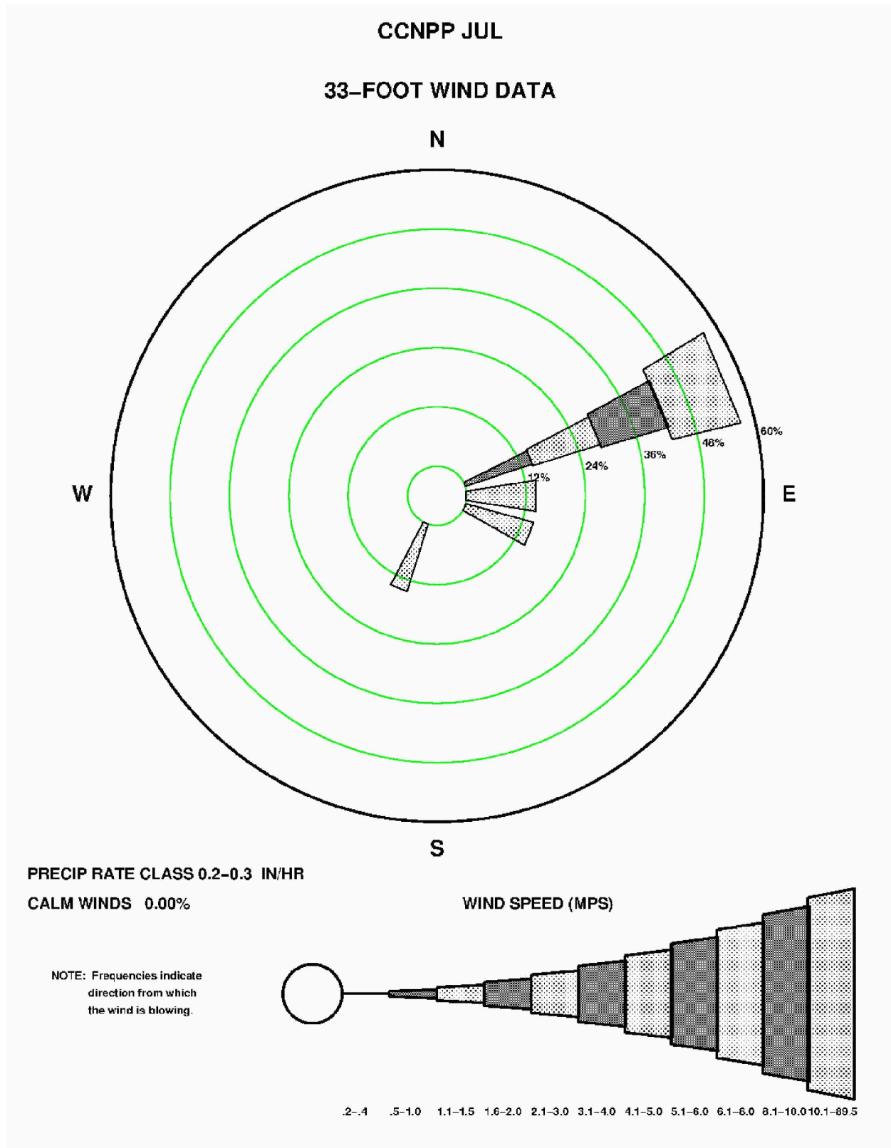
Figure 2.3-87—{CCNPP 33' (10 m) July Precipitation Wind Rose for Rate Class 0.2-0.3 in/hr}
