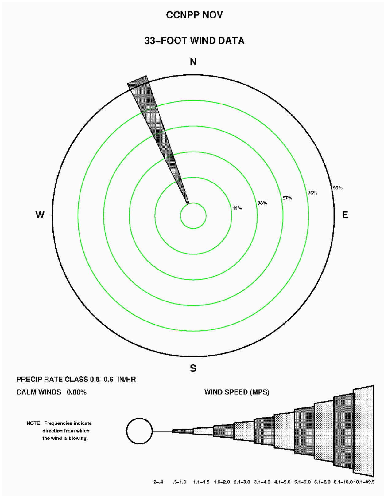
Figure 2.3-122—{CCNPP 33' (10 m) November Precipitation Wind Rose for Rate Class 0.5-0.6 in/hr}
