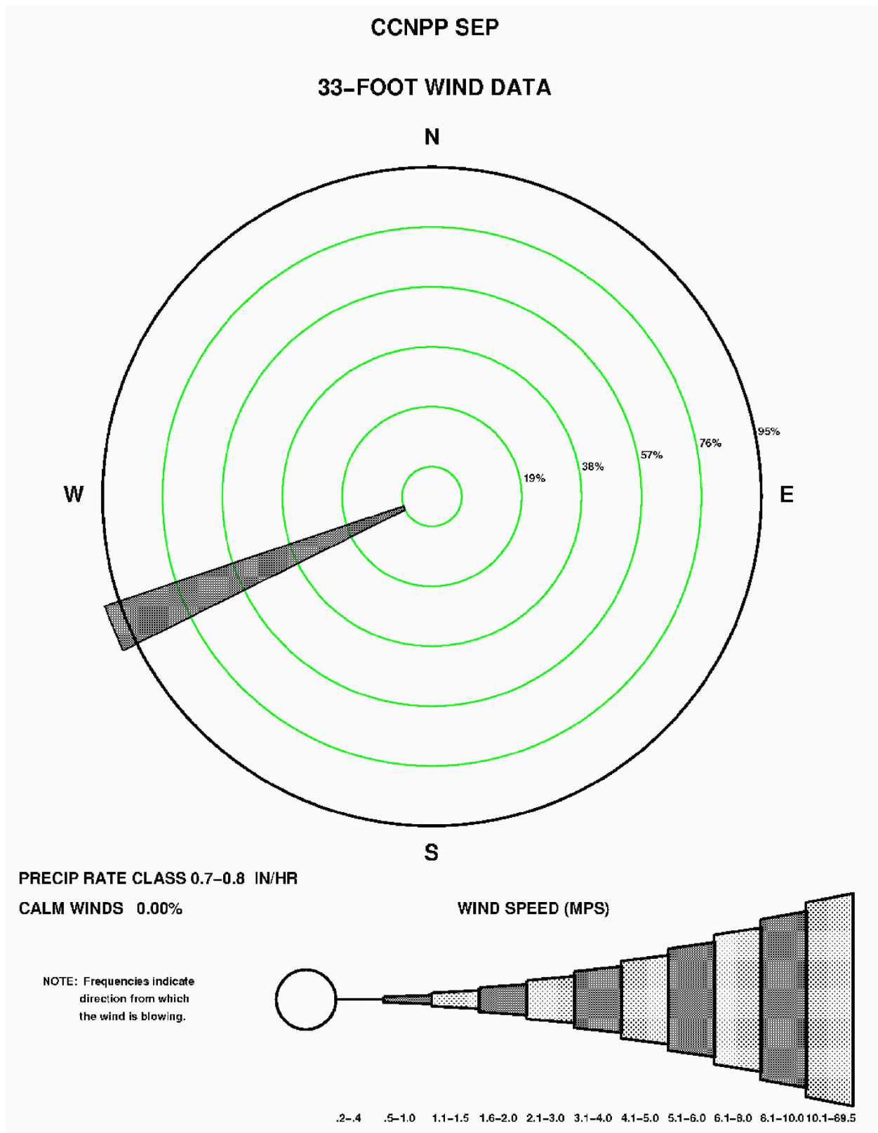
Figure 2.3-109—{CCNPP 33' (10 m) September Precipitation Wind Rose for Rate Class 0.7-0.8 in/hr}
