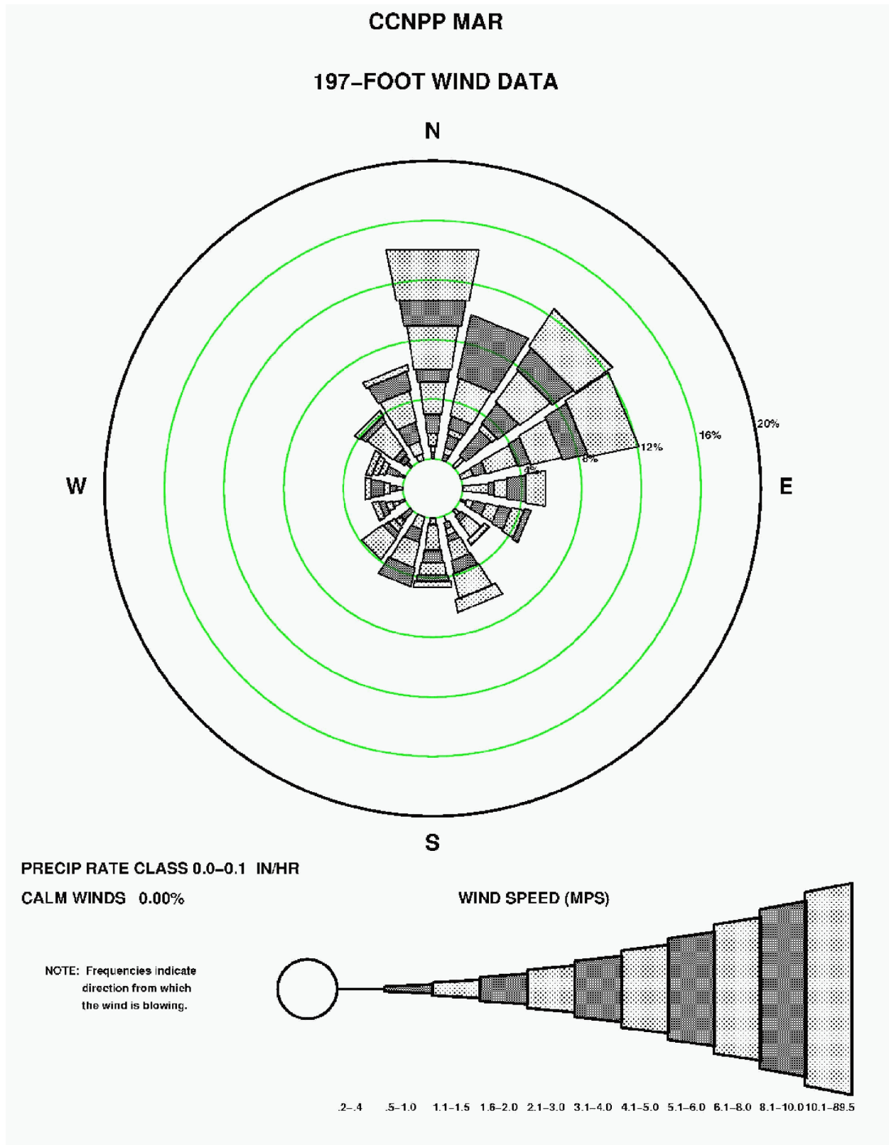
Figure 2.3-140—{CCNPP 197' (60 m) March Precipitation Wind Rose for Rate Class 0.0-0.1 in/hr}
