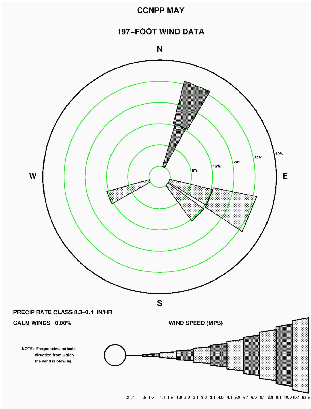
Figure 2.3-156—{CCNPP 197' (60 m) May Precipitation Wind Rose for Rate Class 0.3-0.4 in/hr}
