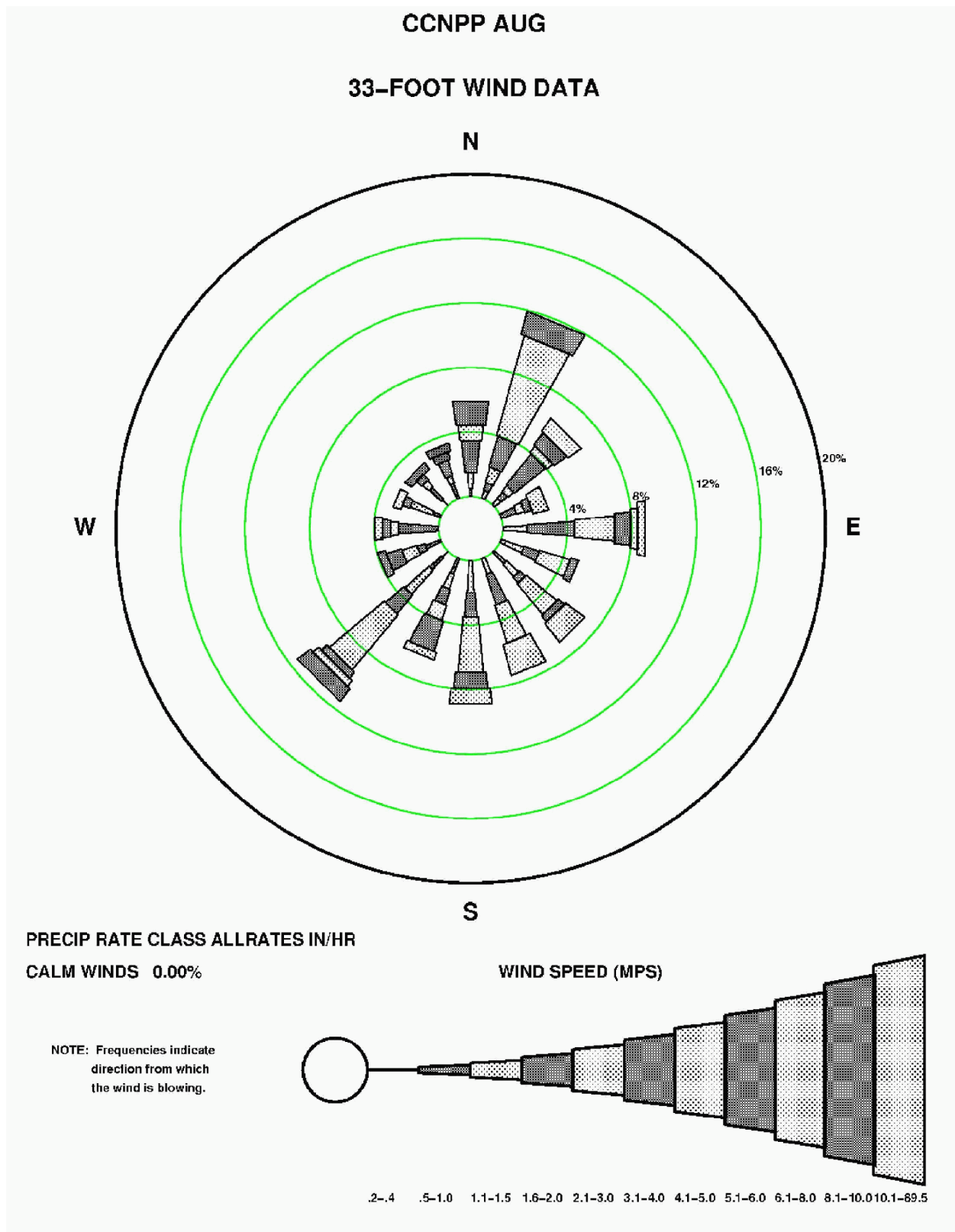
Figure 2.3-101—{CCNPP 33' (10 m) August Precipitation Wind Rose for All Rate classes}
