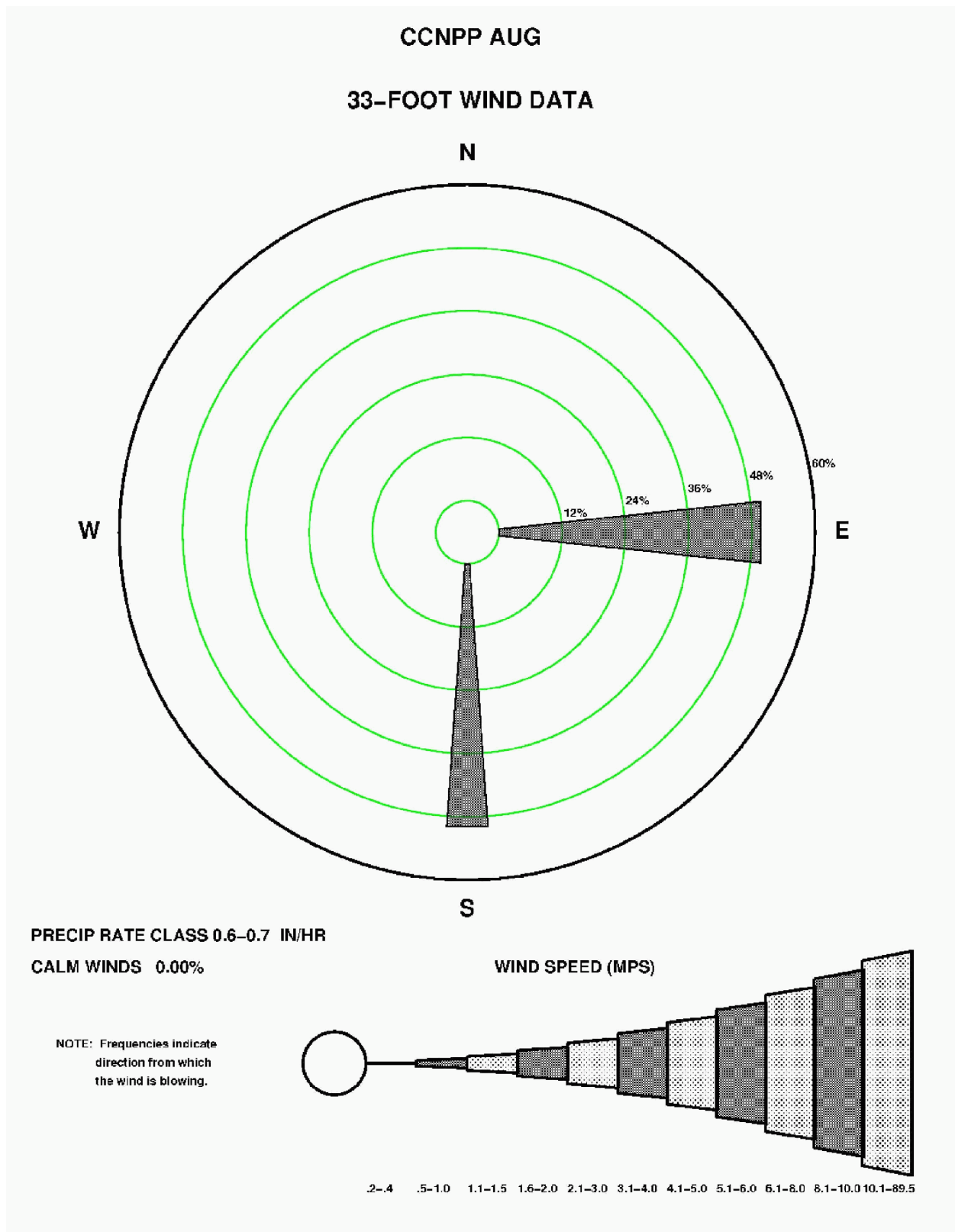
Figure 2.3-99—{CCNPP 33' (10 m) August Precipitation Wind Rose for Rate Class 0.6-0.7 in/hr}
