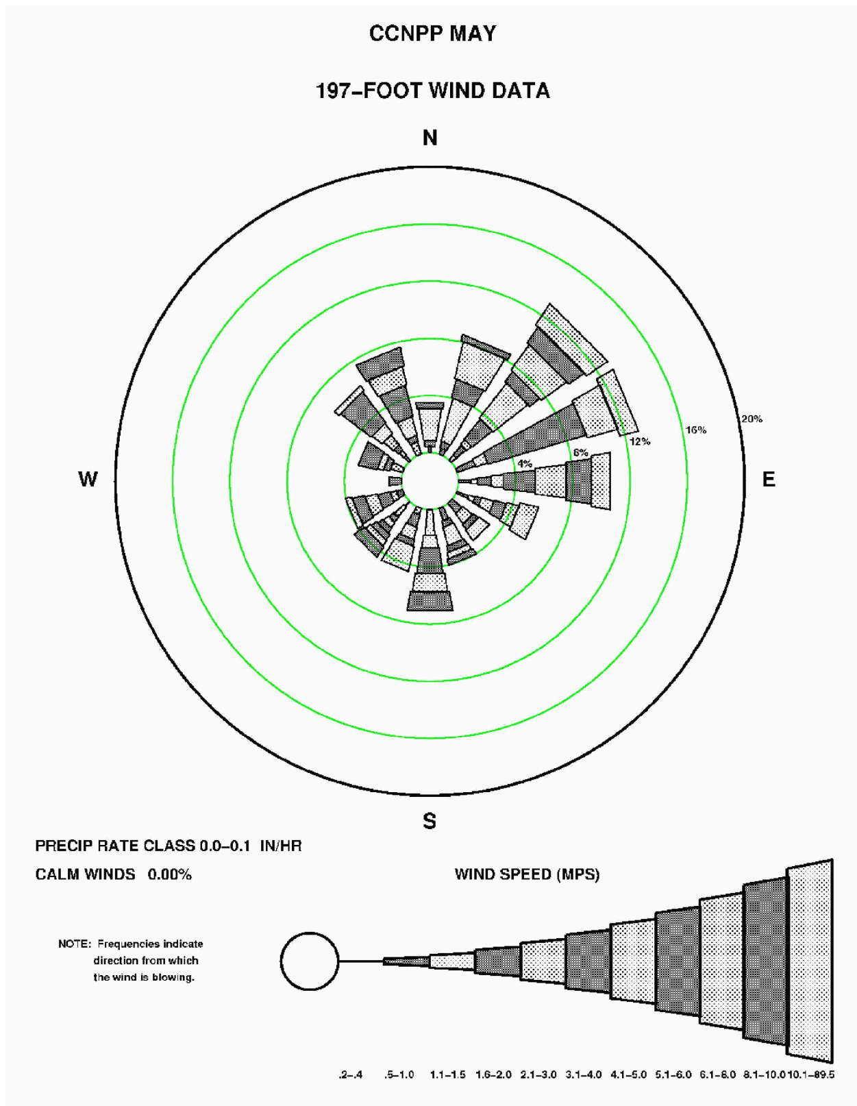
Figure 2.3-153—{CCNPP 197' (60 m) May Precipitation Wind Rose for Rate Class 0.0-0.1 in/hr}
