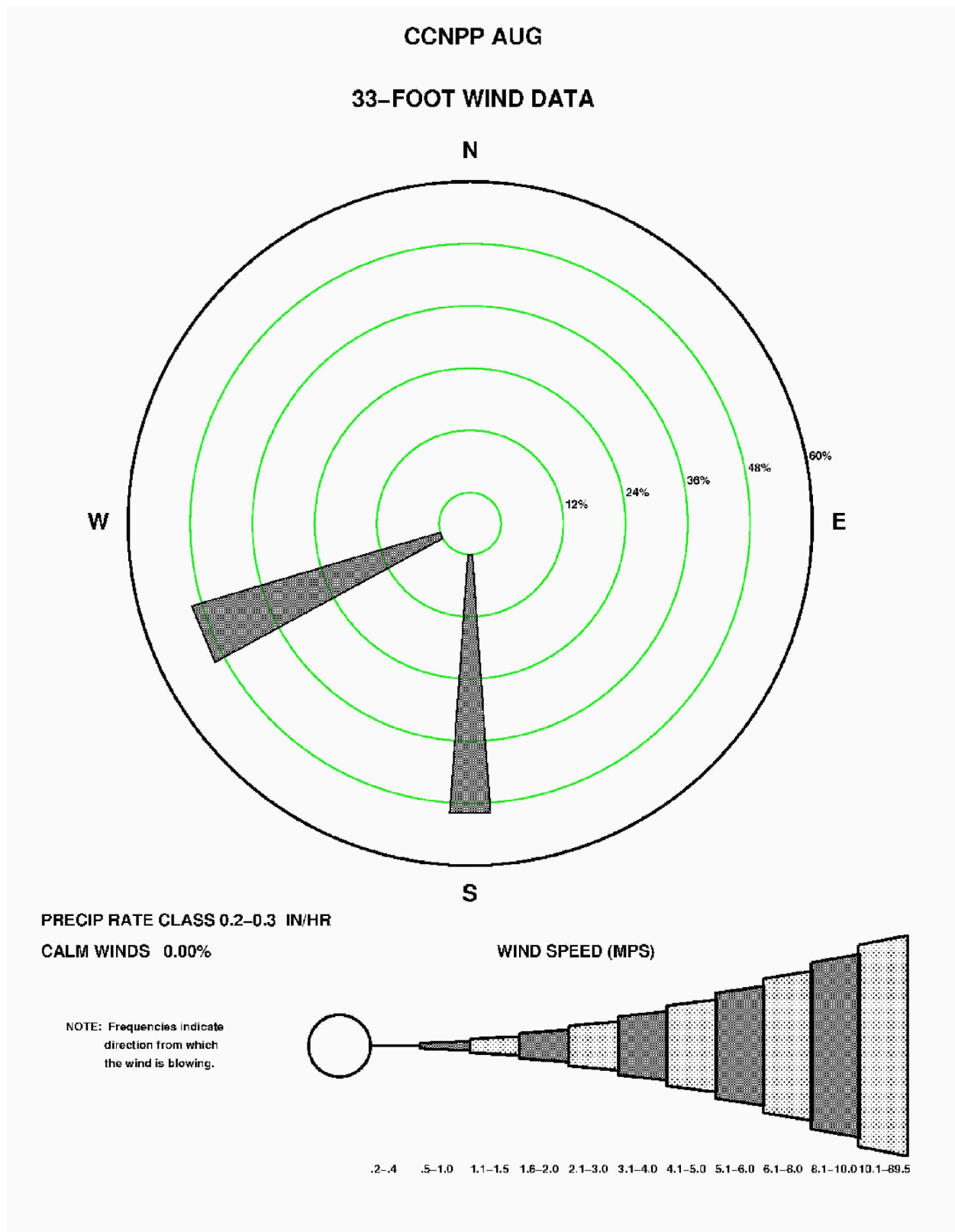
Figure 2.3-96—{CCNPP 33' (10 m) August Precipitation Wind Rose for Rate Class 0.2-0.3 in/hr}
