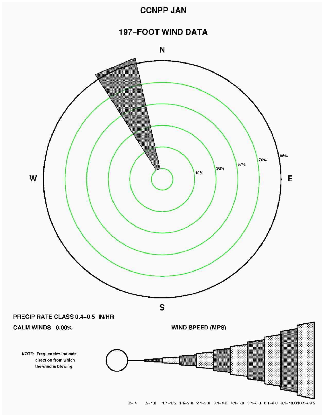
Figure 2.3-133—{CCNPP 197' (60 m) January Precipitation Wind Rose for Rate Class 0.4-0.5 in/hr}
