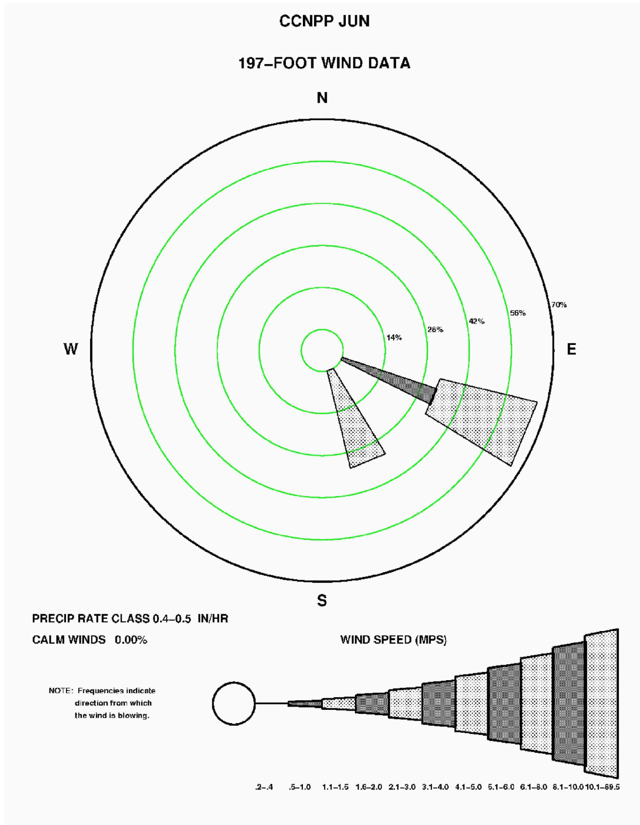
Figure 2.3-165—{CCNPP 197' (60 m) June Precipitation Wind Rose for Rate Class 0.4-0.5 in/hr}
