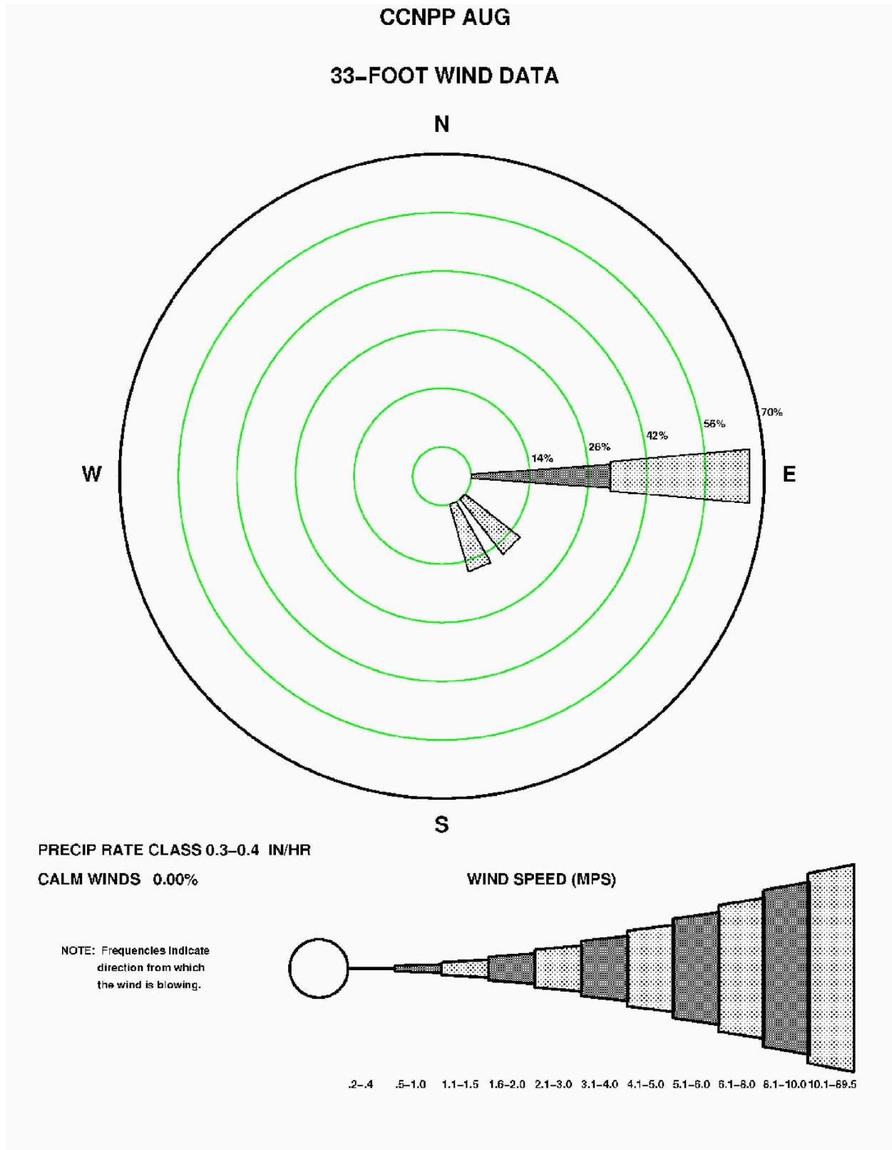
Figure 2.3-97—{CCNPP 33' (10 m) August Precipitation Wind Rose for Rate Class 0.3-0.4 in/hr}
