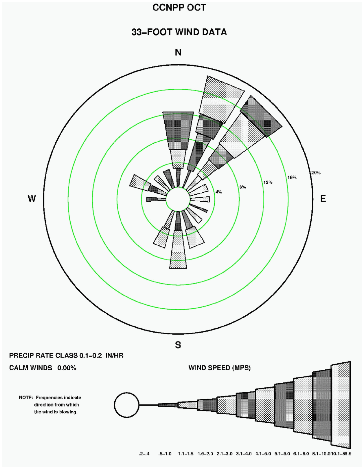
Figure 2.3-112—{CCNPP 33' (10m) October Precipitation Wind Rose for Rate Class 0.1-0.2 in/hr}
