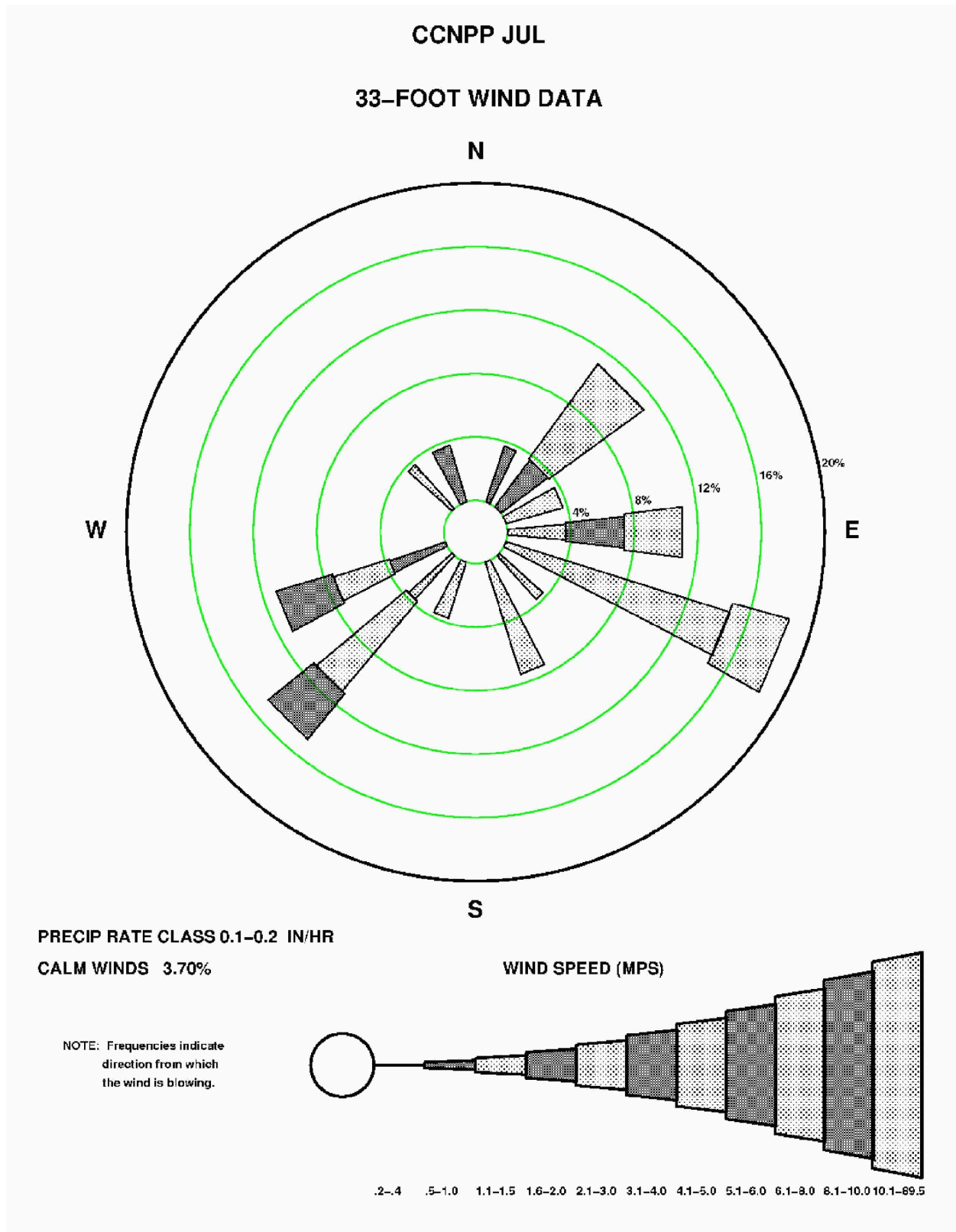
Figure 2.3-86—{CCNPP 33' (10 m) July Precipitation Wind Rose for Rate Class 0.1-0.2 in/hr}
