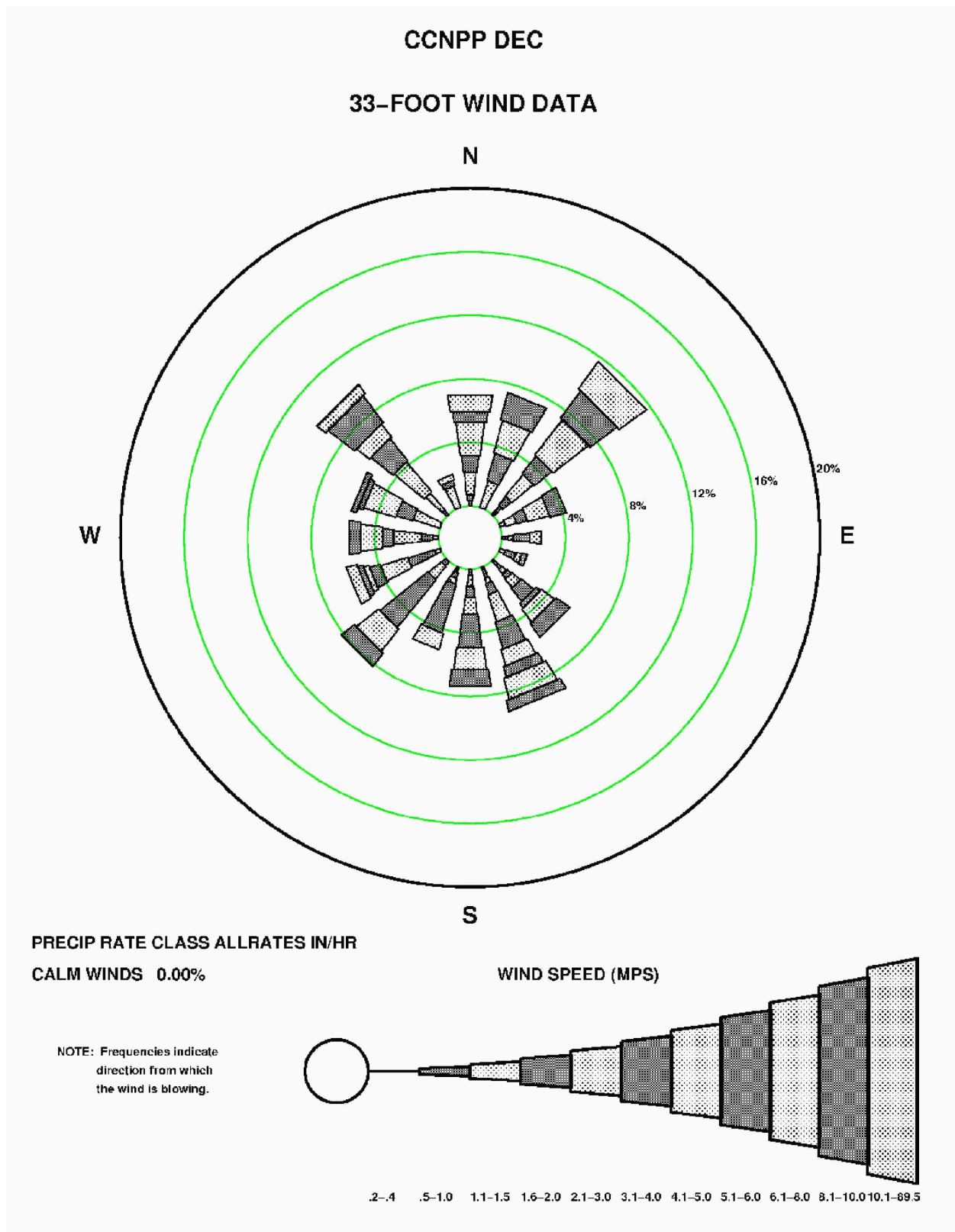
Figure 2.3-128—{CCNPP 33' (10 m) December Precipitation Wind Rose for All Rate classes}
