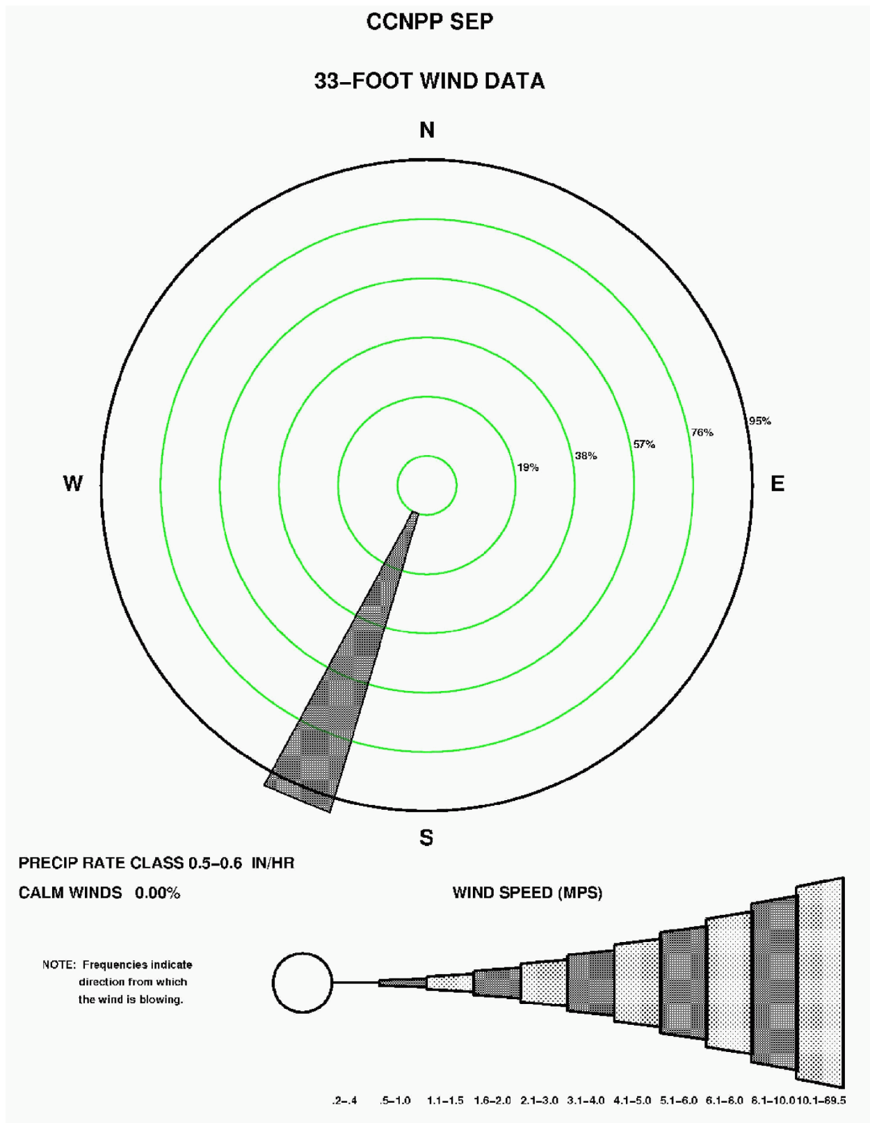
Figure 2.3-107—{CCNPP 33' (10 m) September Precipitation Wind Rose for Rate Class 0.5-0.6 in/hr}
