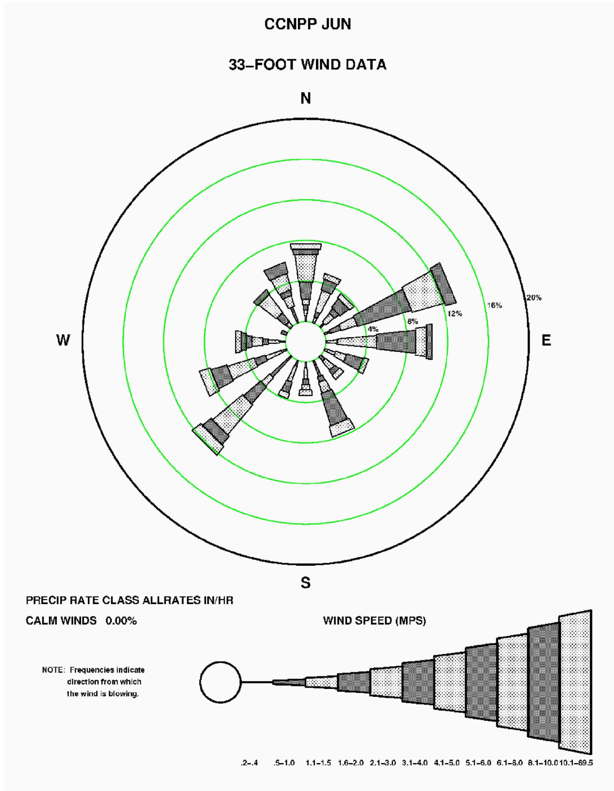
Figure 2.3-84—{CCNPP 33' (10 m) June Precipitation Wind Rose for All Rate classes}
