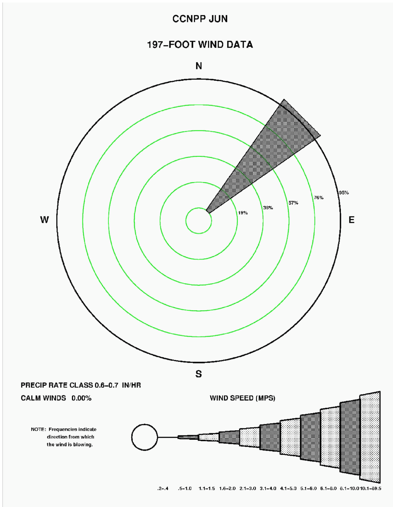
Figure 2.3-166—{CCNPP 197' (60 m) June Precipitation Wind Rose for Rate Class 0.6-0.7 in/hr}
