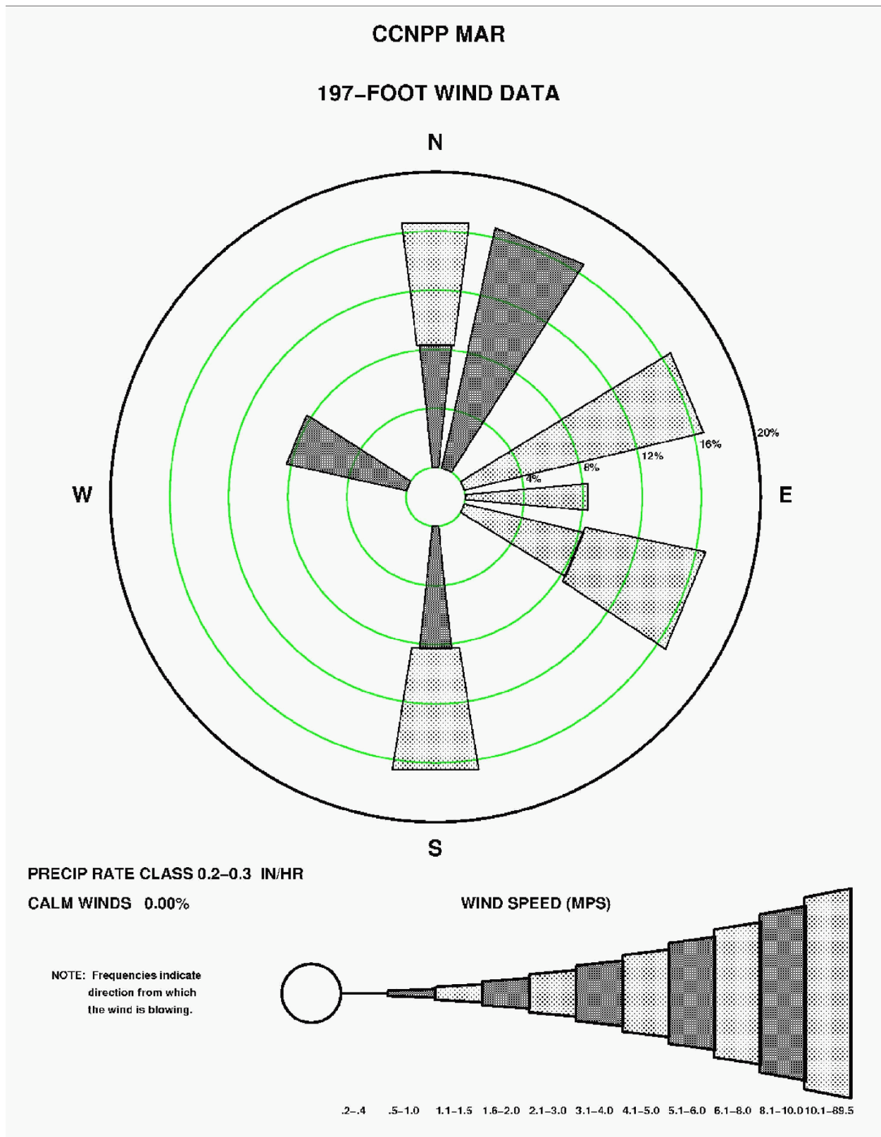
Figure 2.3-142—{CCNPP 197' (60 m) March Precipitation Wind Rose for Rate Class 0.2-0.3 in/hr}
