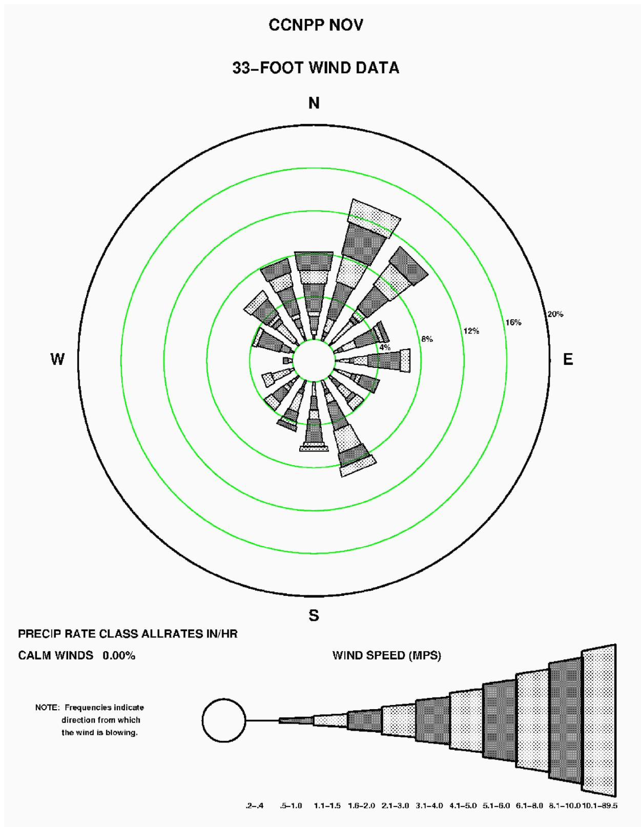
Figure 2.3-123—{CCNPP 33' (10 m) November Precipitation Wind Rose for All Rate classes}
