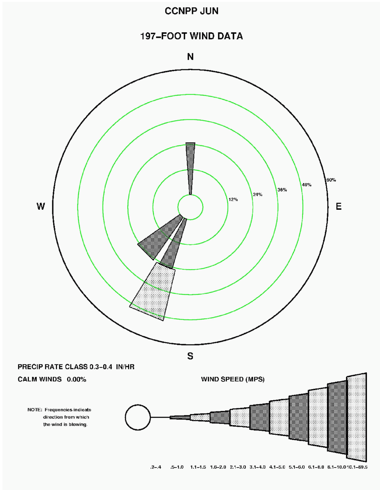
Figure 2.3-164—{CCNPP 197' (60 m) June Precipitation Wind Rose for Rate Class 0.3-0.4 in/hr}
