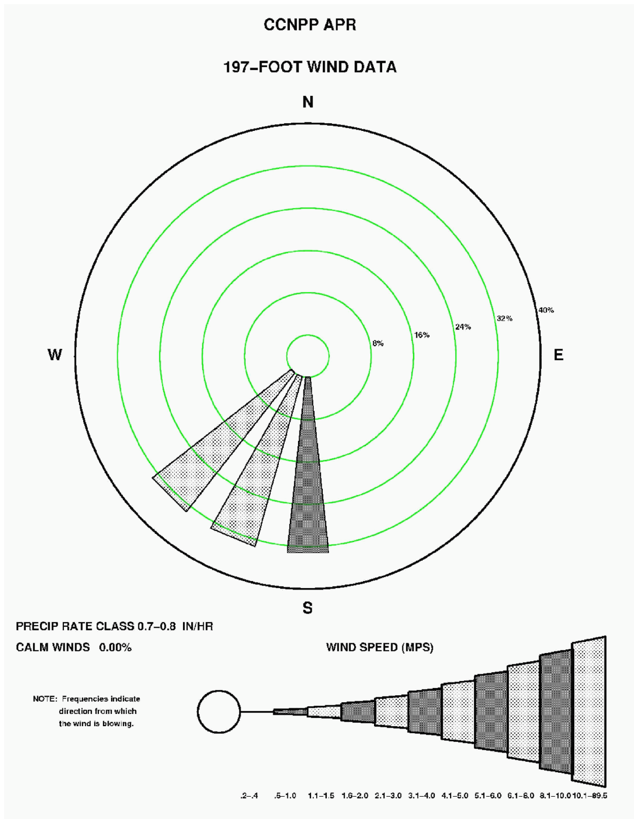
Figure 2.3-151—{CCNPP 197' (60 m) April Precipitation Wind Rose for Rate Class 0.7-0.8 in/hr}
