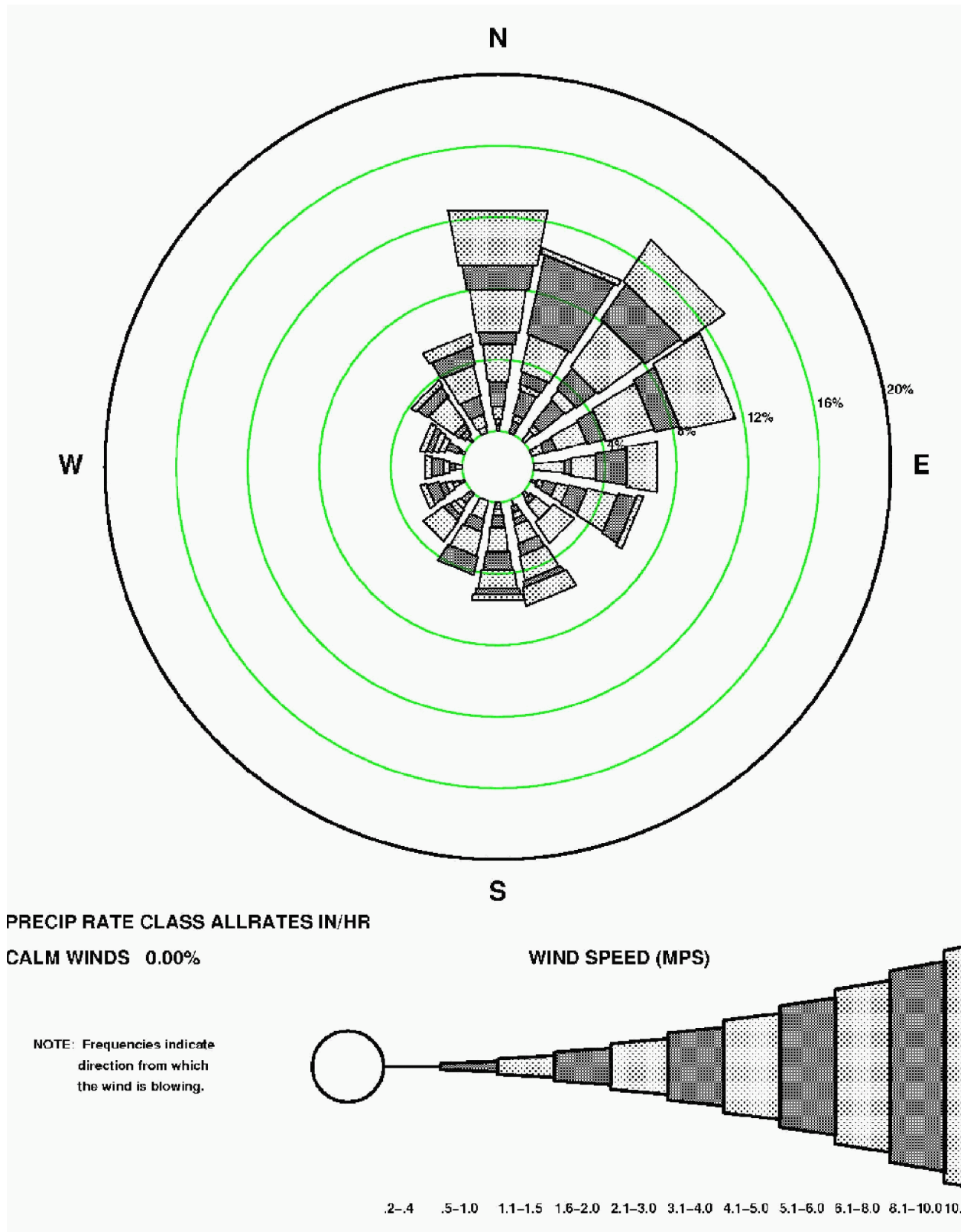
Figure 2.3-145—{CCNPP 197' (60 m) March Precipitation Wind Rose for All Rate classes}
