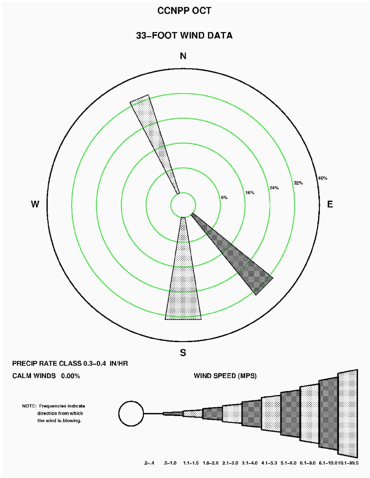
Figure 2.3-114—{CCNPP 33' (10 m) October Precipitation Wind Rose for Rate Class 0.3-0.4 in/hr}
