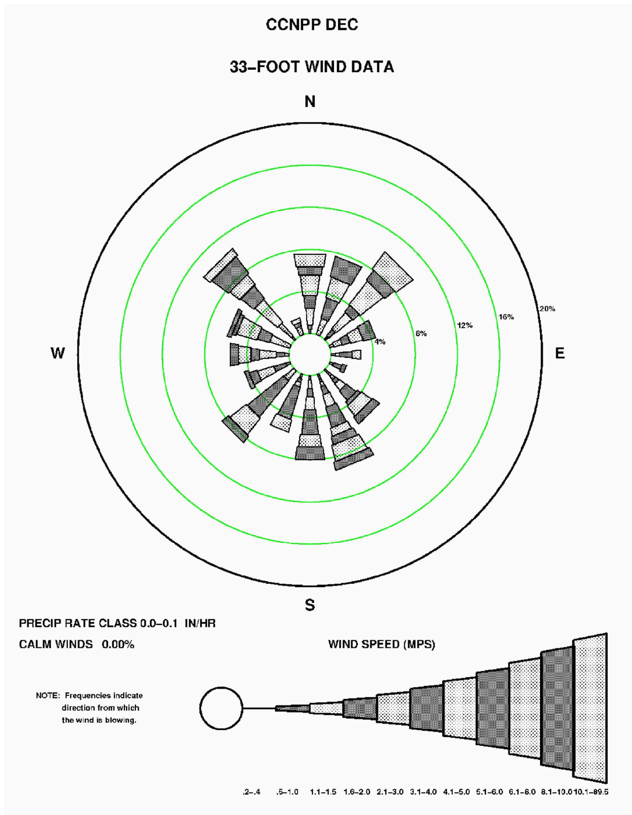
Figure 2.3-124—{CCNPP 33' (10 m) December Precipitation Wind Rose for Rate Class 0.0-0.1 in/hr}
