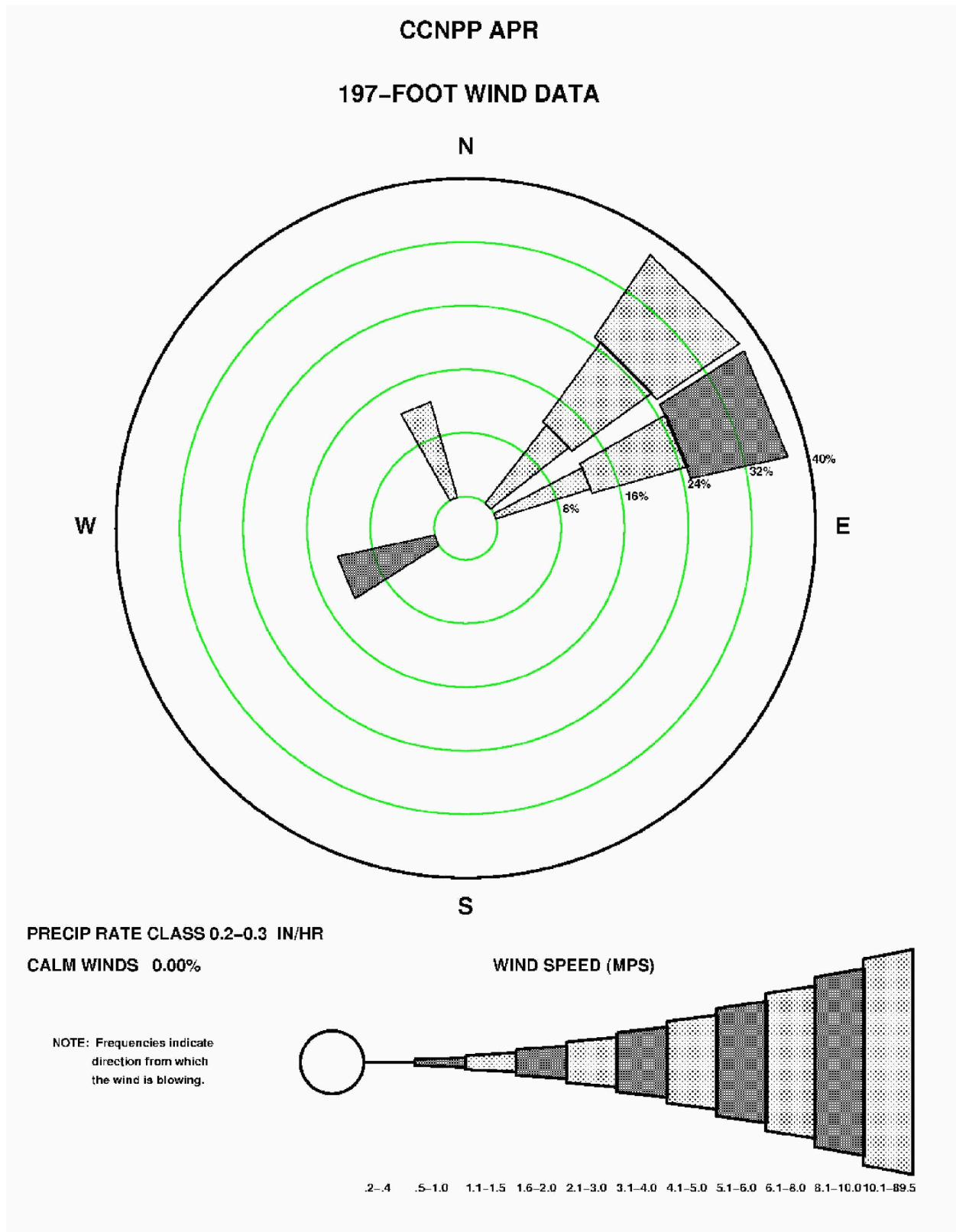
Figure 2.3-148—{CCNPP 197' (60 m) April Precipitation Wind Rose for Rate Class 0.2-0.3 in/hr}
