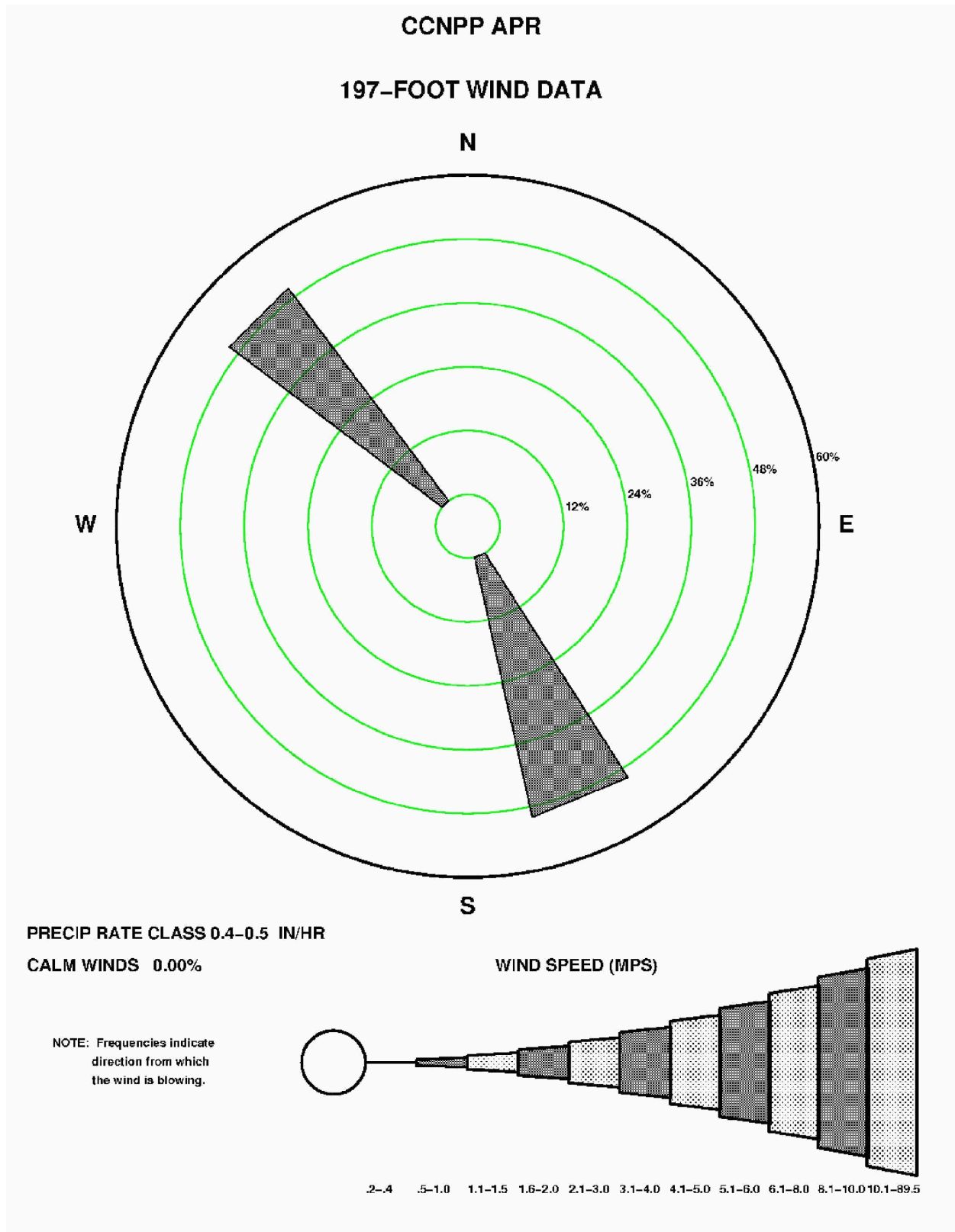
Figure 2.3-150—{CCNPP 197' (60 m) April Precipitation Wind Rose for Rate Class 0.4-0.5 in/hr}
