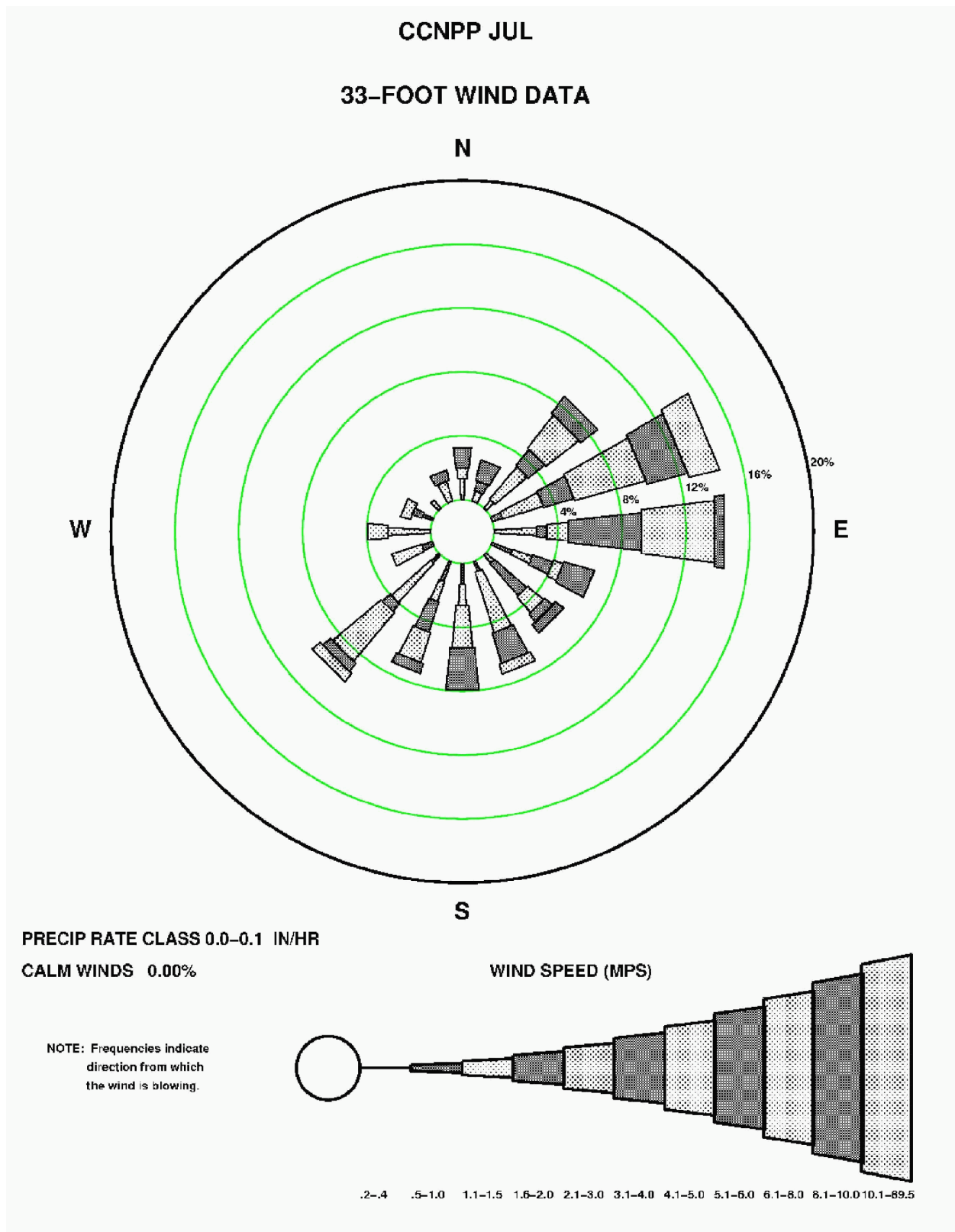
Figure 2.3-85—{CCNPP 33' (10 m) July Precipitation Wind Rose for Rate Class 0.0-0.1 in/hr}
