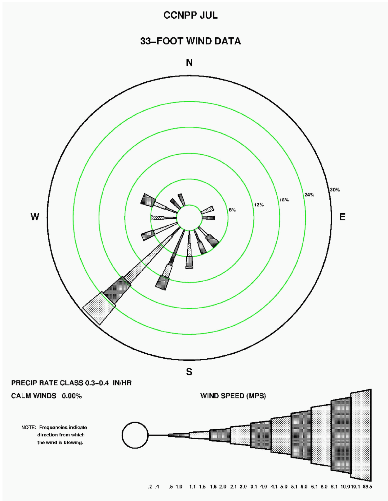
Figure 2.3-88—{CCNPP 33' (10 m) July Precipitation Wind Rose for Rate Class 0.3-0.4 in/hr}
