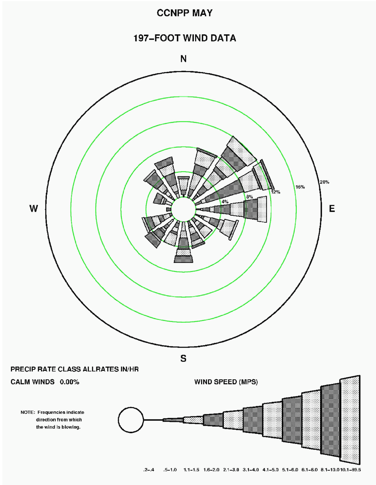
Figure 2.3-160—{CCNPP 197' (60 m) May Precipitation Wind Rose for All Rate classes}
