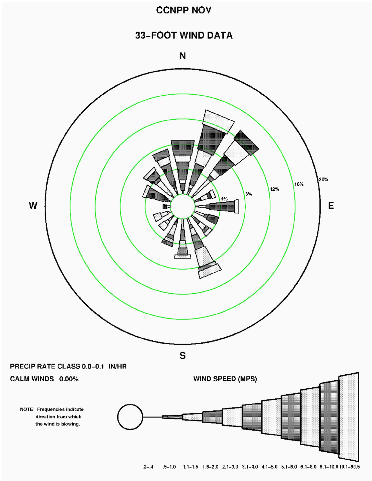
Figure 2.3-118—{CCNPP 33' (10 m) November Precipitation Wind Rose for Rate Class 0.0-0.1 in/hr}
