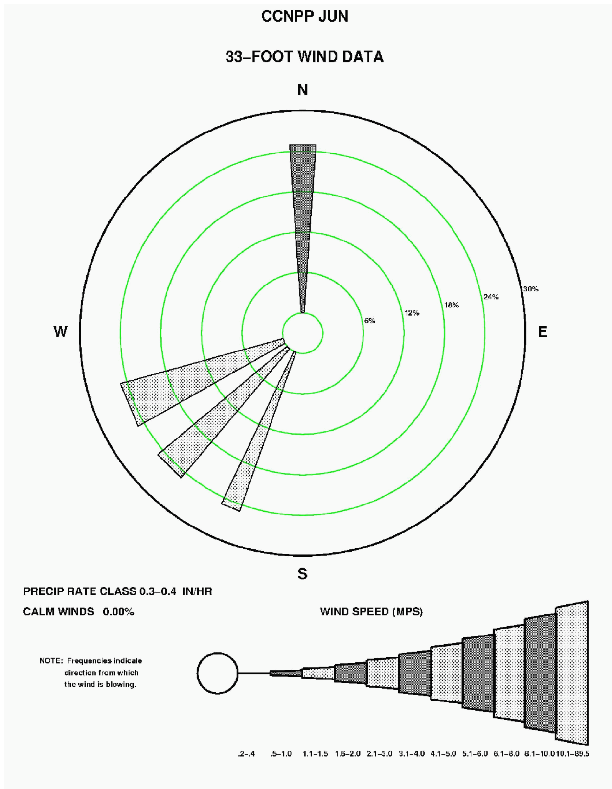
Figure 2.3-80—{CCNPP 33' (10 m) June Precipitation Wind Rose for Rate Class 0.3-0.4 in/hr}
