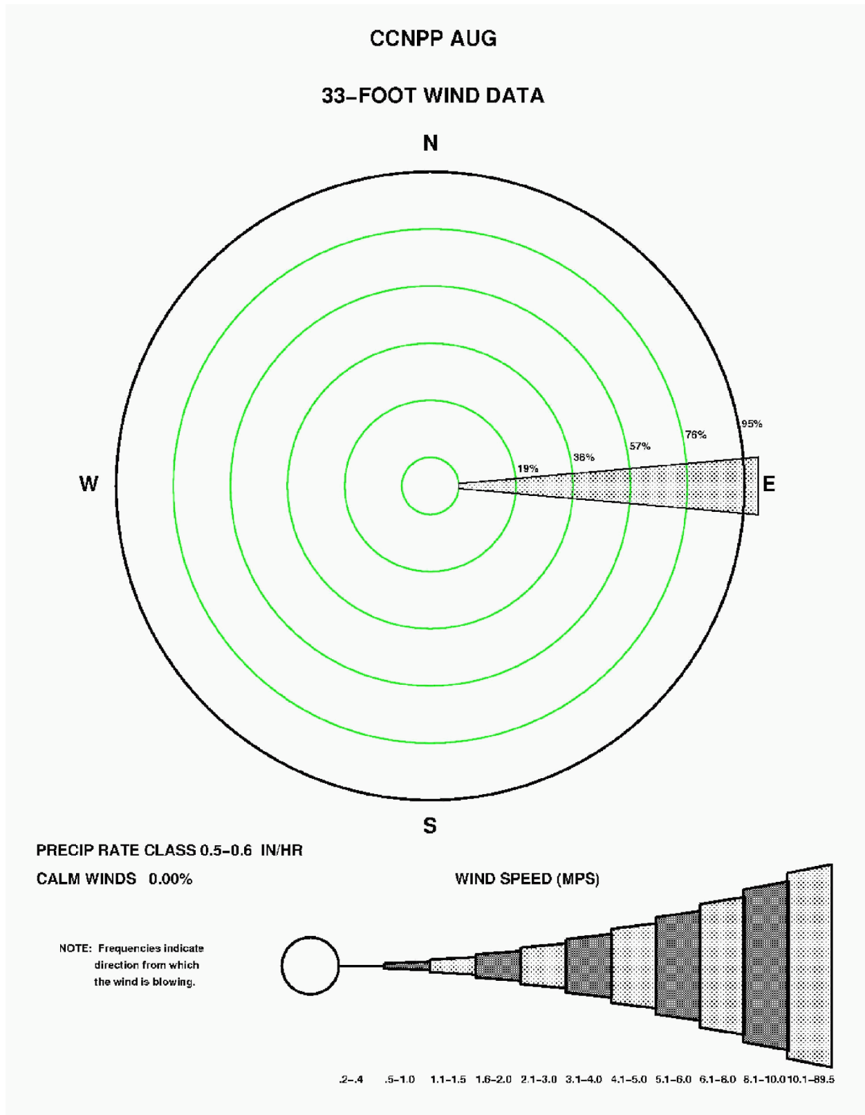
Figure 2.3-98—{CCNPP 33' (10 m) August Precipitation Wind Rose for Rate Class 0.5-0.6 in/hr}
