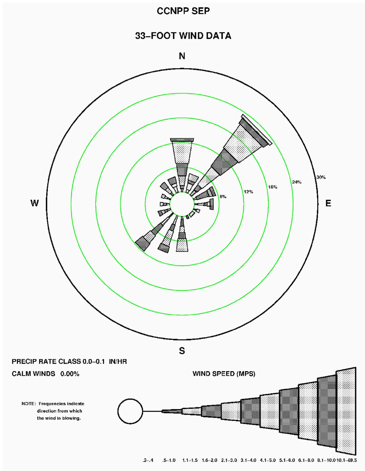
Figure 2.3-102—{CCNPP 33' (10 m) September Precipitation Wind Rose for Rate Class 0.0-0.1 in/hr}
