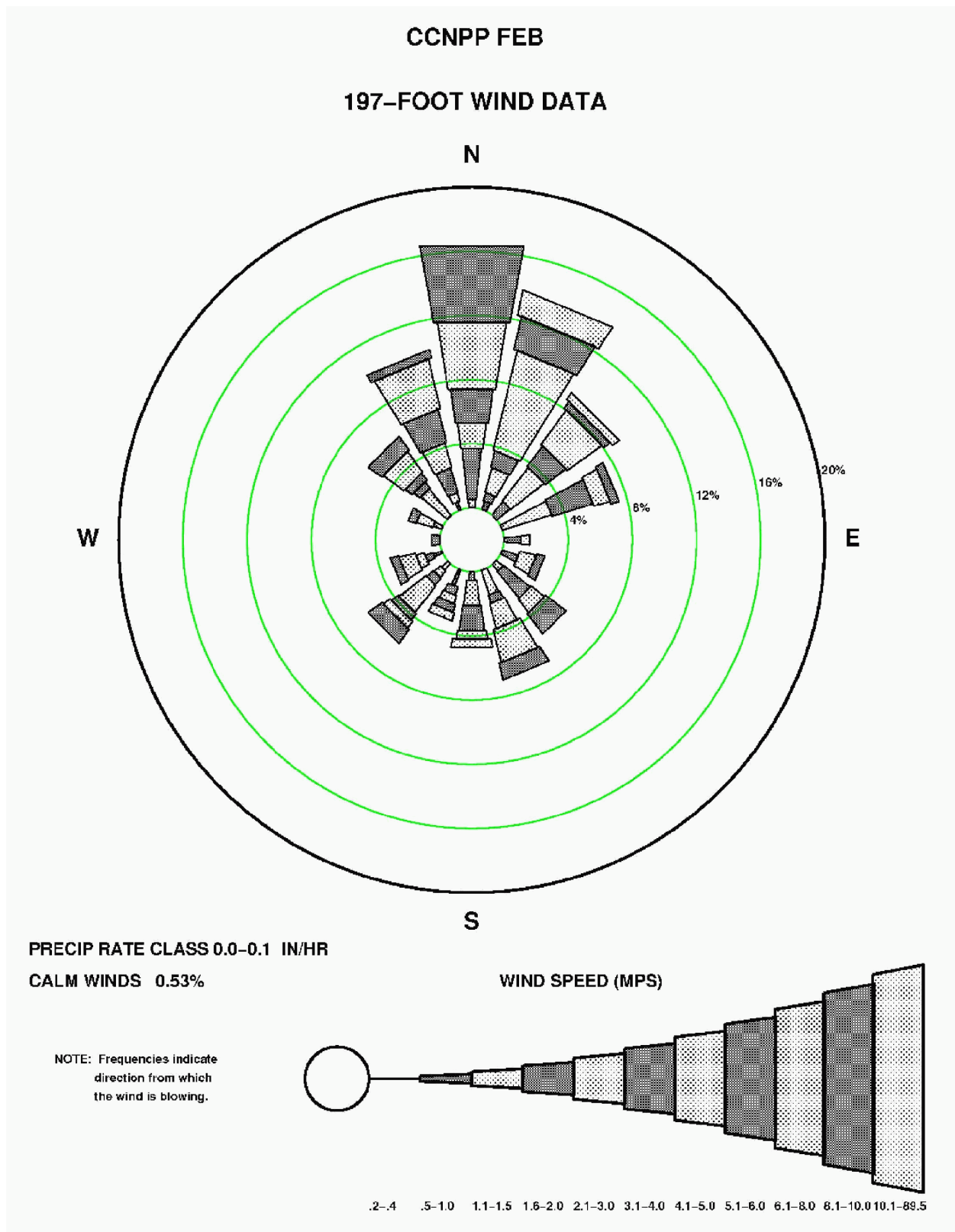
Figure 2.3-135—{CCNPP 197' (60 m) February Precipitation Wind Rose for Rate Class 0.0-0.1 in/hr}
