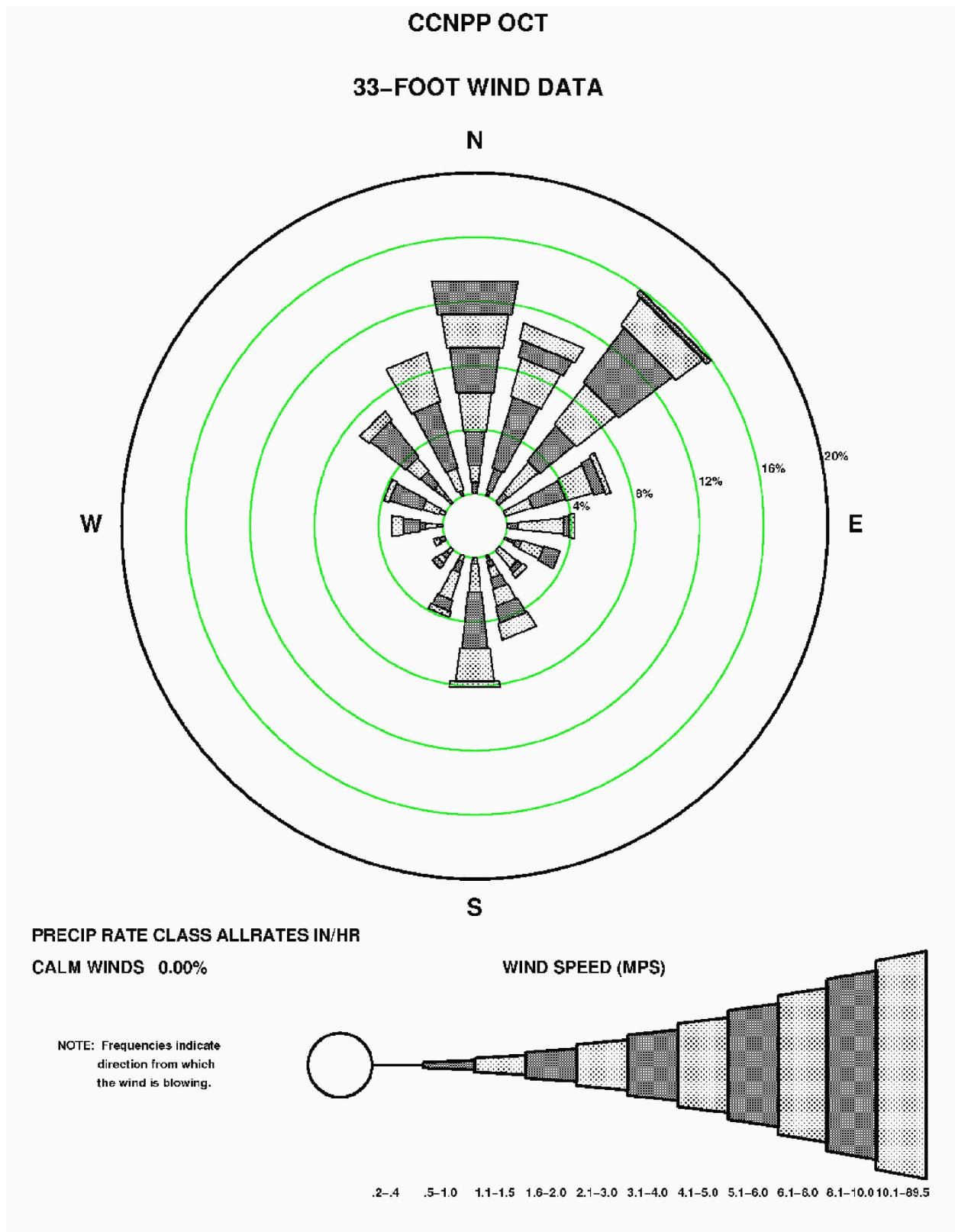
Figure 2.3-117—{CCNPP 33' (10 m) October Precipitation Wind Rose for All Rate classes}
