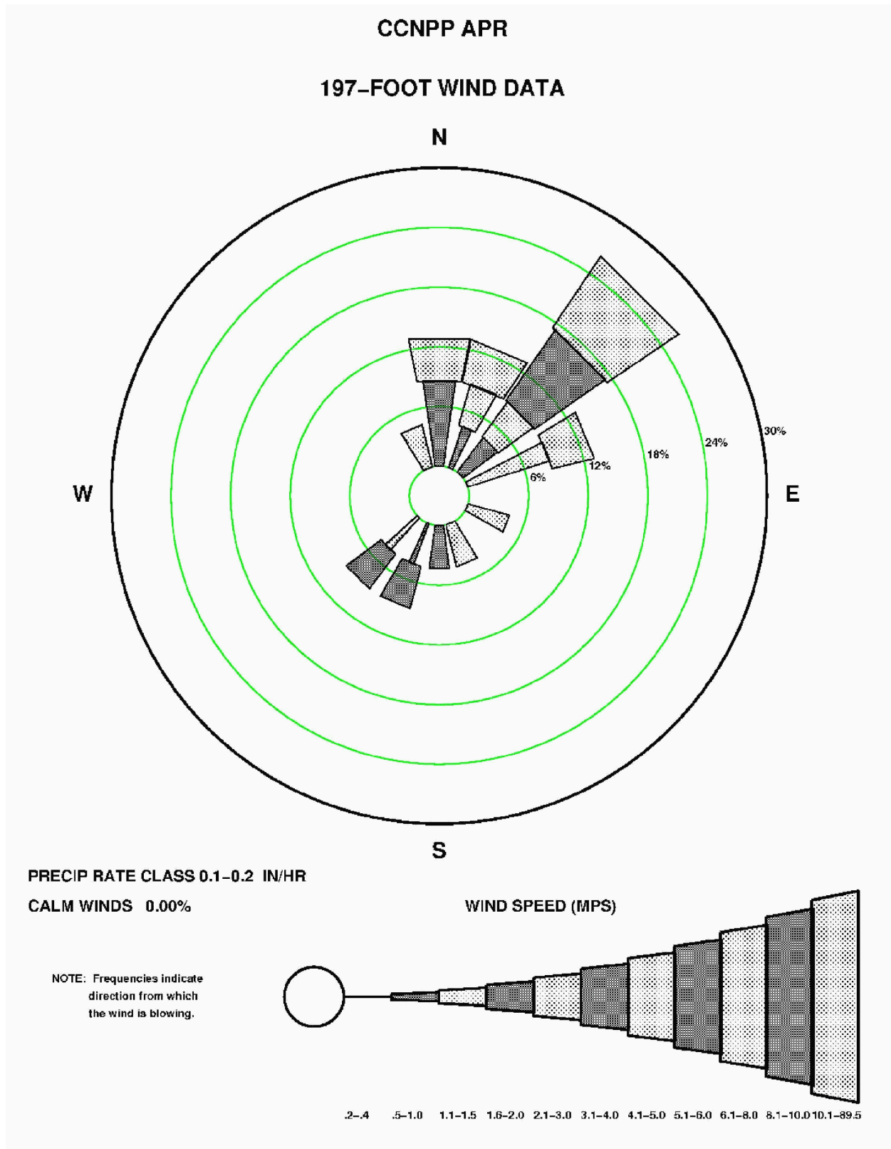
Figure 2.3-147—{CCNPP 197' (60 m) April Precipitation Wind Rose for Rate Class 0.1-0.2 in/hr}
