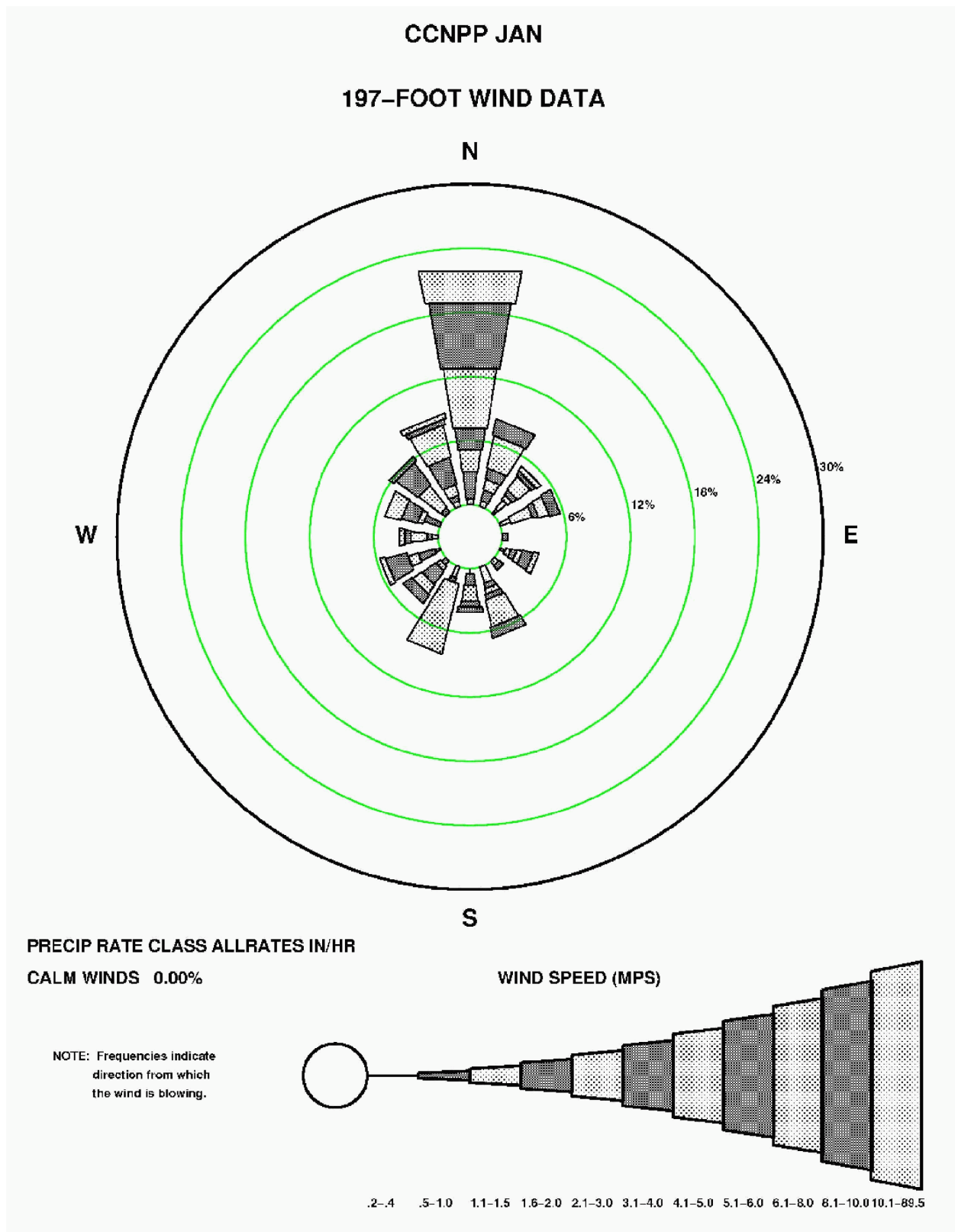
Figure 2.3-134—{CCNPP 197' (60 m) January Precipitation Wind Rose for All Rate classes}
