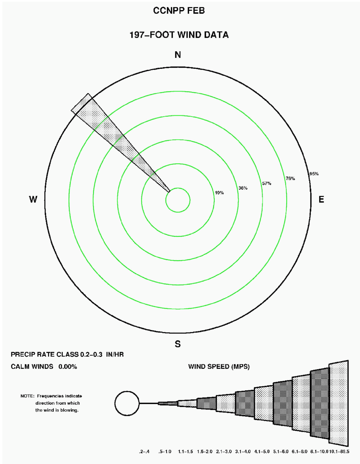
Figure 2.3-137—{CCNPP 197' (60 m) February Precipitation Wind Rose for Rate Class 0.2-0.3 in/hr}
