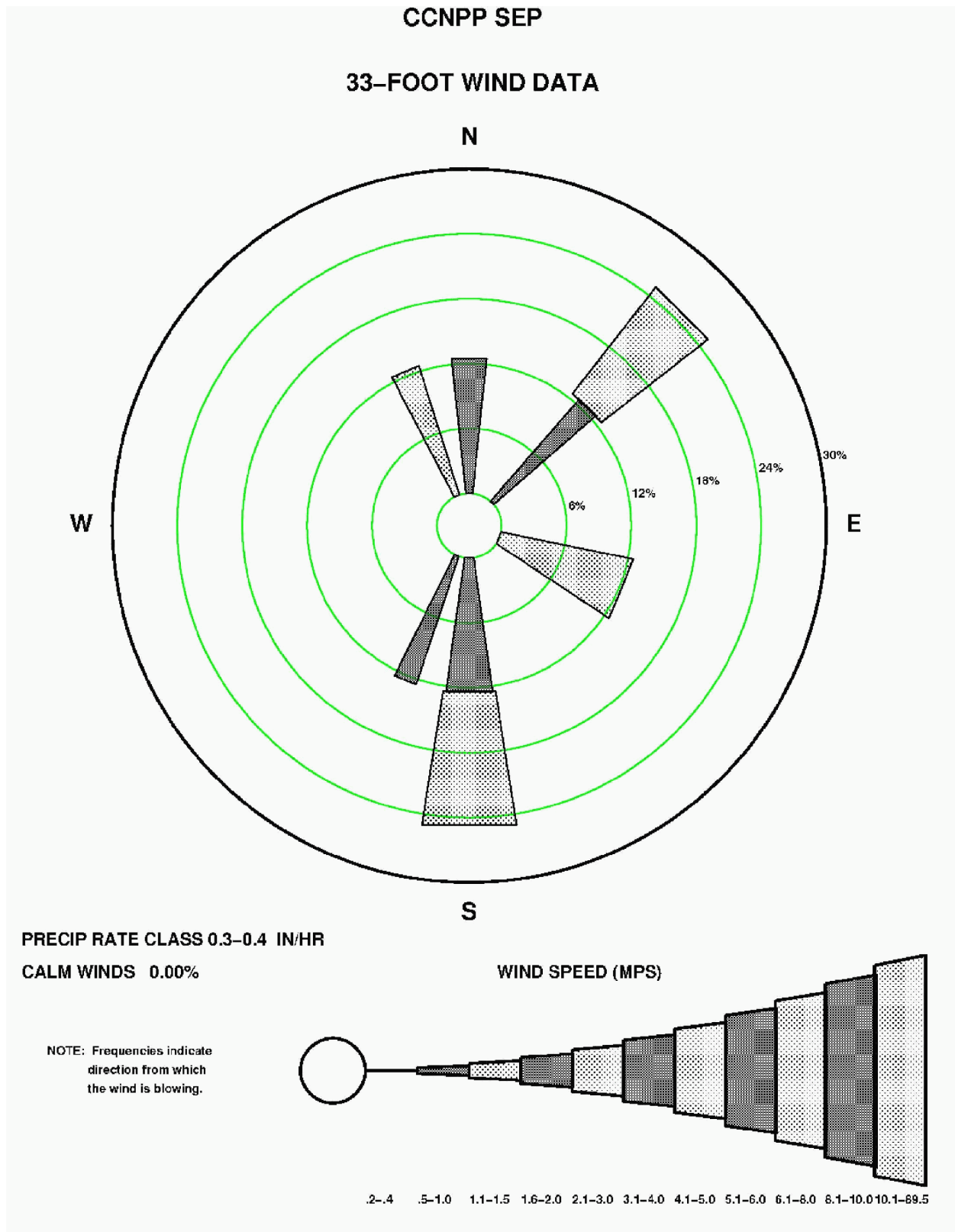
Figure 2.3-105—{CCNPP 33' (10 m) September Precipitation Wind Rose for Rate Class 0.3-0.4 in/hr}
