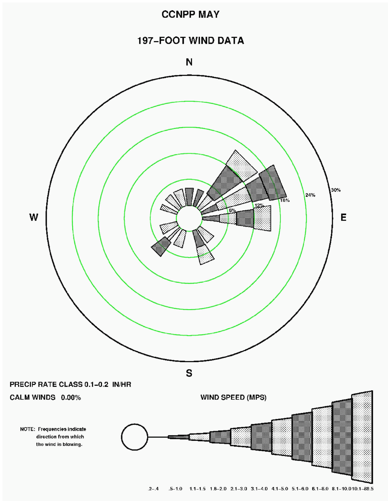
Figure 2.3-154—{CCNPP 197' (60 m) May Precipitation Wind Rose for Rate Class 0.1-0.2 in/hr}
