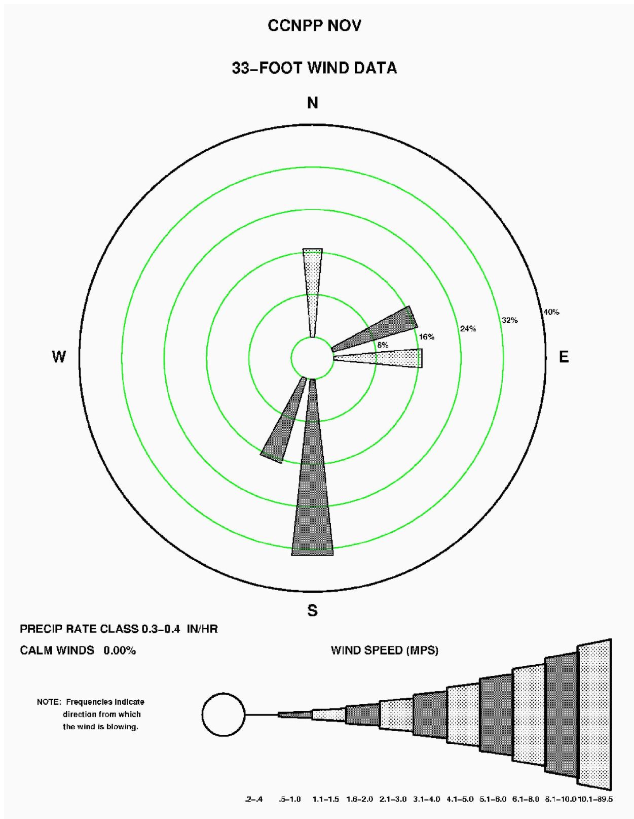
Figure 2.3-121—{CCNPP 33' (10 m) November Precipitation Wind Rose for Rate Class 0.3-0.4 in/hr}
