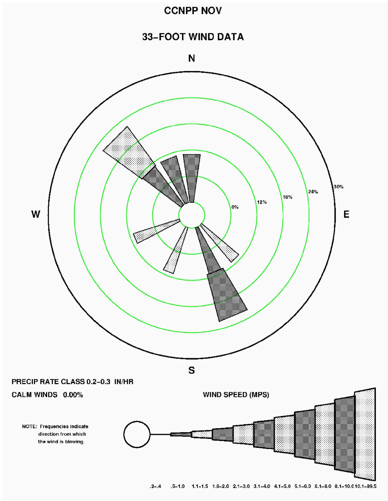
Figure 2.3-120—{CCNPP 33' (10 m) November Precipitation Wind Rose for Rate Class 0.2-0.3 in/hr}
