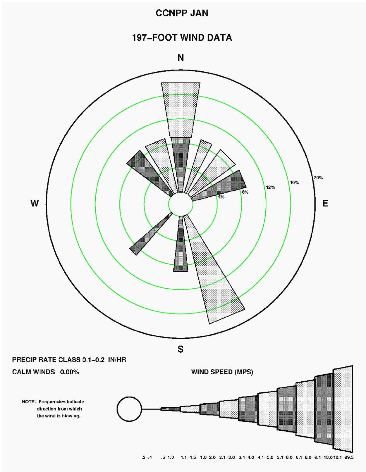
Figure 2.3-130—{CCNPP 197' (60 m) January Precipitation Wind Rose for Rate Class 0.1-0.2 in/hr}
