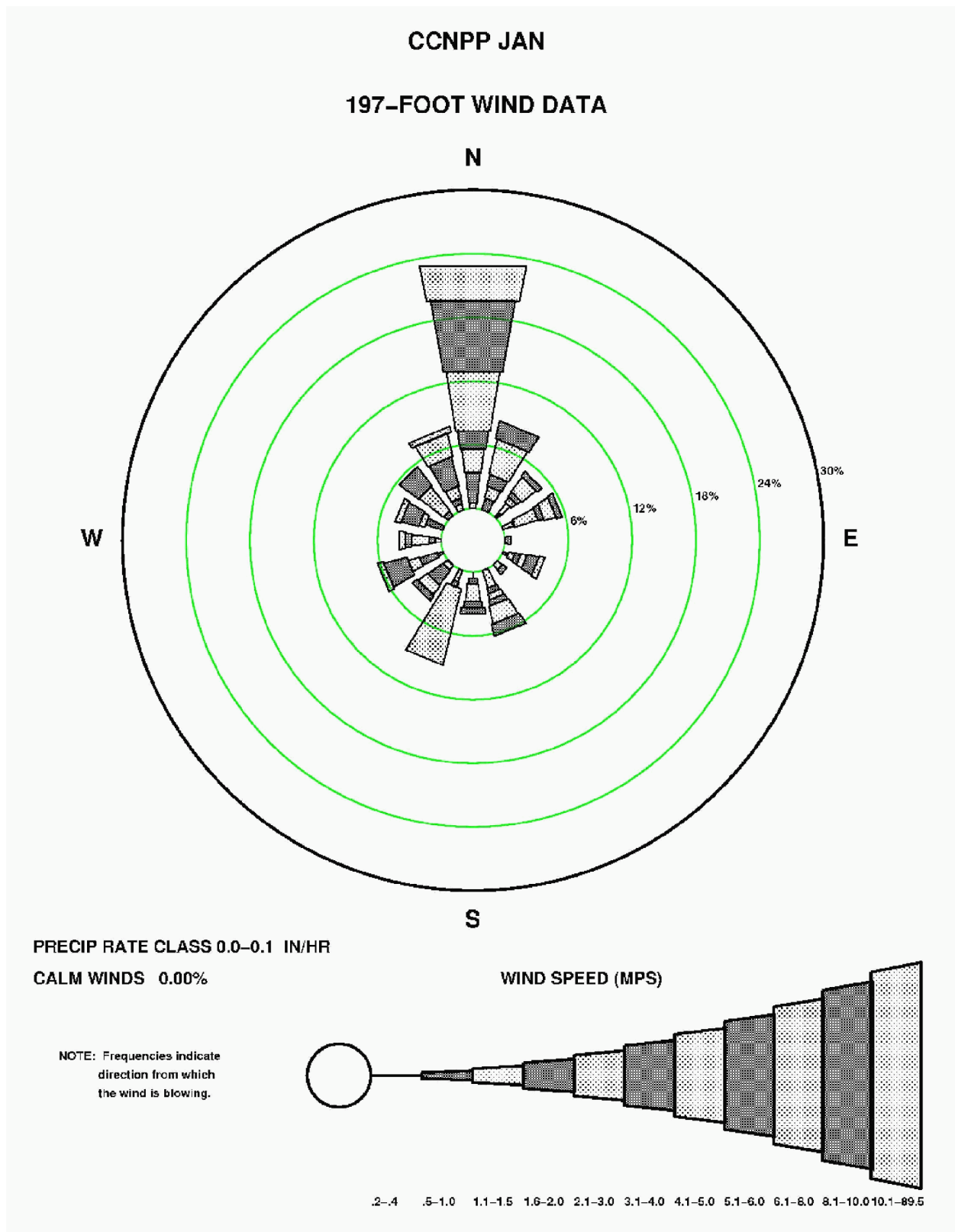
Figure 2.3-129—{CCNPP 197' (60 m) January Precipitation Wind Rose for Rate Class 0.0-0.1 in/hr}
