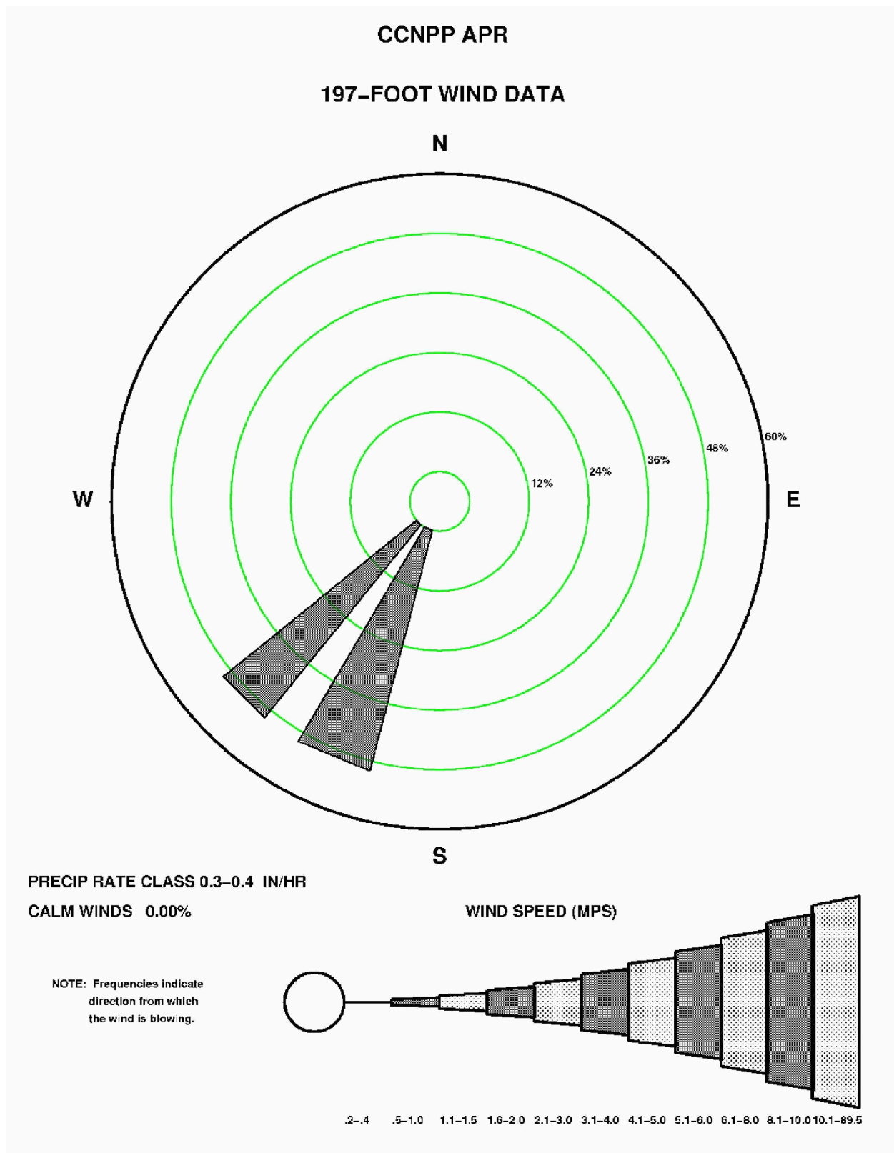
Figure 2.3-149—{CCNPP 197' (60 m) April Precipitation Wind Rose for Rate Class 0.3-0.4 in/hr}
