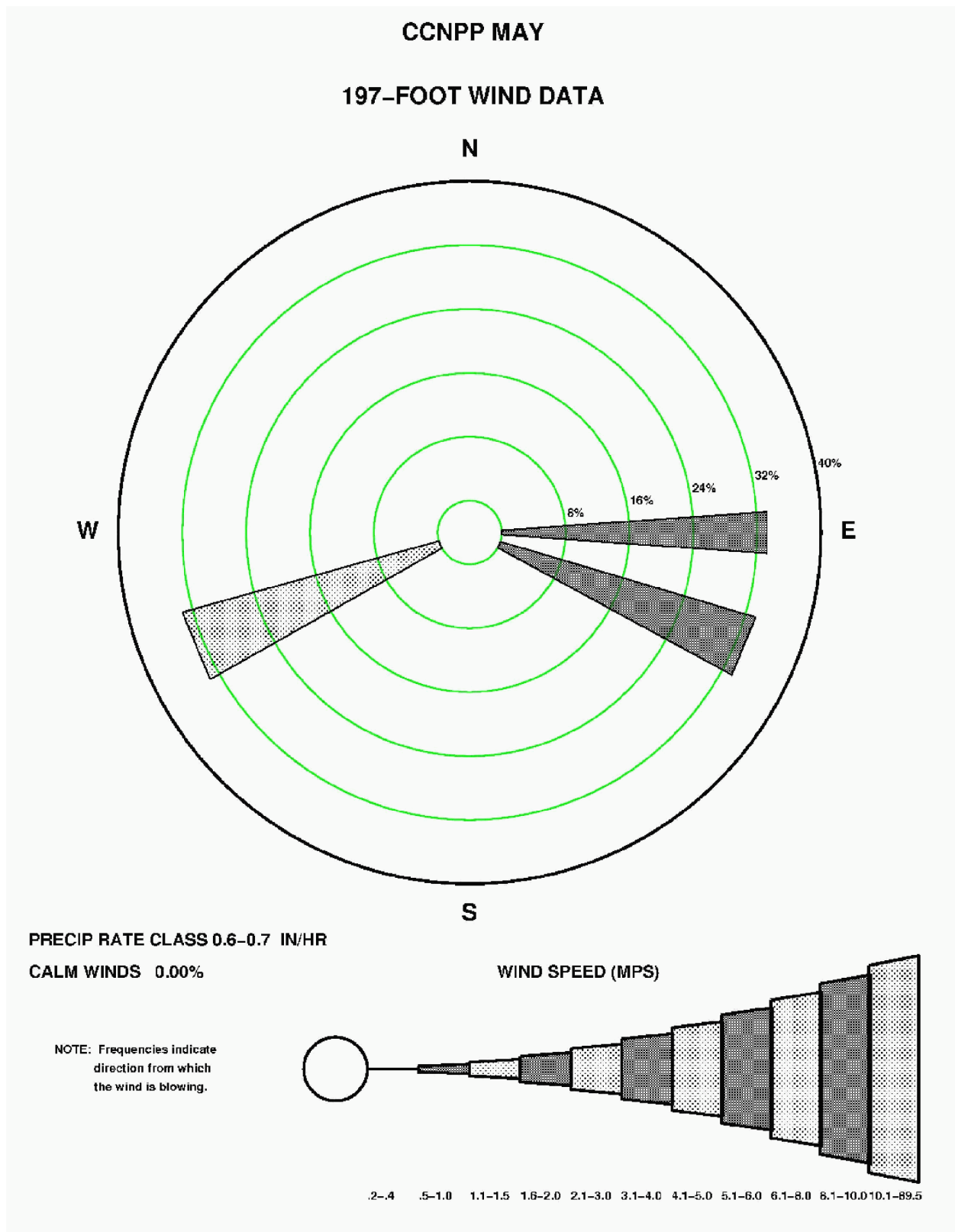
Figure 2.3-158—{CCNPP 197' (60 m) May Precipitation Wind Rose for Rate Class 0.6-0.7 in/hr}
