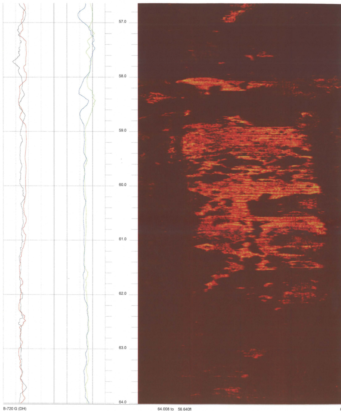
FPL Turkey Point COL Boring B-720 G (DH) Acoustic Televiewer based Caliper rev 1 Sheet 6 of 14
