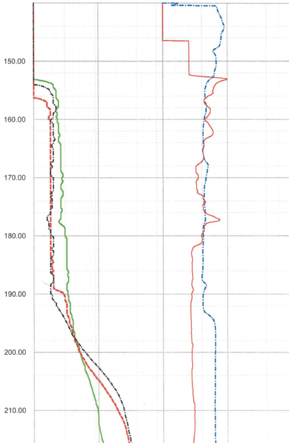
FPL Turkey Point COL Boring B-601 (DH) lower section ELOG, Caliper and Natural Gamma rev 1 Sheet 1 of 4
