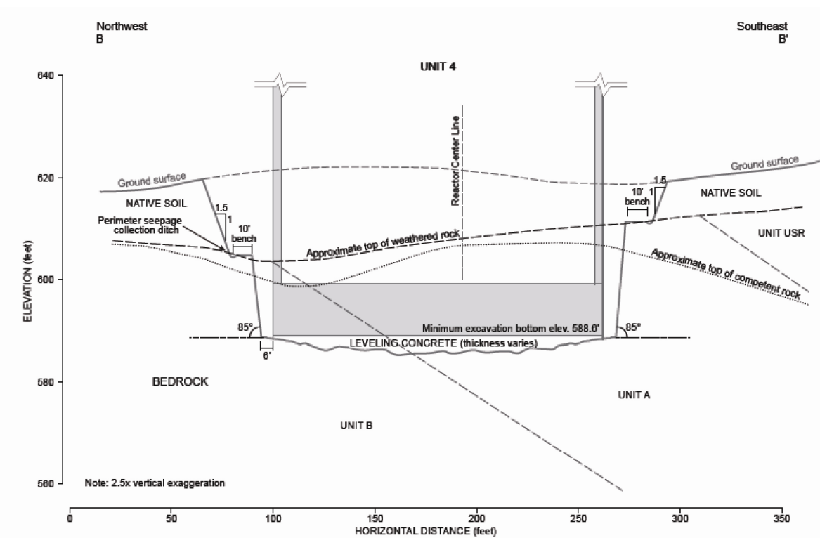
Figure 2.5.4-7b Lateral Extent of Excavation for BLN Unit 4 (FSAR Figure 2.5-348b)
