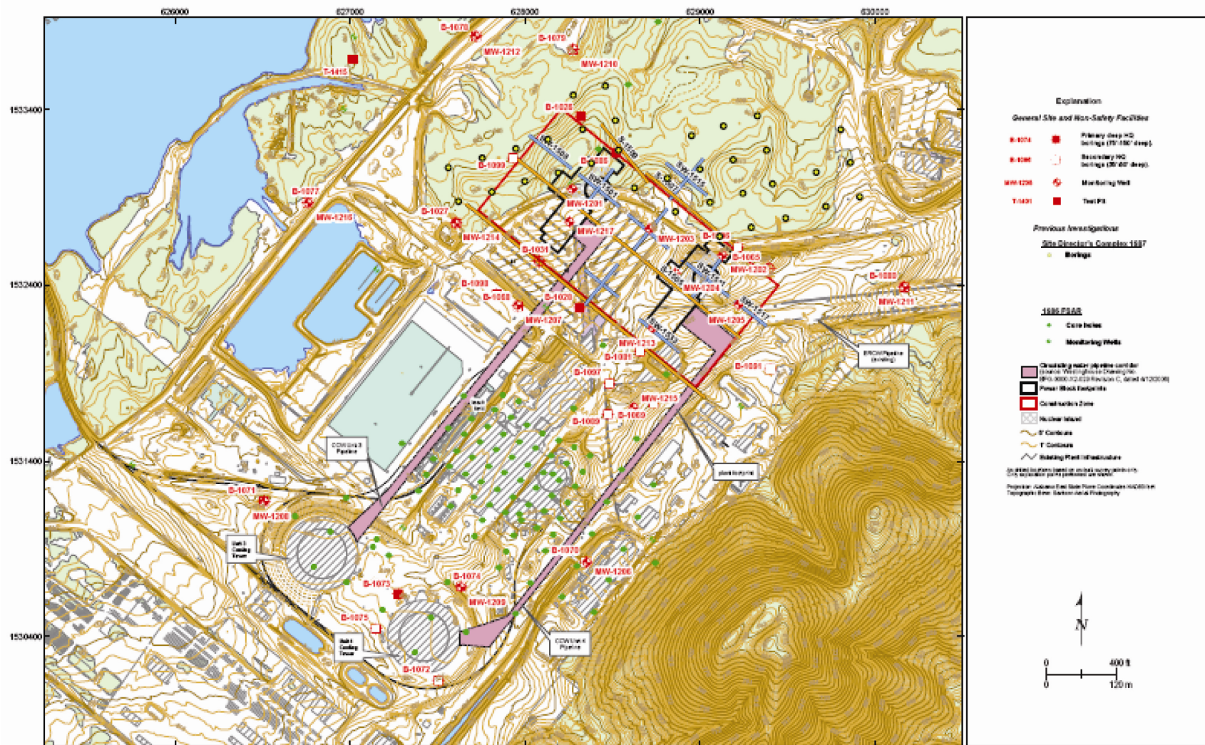
Figure 2.5.4-6 Locations of the Exploration Points Outside of the Power Block Construction Zone (reproduced from FSAR Figure 2.5-327)
