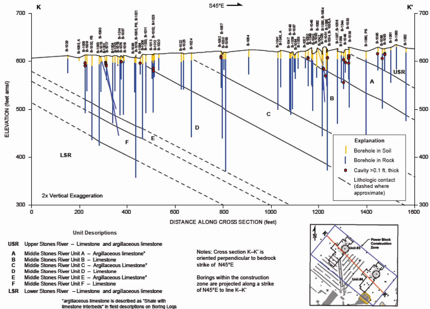
Figure 2.5.4-4 Cross Section Demonstrating the Relationship of Cavities to Boreholes at the BLN Site (reproduced from FSAR Figure 2.5-306)
