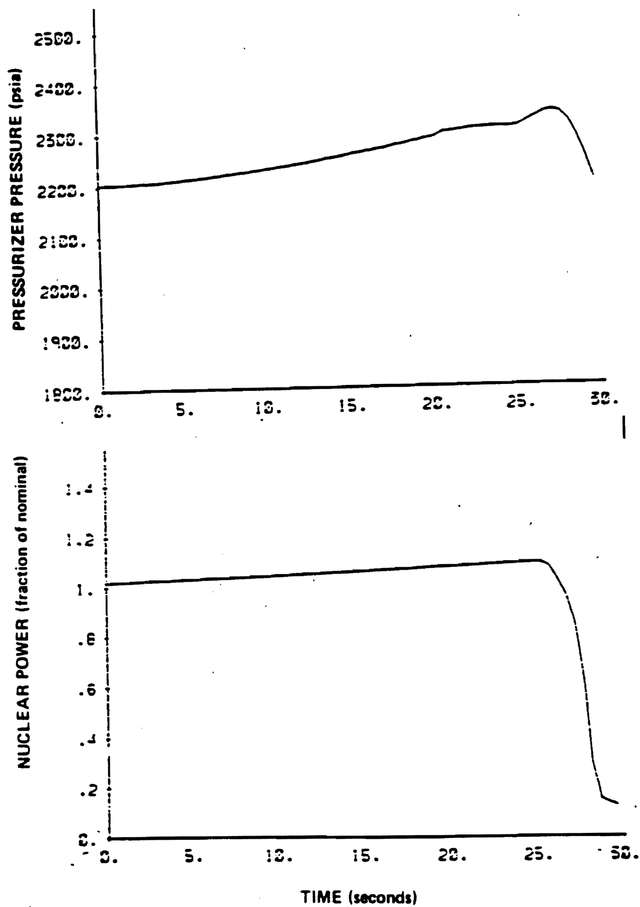
Figure 15.2-6. Pressurizer Pressure Transient and Nuclear Power Transient for Uncontrolled Rod Withdrawal from Full Power with Minimum Feedback and 3 PCM/SEC Withdrawal Rate
