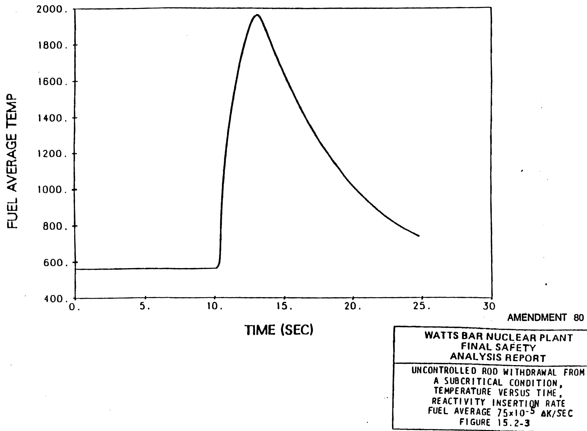
Figure 15.2-3 Uncontrolled Rod Withdrawal from a Subcritical Condition, Temperature Versus Time, Reactivity Insertion Rate Fuel Average 75 \times 10^{-5} \Delta k/sec
