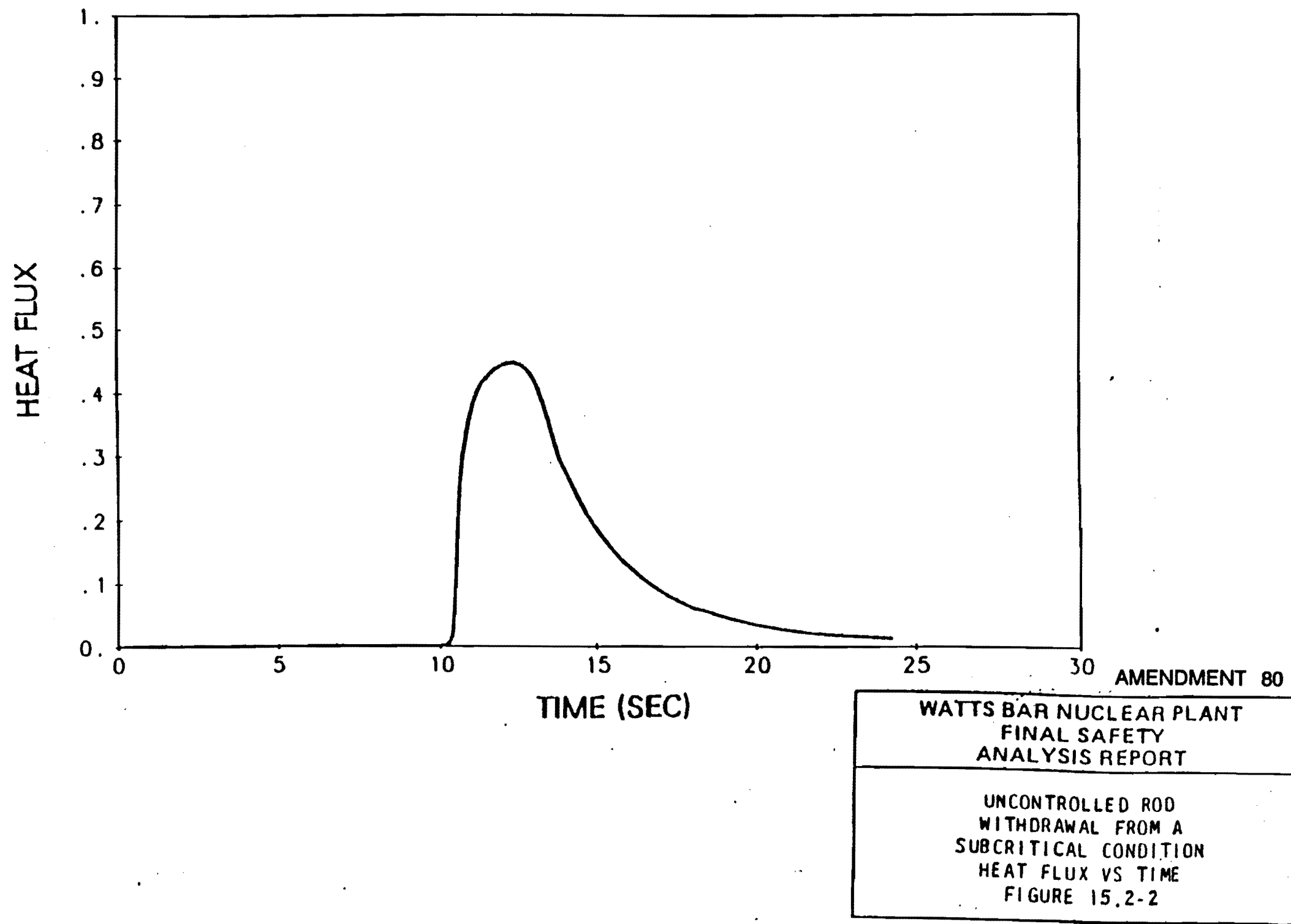
Figure 15.2-2 Uncontrolled Rod Withdrawal From a Subcritical Condition Heat Flux vs Time
