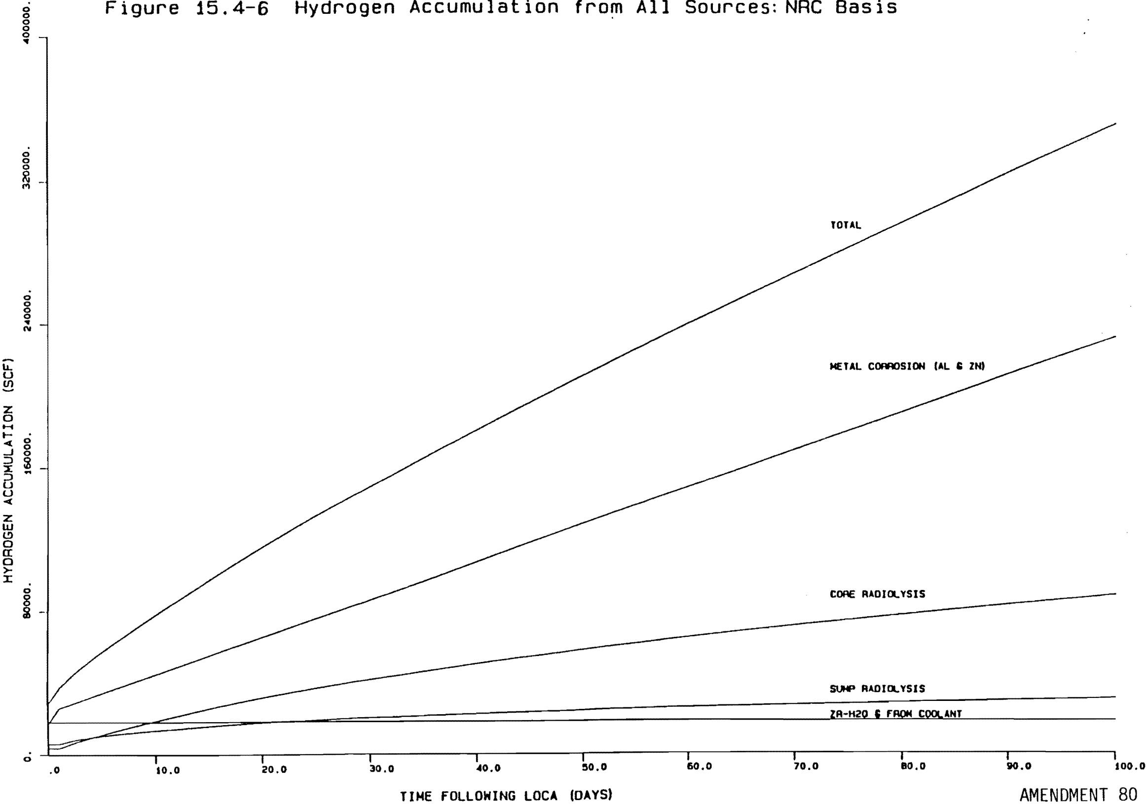
Figure 15.4-6 Hydrogen Accumulation from All Sources: NRC Basis
