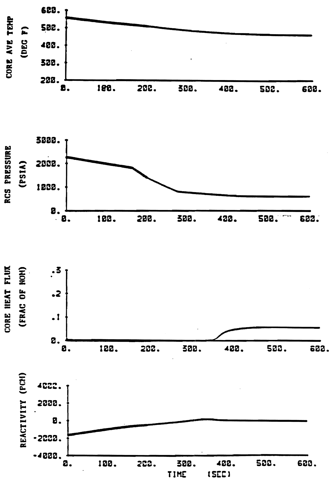
Figure 15.2-41 Transient Response for a Steam Line Break Equivalent to 247 Lbs/Seconds at 1100 PSIA With Outside Power
