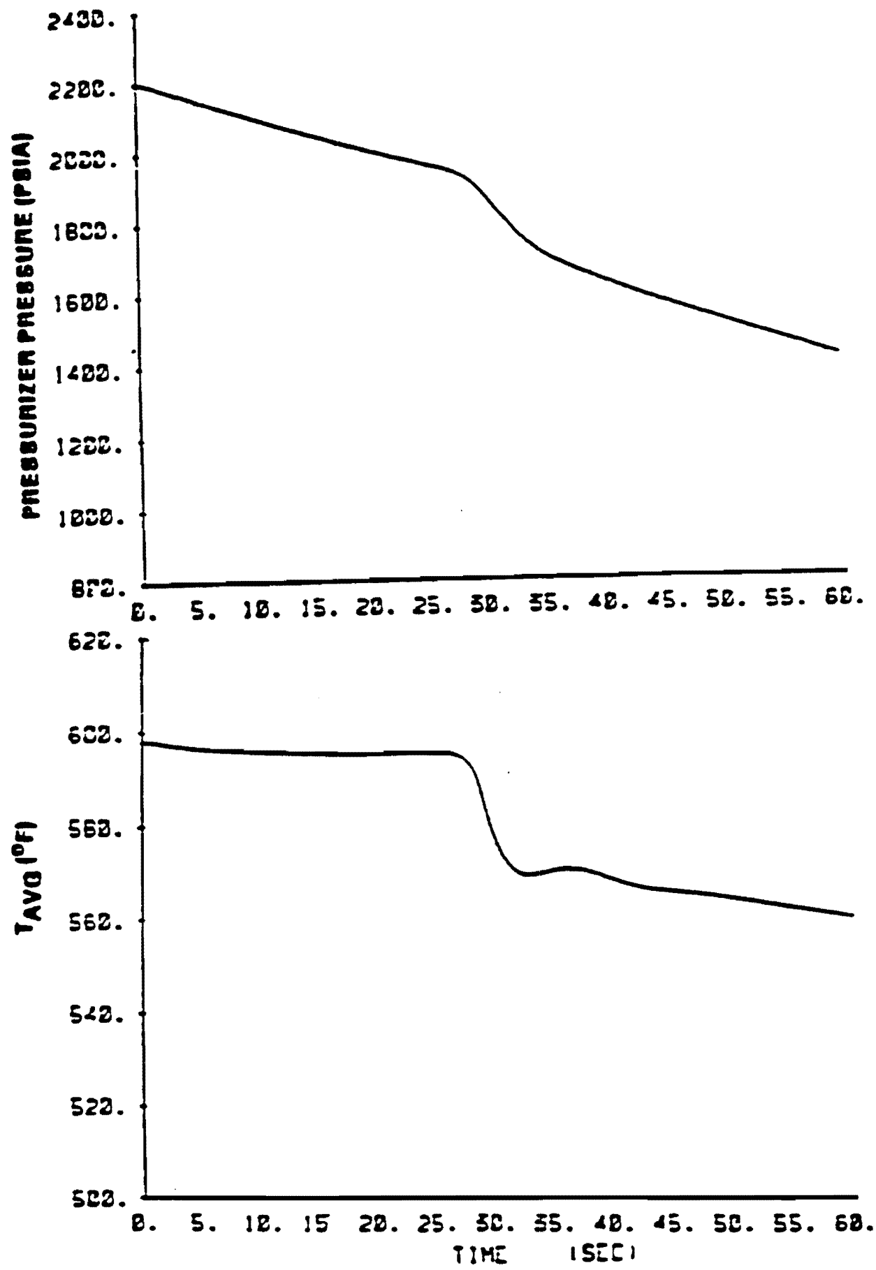
Figure 15.2-38 Pressurizer Pressure Transient and Core Average Temperature for Accidental Depressurization of the RCS
