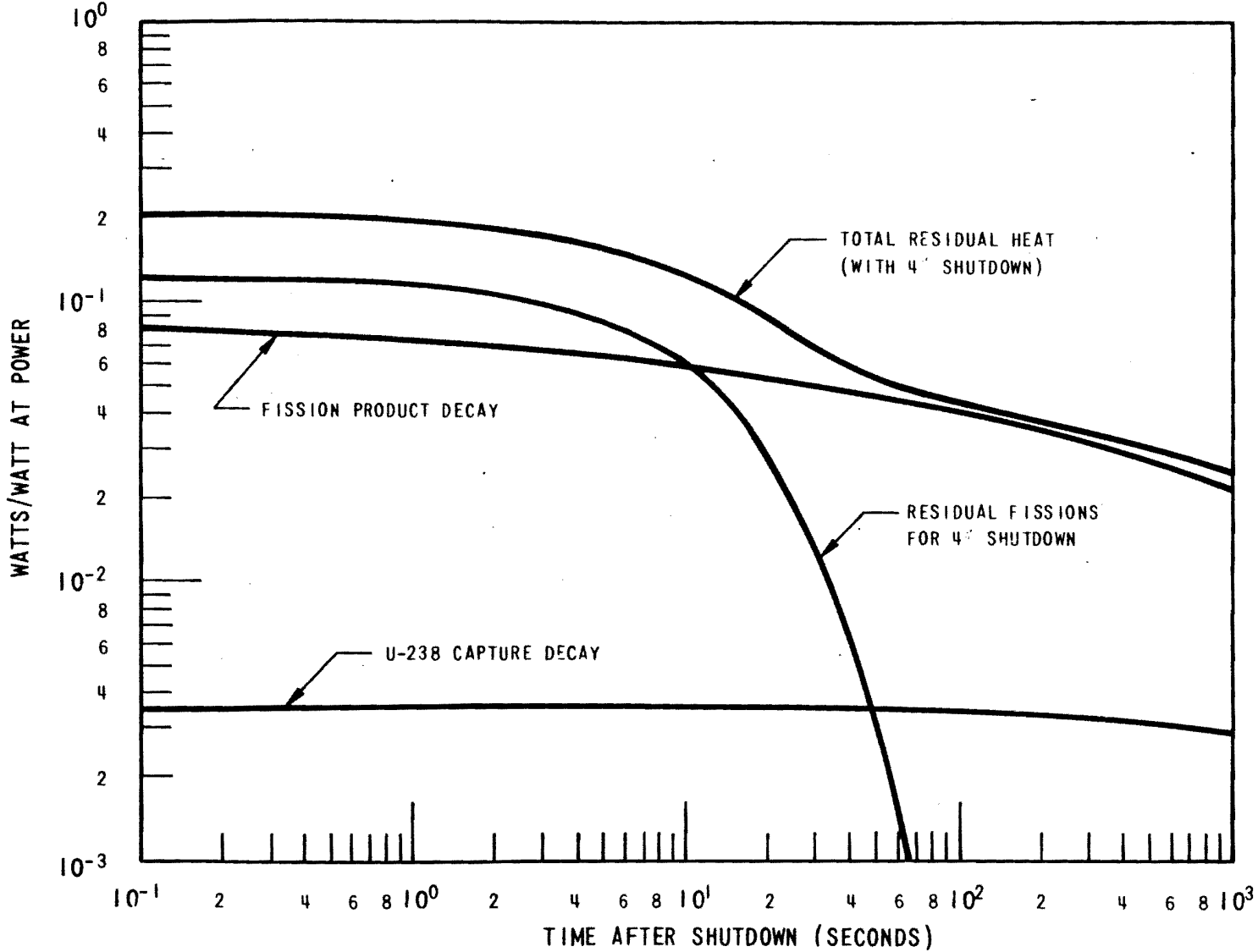
Figure 15.1-6 Residual Decay Heat
