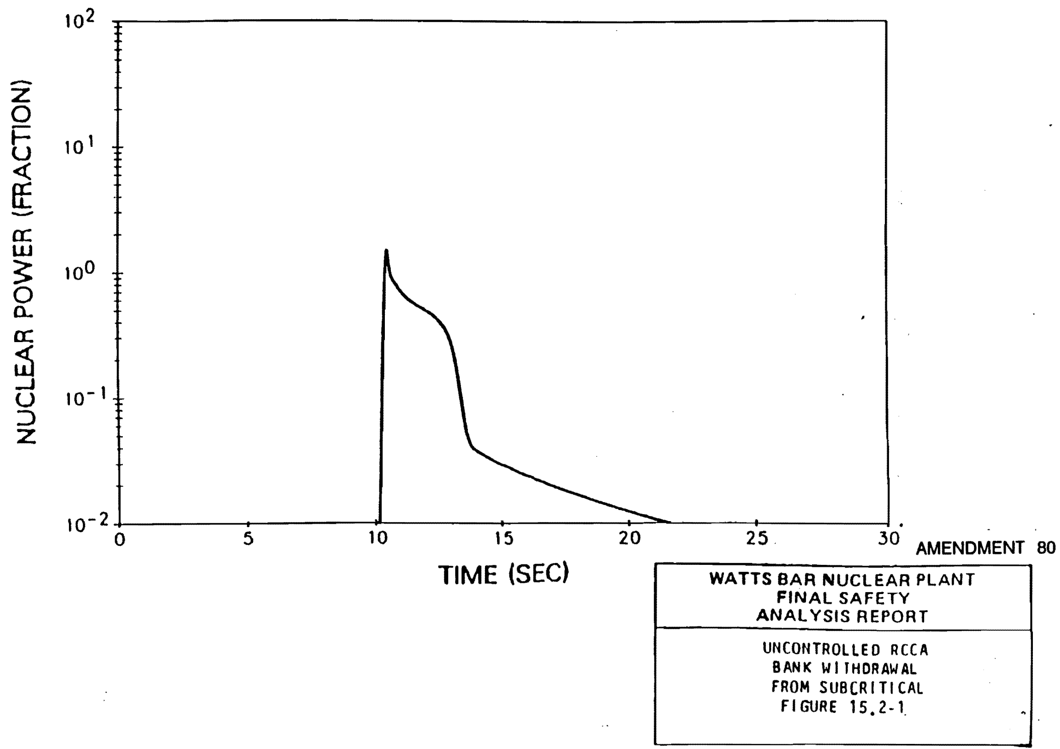
Figure 15.2-1 Uncontrolled RCCA Bank Withdrawal From Subcritical
