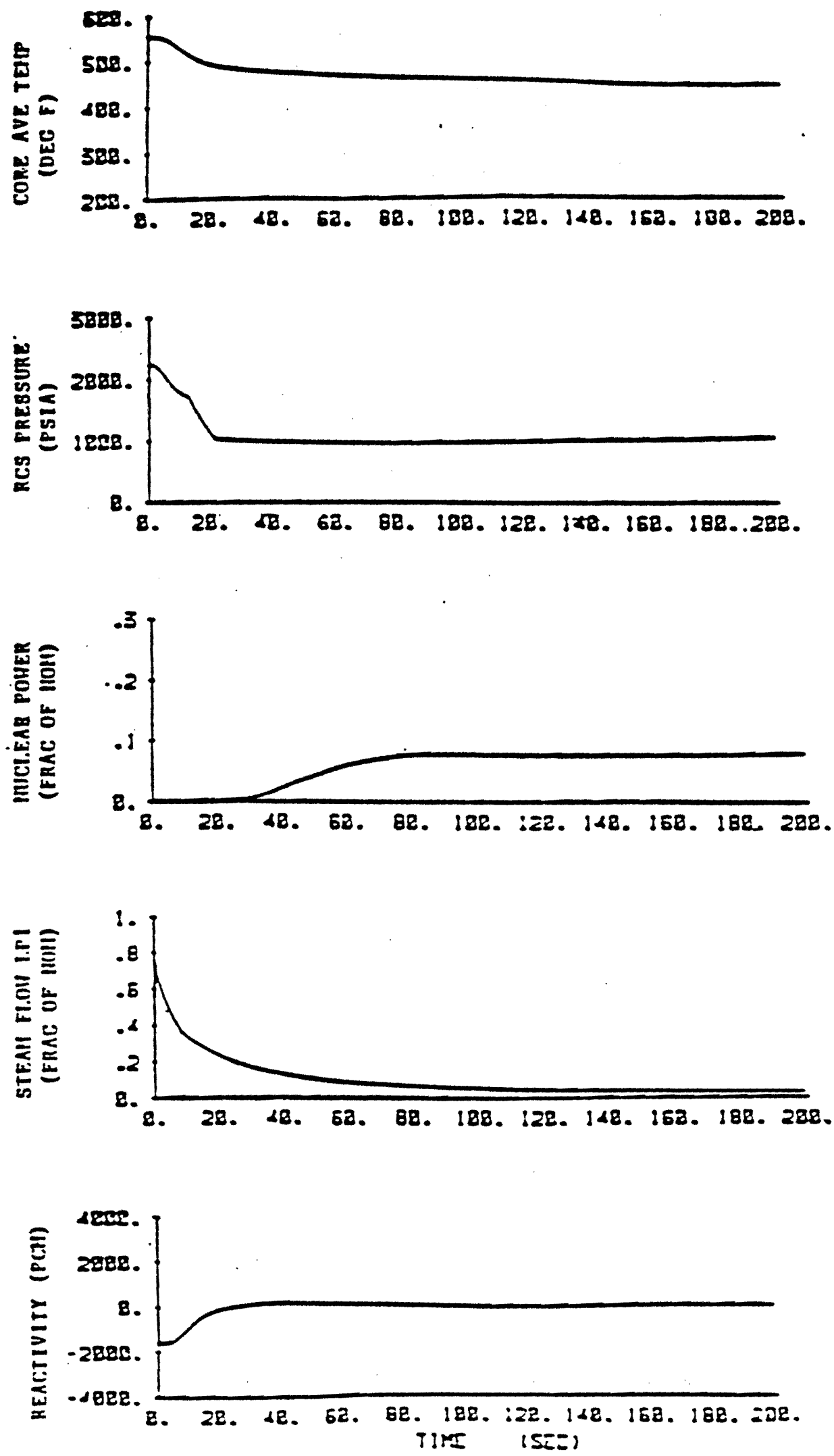
Figure 15.4 12. Transient Response to Steam Line Break with Safety Injection and Without Offsite Power (case b)
