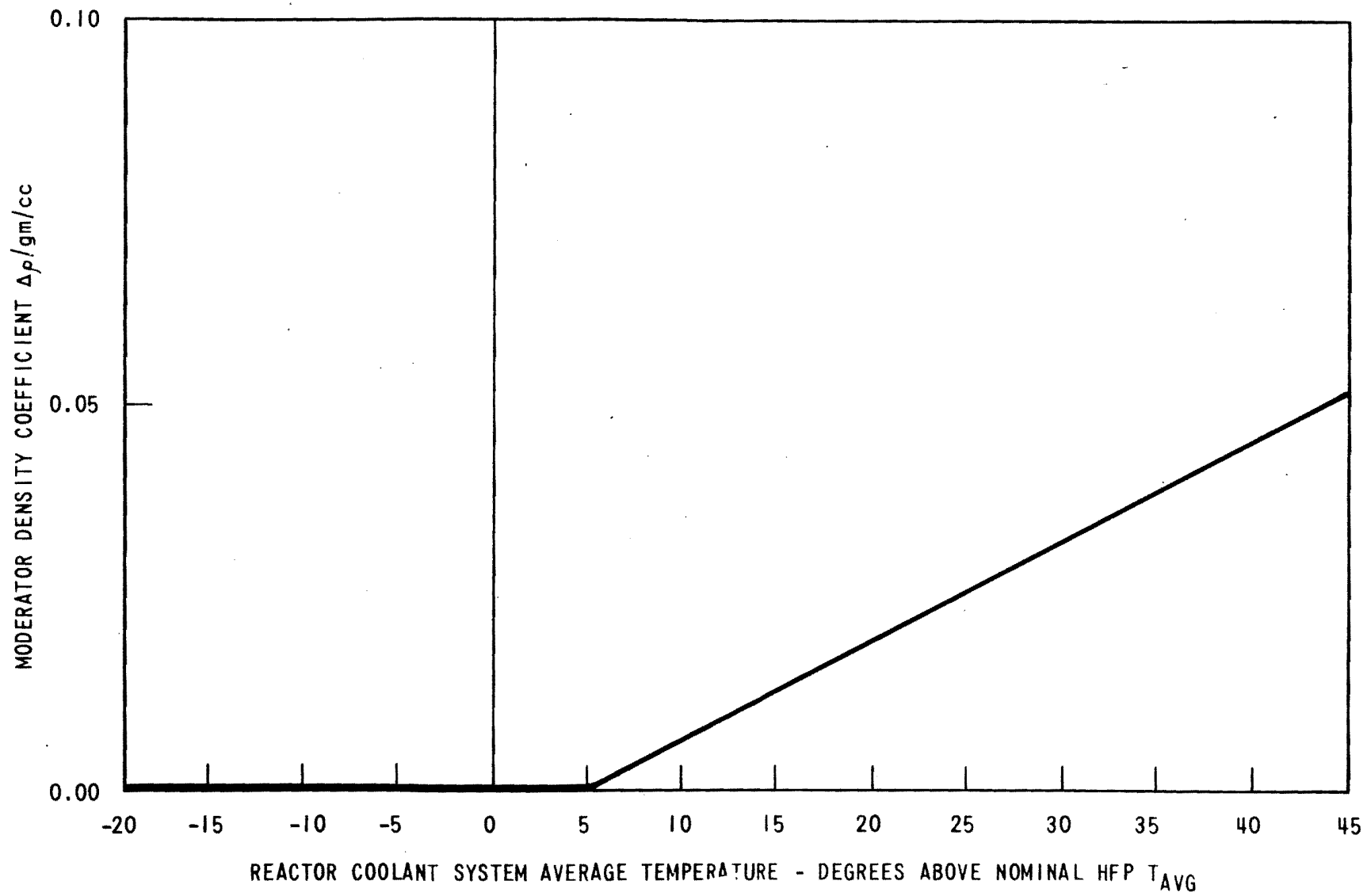
Figure 15.1-7 Minimum Moderator Density Coefficient Used in Analysis
