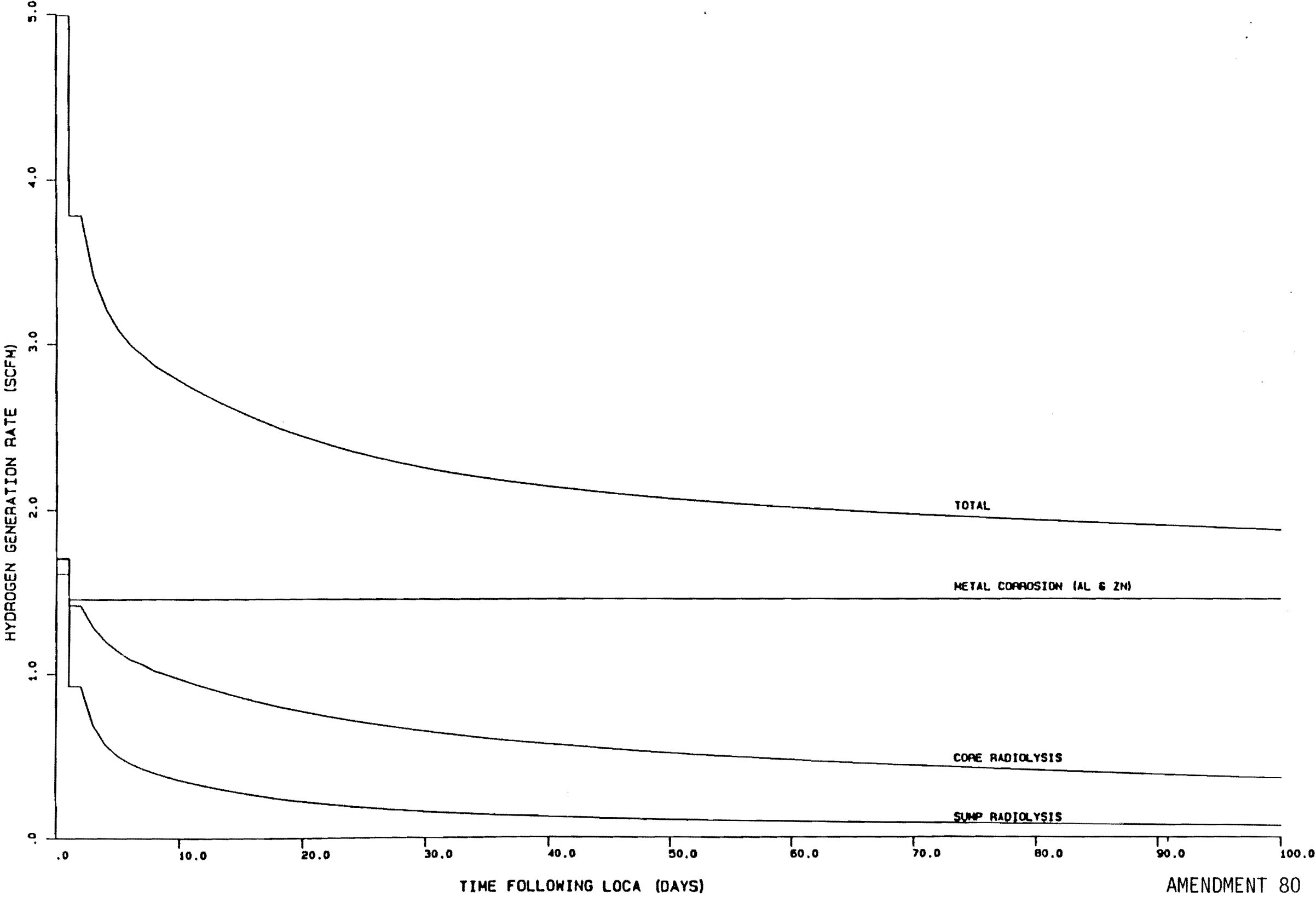
Figure 15.4-4 Hydrogen Generation Rates; NRC Basis
