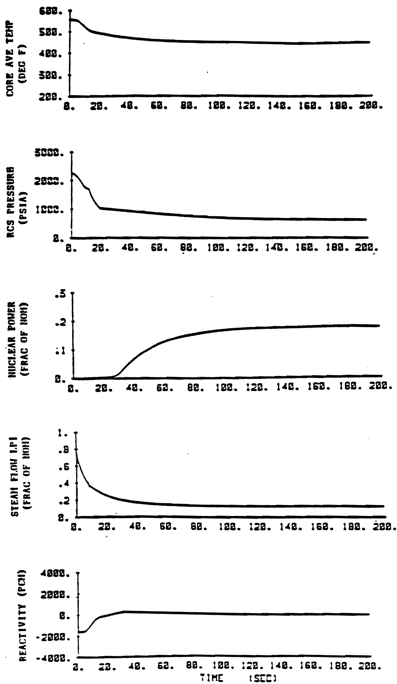
Figure 15.4-11. Transient Response to Steam Line Break with Safety Injection and Offsite Power (case a).
