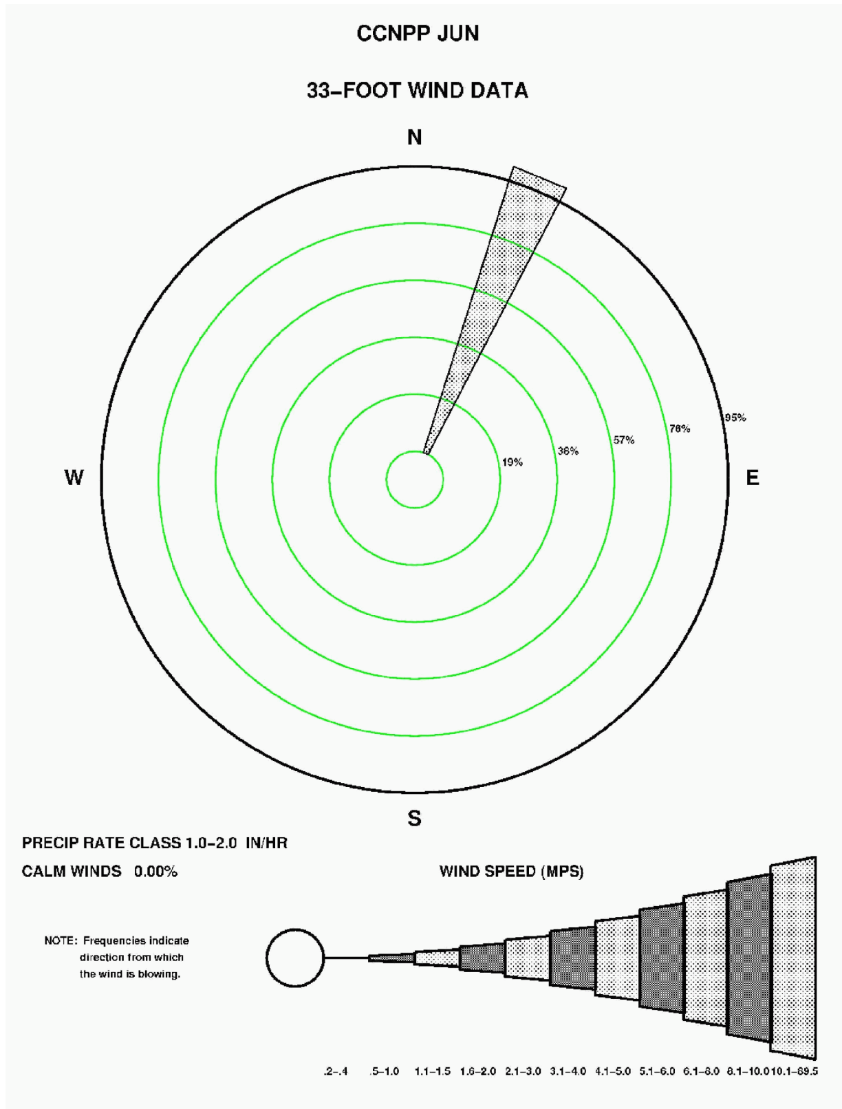
Figure 2.3-83—{CCNPP 33' (10 m) June Precipitation Wind Rose for Rate Class 1.0-2.0 in/hr}
