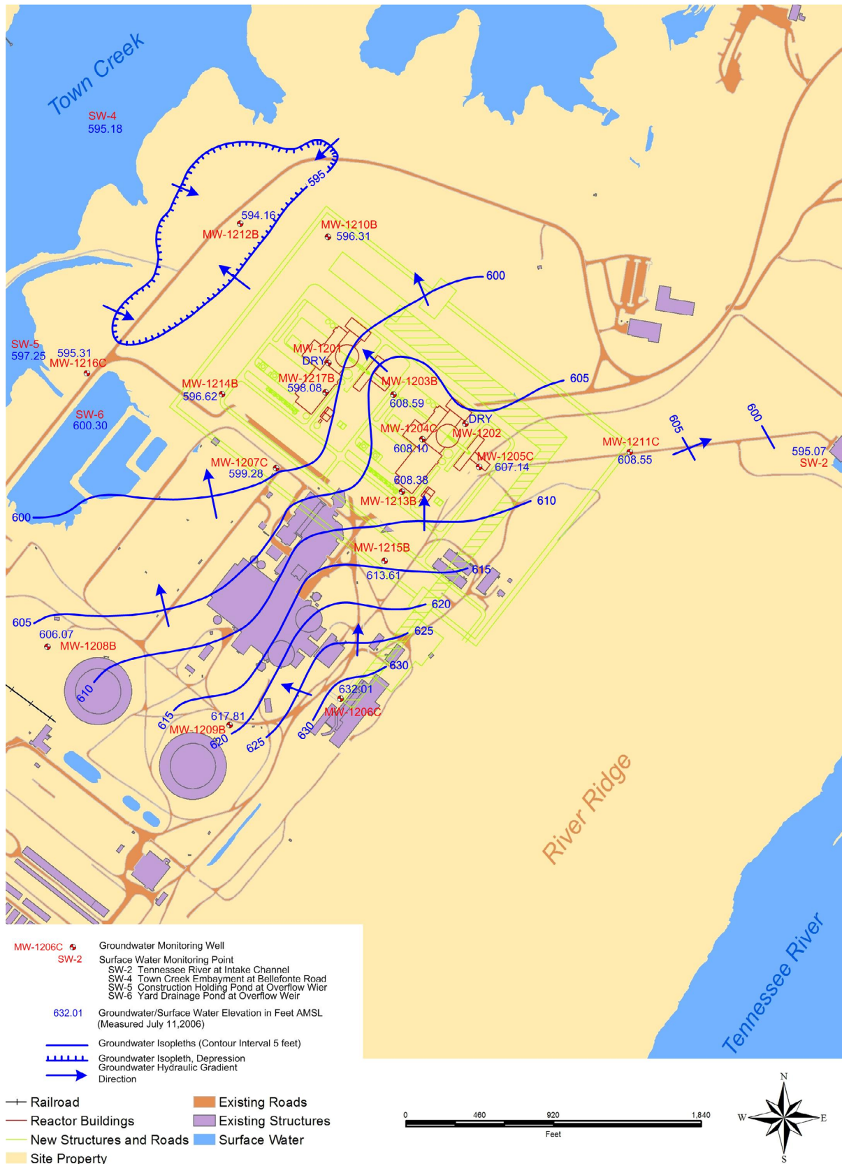
FIGURE 2.4.12-214 July 2006 Groundwater Potentiometric Surface Map
