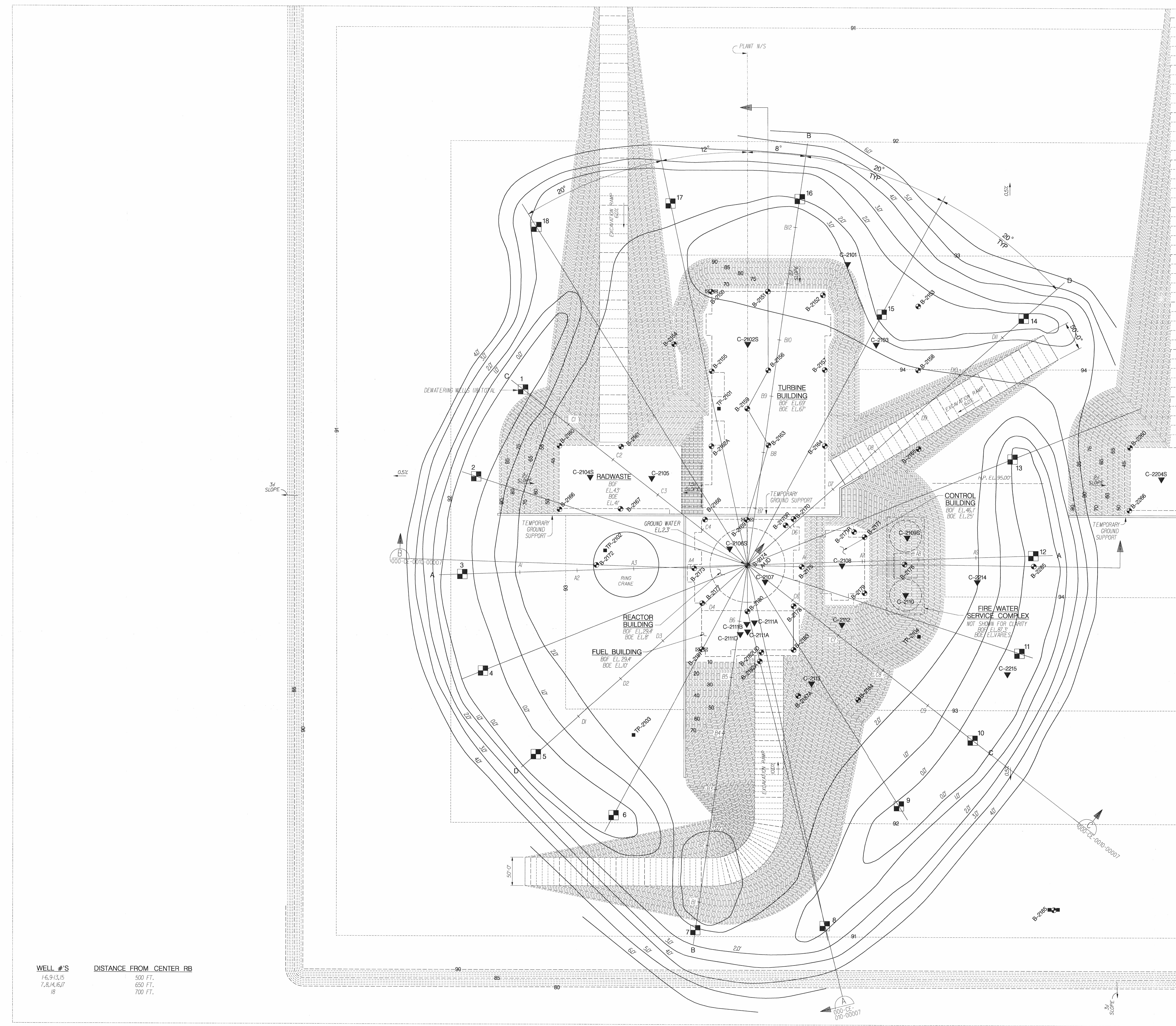
FIGURE 1 - DEWATERING PLAN
