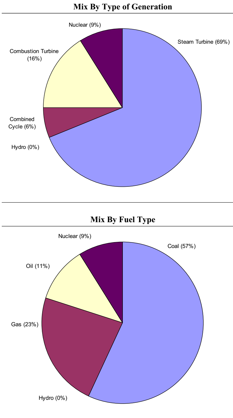
Figure 8.3-1 ITC Transmission Existing Capacity Mix
