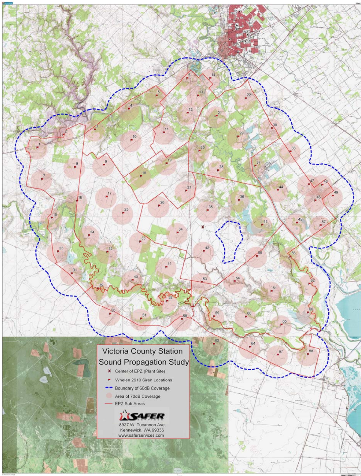
Figure A2 – Proposed VCS EPZ Siren Locations and Coverage
