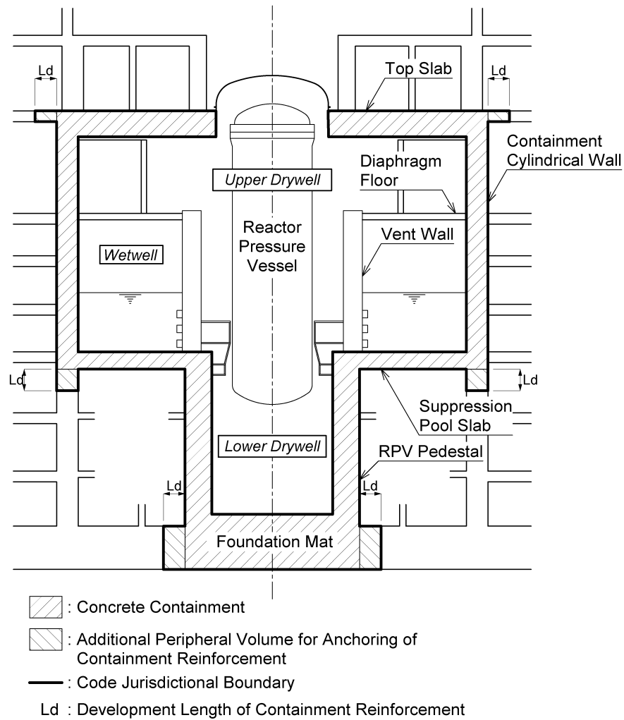
Figure 3.8-1. Configuration of Concrete Containment
