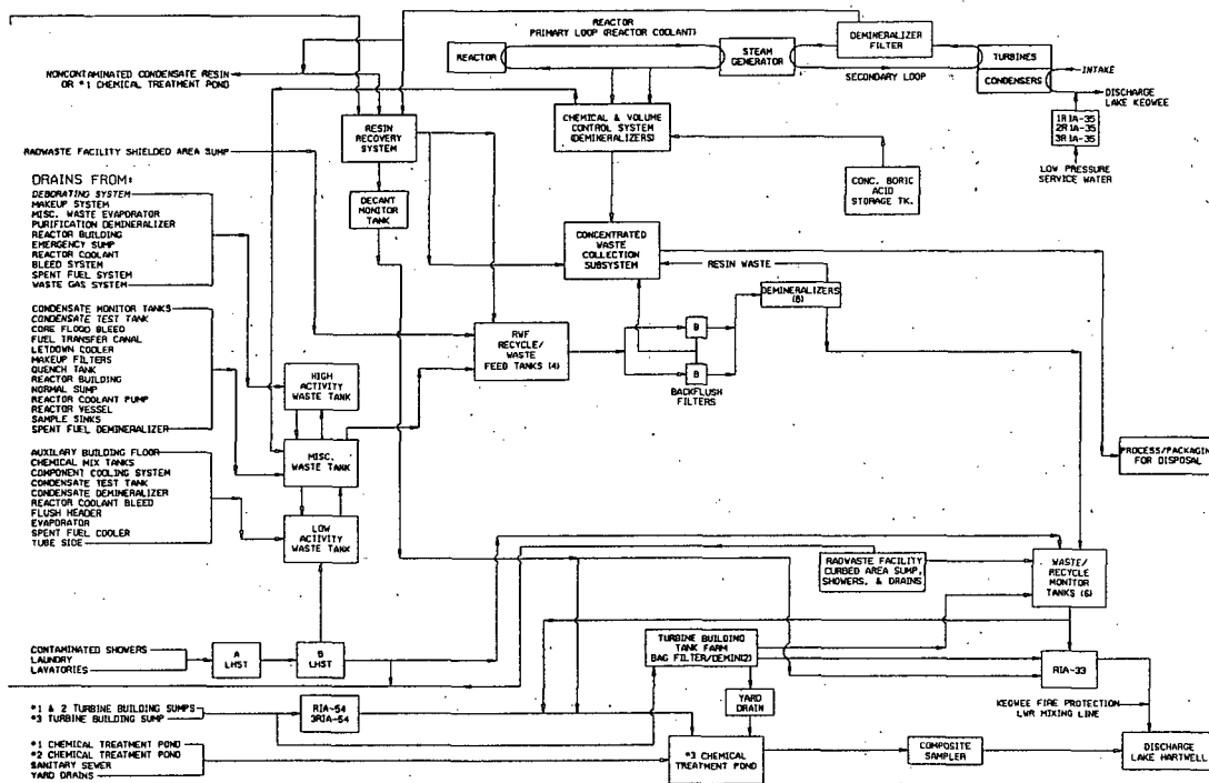
Figure 1.0-1 Oconee Nuclear Station Liquid Radwaste System
