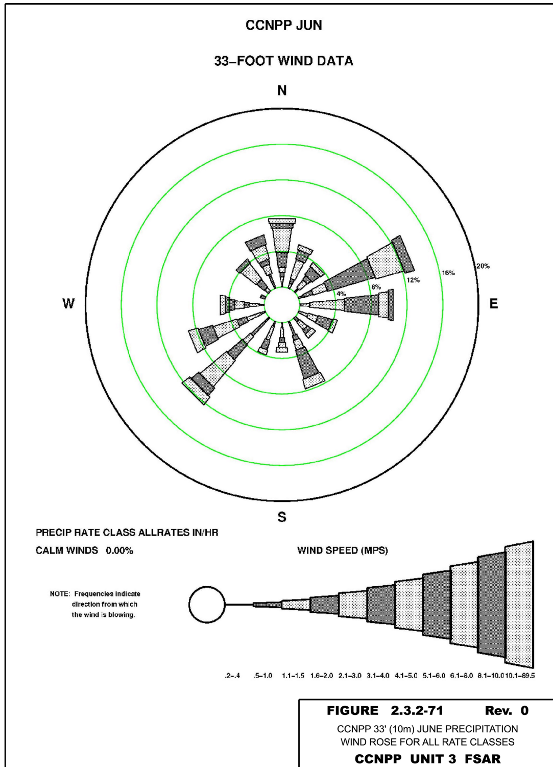
Figure 2.3-84—{CCNPP 33' (10 m) June Precipitation Wind Rose for All Rate classes}
