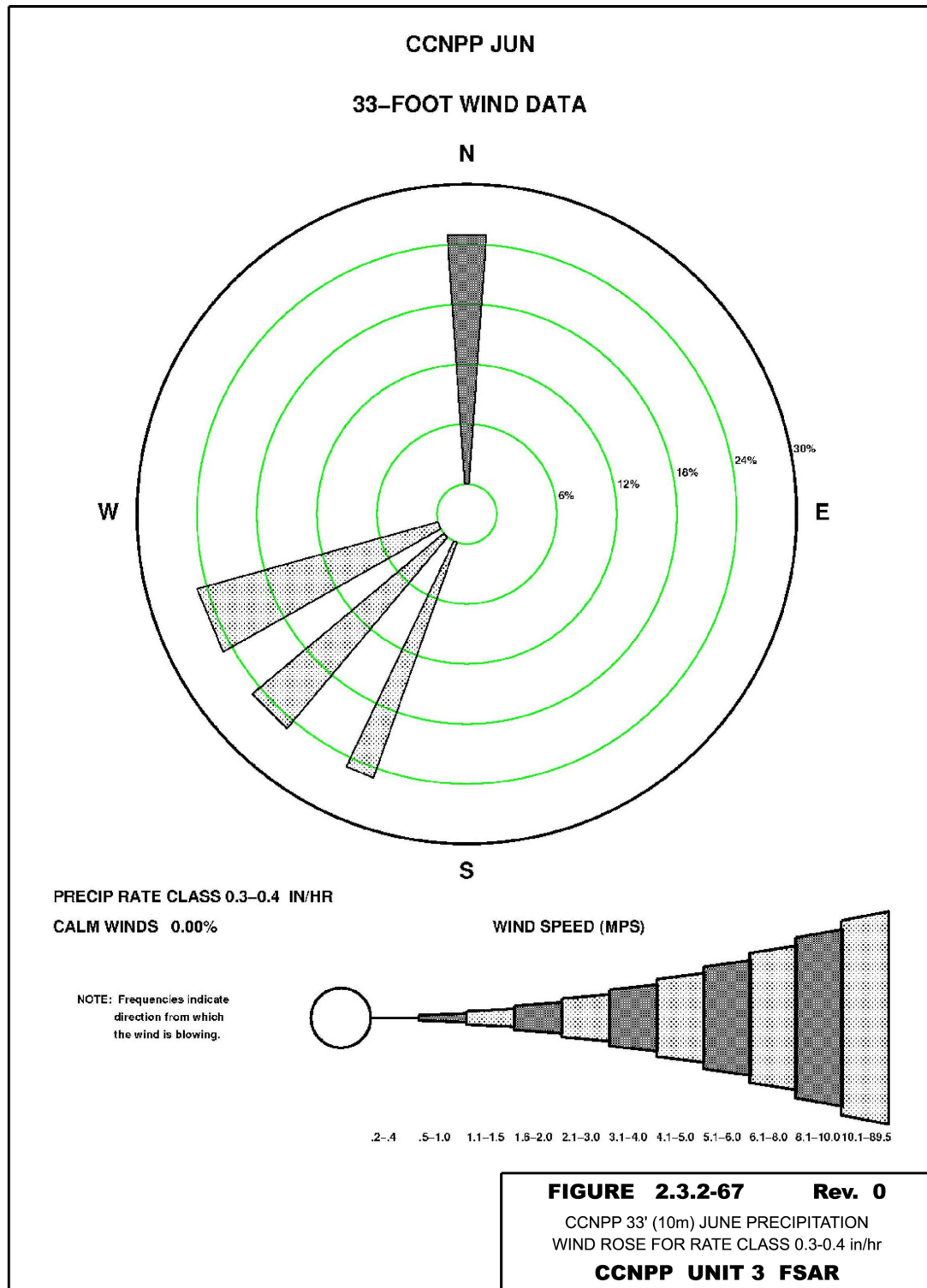
Figure 2.3-80—{CCNPP 33' (10 m) June Precipitation Wind Rose for Rate Class 0.3-0.4 in/hr}
