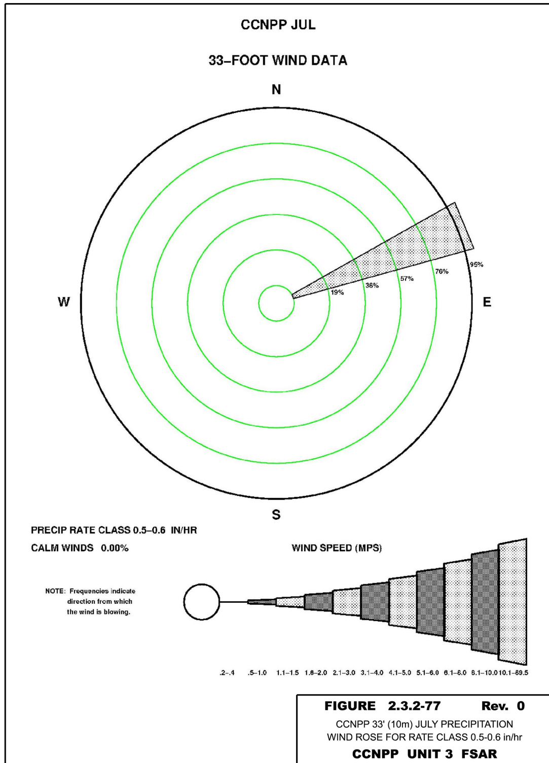
Figure 2.3-90—{CCNPP 33' (10 m) July Precipitation Wind Rose for Rate Class 0.5-0.6 in/hr}
