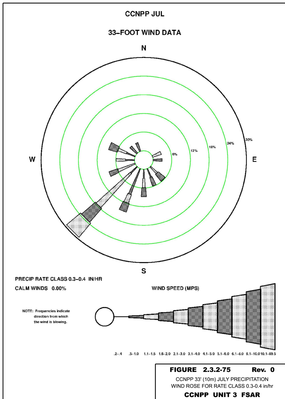
Figure 2.3-88—{CCNPP 33' (10 m) July Precipitation Wind Rose for Rate Class 0.3-0.4 in/hr}
