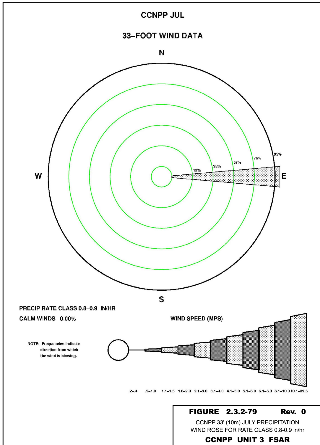
Figure 2.3-92—{CCNPP 33' (10 m) July Precipitation Wind Rose for Rate Class 0.8-0.9 in/hr}
