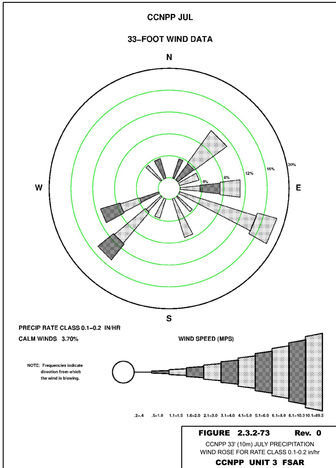
Figure 2.3-86—{CCNPP 33' (10 m) July Precipitation Wind Rose for Rate Class 0.1-0.2 in/hr}
