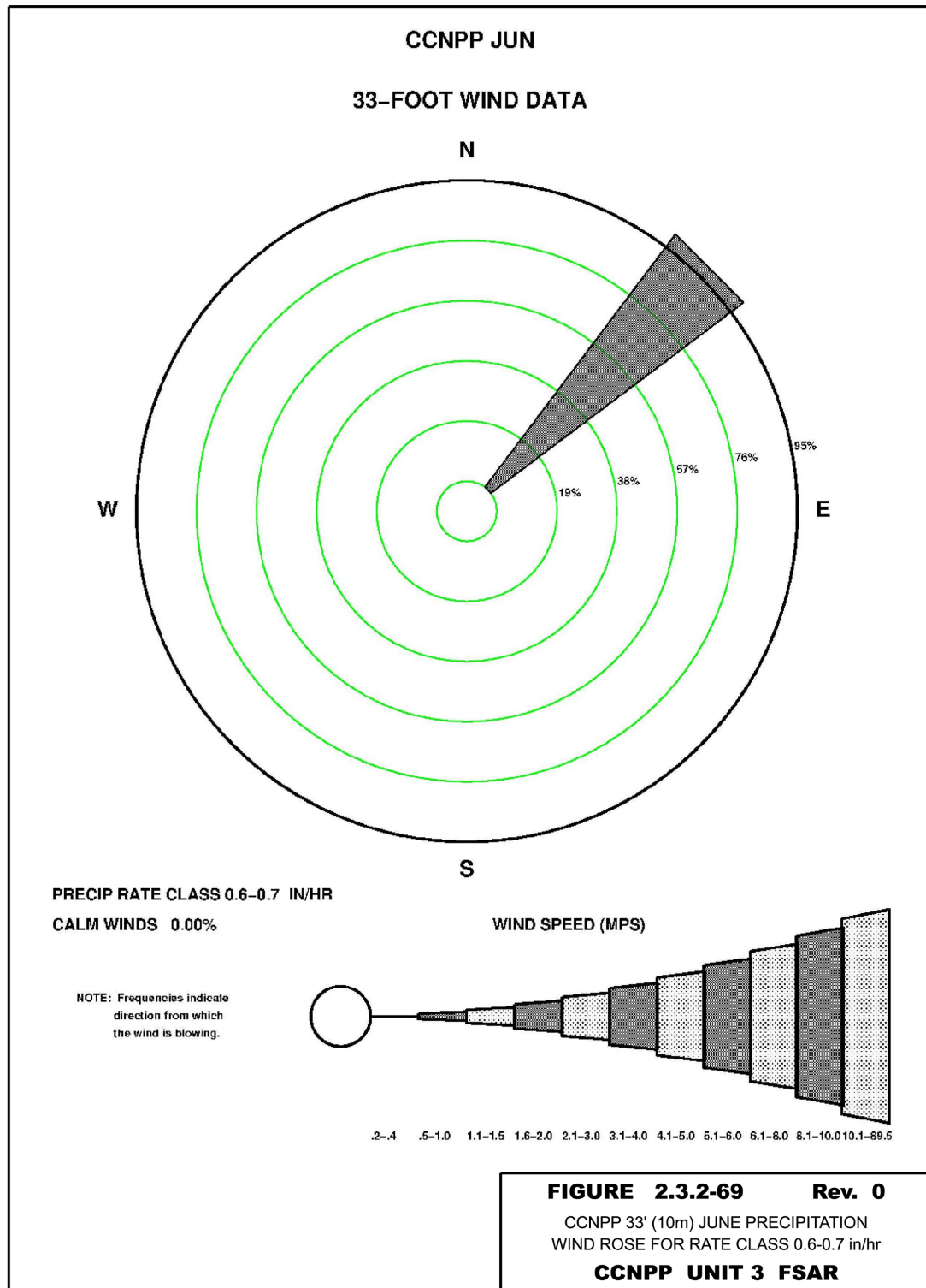
Figure 2.3-82—{CCNPP 33' (10 m) June Precipitation Wind Rose for Rate Class 0.6-0.7 in/hr}
