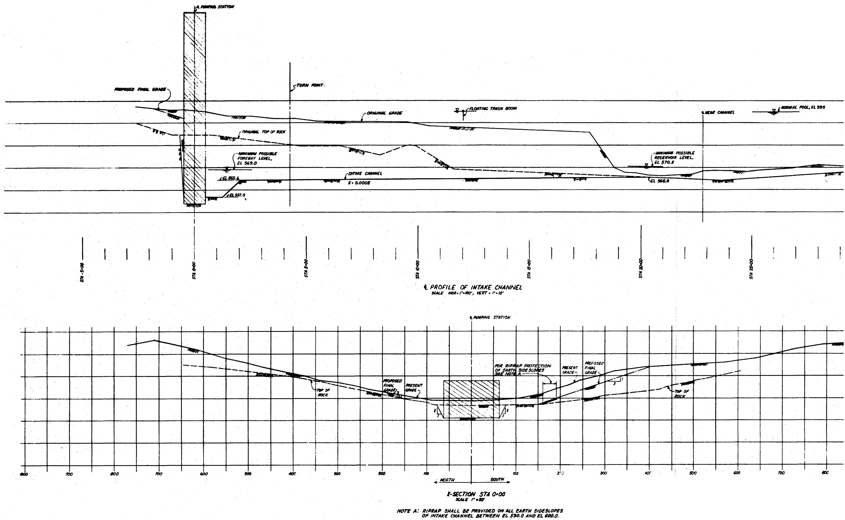
FIGURE 5.3-1 Intake Canal Profile and Section
