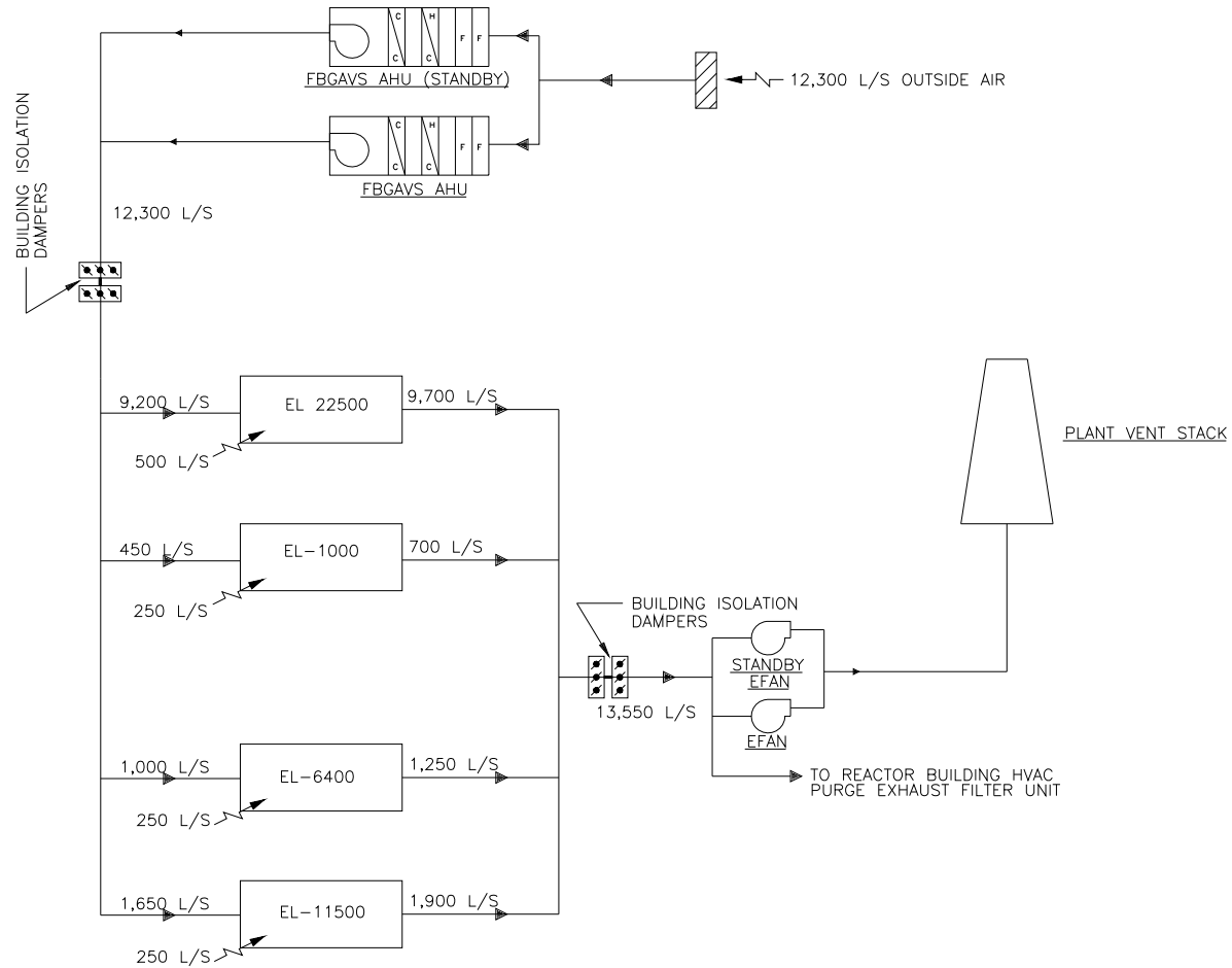
Figure 9.4-5. FBGAVS Simplified System Diagram
