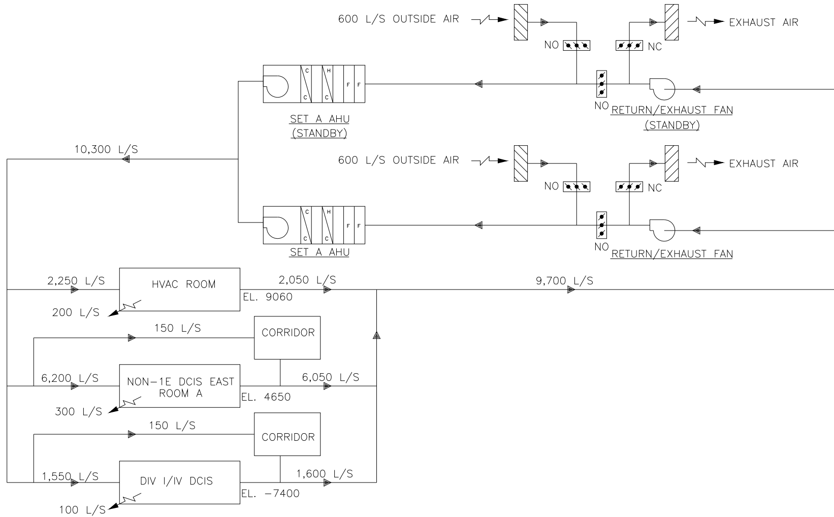
Figure 9.4-3. CBGAVS SET A Simplified System Diagram
