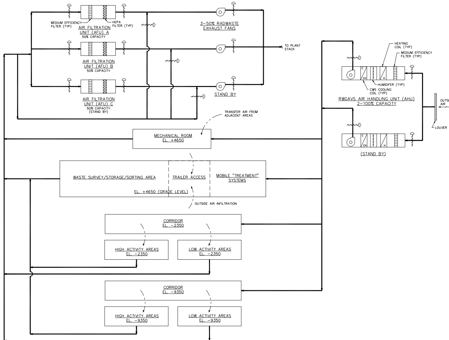
Figure 9.4-7b. RWGAVS Simplified Subsystem Diagram
