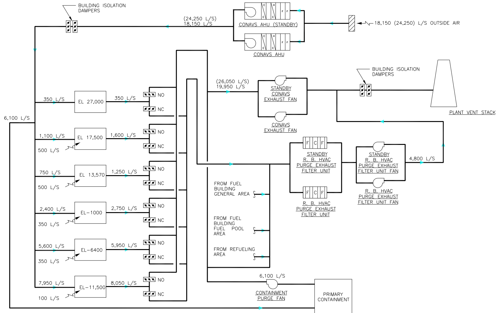
Figure 9.4-10. CONAVS Simplified System Diagram
