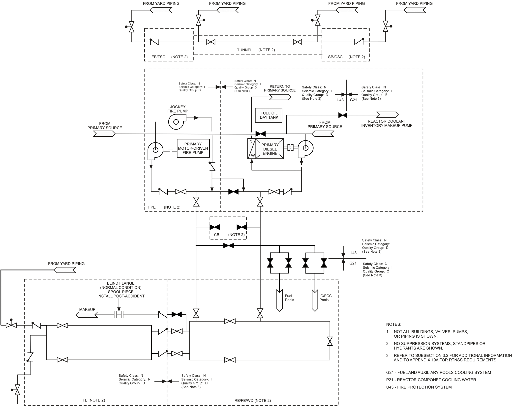
Figure 9.5-1. Fire Protection System Simplified Diagram
