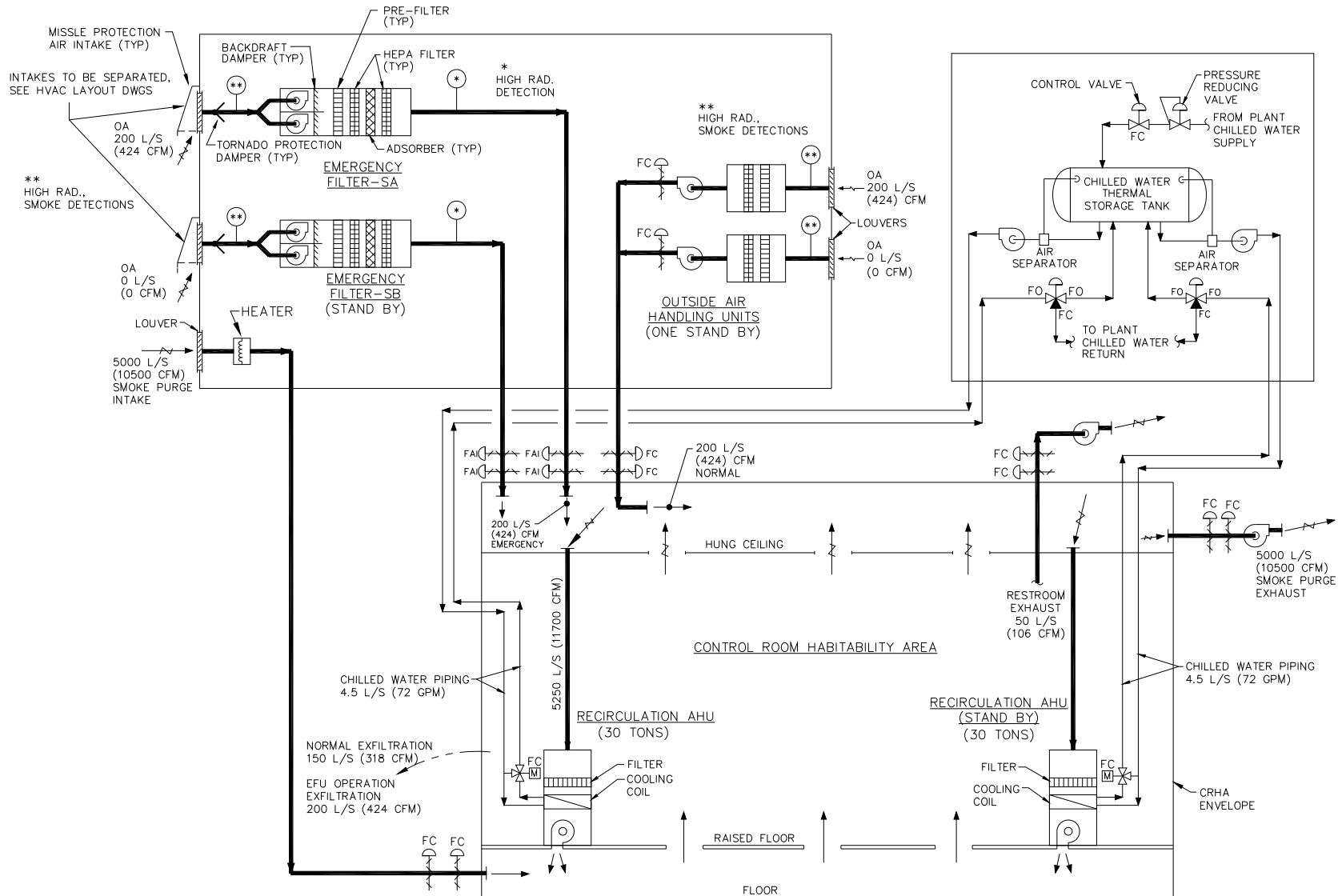
Figure 9.4-1. CRHAVS Simplified System Diagram
