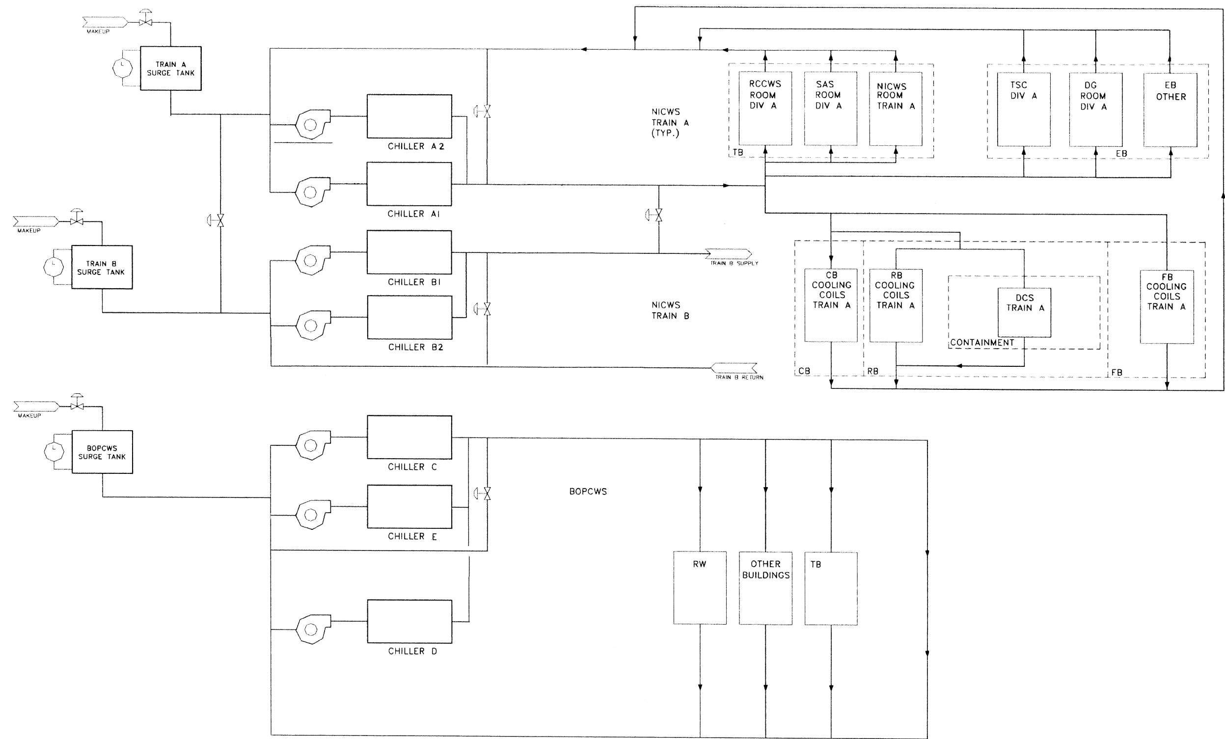
Figure 9.2-3. Chilled Water System Simplified Diagram
