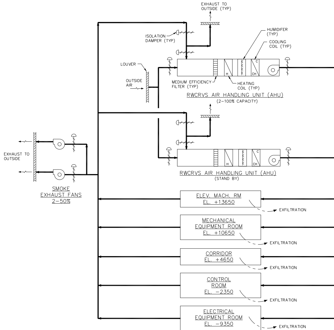
Figure 9.4-7a. RWCRVS Simplified Subsystem Diagram
