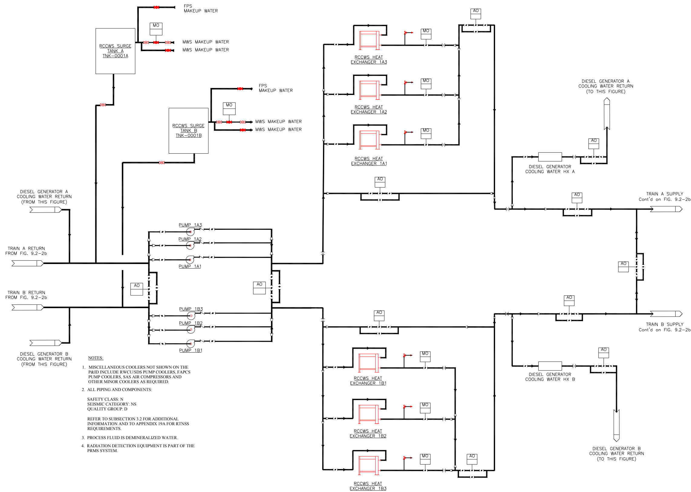
Figure 9.2-2a. Reactor Component Cooling Water System
