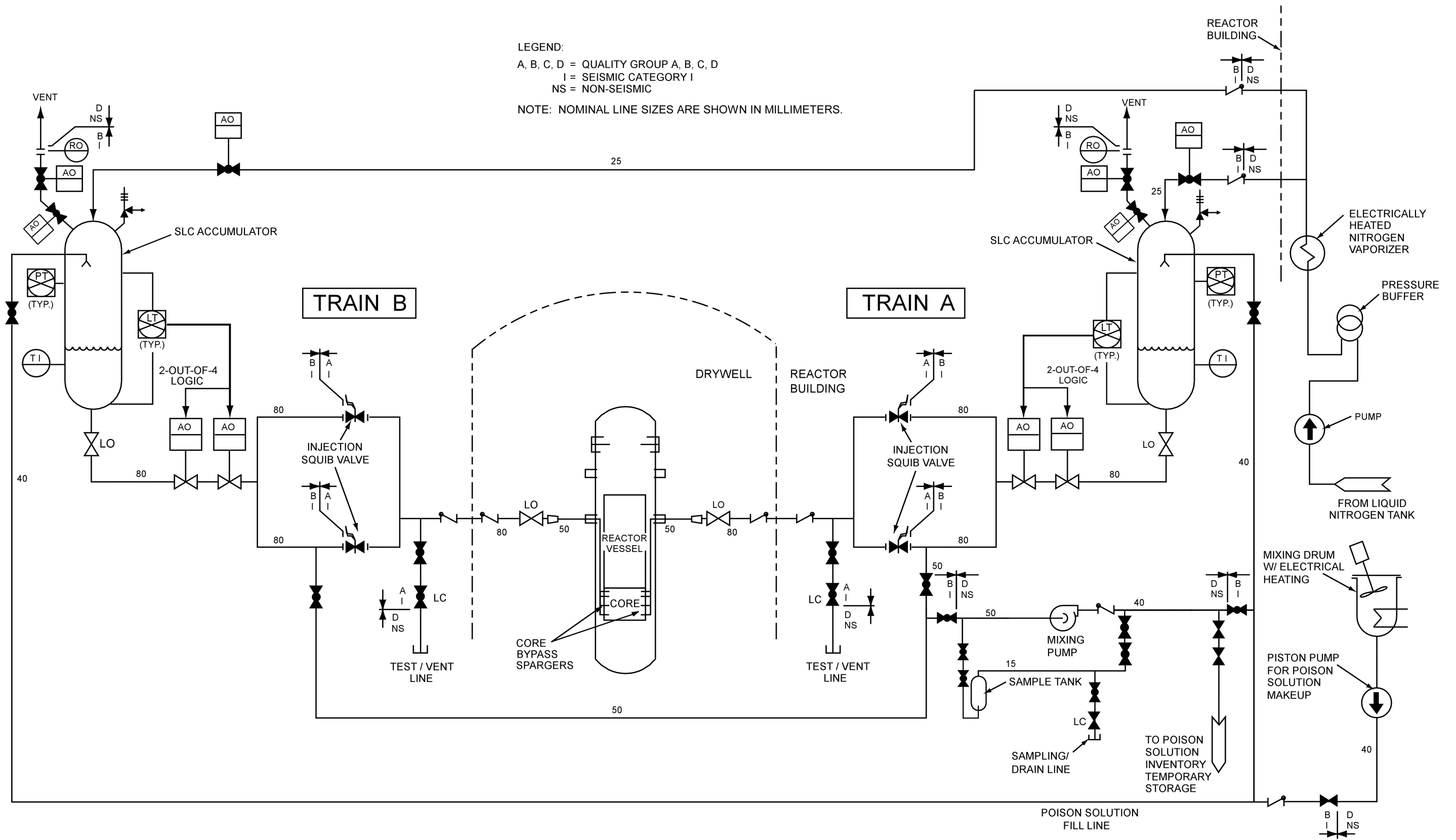
Figure 9.3-1. Standby Liquid Control System Simplified Diagram
