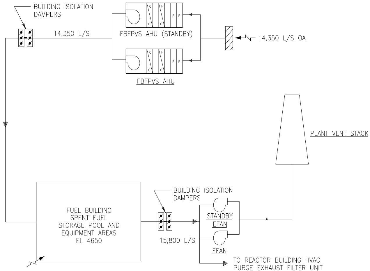
Figure 9.4-6. FBFPVS Simplified System Diagram
