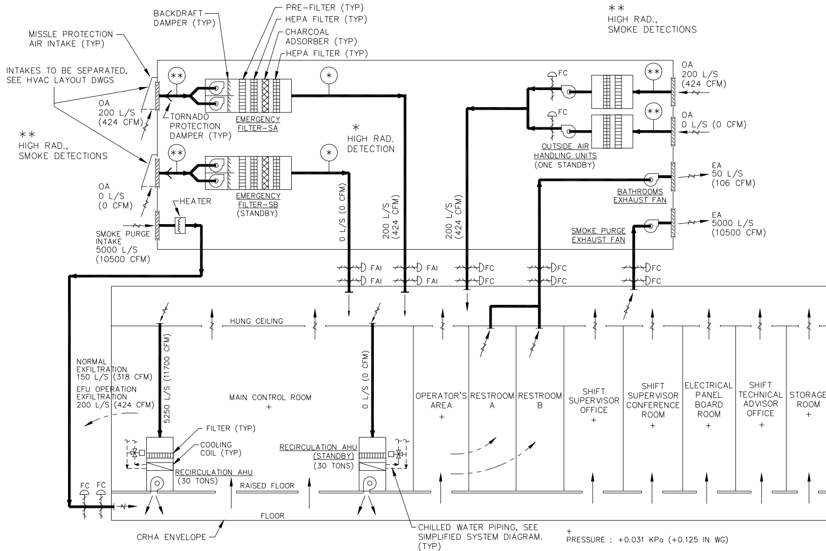
Figure 9.4-2. CRHAVS Air Flow Diagram
