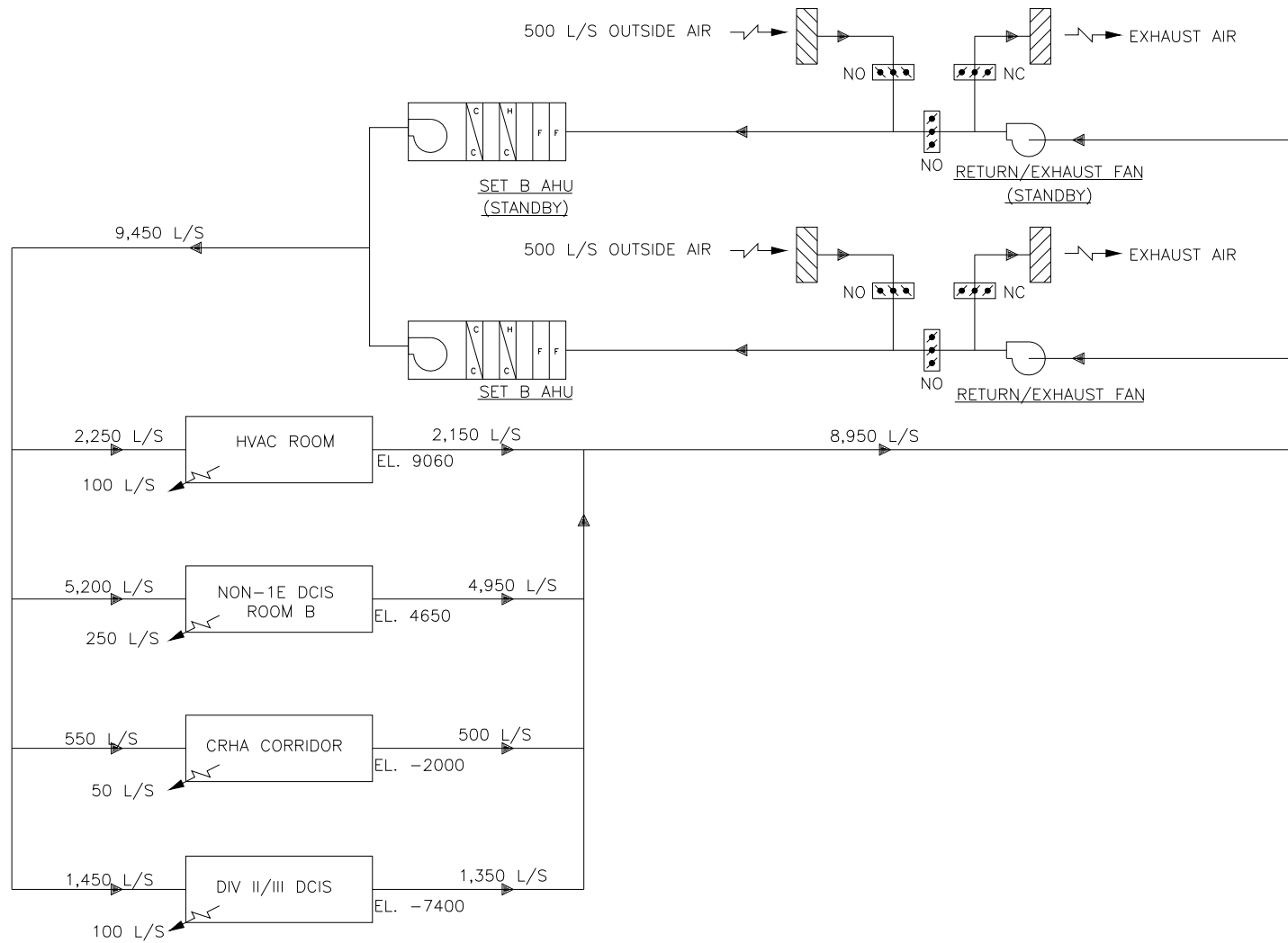
Figure 9.4-4. CBGAVS SET B Simplified System Flow Diagram
