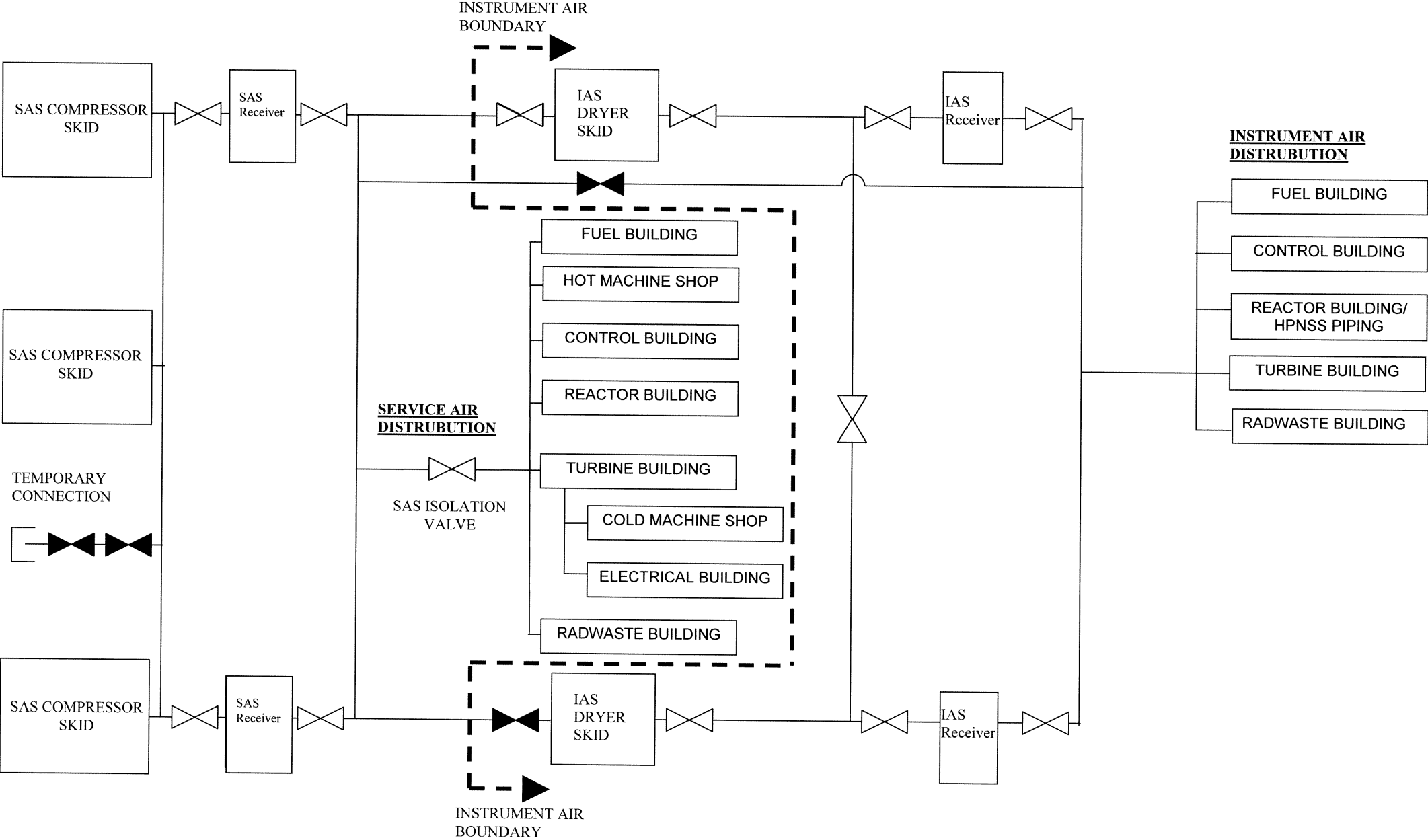
Figure 9.3-3. Service Air and Instrument Air System Simplified Diagram
