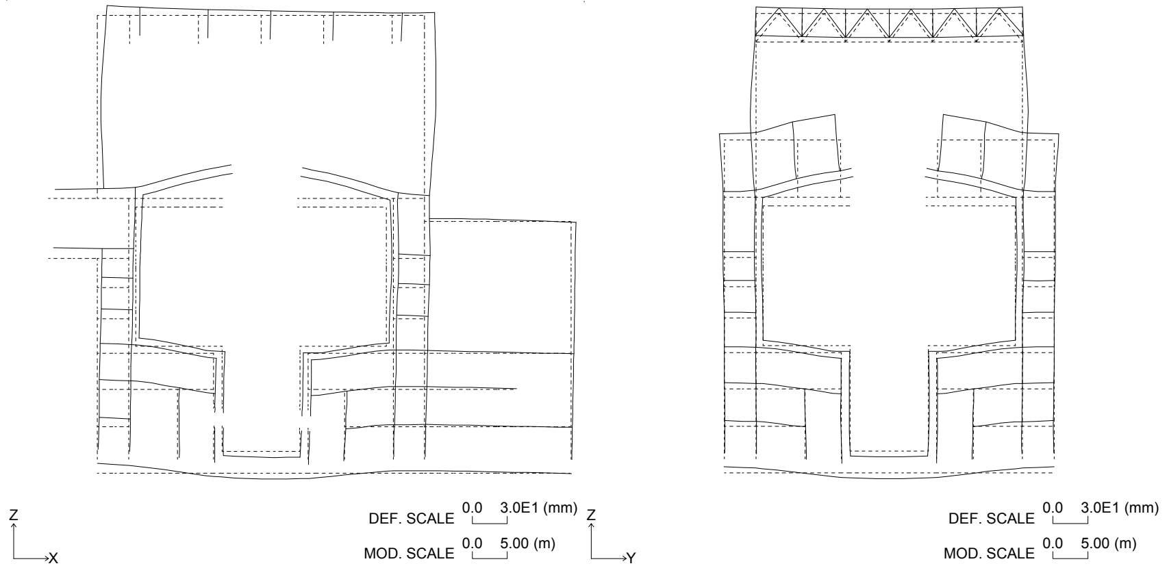
Figure 3G.1-31. Section Deformation for Drywell Unit Pressure (1 MPa)
