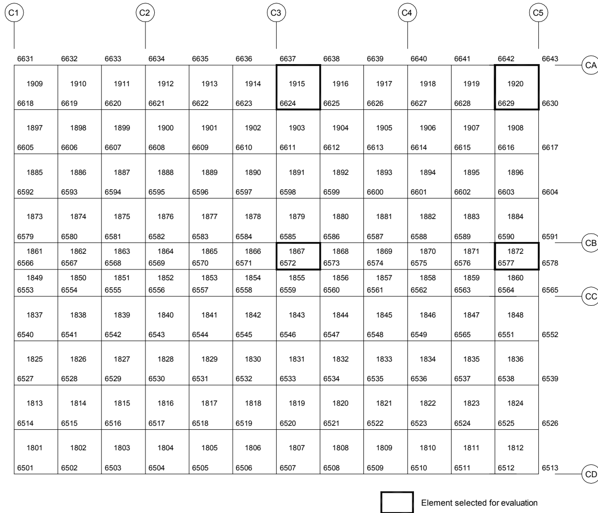
Figure 3G.2-11. FE Model of CB (Roof: EL 13800)
