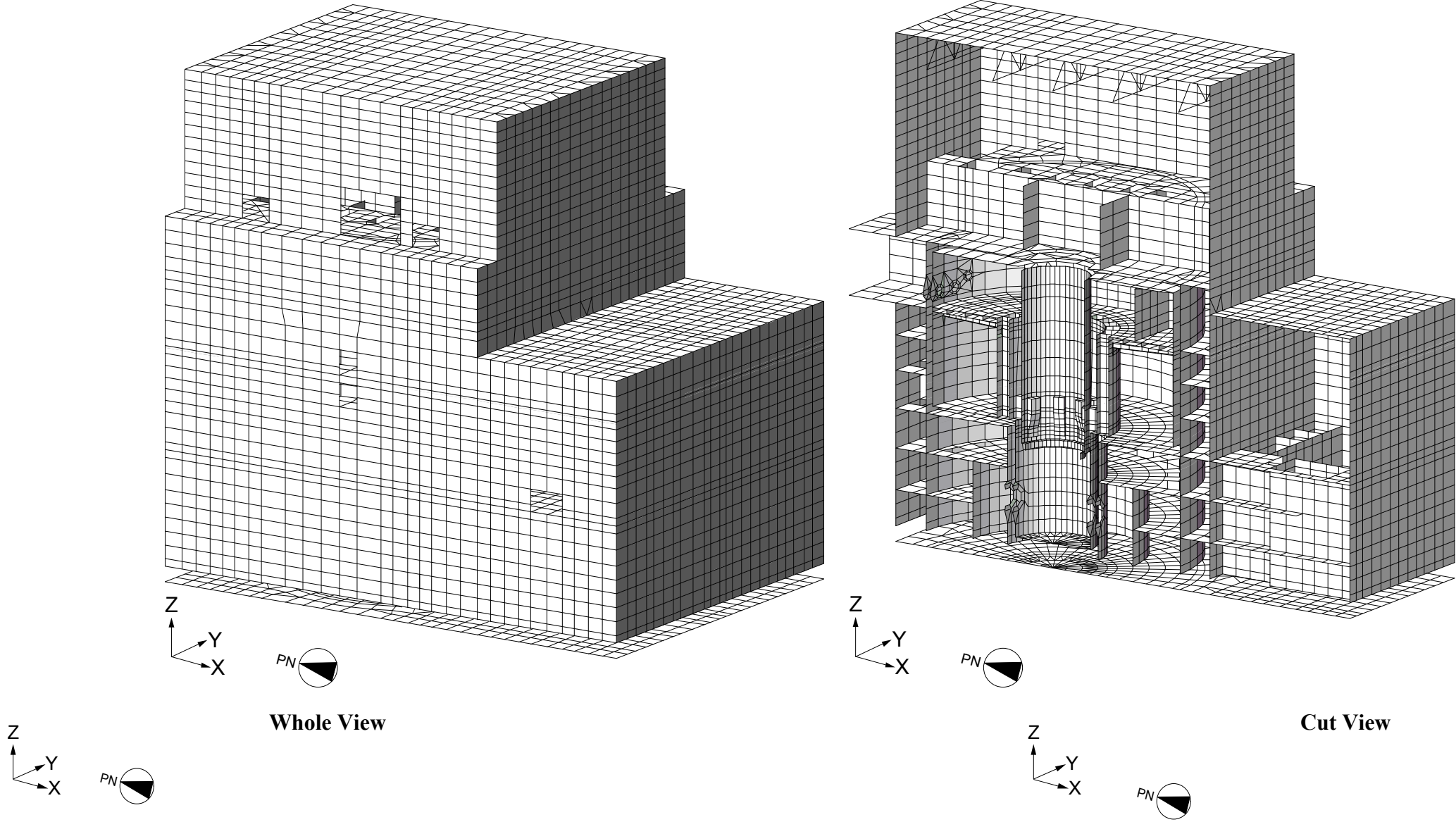
Figure 3G.1-8. FE Model of RB/FB (Isometric View)
