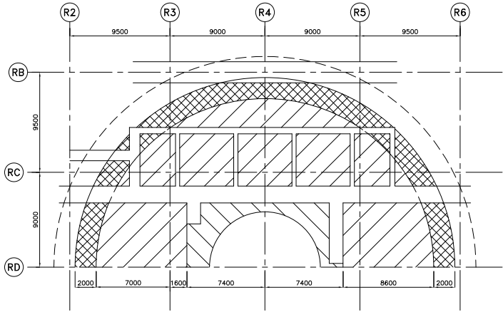
SECTION AT 180°
