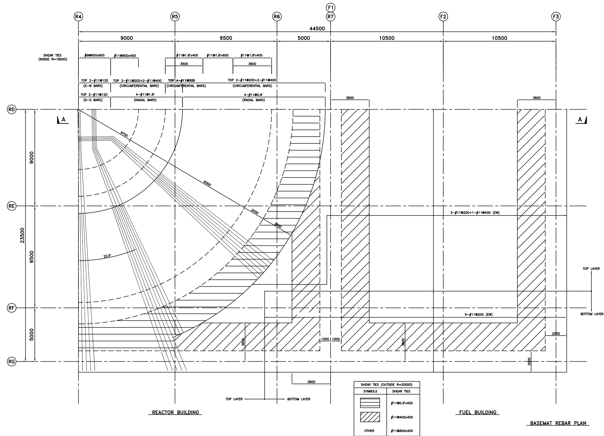
Figure 3G.1-40. Reinforcing Steel of Foundation Mat: Plan
