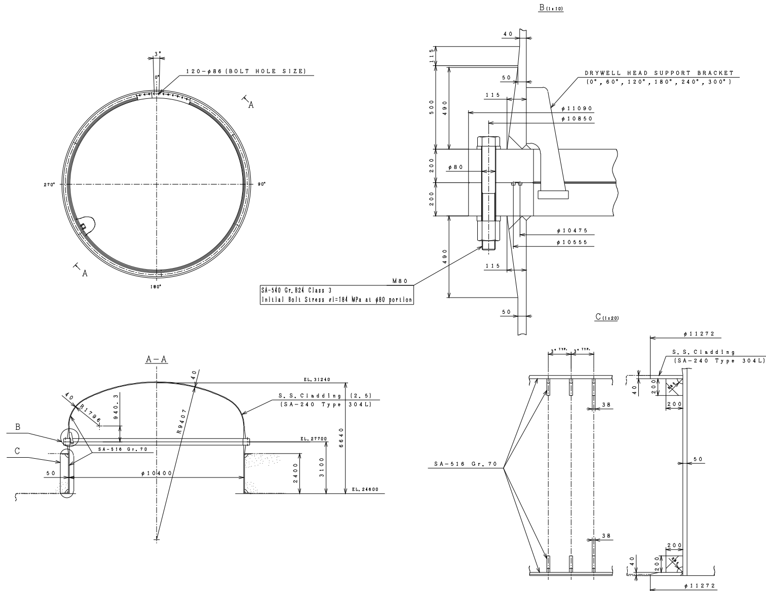
Figure 3G.1-51. Drywell Head
