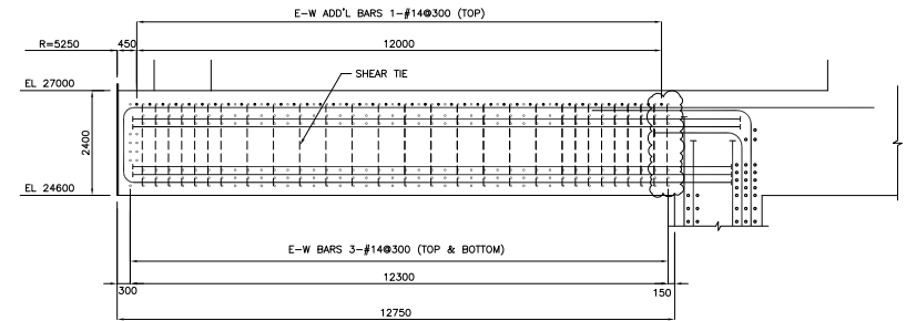
SECTION AT 180°
