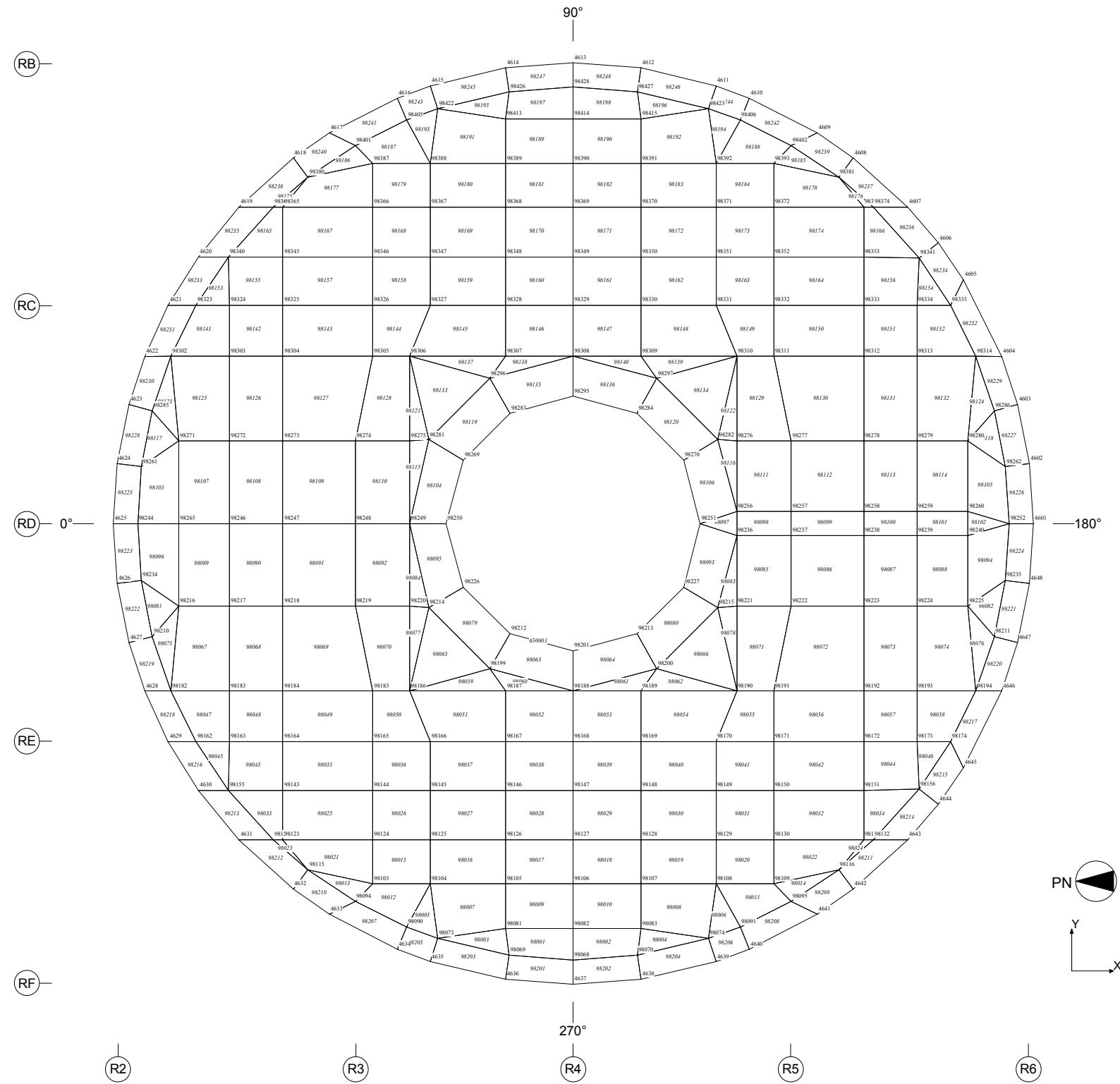
Figure 3G.1-12. FE Model of RB/FB (Top Slab)
