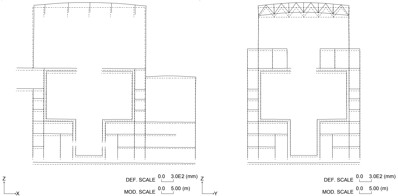
Figure 3G.1-38. Section Deformation for Seismic Load (Vertical: Upward)
