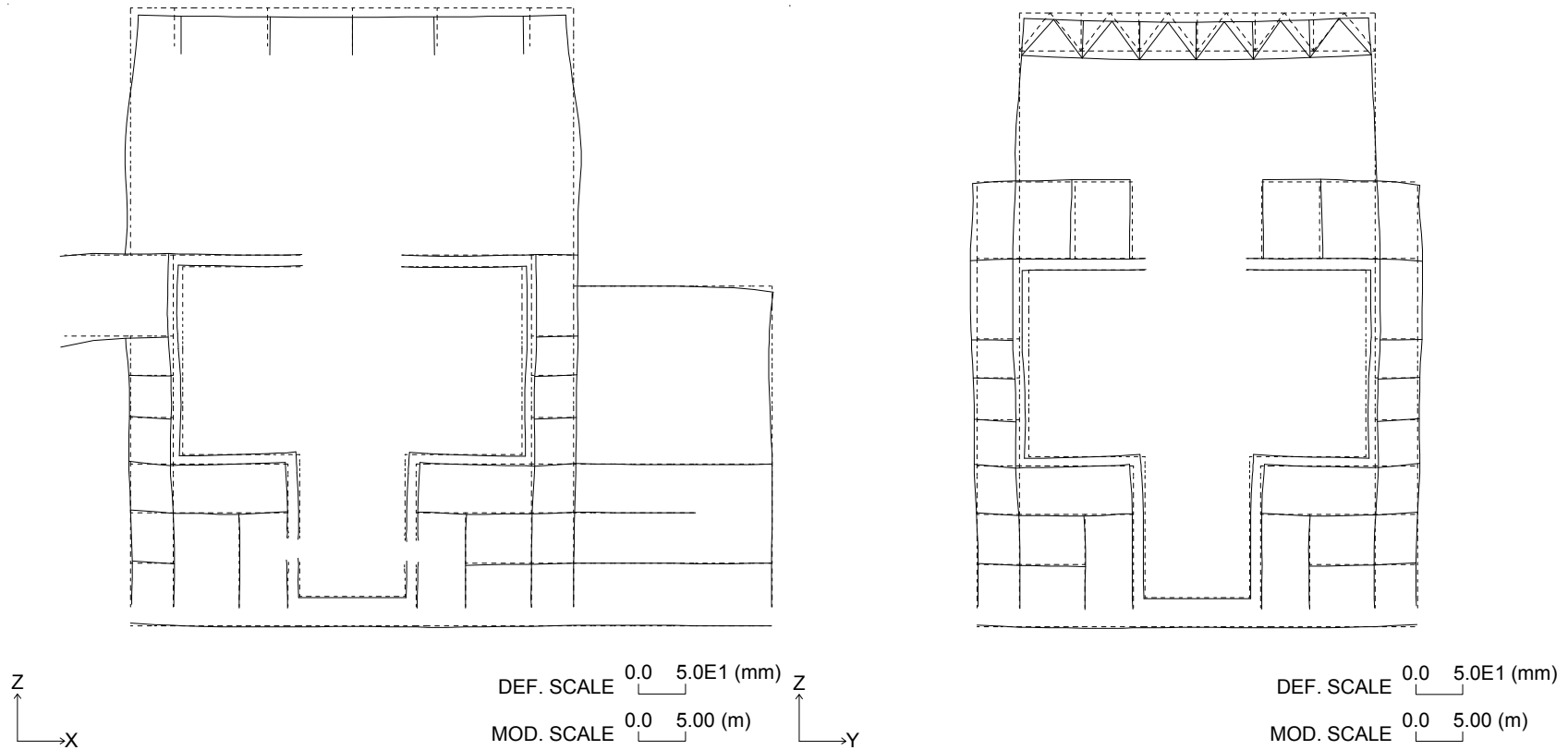
Figure 3G.1-34. Section Deformation for Thermal Load (LOCA After 6 min.: Winter)
