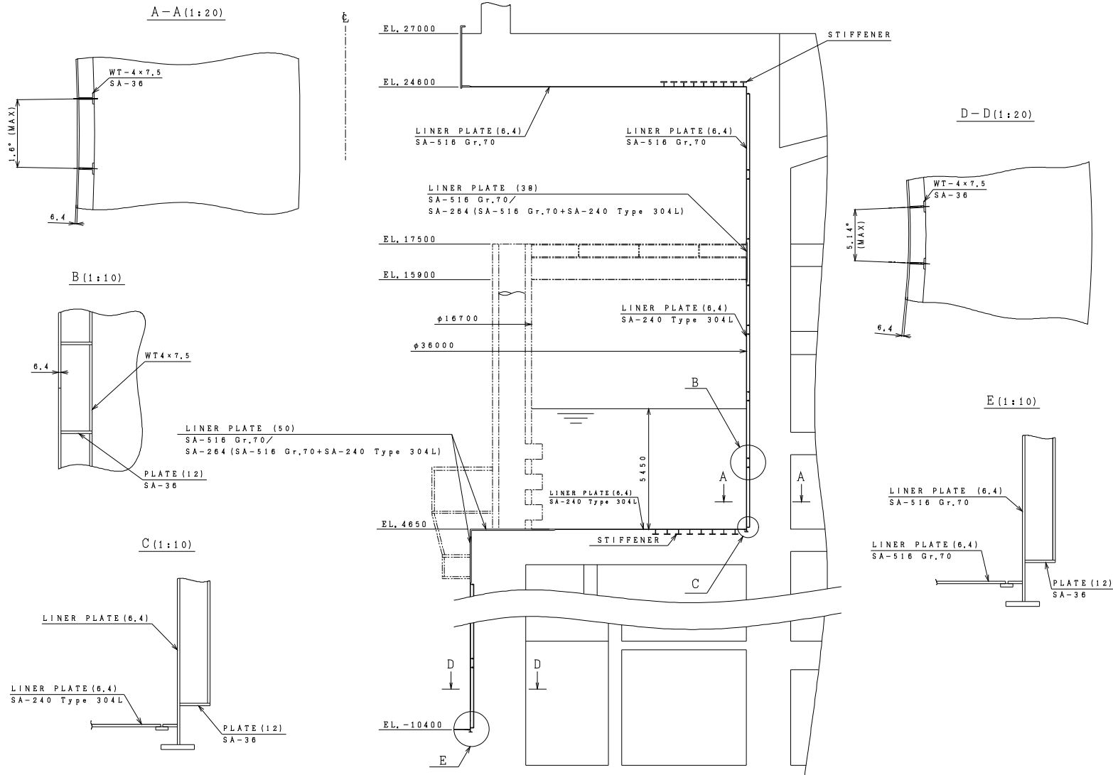
Figure 3G.1-48. Liner Anchor
