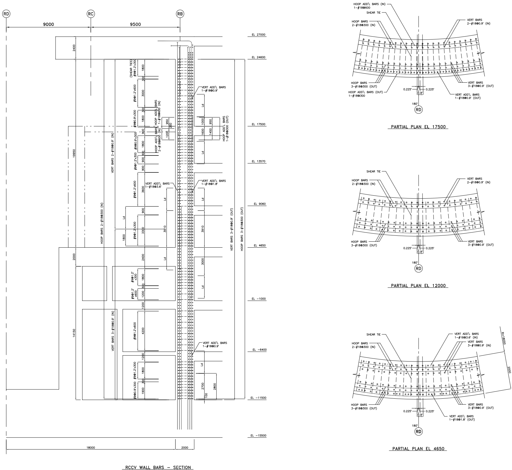
Figure 3G.1-42. Reinforcing Steel of RCCV Wall
