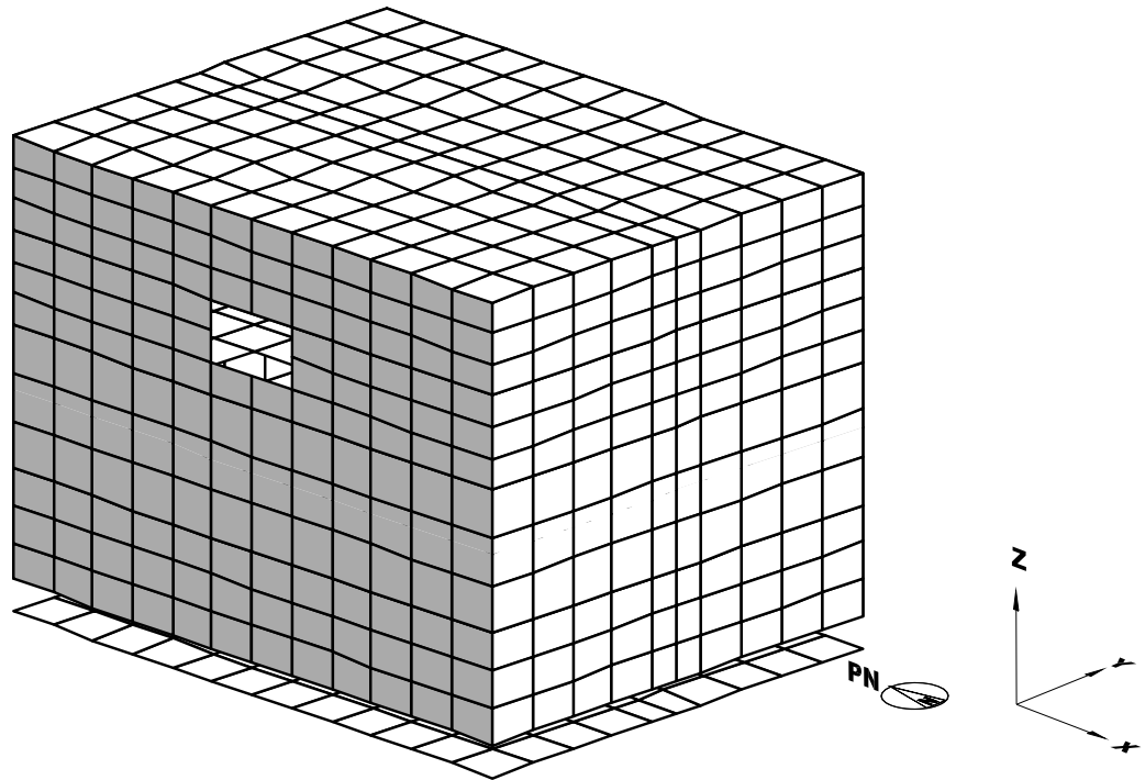
Whole View
