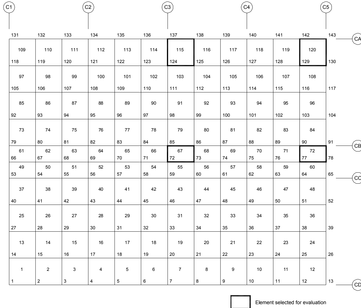
Figure 3G.2-5. FE Model of CB (Foundation Mat)
