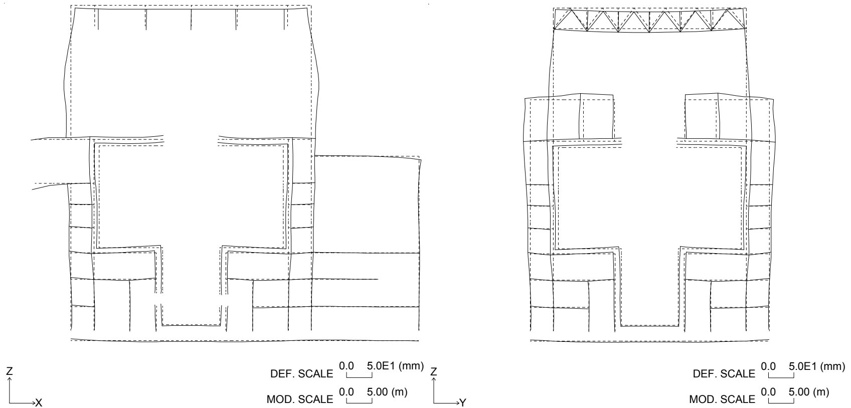
Figure 3G.1-35. Section Deformation for Thermal Load (LOCA After 72 hr.: Winter)
