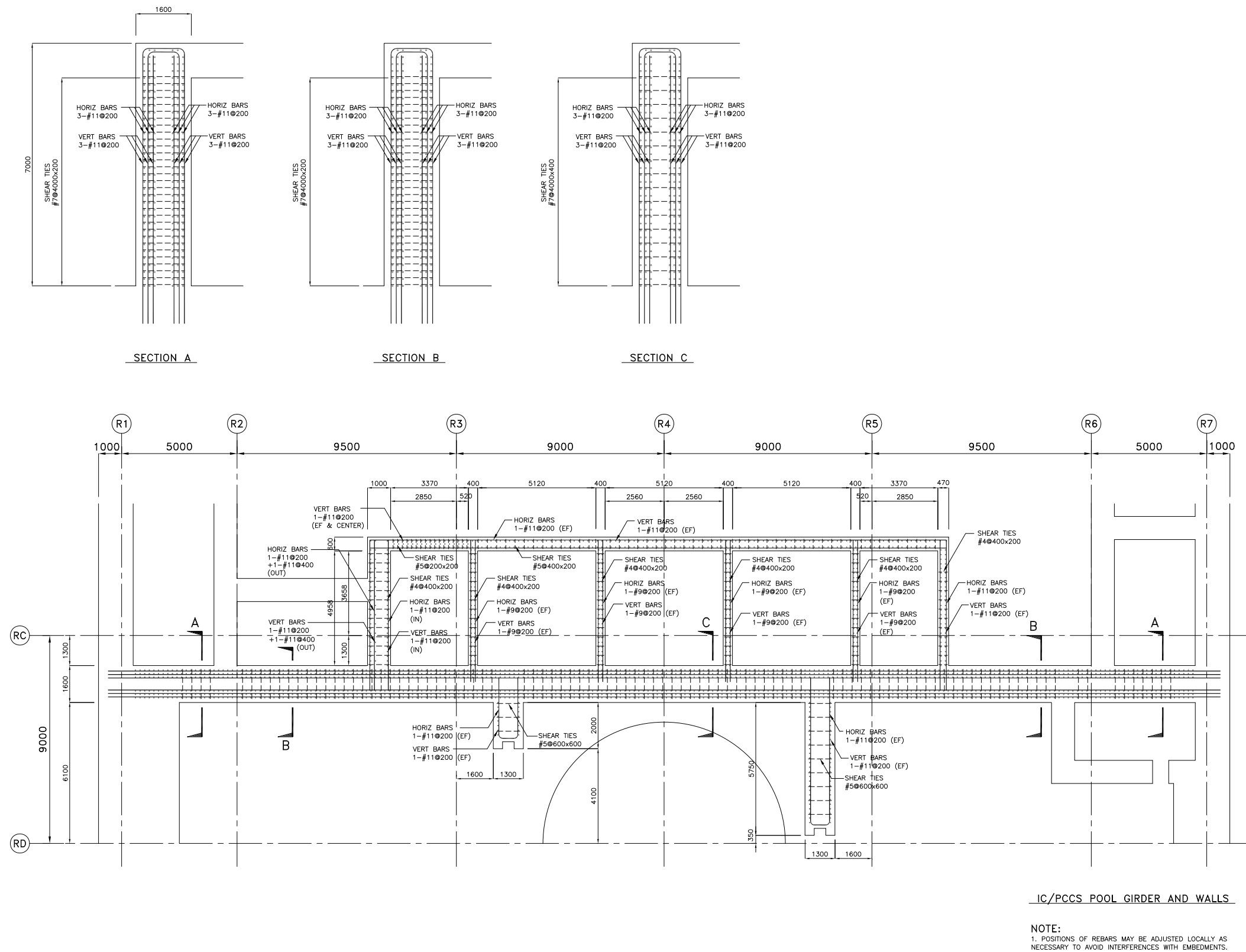
Figure 3G.1-46. Reinforcing Steel of IC/PCCS Pool Girder
