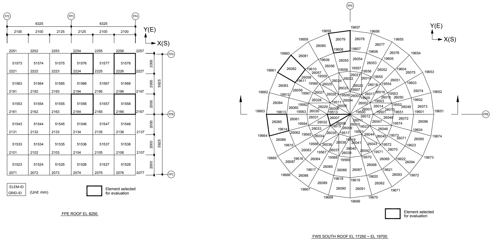
Figure 3G.4-6. FE Model of FWSC (FPE Roof Slab, South FWS Roof Slab)
