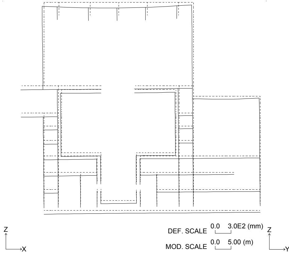
Figure 3G.1-30. Section Deformation for Dead Load
