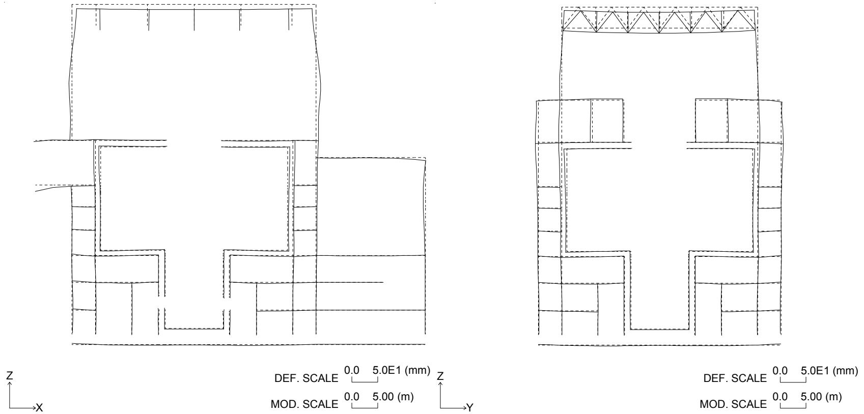
Figure 3G.1-33. Section Deformation for Thermal Load (Normal Operation: Winter)
