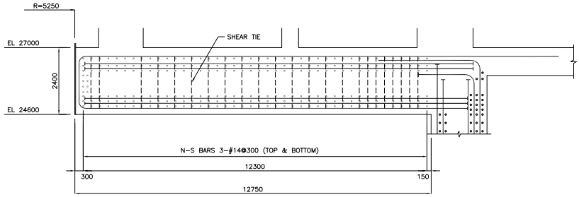
SECTION AT 90°
