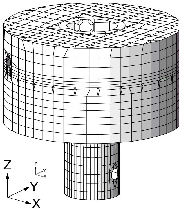
Whole View
