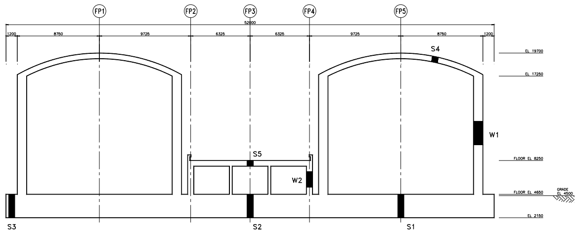
Figure 3G.4-7. Sections Where Thermal Loads Are Defined
