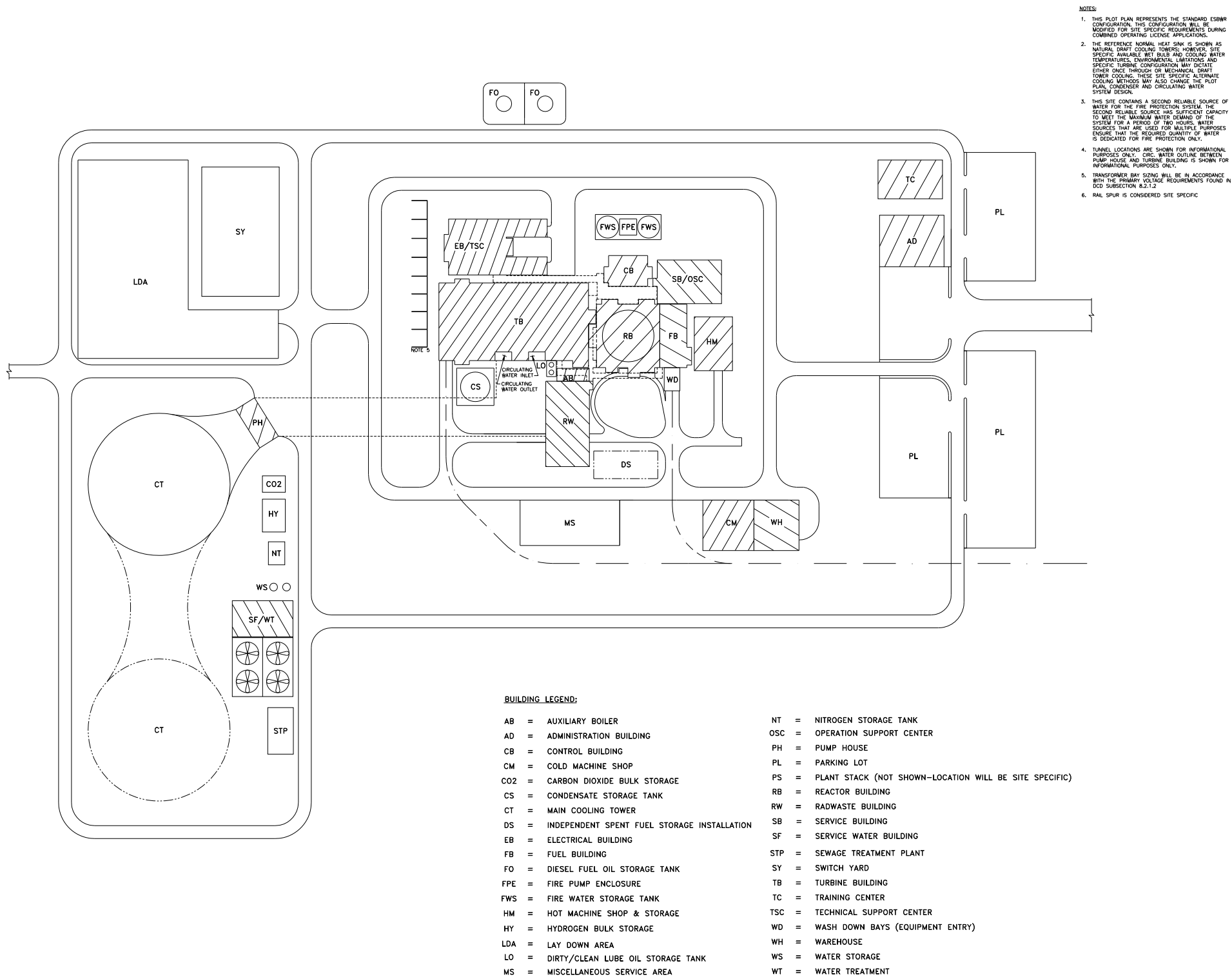
Figure 1.1-1. ESBWR Standard Plant General Site Plan
