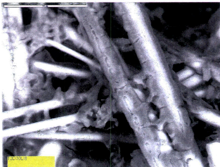
Figure 4-52. Higher-magnification ESEM image of a Test #2, Day-30 low-flow interior fiberglass sample.
