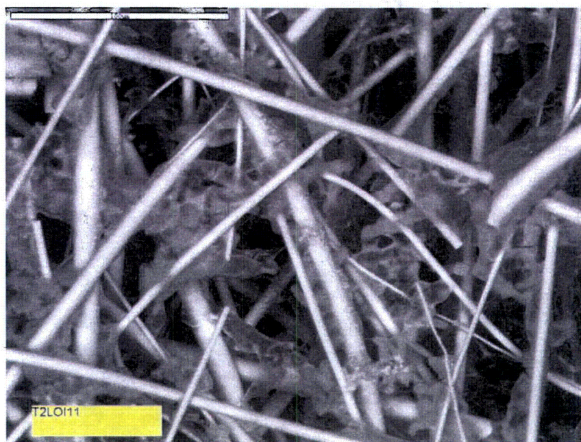
Figure 4-48. Higher-magnification ESEM image of a Test #2, Day-16 interior low-flow fiberglass sample.
