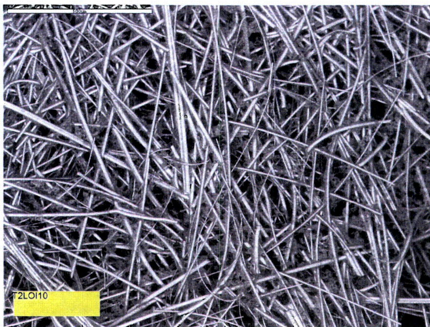
Figure 4-47. ESEM image overview of a Test #2, Day-16 interior low-flow fiberglass sample.
