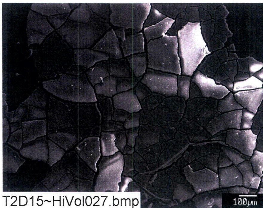
Figure A-1. SEM image at 120× magnification for a Test #2, Day-15 sample of particles on the high-volume filter. (T2D15_HiVol027)
