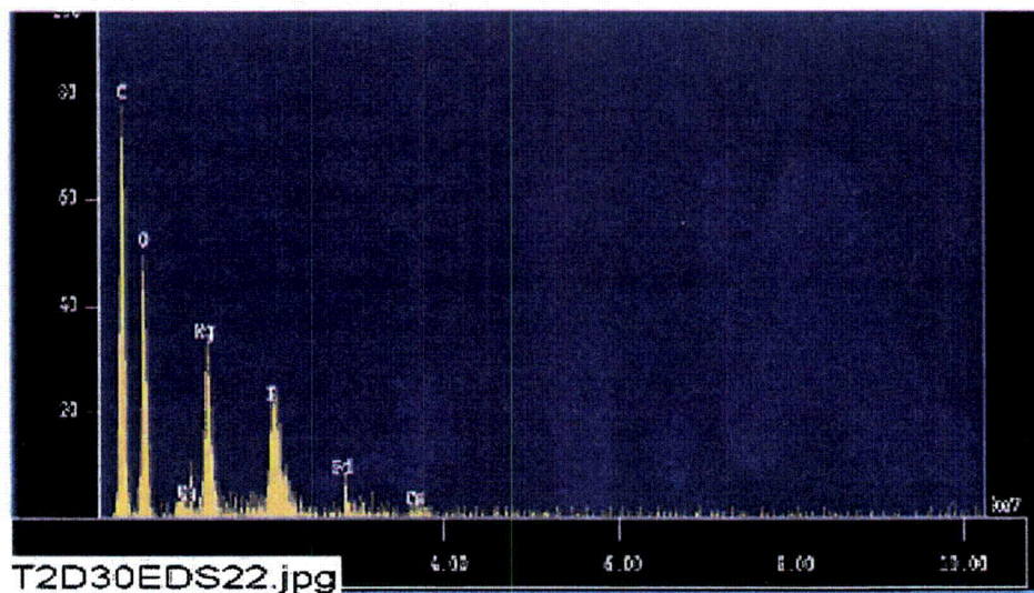
Figure 4-59. EDS counting spectrum for the lathlike crystal on the lower left side of Figure 4-58. From left to right, the element peaks are carbon, oxygen, sodium, magnesium, phosphorus, palladium (coating substance for SEM analyses), and calcium.
