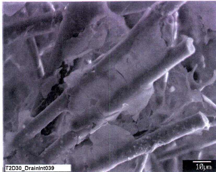
Figure 4-69. Higher-magnification SEM image of a Test #2, Day-30 interior fiberglass sample on the drain collar. The image shows flocculence or growth on the fiberglass.
