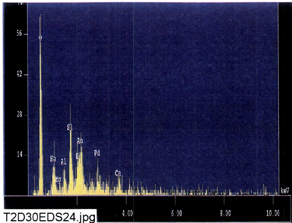
Figure 4-62. EDS counting spectrum for the flocculence on the fiberglass, as shown in Figure 4-61. From left to right, the element peaks are oxygen, sodium, magnesium, aluminum, silicon, phosphorus, gold, palladium, and calcium. (Gold and palladium are coating substances for SEM analyses.)
