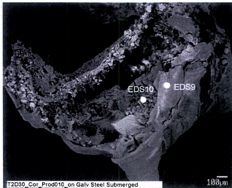
Figure B-17. Backscatter SEM image at 55× magnification for a Test #2, Day-30 sample of corrosion products on a submerged GS coupon, annotated to show EDS sample locations. (T2D30_Cor_Prod010_on Galv Steel Submerged)
