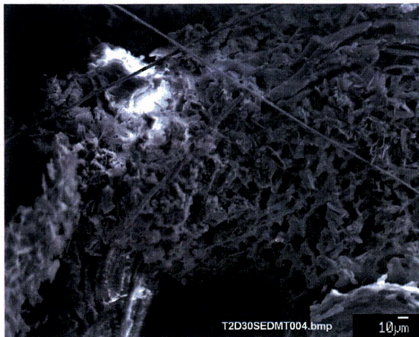
Figure 4-82. Higher-magnification SEM image of a Test #2, Day-30 sediment sample.
