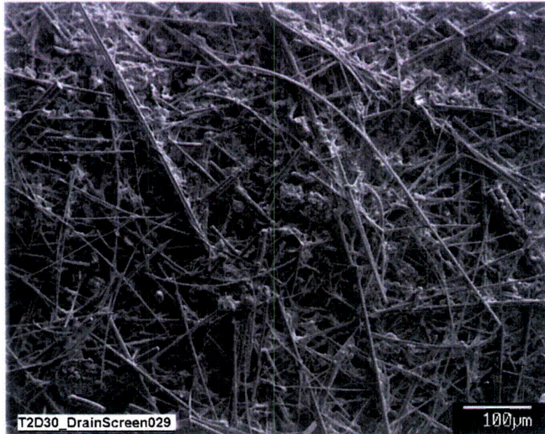
Figure 4-65. SEM image of a Test #2, Day-30 fiberglass sample on the drain collar, next to the drain screen.
