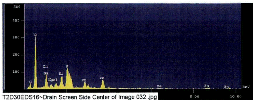
Figure 4-67. EDS counting spectrum for the center of the image shown in Figure 4-66. The deposits are composed of carbon, oxygen, sodium, magnesium, aluminum, silicon, phosphorus, and calcium.
