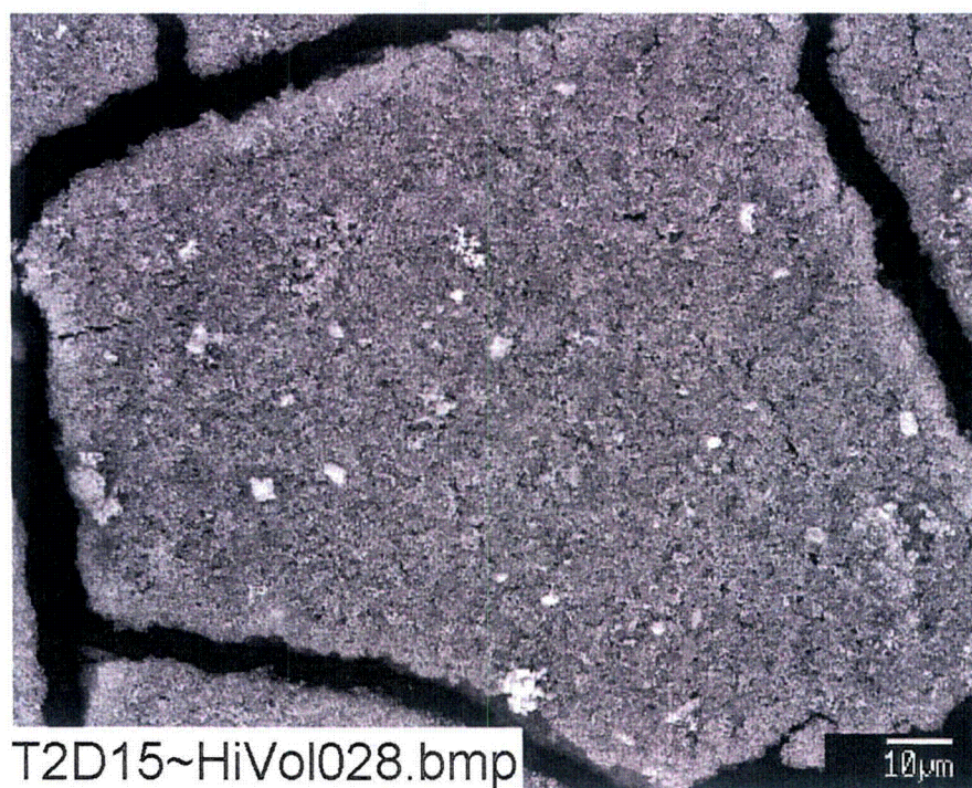
Figure A-2. Backscatter SEM image at 800× magnification for a Test #2, Day-15 sample of particles on a high-volume filter. (T2D15_HiVol028)
