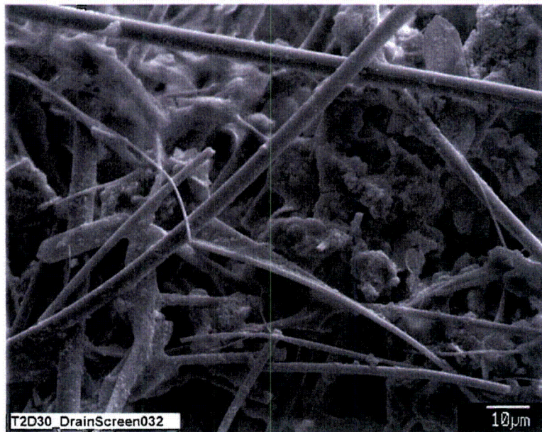
Figure 4-66. Higher-magnification SEM image of a Test #2, Day-30 fiberglass sample on the drain collar, next to the drain screen.
