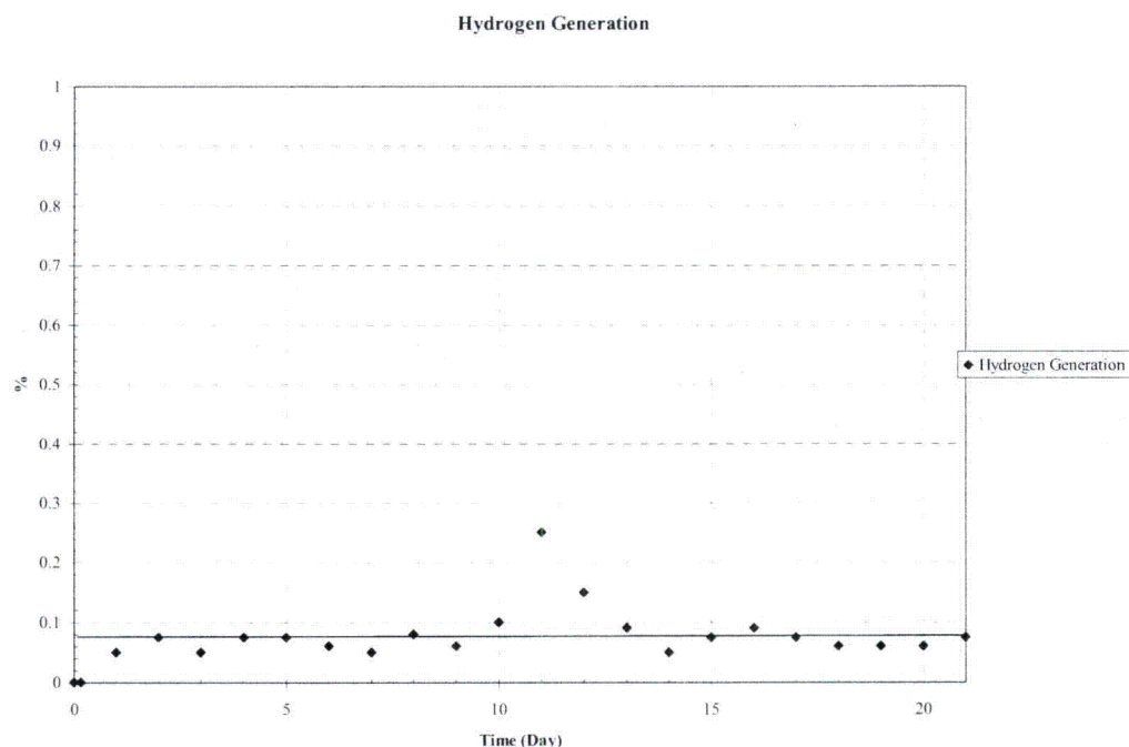
Figure 4-79. Test #2 hydrogen concentration.
