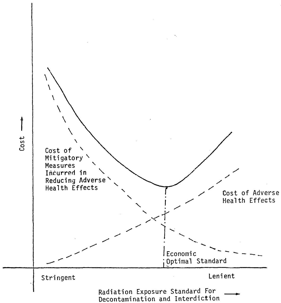
Fig. 10.2. Economic optimal radiation exposure standard for decontamination and interdiction.
