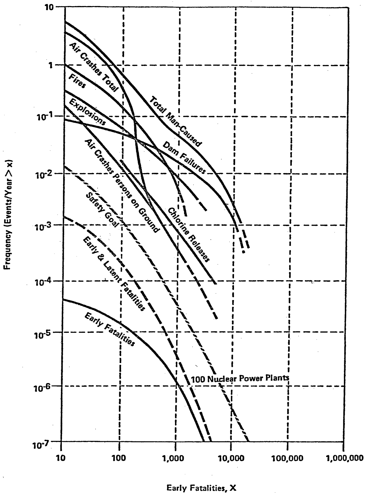
Fig. 9.2 Safety goal proposed by Levine.
