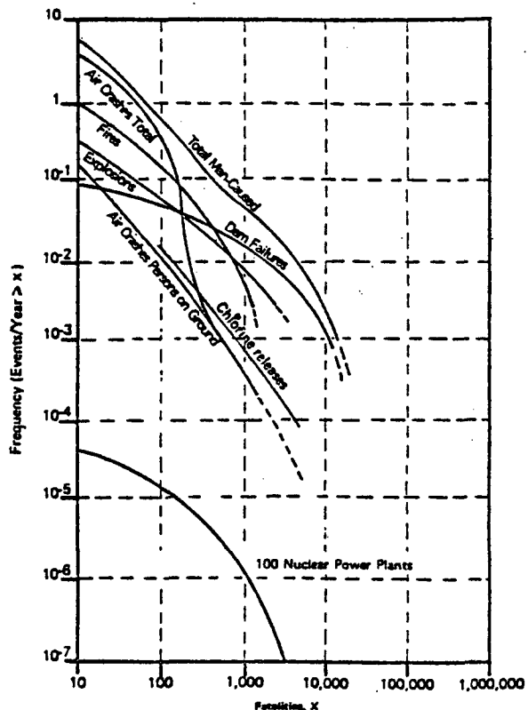
Fig. 2.2 Frequency of Man-Caused Events Involving Fatalities (Ref. 4)
