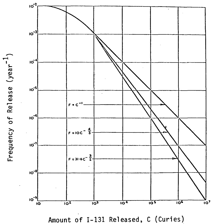
Fig. 7.1 Farmer's release frequency limit lines.
