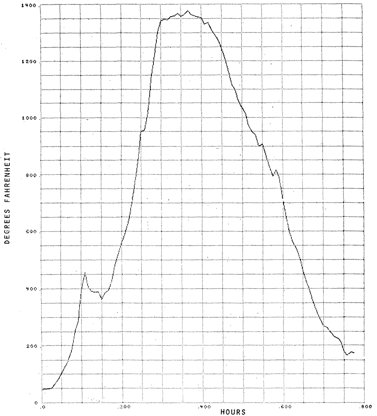
Figure B-4. Burn Test Number 48B, Channel 3, Center Lower Tray
