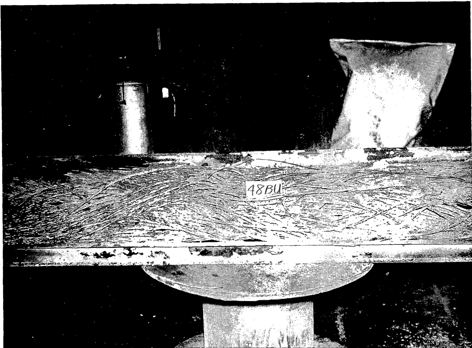
Figure 4. IEEE-383 Qualified Cable in Upper Tray After Corner Effects Test with Smallest Distance to Corner
