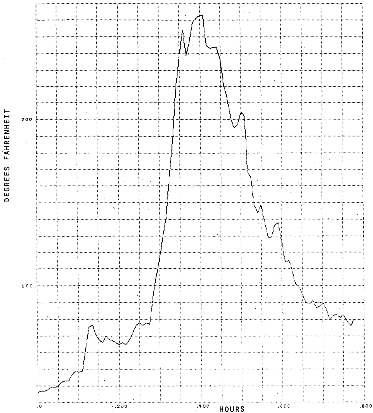
Figure B-14. Burn Test Number 48B, Channel 13, North Tray West
