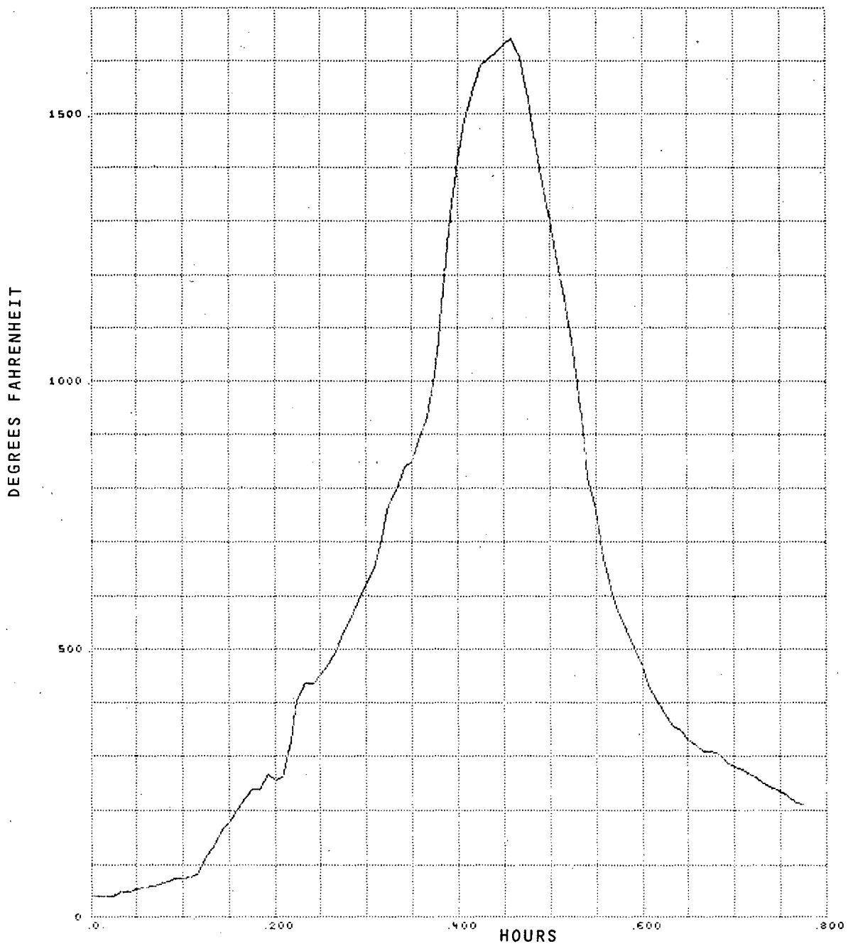
Figure B-9. Burn Test Number 48B, Channel 8, Center Upper Tray
