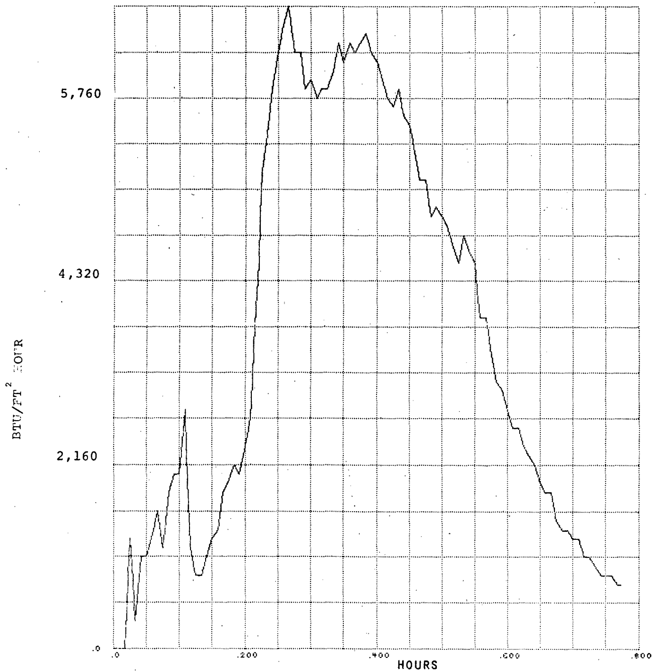
Figure B-15. Burn Test Number 48B, Channel 22, Lower Heat Flux
