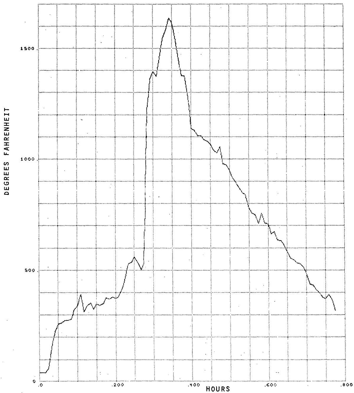
Figure B-12. Burn Test Number 48B, Channel 11, West Ceiling
