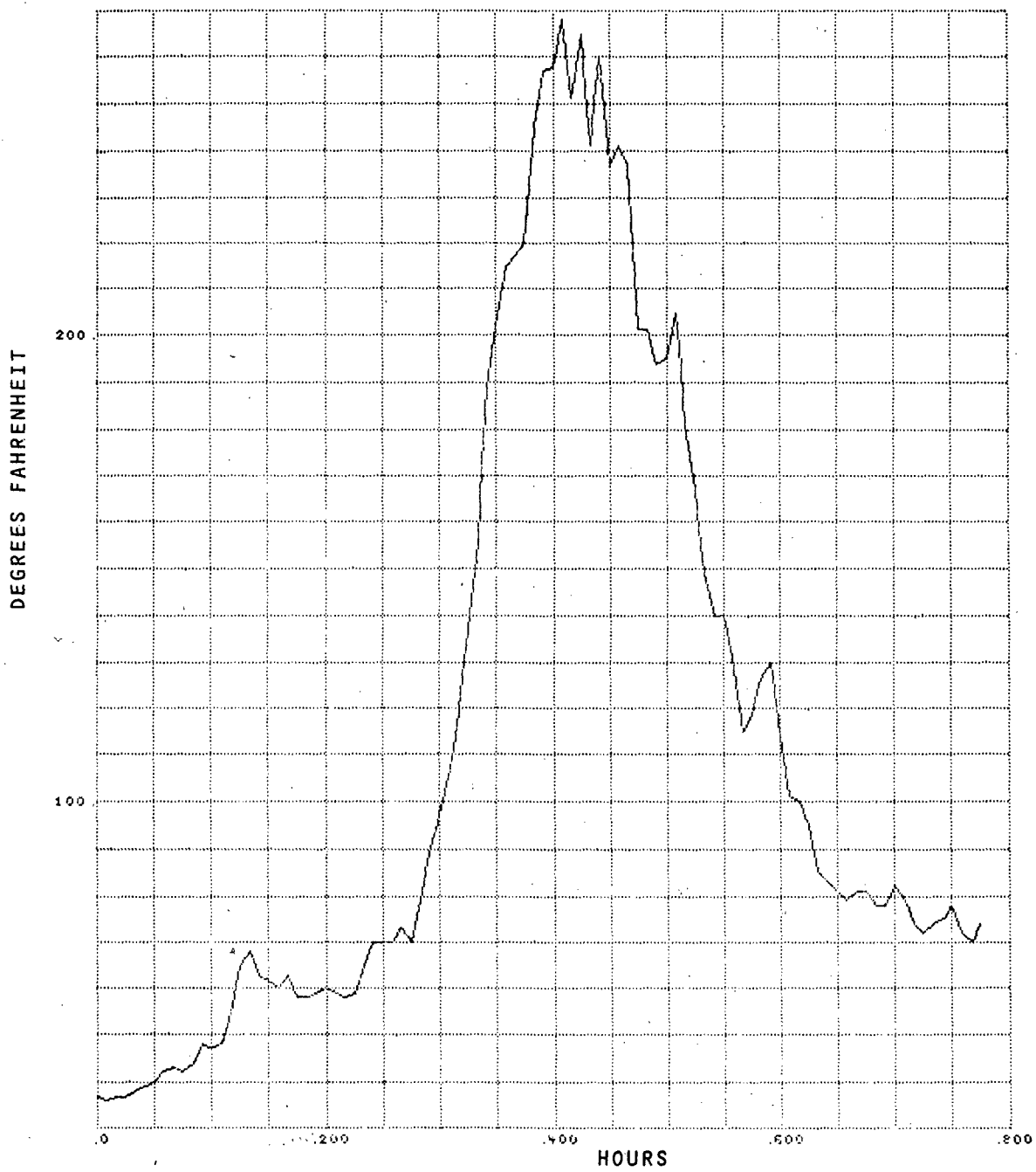
Figure B-13. Burn Test Number 48B, Channel 12, North Tray East
