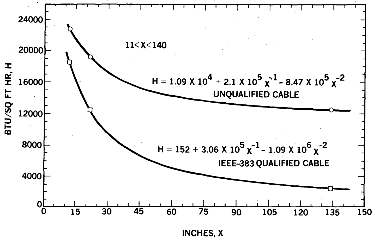
Figure 7. Corner Effects Tests Heat Flux, Top Tray
