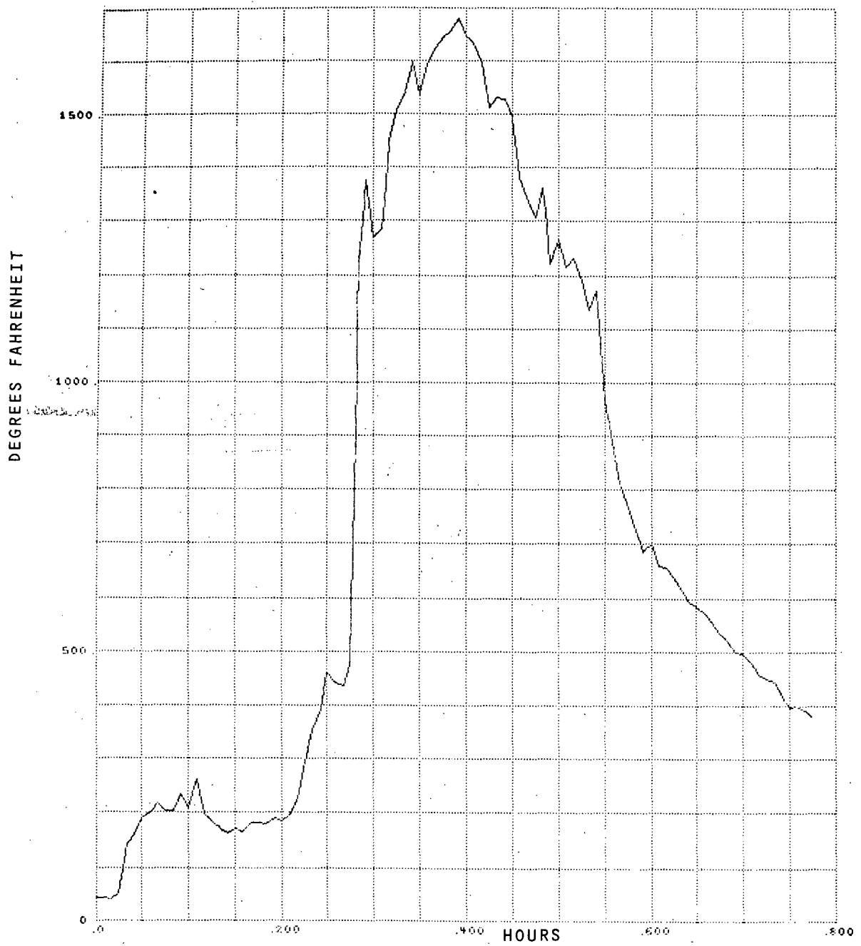
Figure B-11. Burn Test Number 48B, Channel 10, East Ceiling
