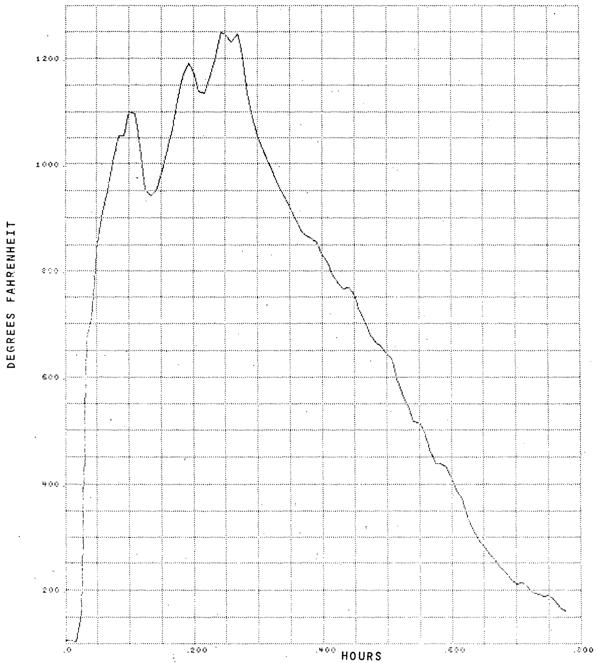
Figure B-3. Burn Test Number 48B, Channel 2, East Lower Tray
