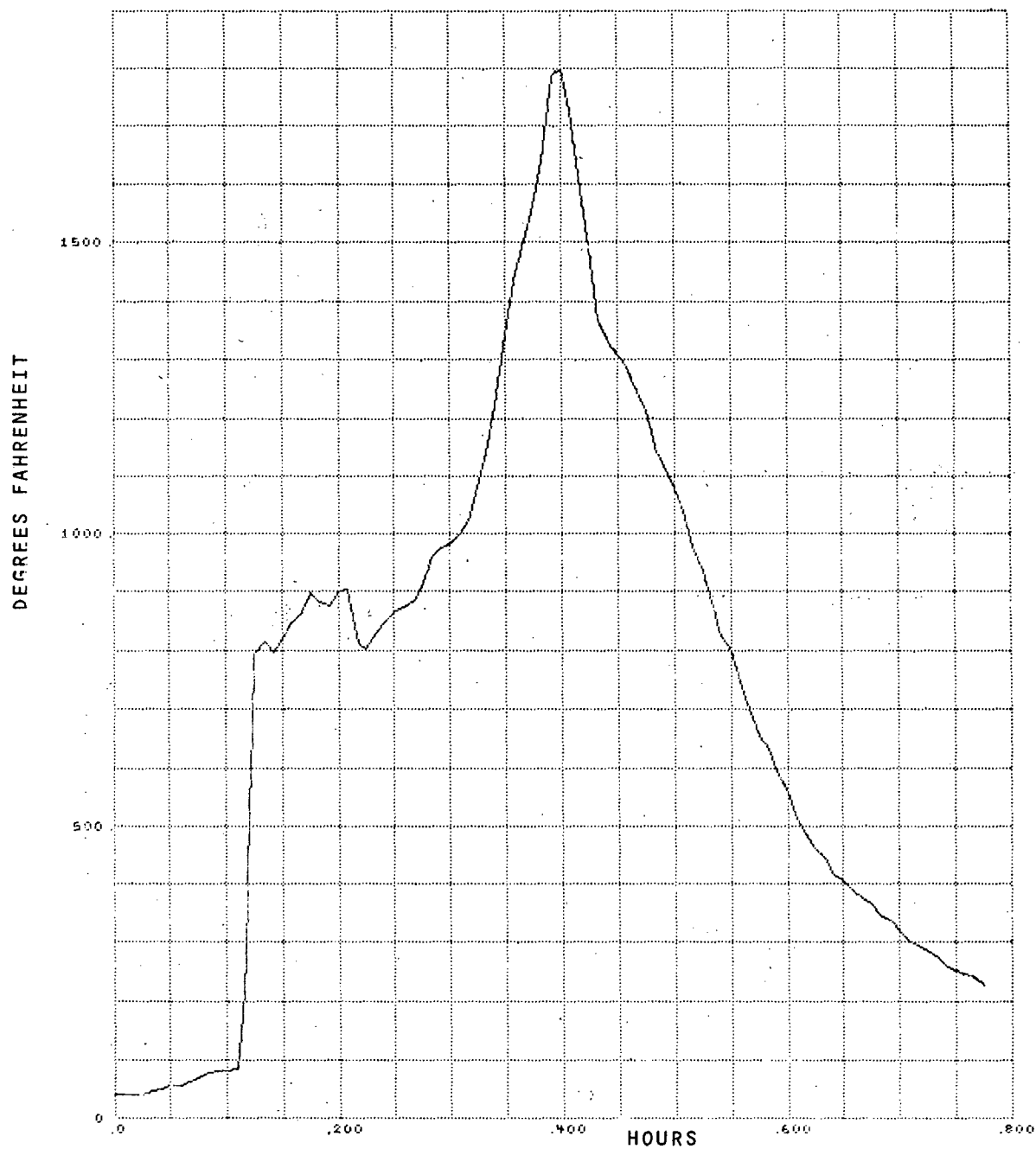
Figure B-10. Burn Test Number 48B, Channel 9, West Upper Tray
