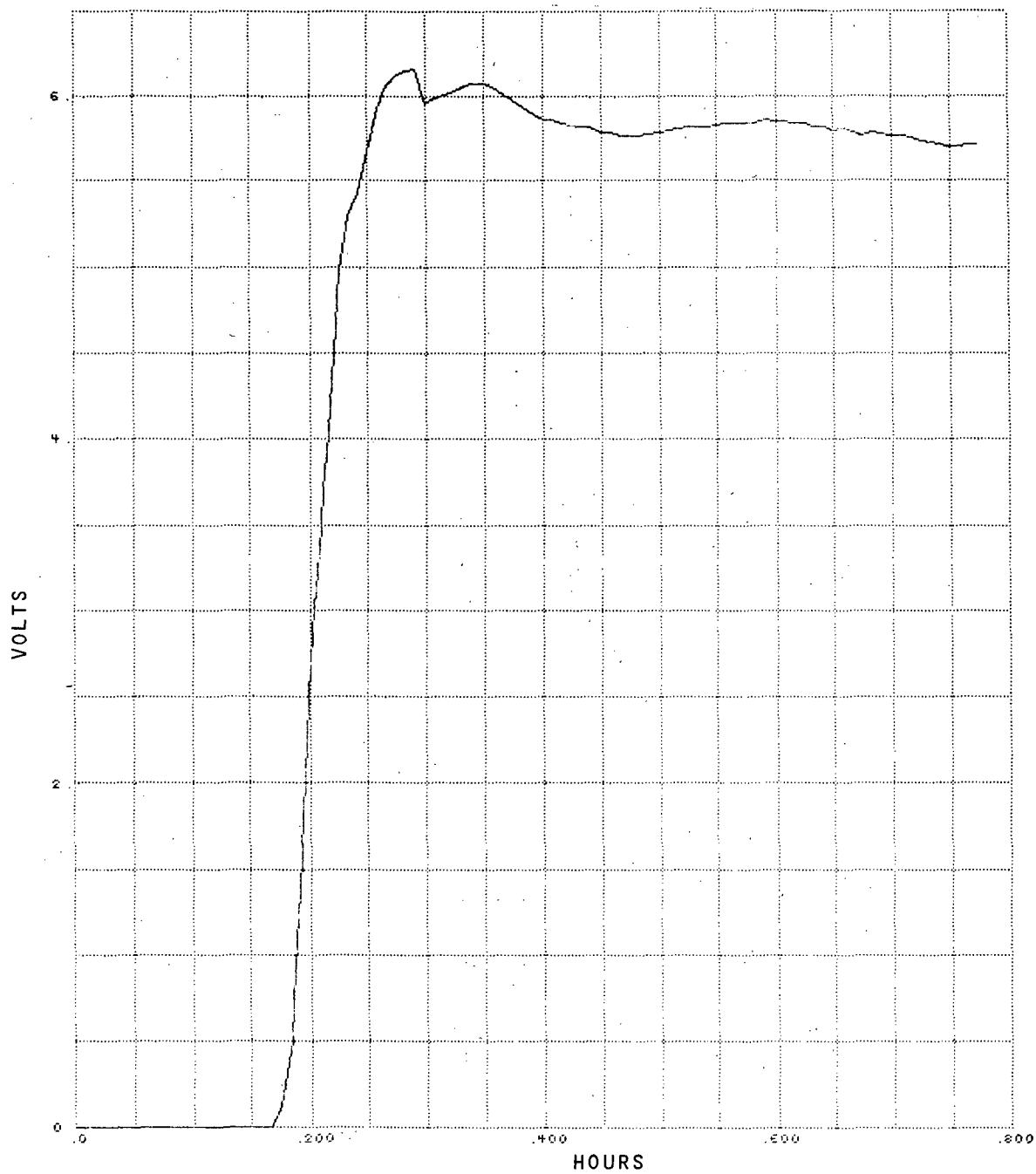
Figure B-18. Burn Test Number 48B, Channel 25, Upper Tray to Ground
