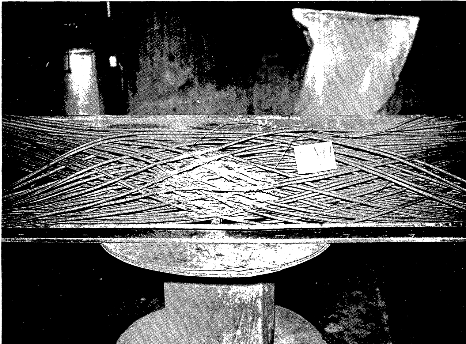
Figure 5. IEEE-383 Qualified Cable in Upper Tray After Corner Effects Test with Largest Distance to Corner
