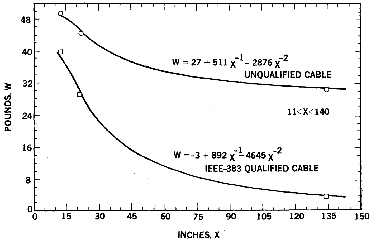
Figure 6. Corner Effects Tests Weight Loss, Top Tray
