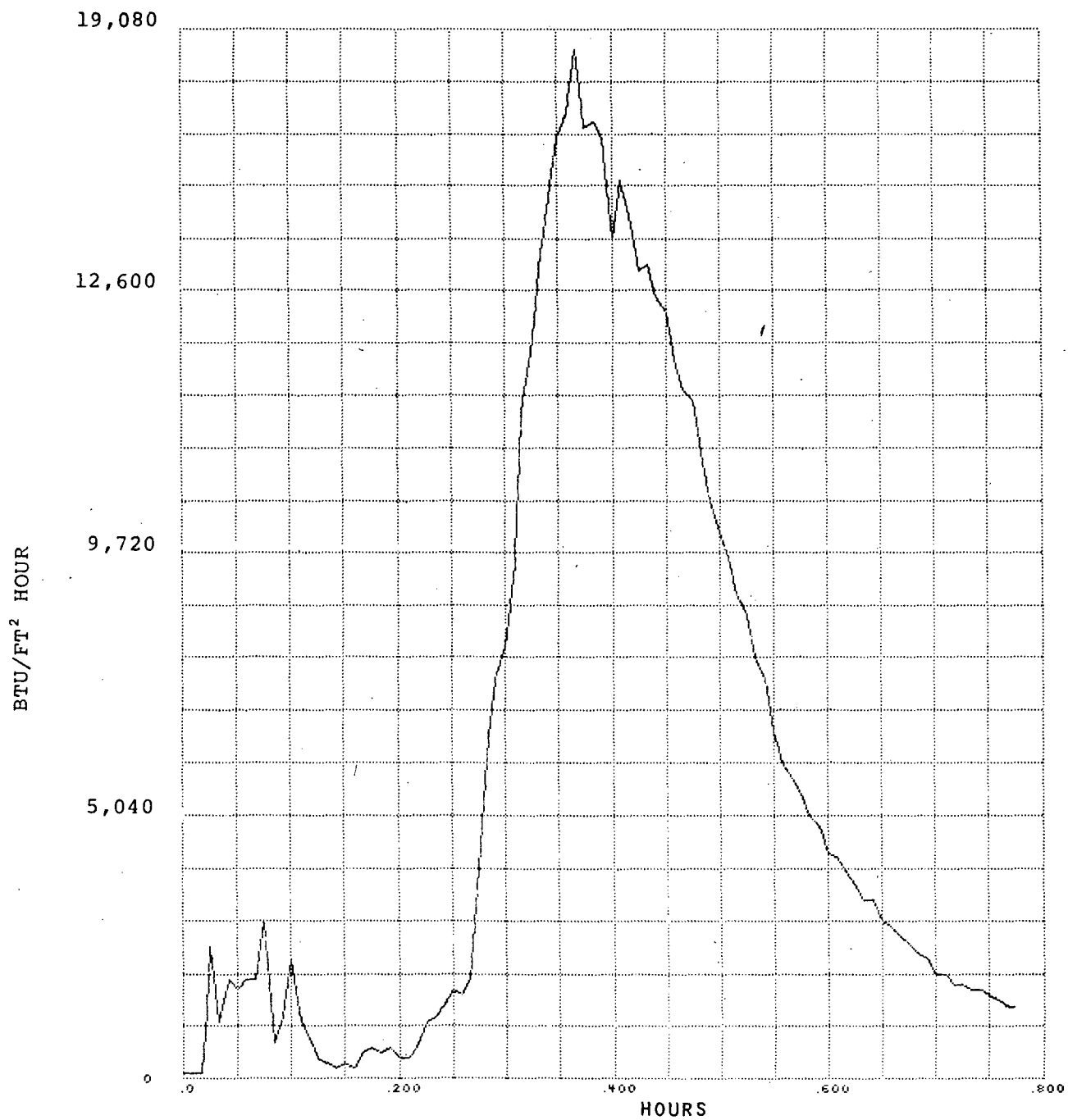
Figure B-16. Burn Test Number 48B, Channel 23, Upper Heat Flux
