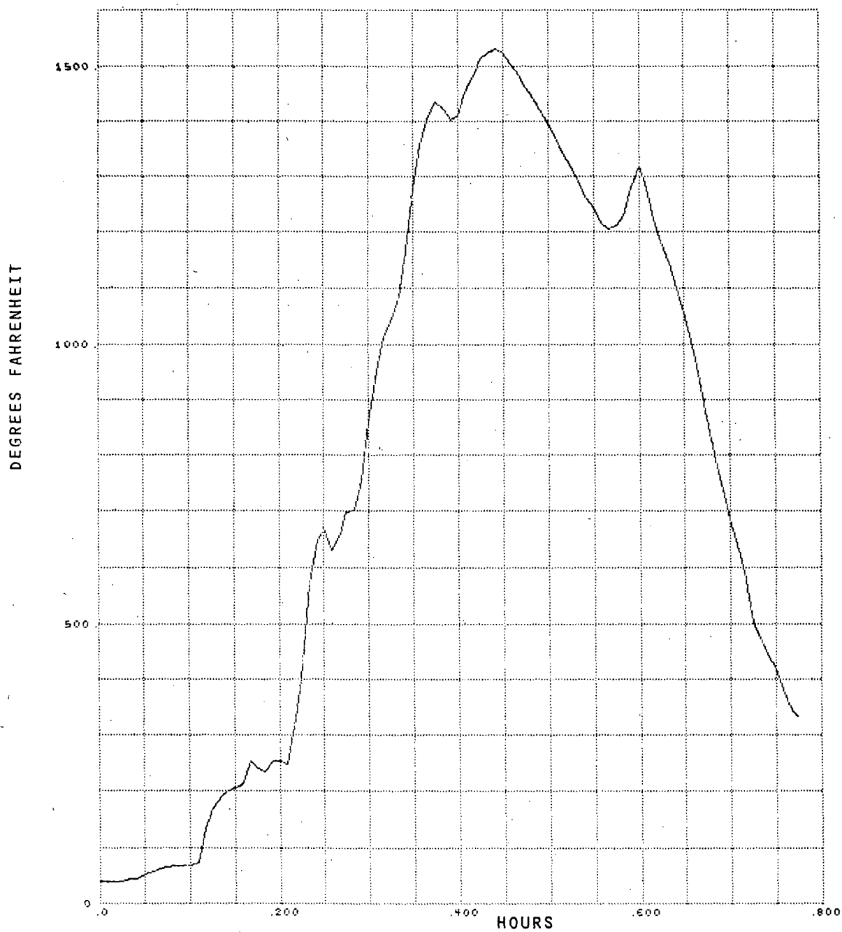
Figure B-8. Burn Test Number 48B, Channel 7, East Upper Tray
