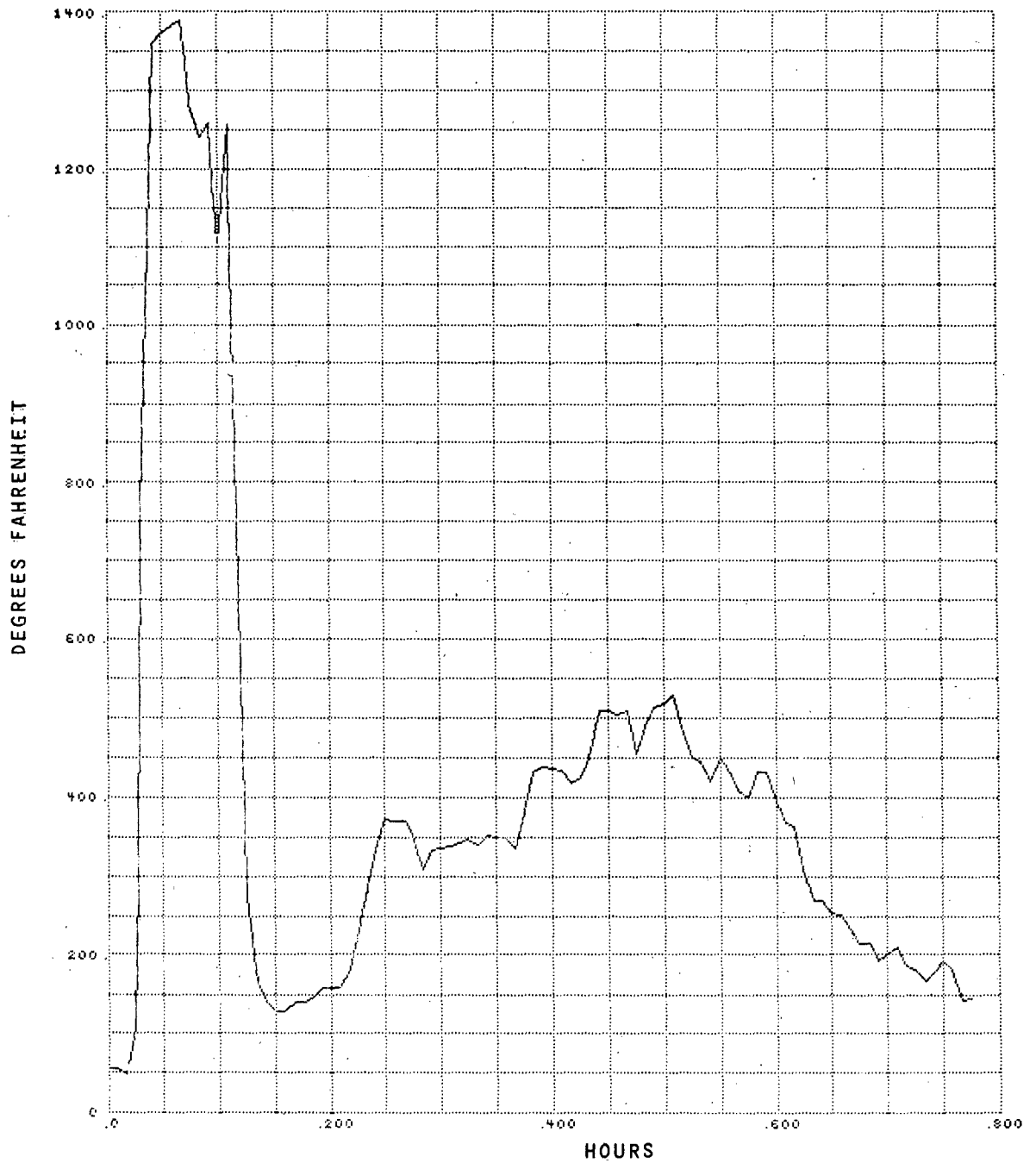
Figure B-6. Burn Test Number 48B, Channel 5, East Lower Barrier
