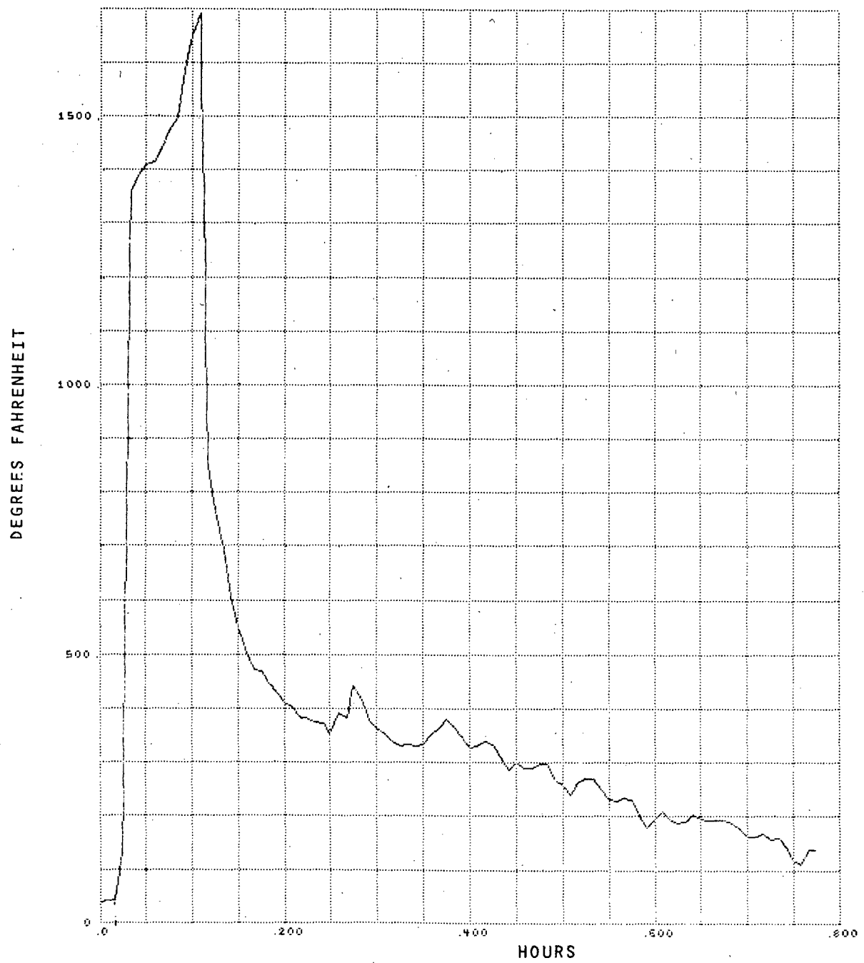
Figure B-5. Burn Test Number 48B, Channel 4, West Lower Tray
