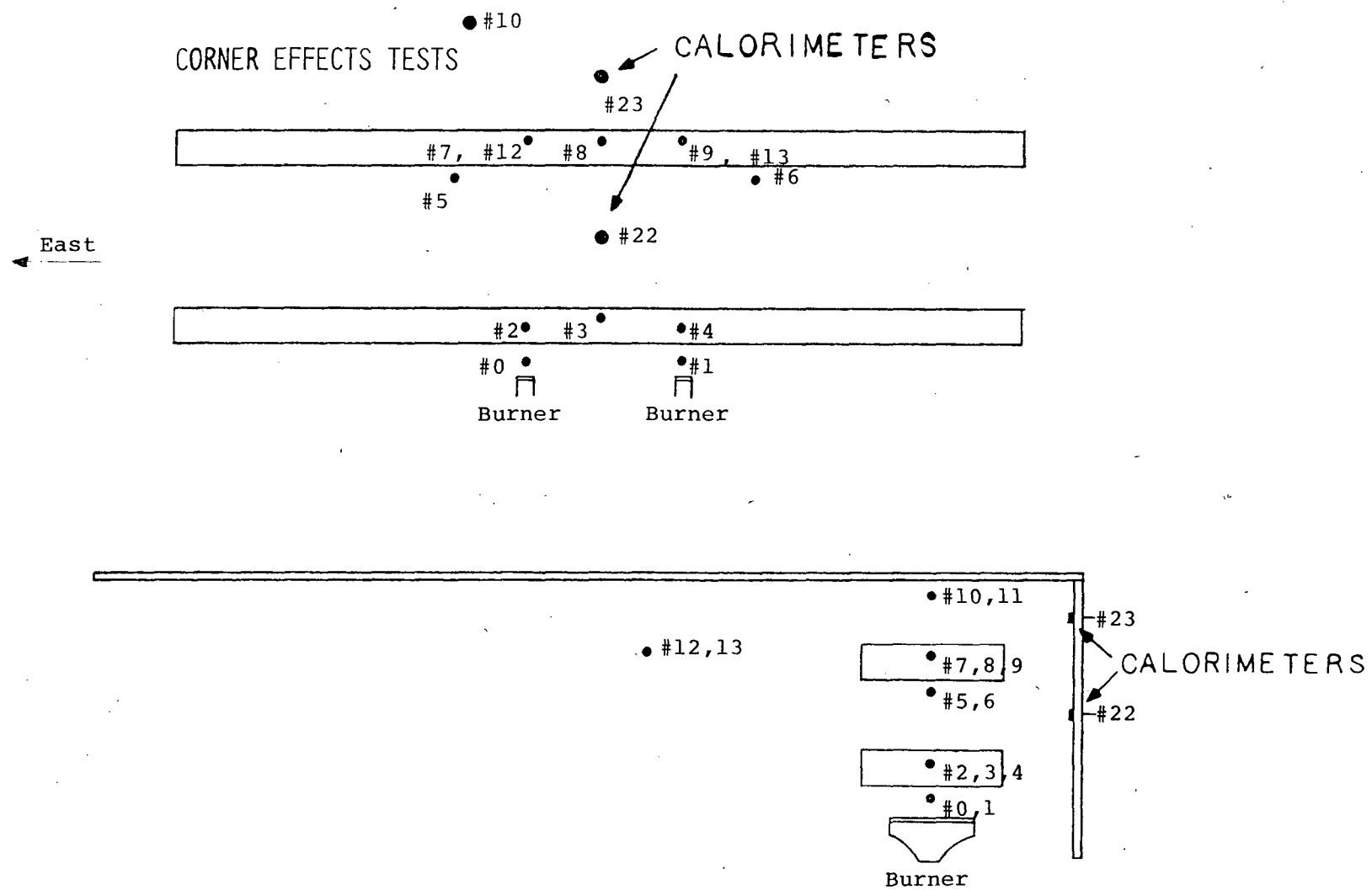
Figure 3. Thermocouple and Calorimeter Placement (Data channel numbers shown, see Appendix B)
