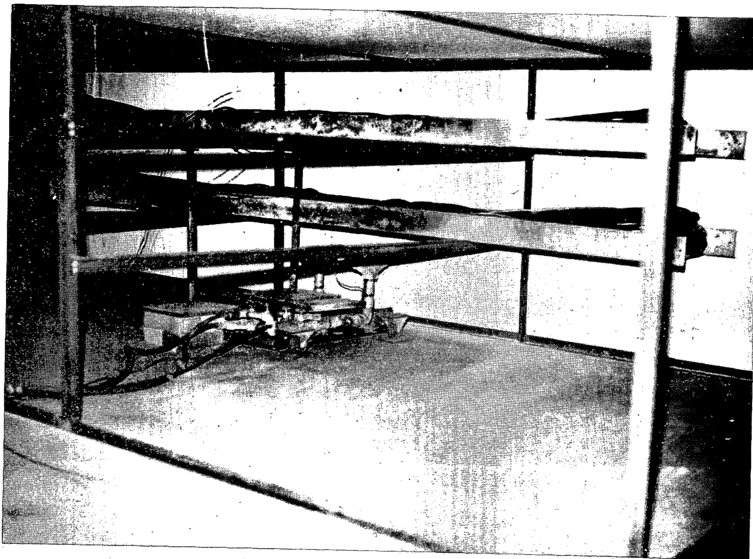
Figure 2 Cable Tray and Burner Arrangement
