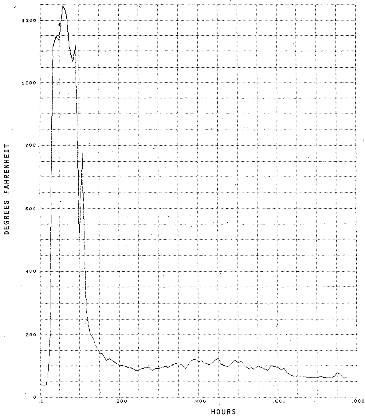
Figure B-1. Burn Test Number 48B, Channel 0, East Burner
