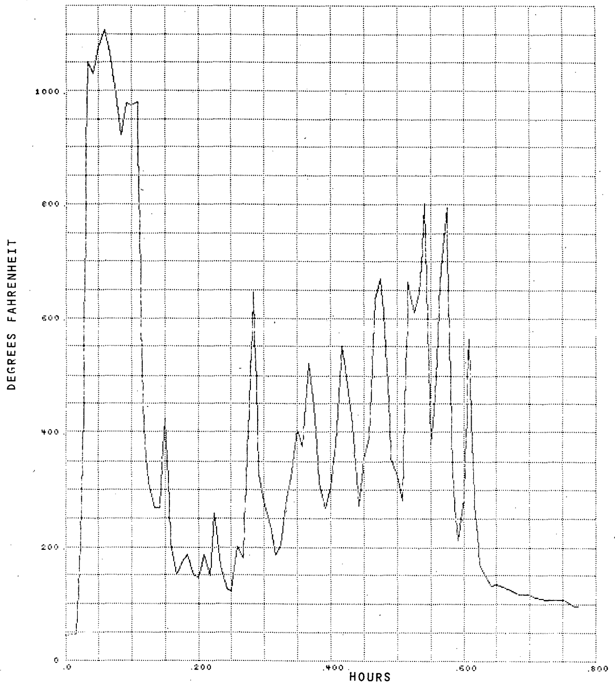
Figure B-2. Burn Test Number 48B, Channel 1, West Burner
