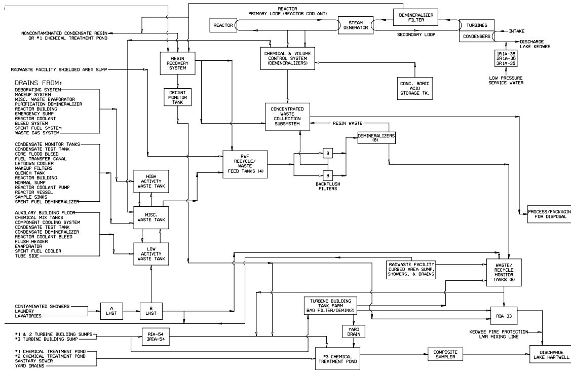
Figure 1.0-1 Oconee Nuclear Station Liquid Radwaste System
