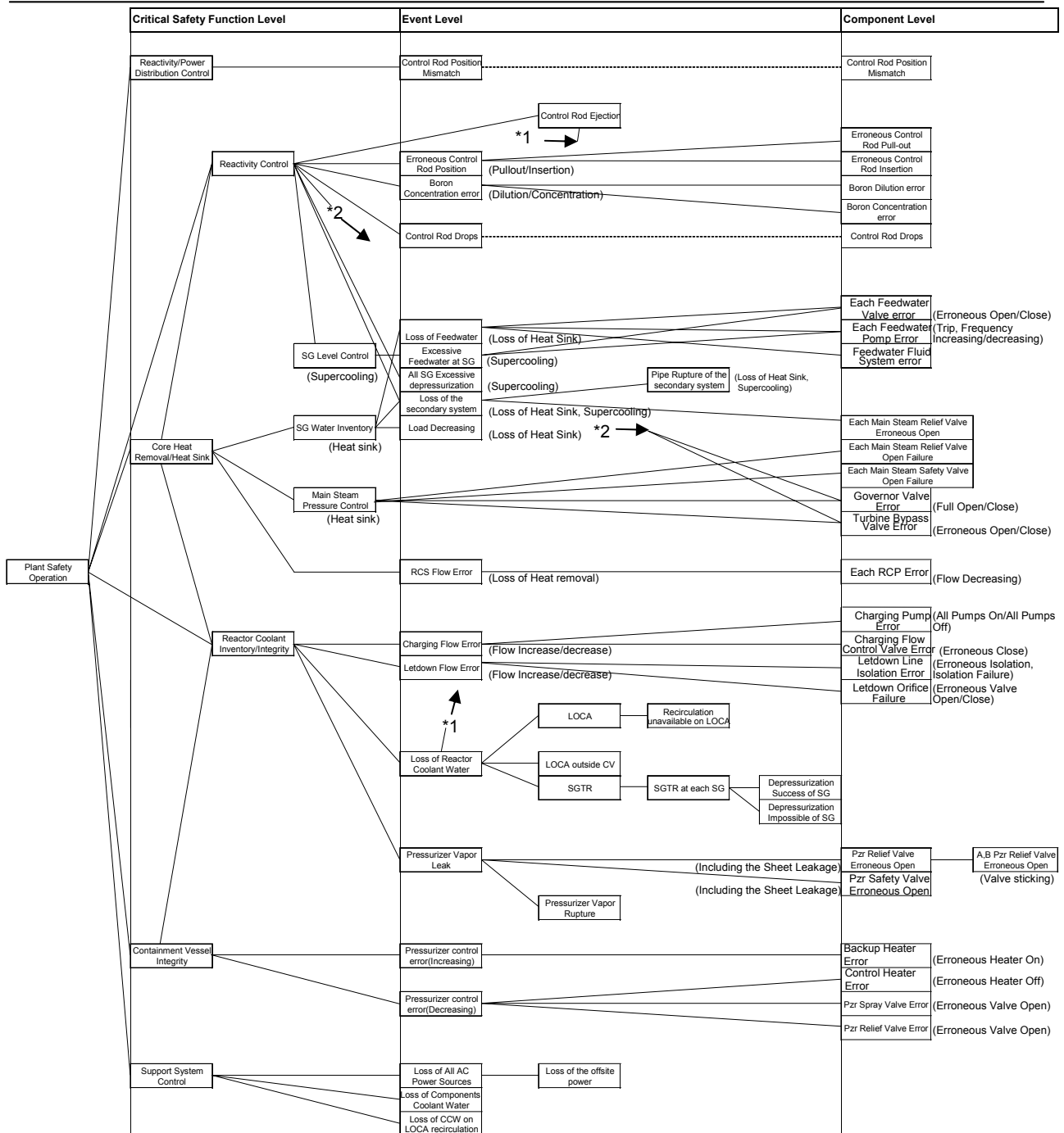
Figure 5.3-1 Hierarchical Structure of Safety Plant Functions
