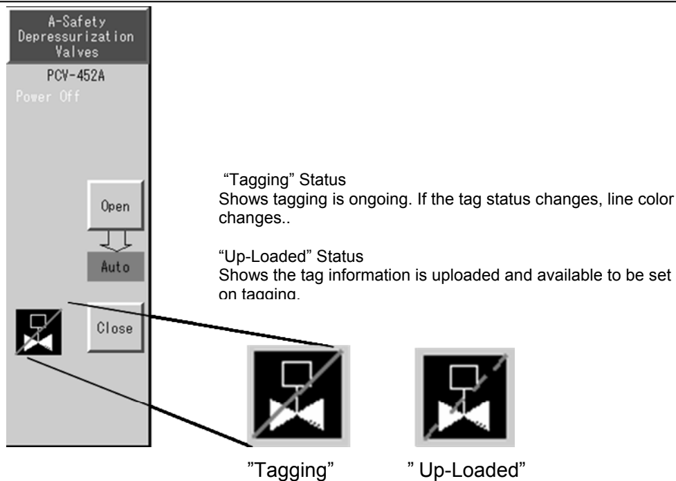
Figure 4.5-6 Example of Tag Status Display
