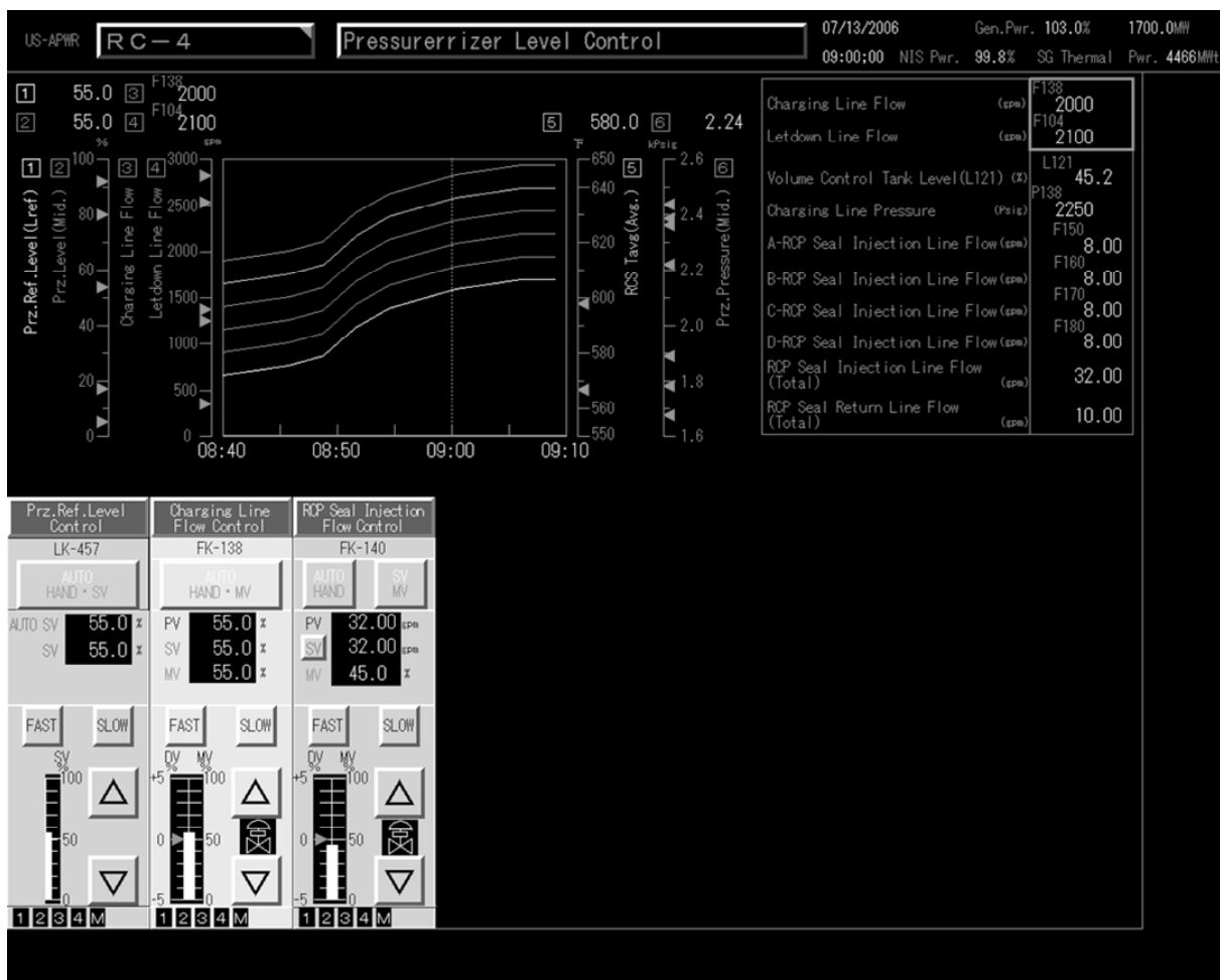
Figure 4.5-2 Example of Controller Screen
