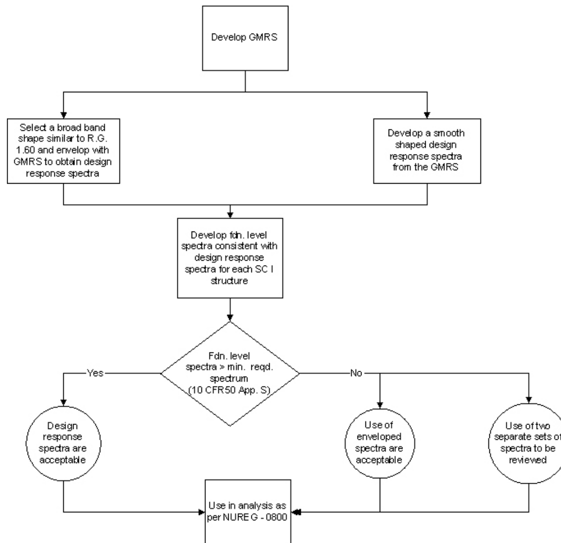
Figure 3 - Process When a Certified Design is Not Used
