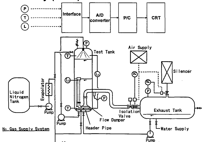
Outline of the Test Facility
