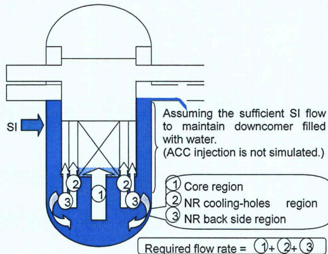
Required ECCS injection flow rate
