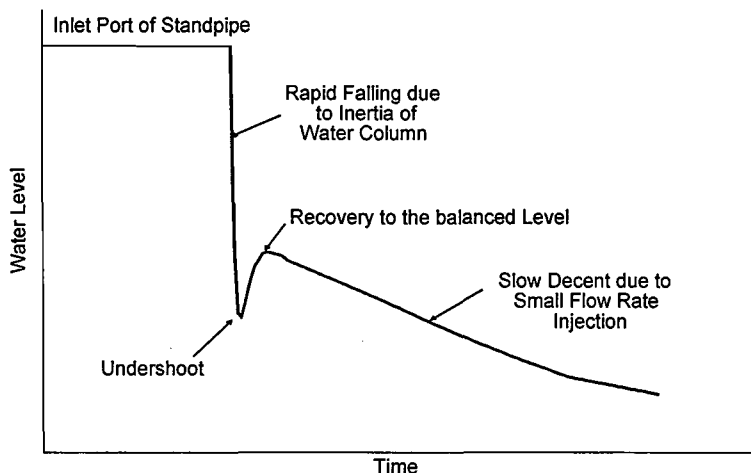
Water Level in Standpipe (schematic chart)
