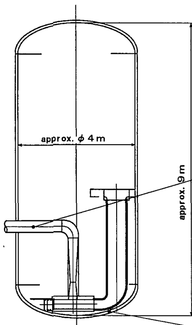
Outline drawing of ACC
