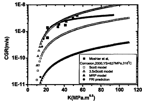
Figure 10 PWR SCC CGR data for cold worked alloy 600 (YS of 827MPa) as a function of K at 316°C [9] and predicted values of CGR by several models.
