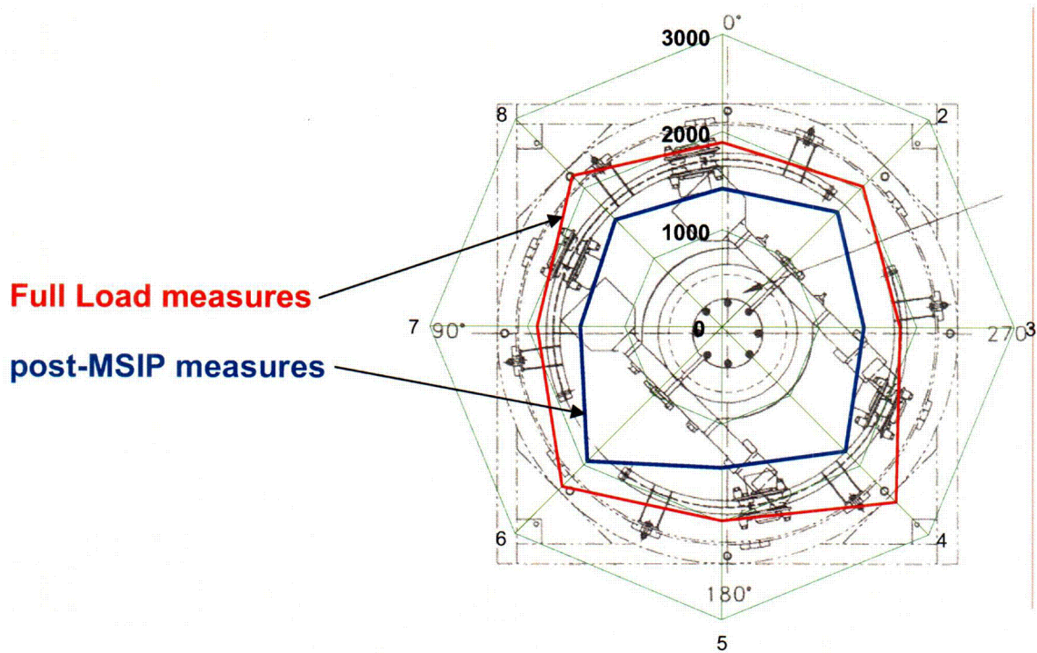
Figure 7 - Polar Plot of Hoop Strains (Micro-Inches per Inch)
