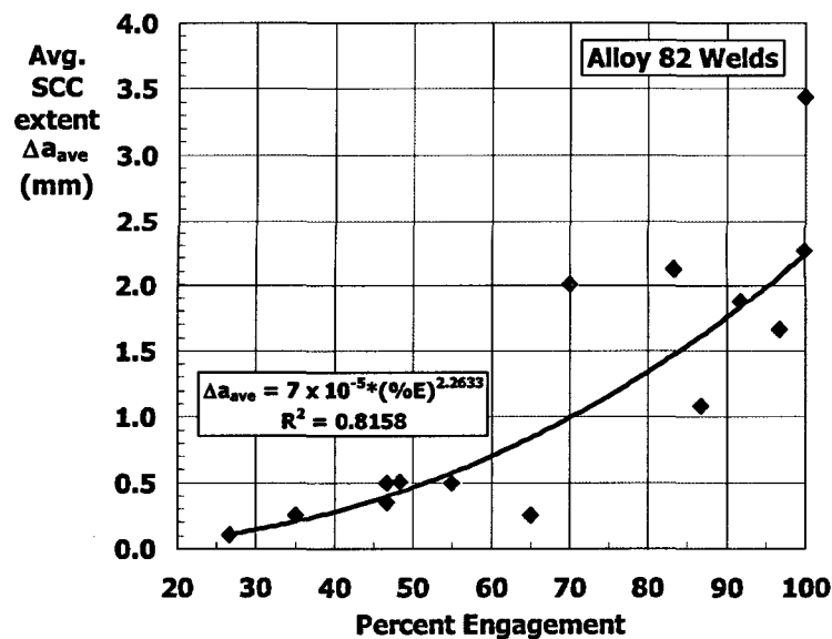
Figure A3. Correlation of average SCC extent (i.e., \Delta a_{\text{ave}} ) with percent engagement (%E). This correlation shows that, as expected, cracks with a larger depth of SCC also tend to be closer to full engagement across the precrack. This correlation may also be useful in certain cases for analyzing historical data for which %E is not available.
