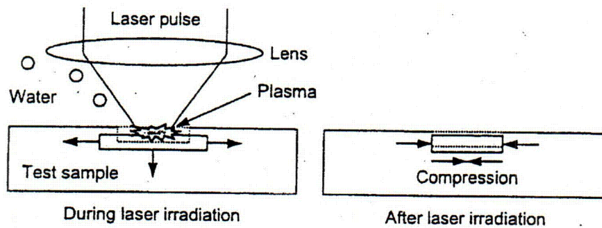
Figure 4. Typical Laser Peening Process.
