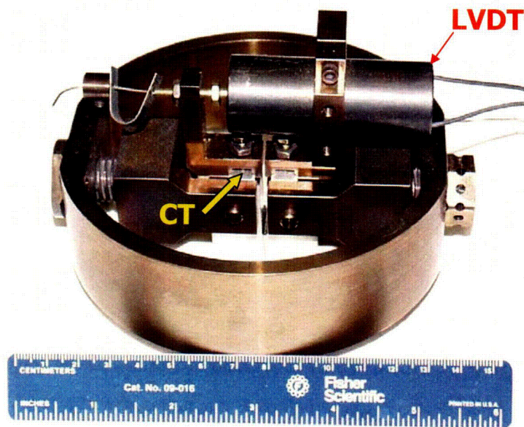
Figure 4. Compliant self-loaded compact tension (CSLCT) specimen hardware (a) and assembly (b). The unloaded length of the ring ( L_U ) is shown in (a).
