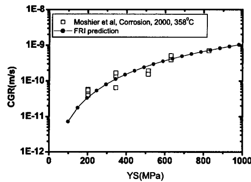
Figure 13. Experimental CGR [9] and CGR values predicted by the FRI generalized CGR formulation for alloy 600 in simulated PWR primary water
