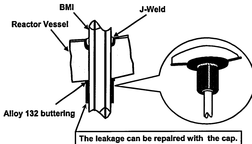
Fig.4 Concept of cap repair method for BMI nozzles
