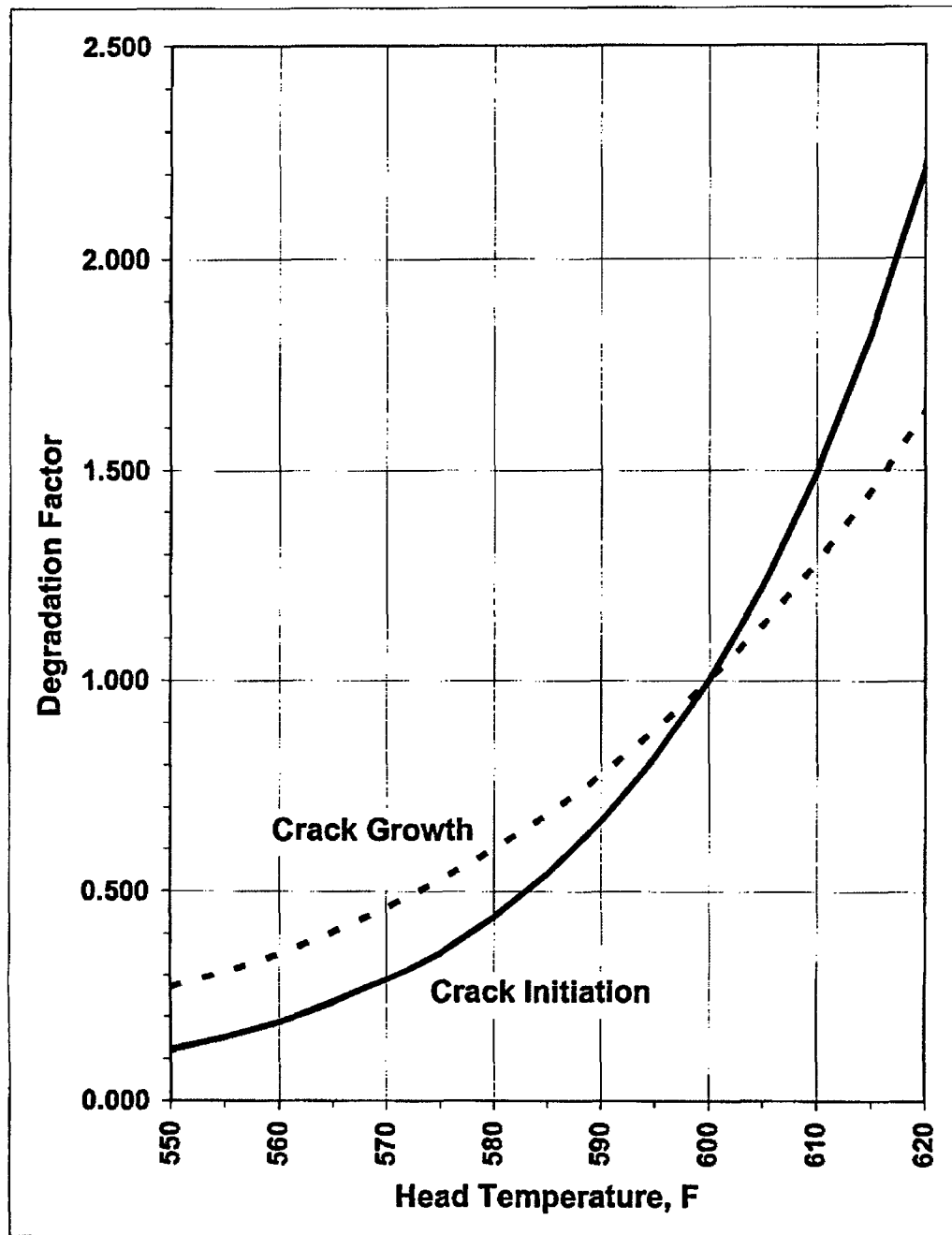
Figure 4: Degradation Factor as a Function of Temperature
