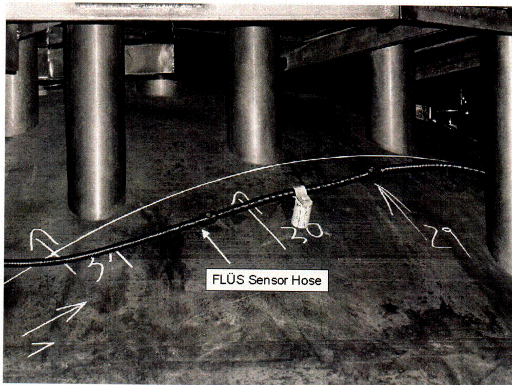
Figure 5 FLÜSS Sensor Hose installed on RPV head of KWO
