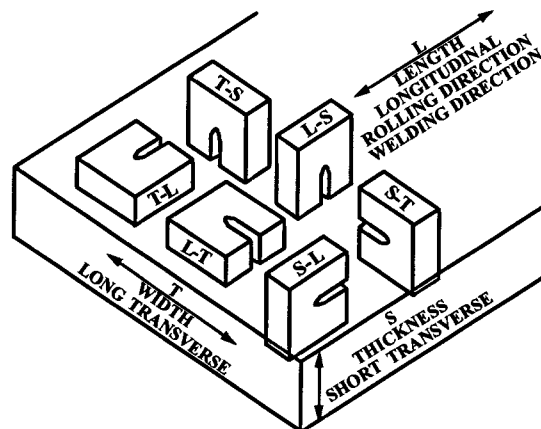
Figure 6 Terminology used for orientation of cracks in the test specimens with respect to the weld
