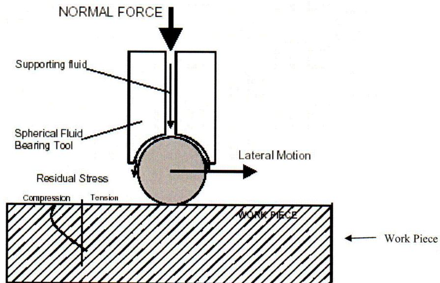
Figure 7. Low Plasticity Burnishing Schematic.
