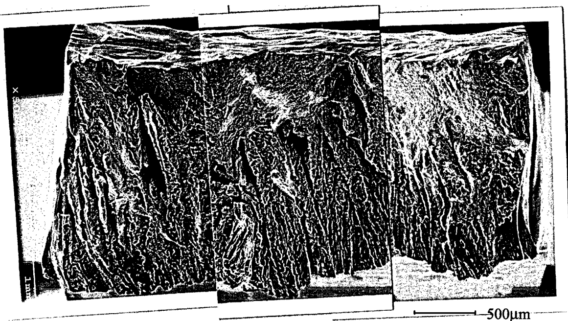
FIGURE 5 - SEM microphotograph of the fractured surface of Alloy 82 weld metal of the SSRT test specimen (Temp.: 360 °C)
