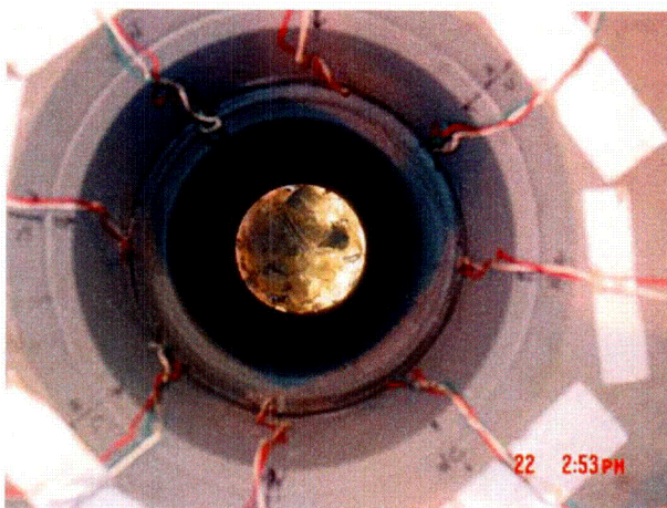
Figure 4(a) Illustration of the Instrumented Strain Gauges Installed on the ID Surface Near the Weld Location of the Mockup Pressurizer Nozzle
