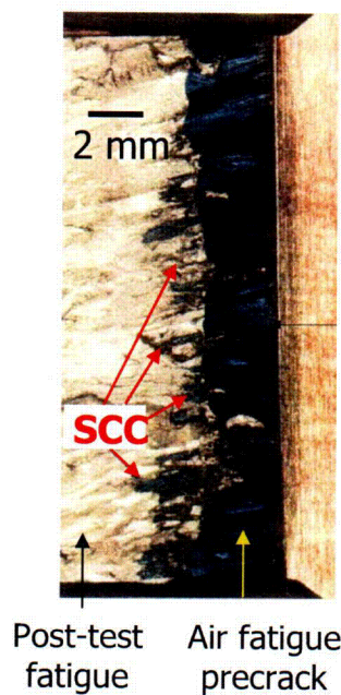
Figure 3. A specimen showing the air fatigue precrack, SCC, and post-test fatigue regions.
