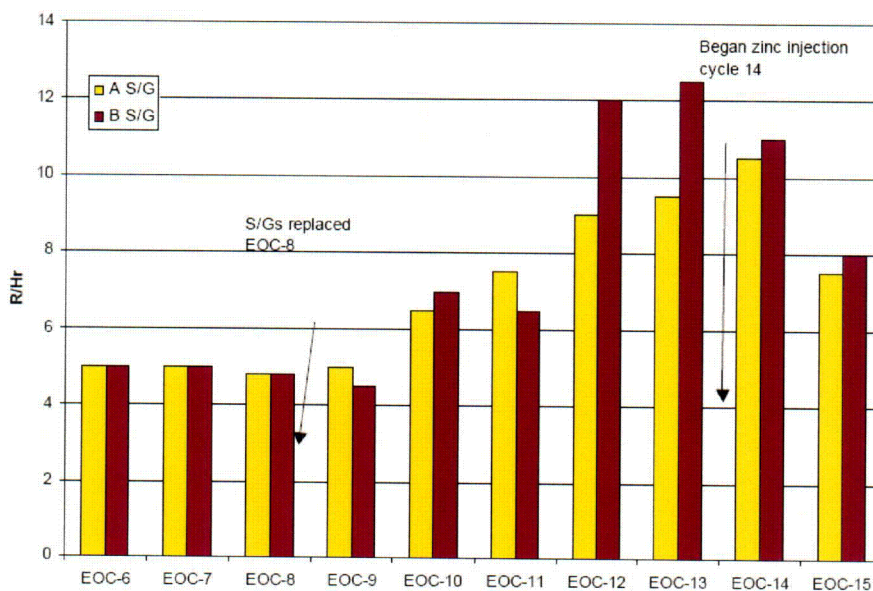
Figure 2 Post zinc dose rate trends for Palisades channel head (levels up to 10 ppb)
