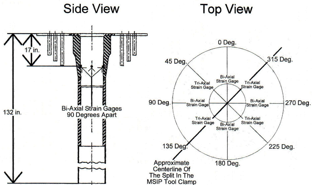
Figure 3 – Schematic Illustration of the Positions of Bi-axial and Tri-axial (Rosette) Strain Gauges near the Weld Region at the ID Surface
