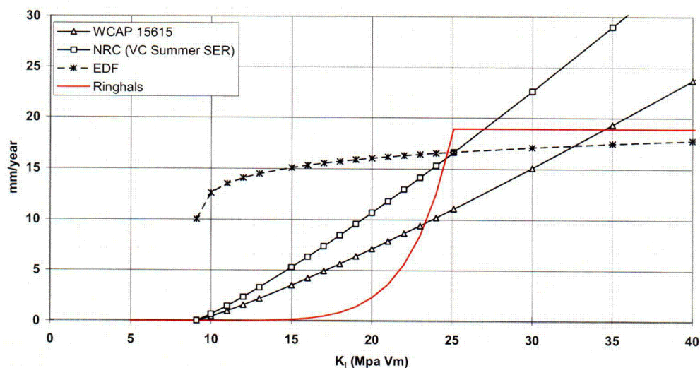
Upper bound crack growth rates - Inconel 182 at 323°C
