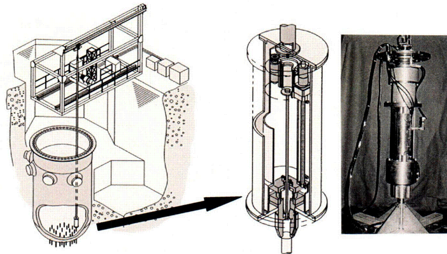
Fig.2 Concept of WJP for BMI nozzle and the system
