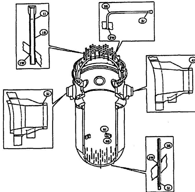
Fig.1 Alloy 600 components of the RV pressure boundary
