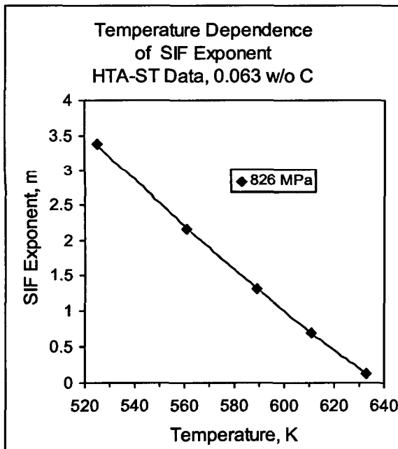
Figure 4. Temperature Dependence of the SIF Exponent for HTA-ST CGR Data.
