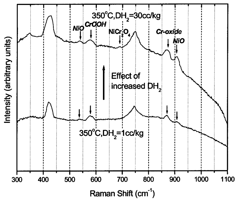
FIGURE 7. In-situ Raman spectra obtained for Alloy 600 at 350°C in PWR water as the \text{DH}_2 in water was increased from 1 to 30 cc/kg.
