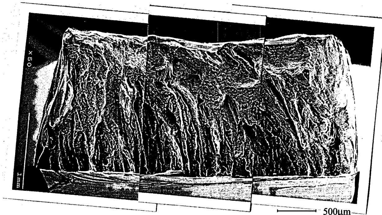
FIGURE 6 - SEM microphotograph of the fractured surface of Alloy 132 weld metal of the SSRT test specimen (Temp.: 360 °C)
