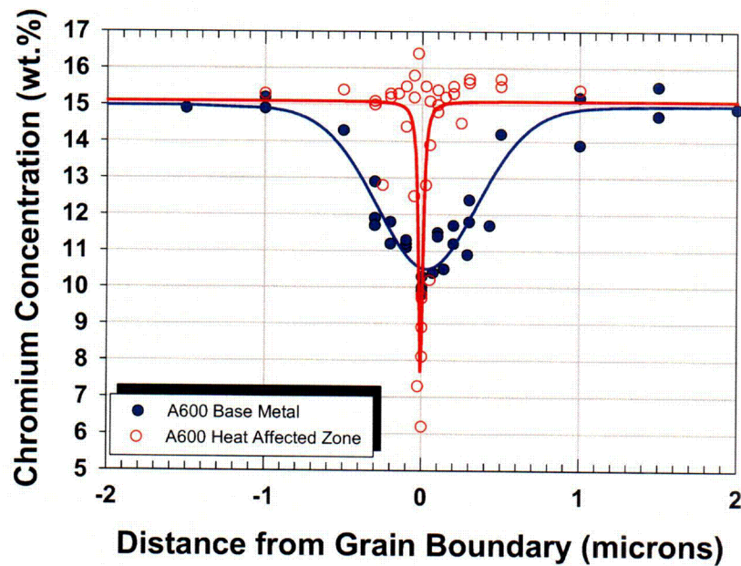
Figure 9. Comparison of chromium depletion near unaffected base metal (solid blue points) and the heat affected zone (open red points). The HAZ shows a much sharper Cr depleted zone, consistent with the fewer, finer Cr_{23}C_6 -type carbides relative to the extensive Cr_7C_3 carbide precipitation in the base metal.
