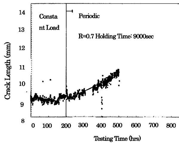
Figure 12 CGR on line monitoring results ( K=35\text{MPa}\sqrt{\text{m}} , TP. No. MG7T-2)
