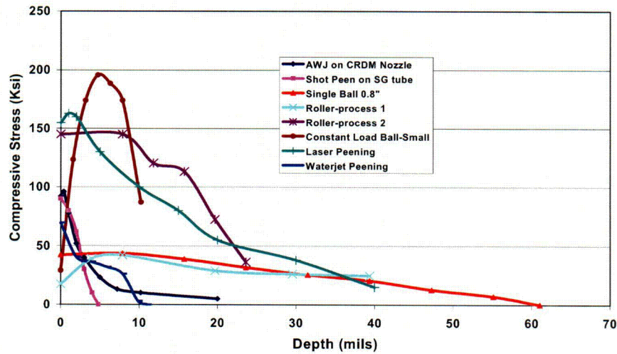
Figure 6. Typical Compressive Stress Distribution Comparison of Several Remediation Techniques.
