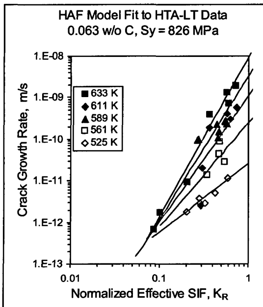
Figure 6. HAF Model Fit to HTA-LT CGR Data.
