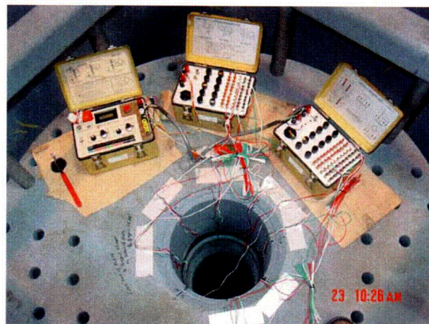
Figure 4(b) Illustration of the Installed Strain Gauges and the Strain Measuring Instrumentation at the Girard Site, Prior to MSIP Load Test
