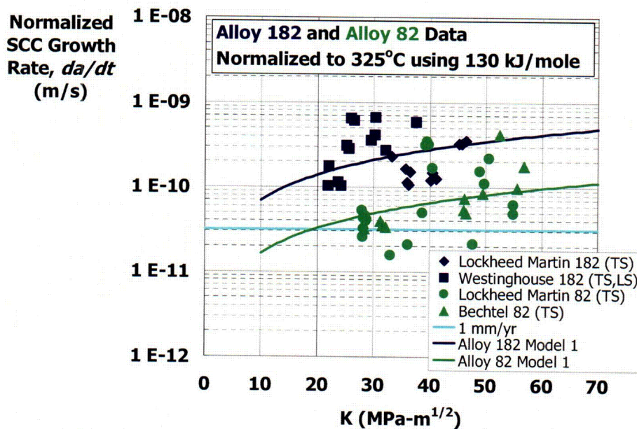
Figure 12. Fit of the SCCGR data to Model 1. This model does not employ a threshold, and the K_1 dependency is not fixed.
