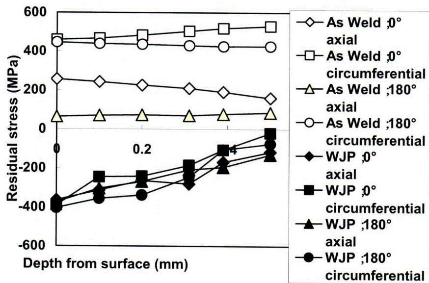
Fig.3 Results of residual stress measurement before and after WJP
