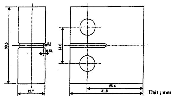
Figure 5 Configuration of 1/2 CT specimen
