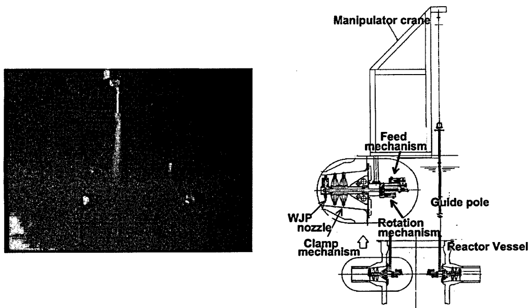
Fig.5 Concept of WJP for outlet/inlet nozzle safe ends
