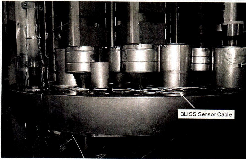
Figure 4 BLISS Sensor Cable installed on RPV Head
