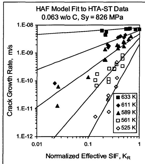
Figure 3. HAF Model Fit to HTA-ST CGR Data. Log-log plot emphasizes temperature dependence of the SIF exponent.
