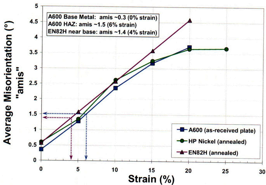
Figure 13. Calibration curves relating the applied tensile strain at room temperature to the average intra-grain misorientation (amis) parameter. The HAZ samples exhibited ~6% plastic strain.
