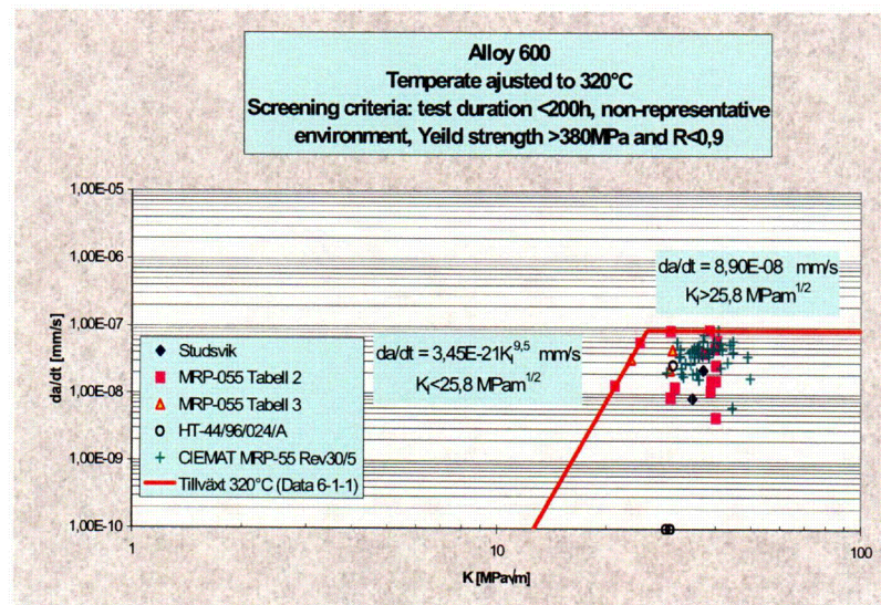
Figure 2, The final results after screening the Alloy 600 database with regards to the criteria presented in [2].
