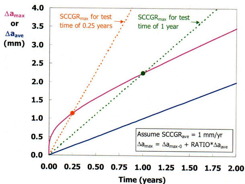
Figure 8. Schematic illustration of the effect of test time on the apparent maximum SCCGR. The \Delta a_{\max} curve (magenta) was obtained by integrating the RATIO data in Figure 7, and by assuming an \text{SCCGR}_{\text{ave}} of 1 mm/yr.
