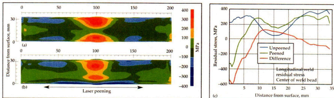
Figure 5. Residual Stress in a 33-mm Thick Alloy 22 Welded Plate: (a) Map of Residual Stress in Unpeened Weld; (b) Map of Residual Stress in Laser Peened Weld; (c) Line Plot of Residual Stress Versus Depth at the Center of the Weld Bead,
