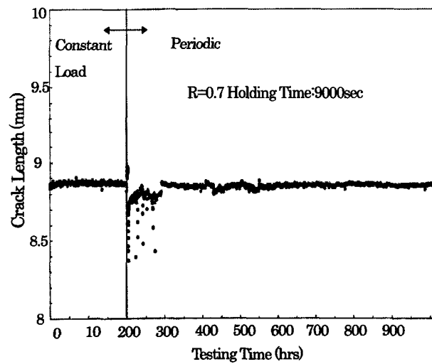
Figure 10 CGR on-line monitoring results ( K=20\text{MPa}\sqrt{\text{m}} , TP. No. MG7-1)
