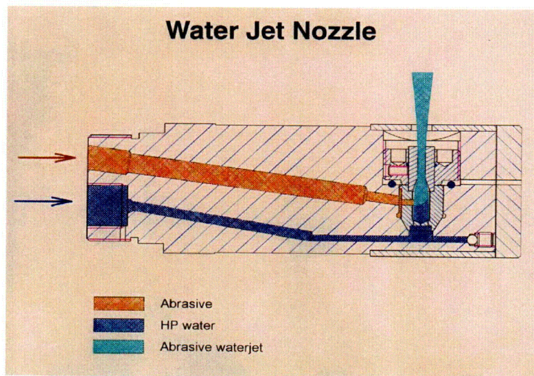
Figure 1. Typical Configuration of an Abrasive Waterjet Conditioning Nozzle.
