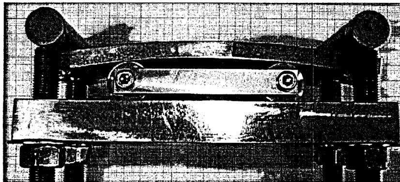
Figure 1 - Photographs of Alloy 52M (Upper 1 thru 4), Alloy 600 (600-1 thru-4), and Alloy 182- 4 (lower photo) bent beam test specimens. [Specimens with suffixes -1 and -2 were strained 0.35%; those with suffixes -3 and -4 wee strained 1.0%]
