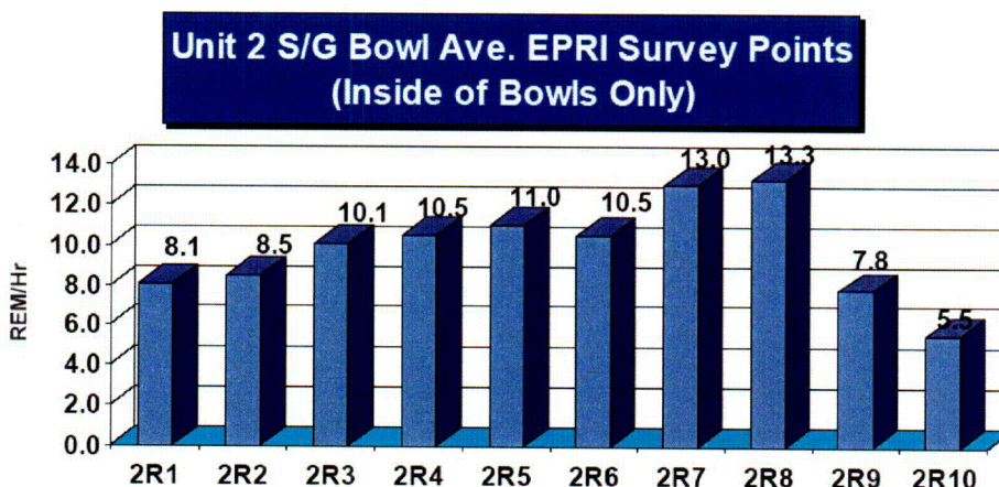
Figure 1 Post zinc dose rate trends for Diablo Canyon Unit 2 (first additions during cycle 9; range 15 to 30 ppb)
