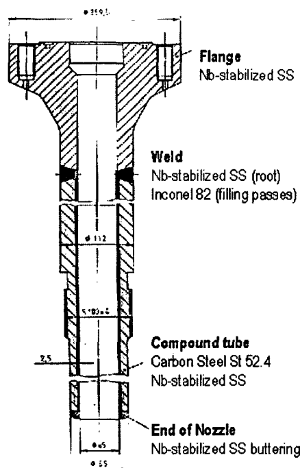
Figure 6 Head Penetration Nozzles: Compound tube St 52.4/1.4550; end of nozzle buttered with Nb-stabilized austenitic SS
