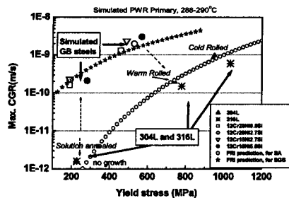
Figure 15 Experimental and predicted CGRs for SGB materials and stainless steels of various YS values in simulated PWR water at 290°C [26]
