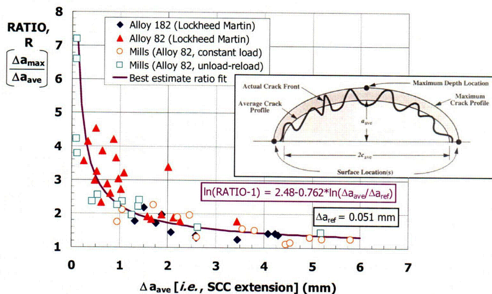
Figure 7. Quantification of the RATIO ( \equiv \Delta a_{\max}/\Delta a_{\text{ave}} ) as a function of crack depth, based on data from [8] and the present work.
