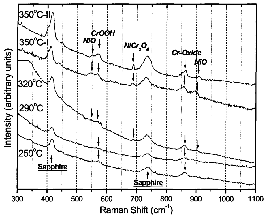
FIGURE 5. In-situ Raman spectra obtained for Alloy 600 by holding at 250, 290, 320 and 350°C, respectively, during heating up to 350 °C in PWR water condition with DH_2=30\text{cc(STP)/kg} .
