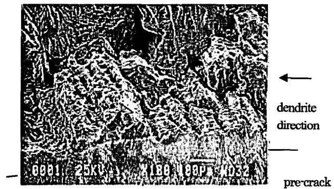
Figure17 Magnification of TP. No. 132-LT2 (Perpendicular to dendrite)
