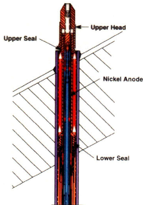
Figure 3. Typical End Effector Tool for Nickel Plating Pressurizer Heater Nozzles.
