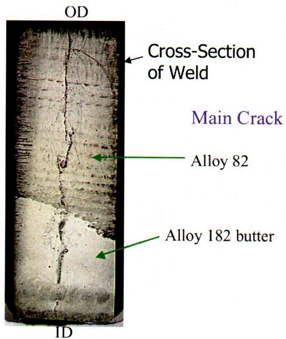
Figure 1. Photographs from the VC Summer hot leg, showing that both Alloys 182 and 82 are susceptible to primary water stress corrosion cracking (source: http://www.nrc.gov/NRC/REACTOR/SUMMER/index.htm ).
