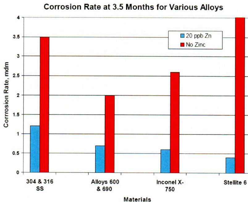
Figure 3 Effect of zinc on corrosion rates of various alloys in laboratory tests (after Esposito et al. [1])
