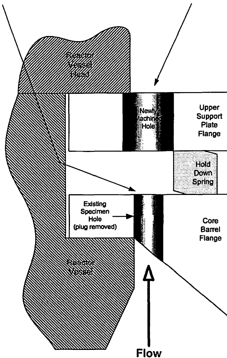
Figure 7: Westinghouse UHTR Implementation Design (1 Unit)
