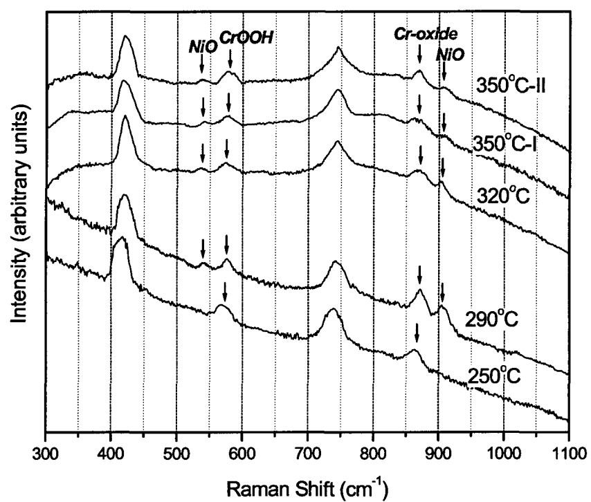
FIGURE 6. In-situ Raman spectra obtained for Alloy 600 by holding at 250, 290, 320 and 350°C, respectively, during heating up to 350°C in PWR water condition with DH_2=1cc(STP)/kg .
