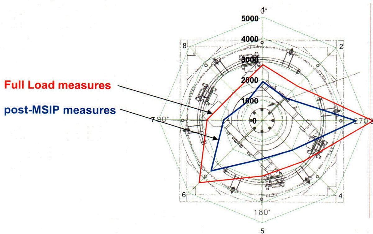
Figure 6 - Polar Plot of Axial Strains (Micro-Inches per Inch)
