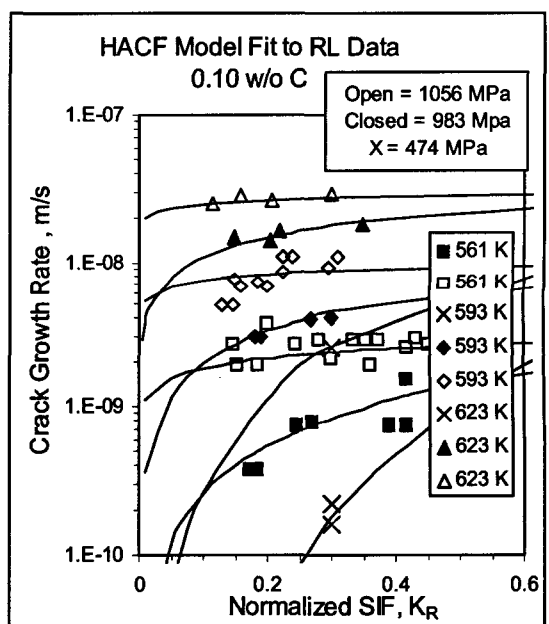
Figure 9. HAF Model Fit to RL CGR Data. Both temperature and yield stress (cold work) effects on CGR are shown.
