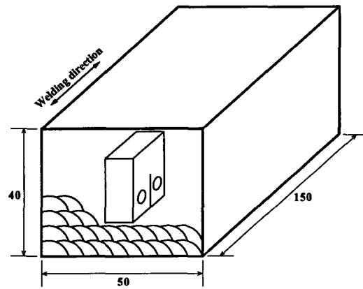
Figure 4 Machining orientations of CT specimens from deposited metal model of TIG welding by Alloy 82
