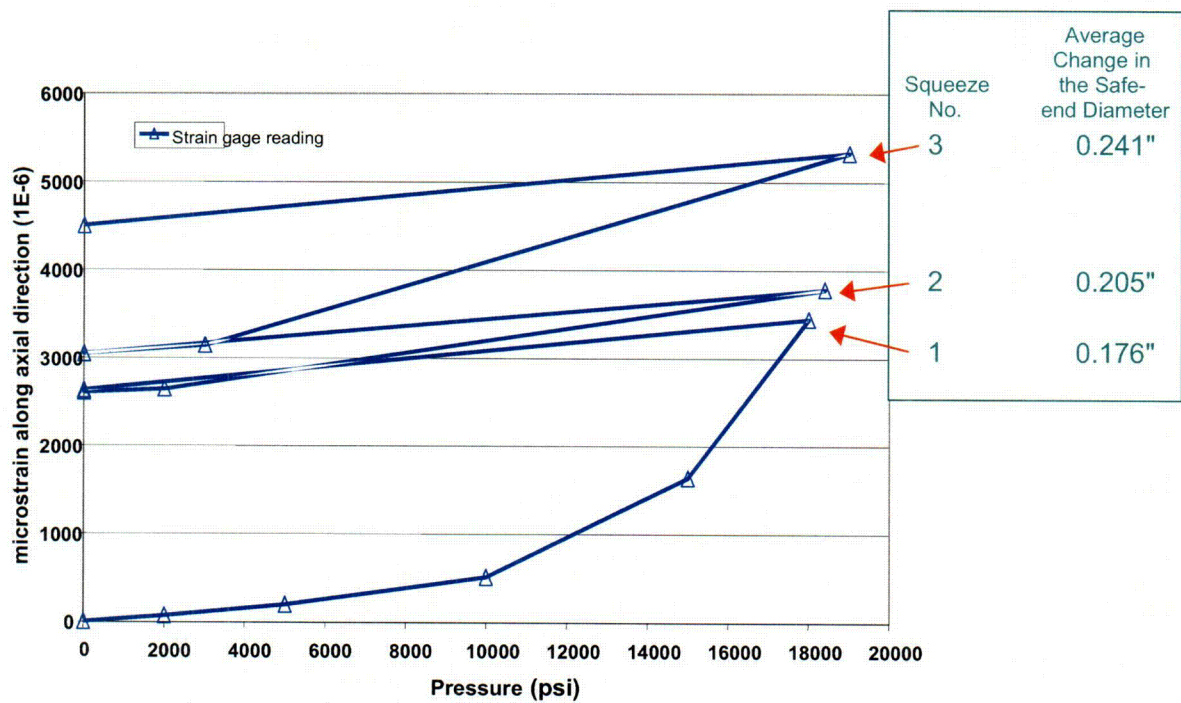
Figure 5 - Safe-end Diameter Changes Associated with the Three MSIP Squeezes
