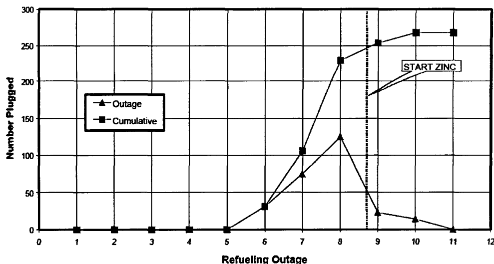
Figure 6 Example of field data from Diablo Canyon Unit 1: plugging for PWSCC at tube-support-plate (TSP) locations
