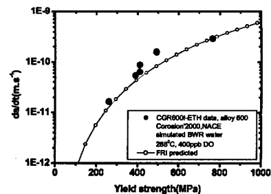
Figure 16 Experimental da/dN-YS curve (ETH data) [25] and FRI prediction line for alloy 600 in simulated BWR water.
