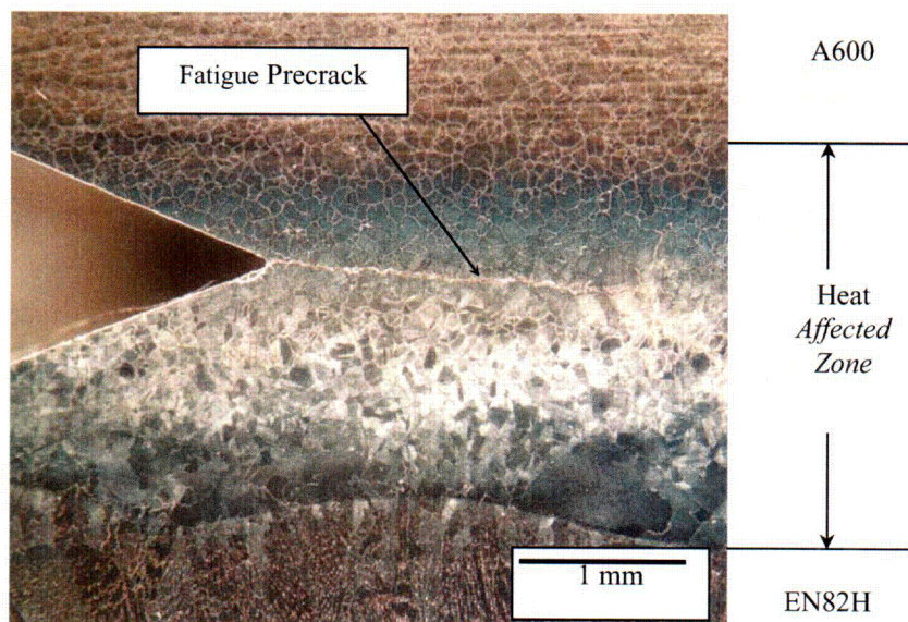
Figure 2. Light macrograph of the CT specimen notch and fatigue precrack. Note that the precrack is entirely within the A600 HAZ. 8:1 Phosphoric Acid, Electrolytic Etch.
