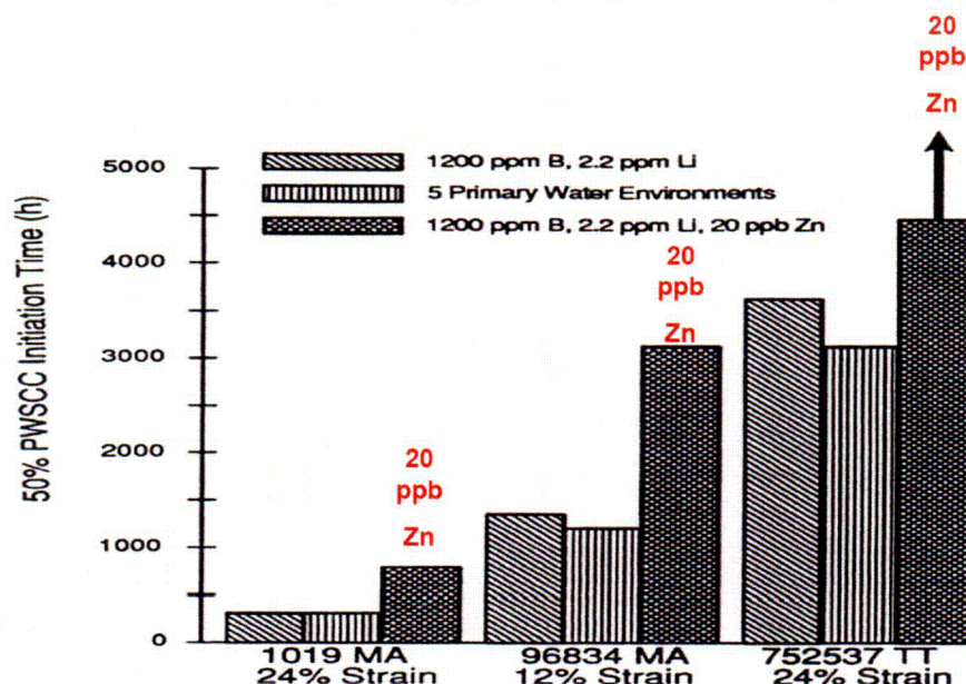
Figure 4 Example for the effect of zinc on time to initiate PWSCC in laboratory tests (after Esposito et al. [1])
