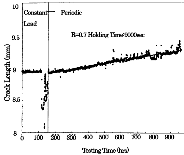
Figure 11 CGR on-line monitoring results ( K=35\text{MPa}\sqrt{\text{m}} , TP. No. MG7-2)
