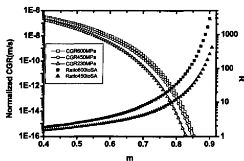
Figure 5. Sensitivity analysis of the effect of YS on CGR for different values of m ( \kappa_a = constant) using Equation (17)
