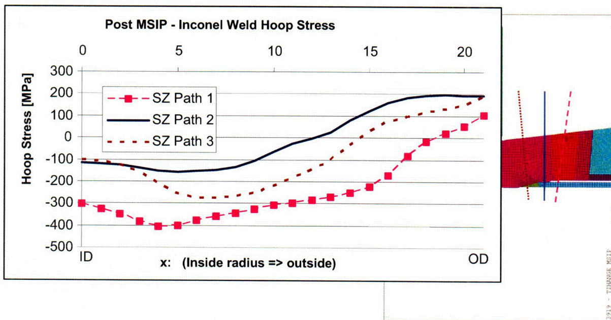
Figure 8 - Predicted Distribution of Through-Wall Strains at the Weld Joint (Ref. 2)
