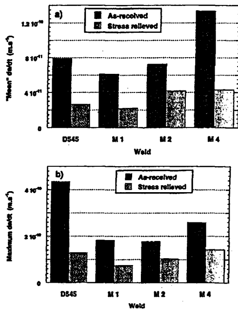
Figure 3 Effects of heat treatment on SCC susceptibility of Alloy 182 [2], results of CGR tests carried out in primary water at 330 °C and an initial K_I of 20 MPaKm
