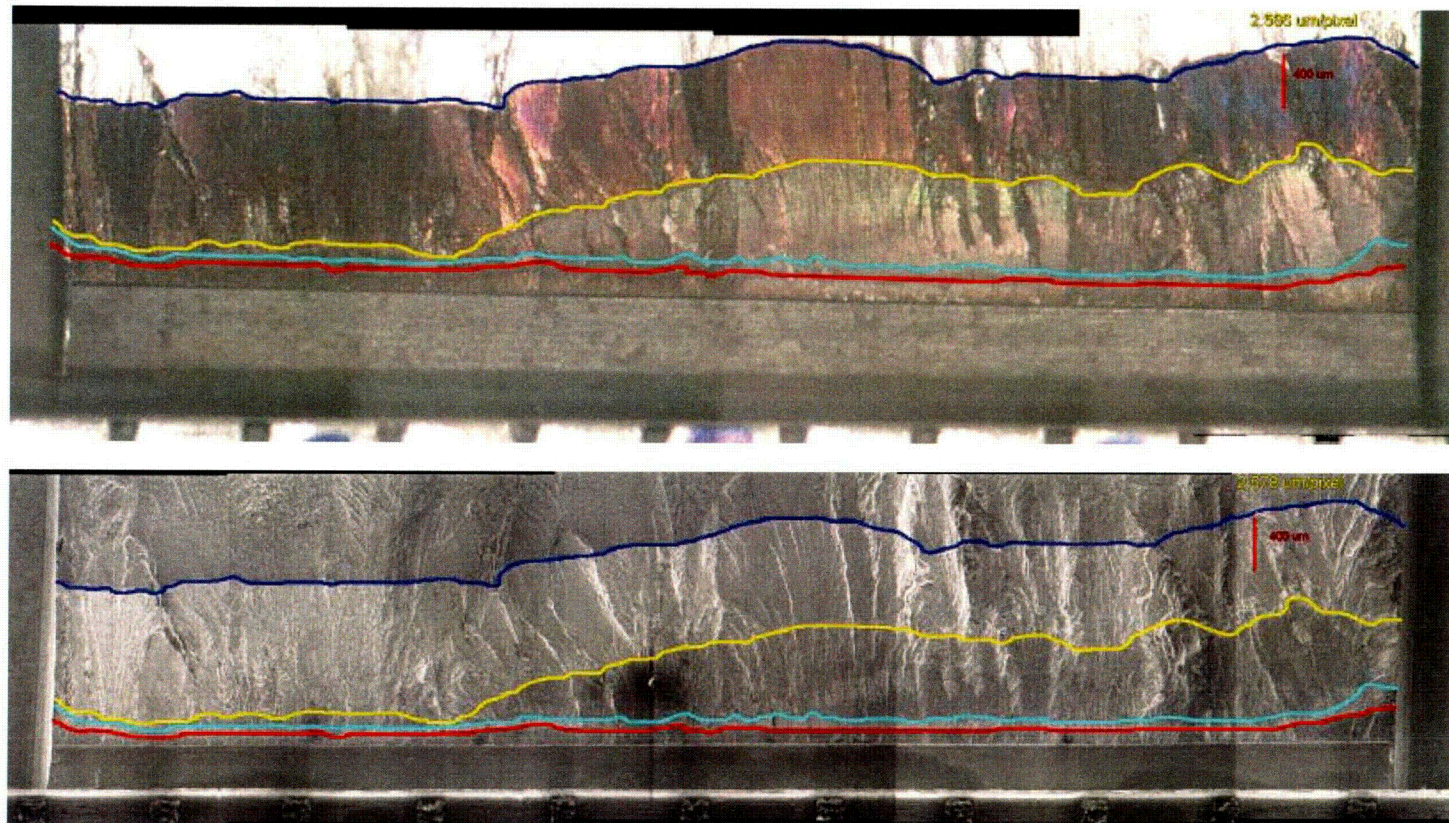
Figure 4 – Optical (top) and SEM (bottom) micrographs of an Alloy 182 crack growth specimen, showing the precrack and environmental crack extension across the face of the specimen.
