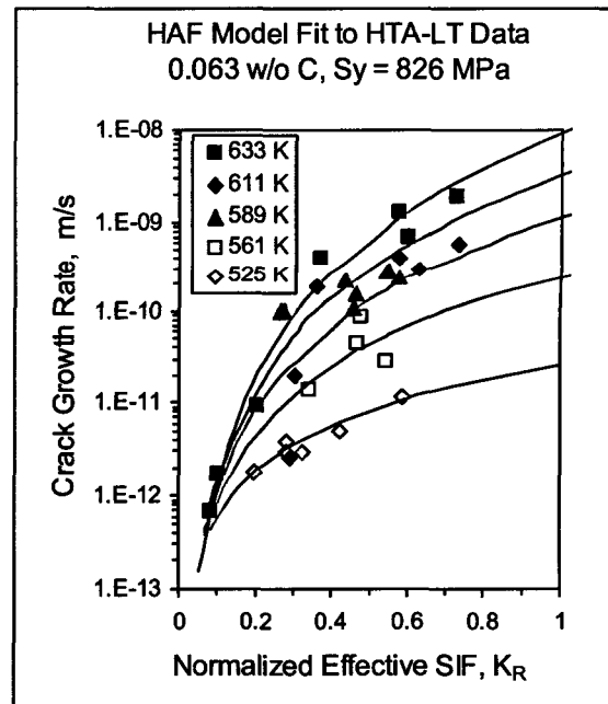
Figure 5. HAF Model Fit to HTA-LT CGR Data. Significant differences exist between LT and ST sensitivities to applied SIF.
