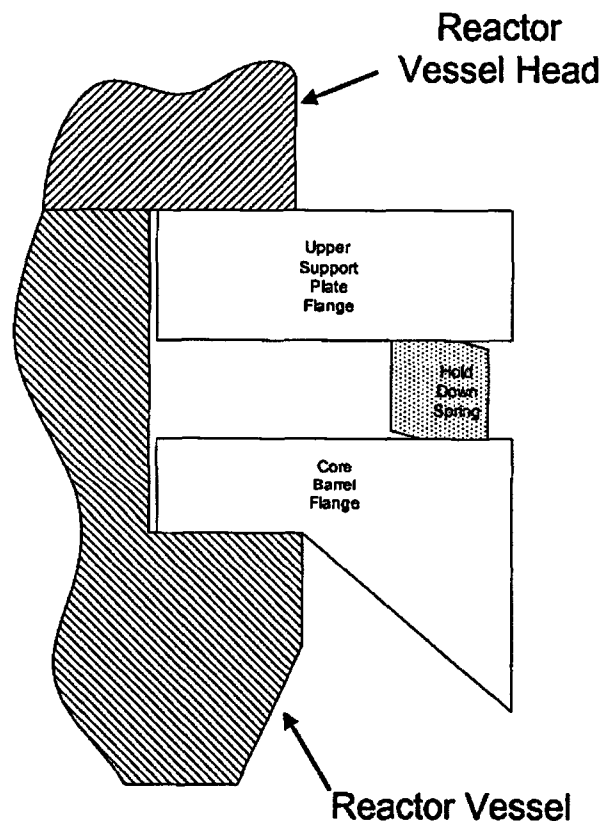
Figure 2: Detail of Components where UHTR Modification is Implemented
