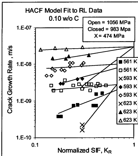
Figure 10. HACF Model Fit to RL CGR Data. Temperature dependence of the SIF exponent is similar to that of HTA-ST data.
