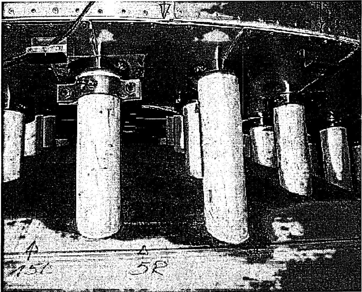
Figure 11 Good accessibility to RPV head penetrations in Siemens/KWU plants
