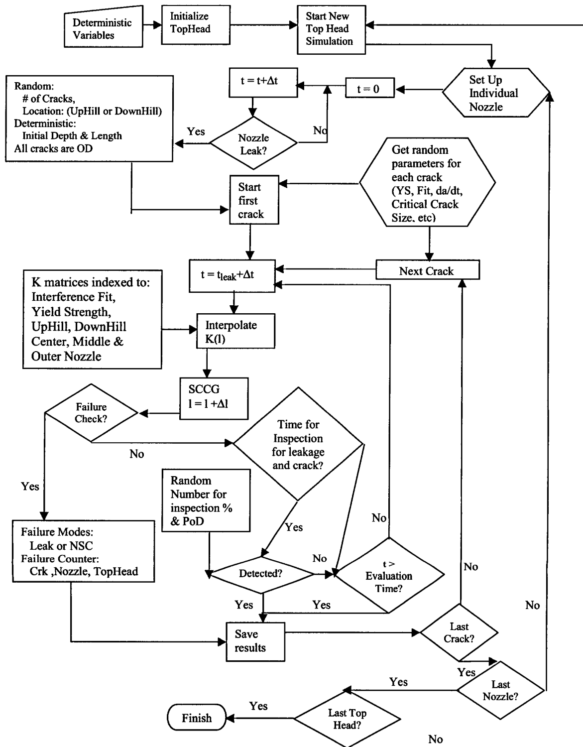
Figure 2 Flow Chart of PFM Methodology
