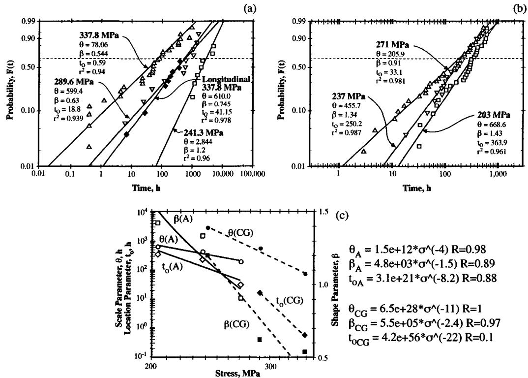
Figure 15 a) Probability vs. time for sensitized Type 304 stainless steel tested at 288°C in high purity oxygenated water. From Clark and Gordon. 31 (b) Probability vs. time for sensitized Type 304 stainless steel tested at 288°C in high purity oxygenated water. From Akashi and Ohtomo. 32 (c) Weibull parameters vs. stress from both the Clark and Gordon (CG) (dotted lines) and Akashi (A) (solid lines) distributions.
