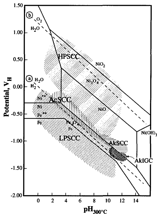
Figure 7 Major submodes of SCC and IGC for Alloy 600 in mill annealed conditions in the range of 280° to 350°C in aqueous solutions. Regions of SCC shown with respect to thermodynamic boundaries for iron and nickel species in water. Regions of SCC submodes shown are based on published experimental data. LPSCC = "low potential SCC." HPSCC = "high potential SCC," MA = "mill annealed." P = "pure water." C = "contaminated."
