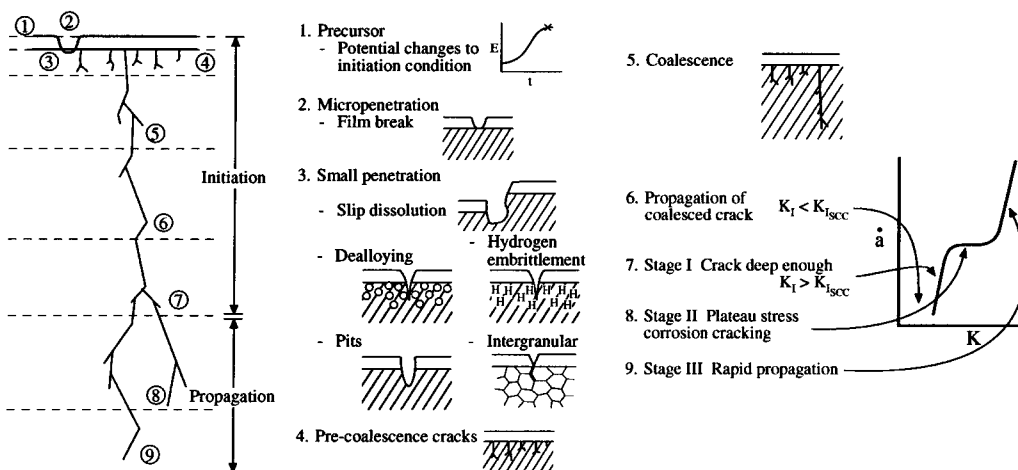
Figure 9 Nine sequential segments of SCC. Practical transition from initiation to propagation shown. Protective film adjusts to the environment.
