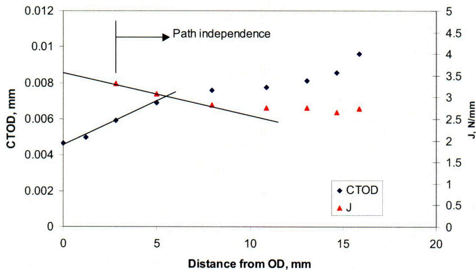
Figure 21 Relationship between CTOD and J at the OD of the nozzle for the baseline case with a 240-degree through-wall crack
