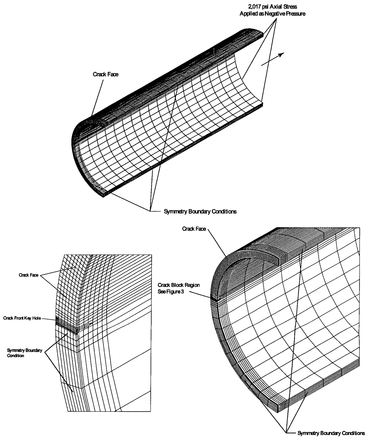
Figure 13 Stress Intensity Model Verification – Pipe with Axial Tension
