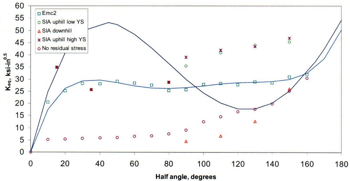
Figure 27 K-solutions for the steepest side-hill baseline case
