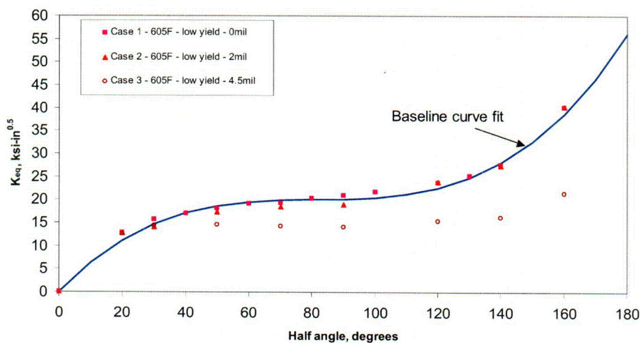
Figure 22 Effects of radial interference fit on the center-hole K-solution
