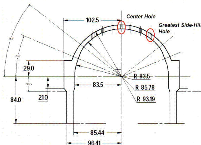
Figure 1 RPV head geometry used in the weld residual stress analysis (length in inches)
