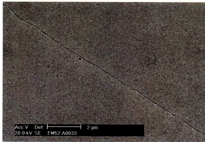
Figure 8. Straight, precipitate-free grain boundary in Filler Metal 52 weld metal.
