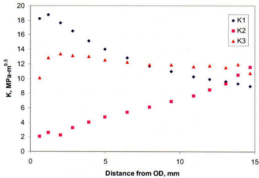
Figure 19 K-solutions for the baseline case with a 100-degree through-wall crack in the center nozzle
