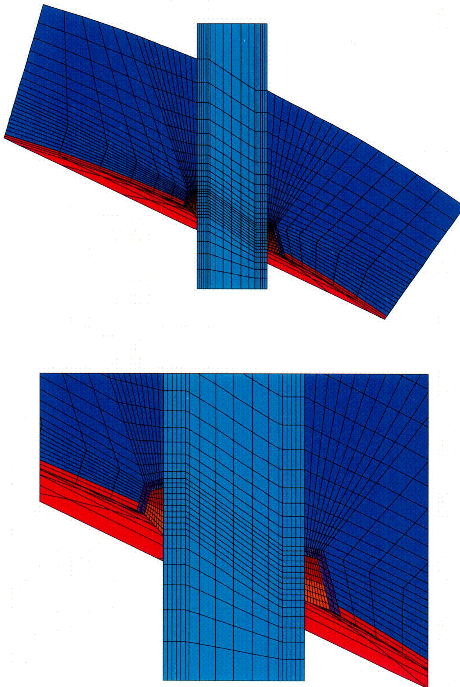
Figure 2 Typical CRDM Nozzle FEA Model
