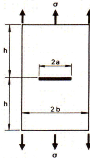
Figure 14 Stress Intensity Model Verification – Through-Wall Center Crack in Plate
