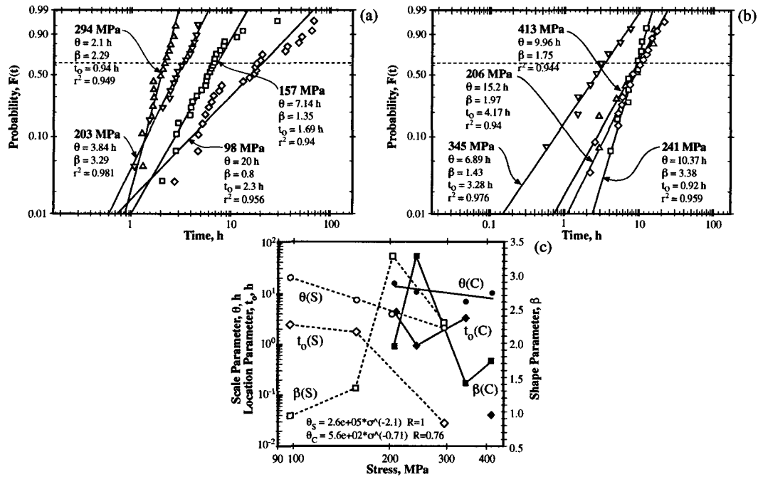
Figure 16 a) Probability vs. time for SCC of Fe-17Cr-11Ni stainless steel exposed to boiling \text{MgCl}_2 at 154^\circ\text{C} and tested at four stresses. These data are a three-parameter fit of the data shown in Figure 31b. From Shibata and Takeyama. 33 (b) Probability vs. time for SCC of Type 310 stainless steel exposed to boiling \text{MgCl}_2 at 154^\circ\text{C} and tested at four stresses. Specimens were prestrained to 130% yield strength. From Cochran and Staehle. 34 (c) Correlation of \theta , \beta , t_o vs. stress.
