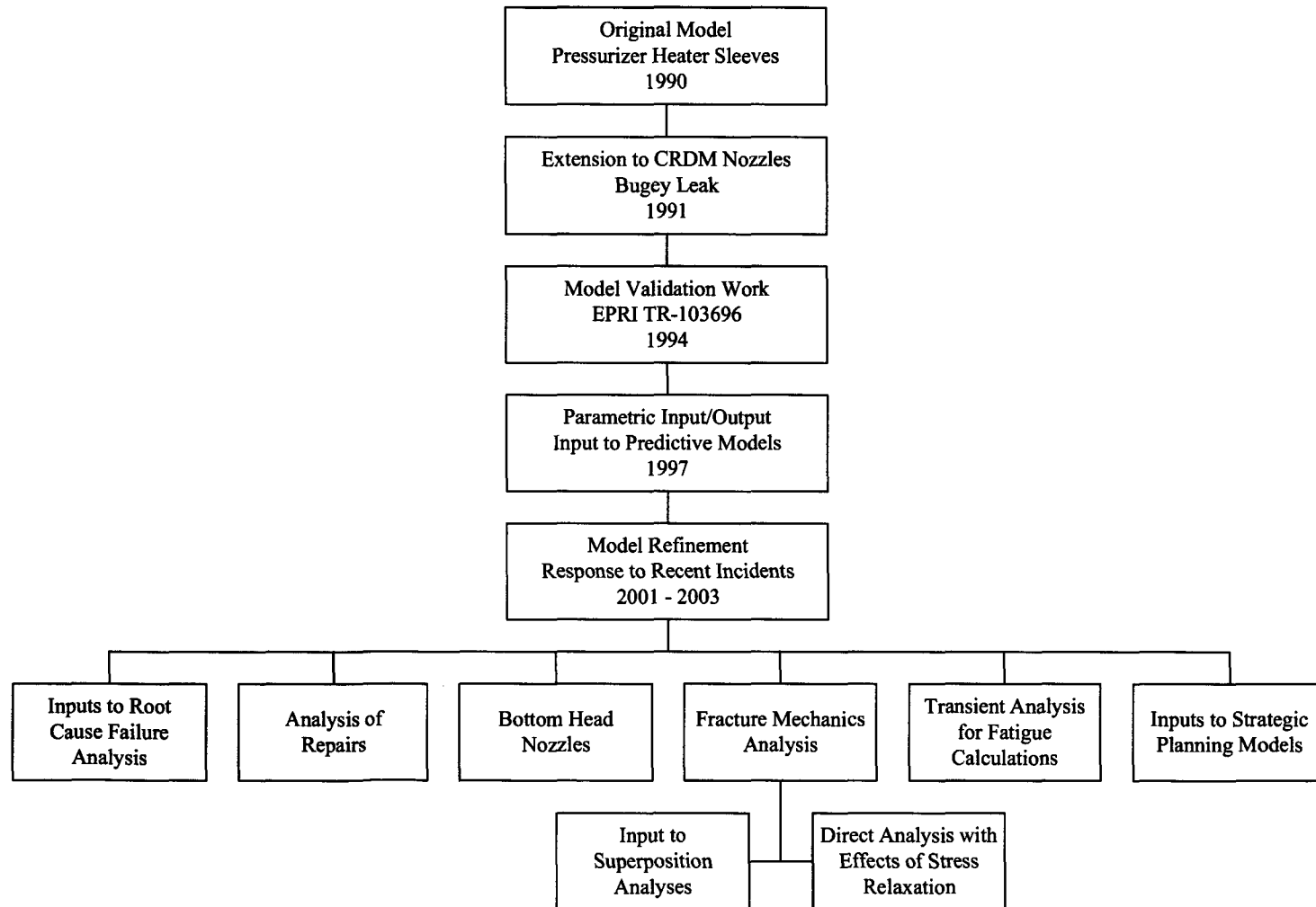
Figure 1 Development of RPV Head Nozzle Stress Analysis Model
