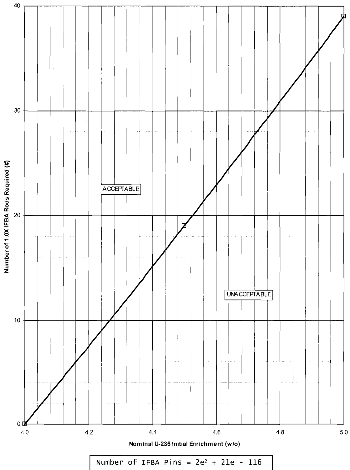
Figure 4.3.1-8 Fresh Fuel IFBA Requirements
