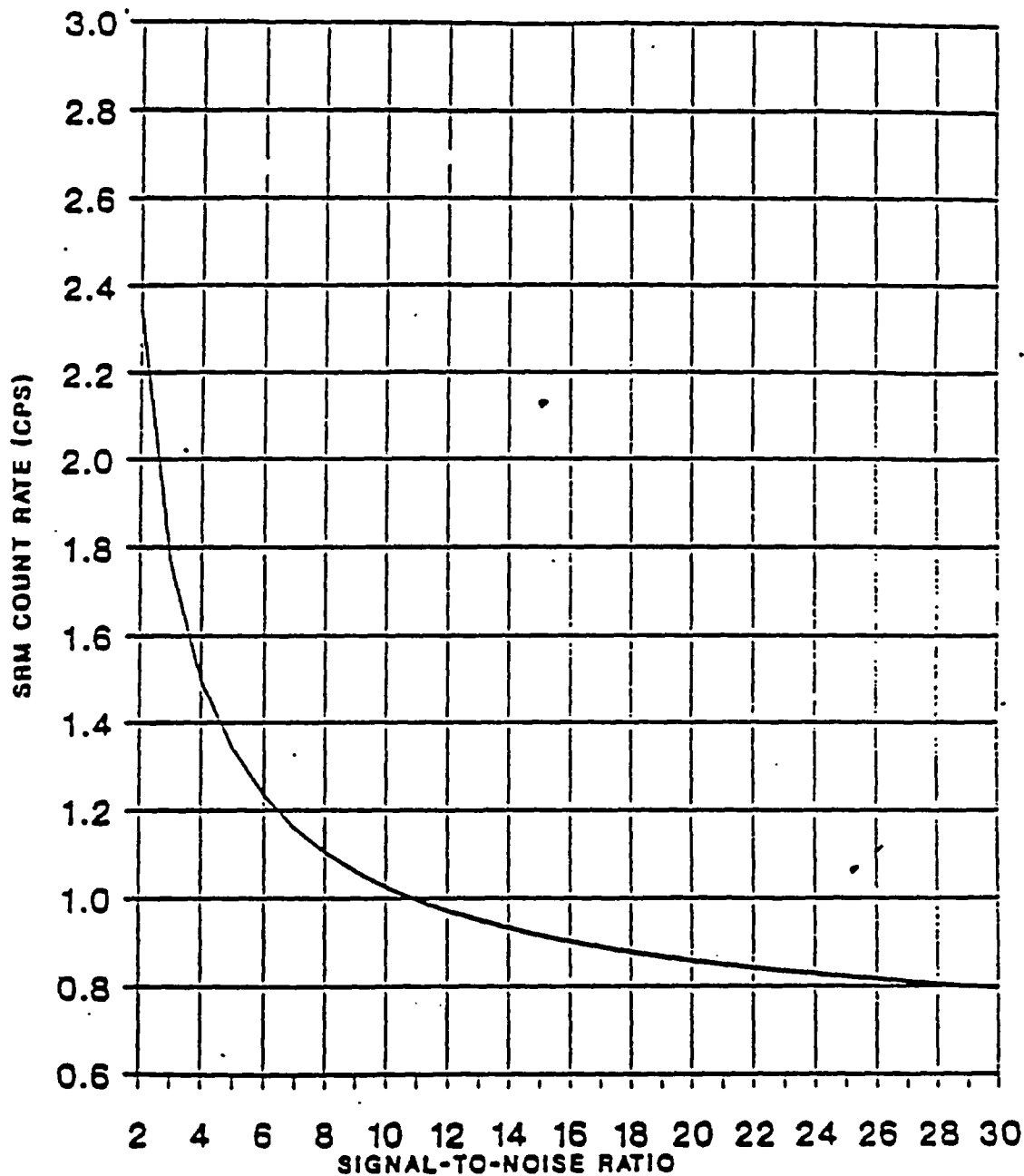
SRM COUNT RATE VERSUS SIGNAL-TO-NOISE RATIO
