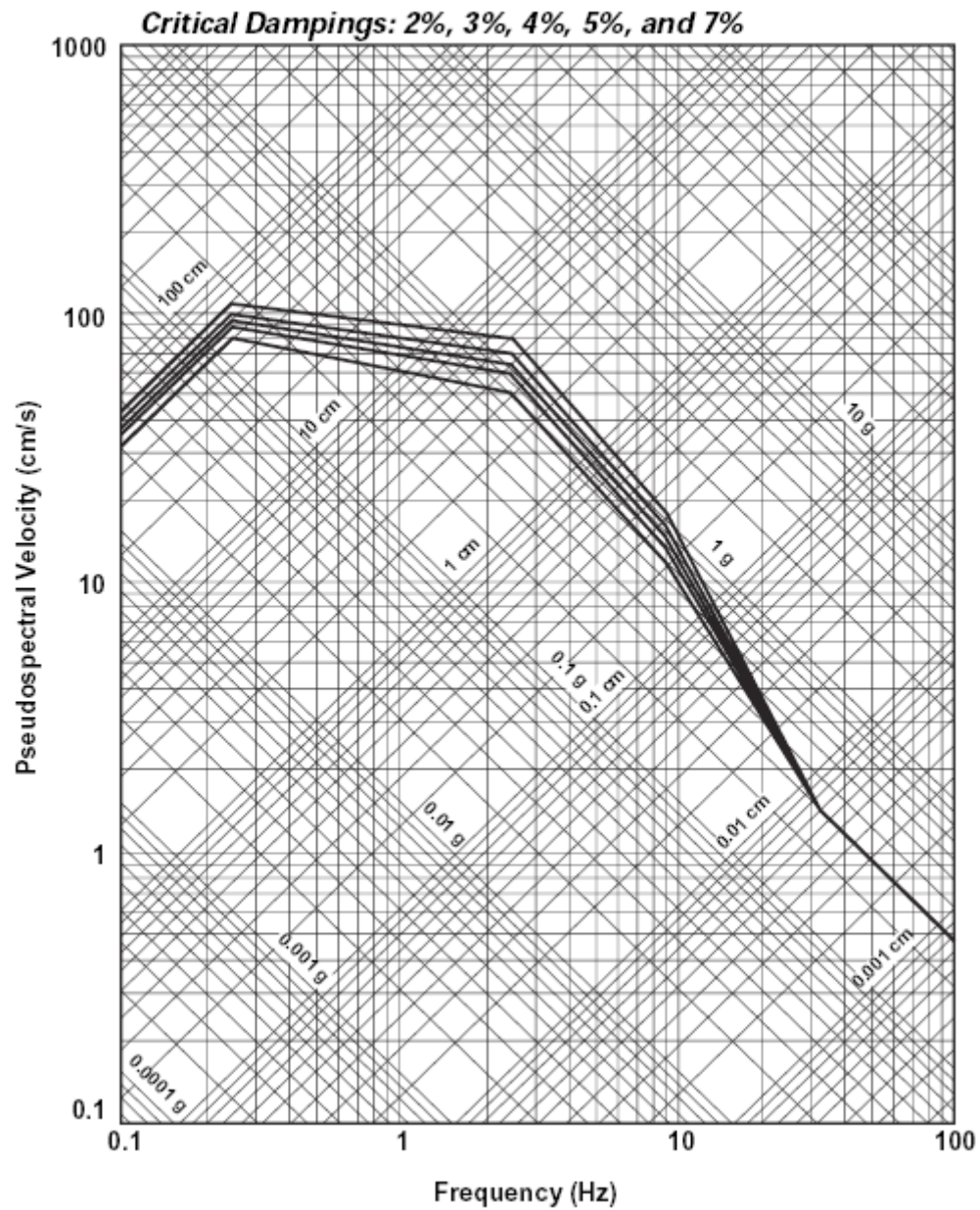
Figure 3.7-1. Horizontal SSE Design Spectra, Generic Site
