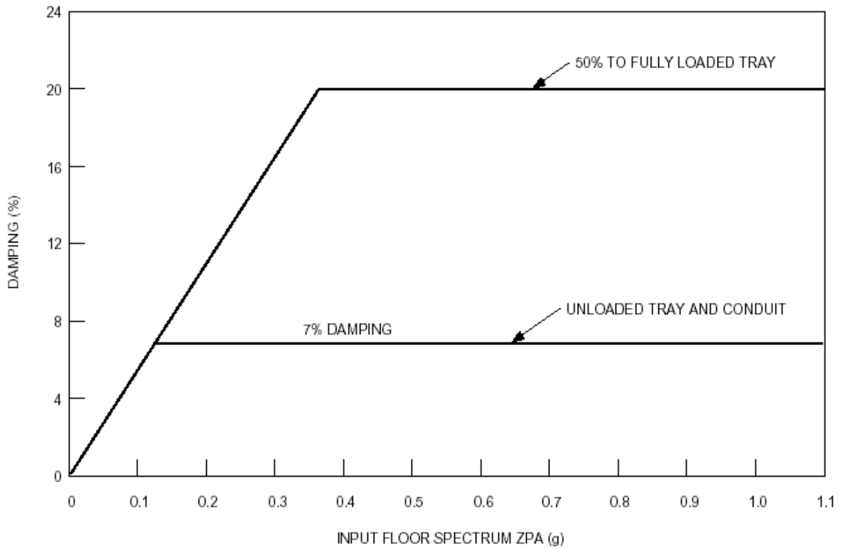
Figure 3.7-36. Damping Values for Electrical Raceway Systems
