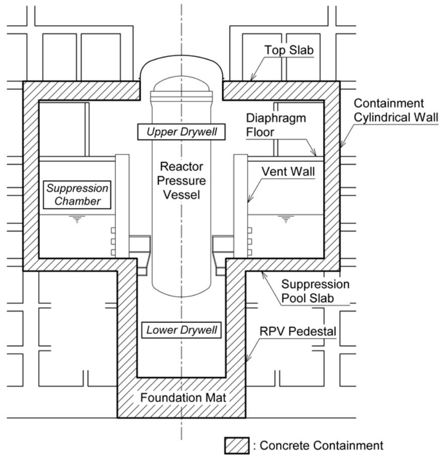
Figure 3.8-1. Configuration of Concrete Containment
