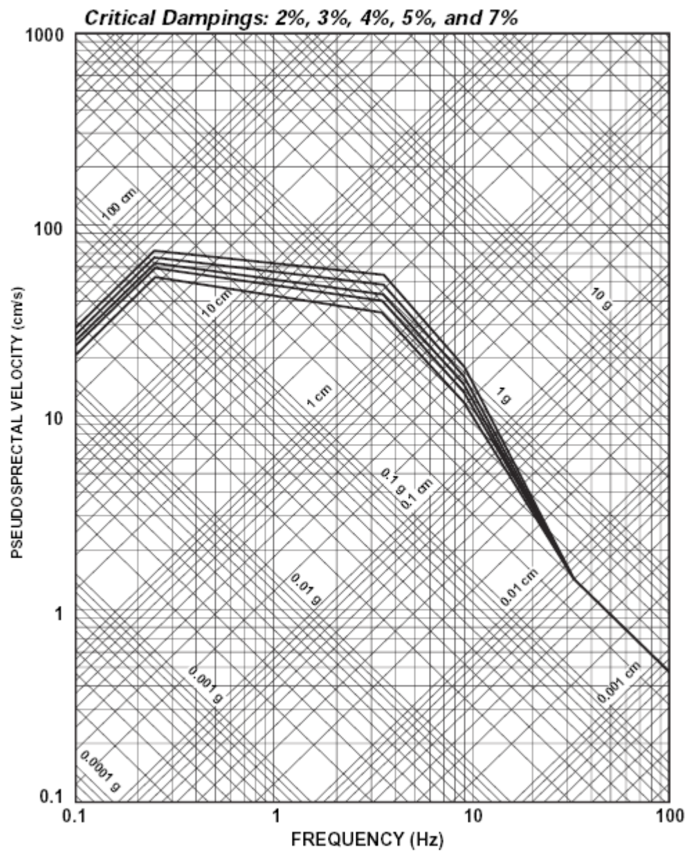
Figure 3.7-2. Vertical SSE Design Spectra, Generic Site
