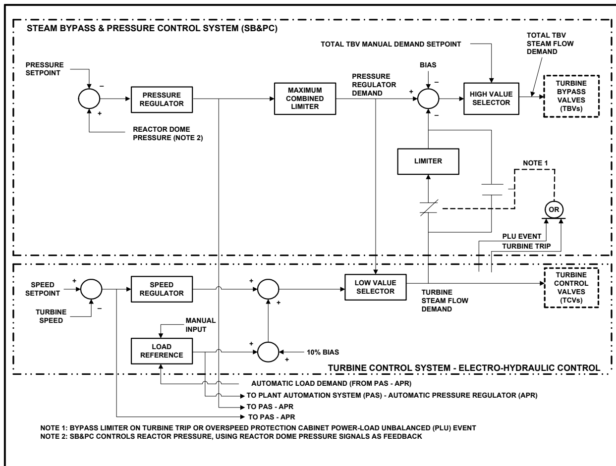
Figure 2.2.9-2. SB&amp;PC Simplified Functional Block Diagram
