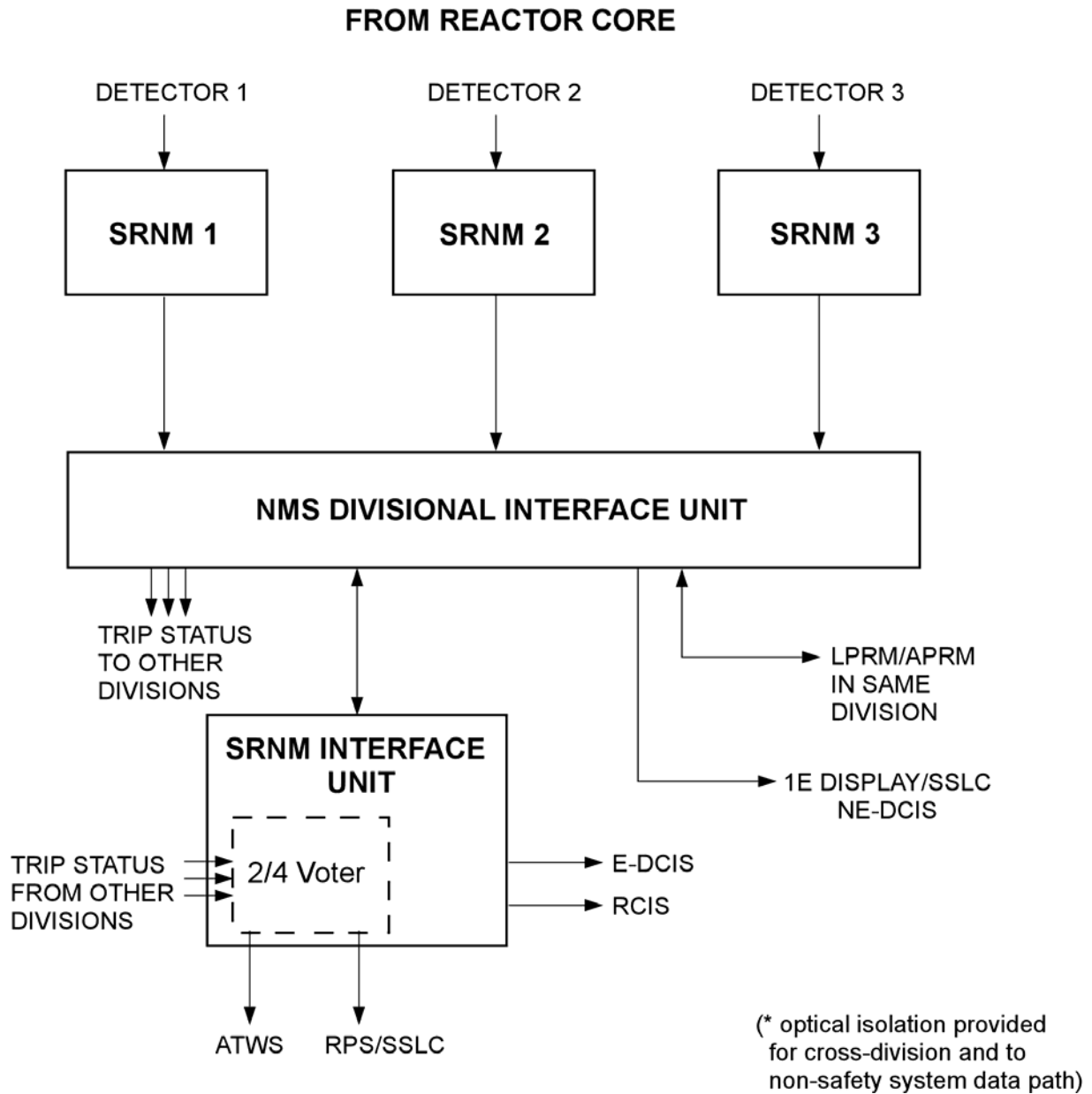
Figure 2.2.5-1A Basic Configuration of a Typical SRNM Division
