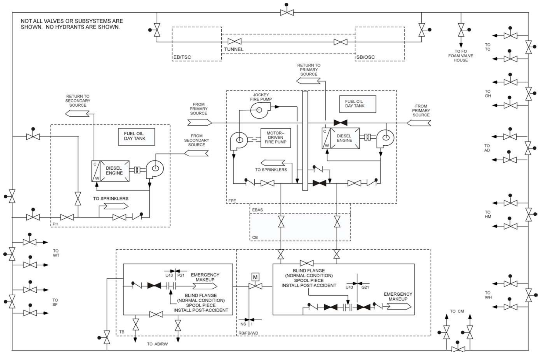
Figure 2.17.3-1 Fire Protection System
