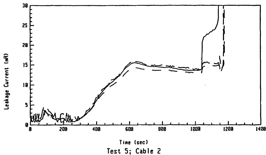
Figure A-2: Leakage Current Data For Test 5 Involving an Aged Rockbestos Cable at an Exposure Temperature of 375°C.
