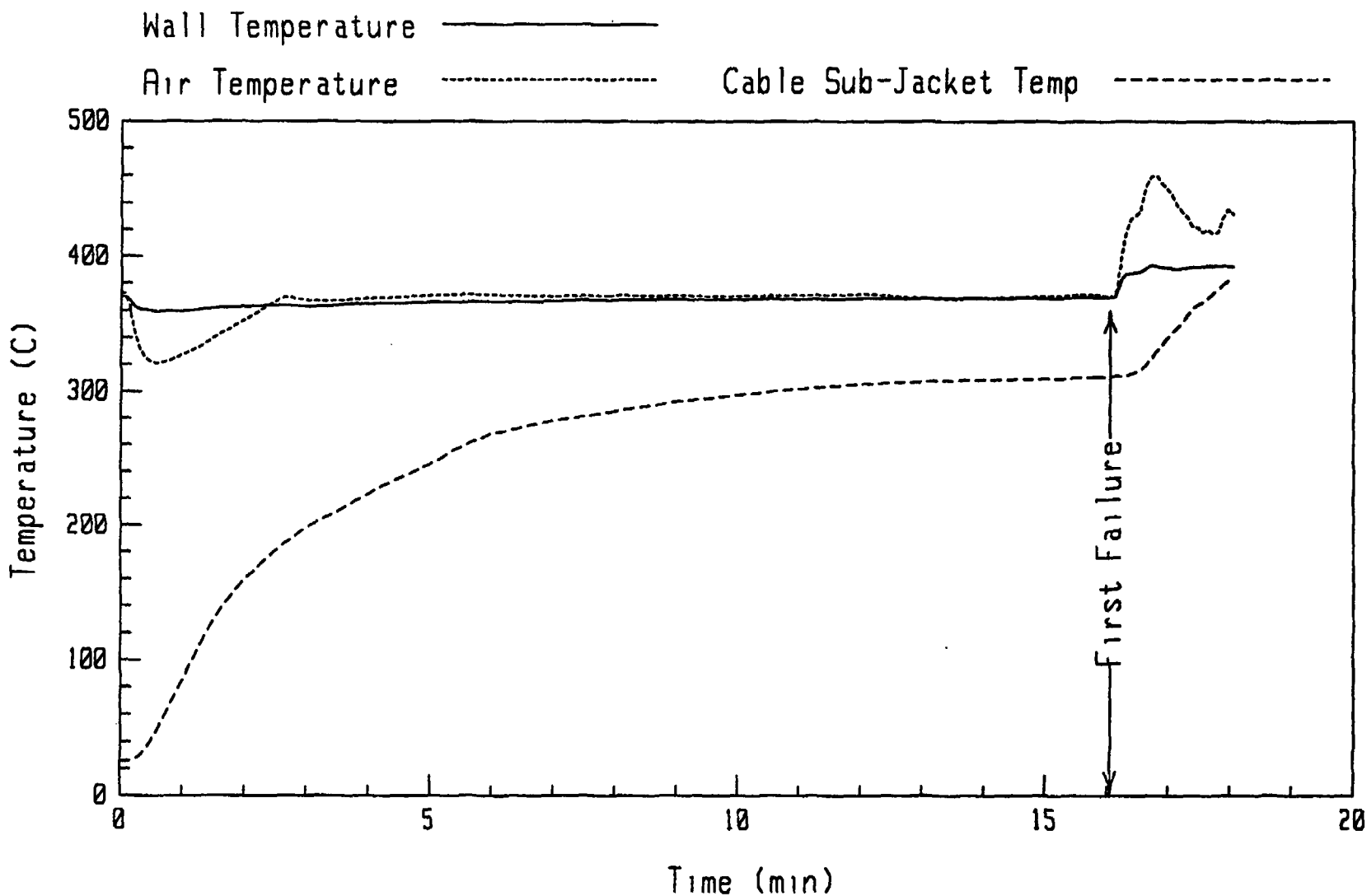
Figure 4.1: Typical Cable Internal Temperature Response for an Unaged Sample of the BIW Cable. This Plot was Taken from Test 31, and Also Illustrates the Consistency of the Exposure Environment. Note that Cable Insertion Occurred at (Time = 0) in this Plot.
