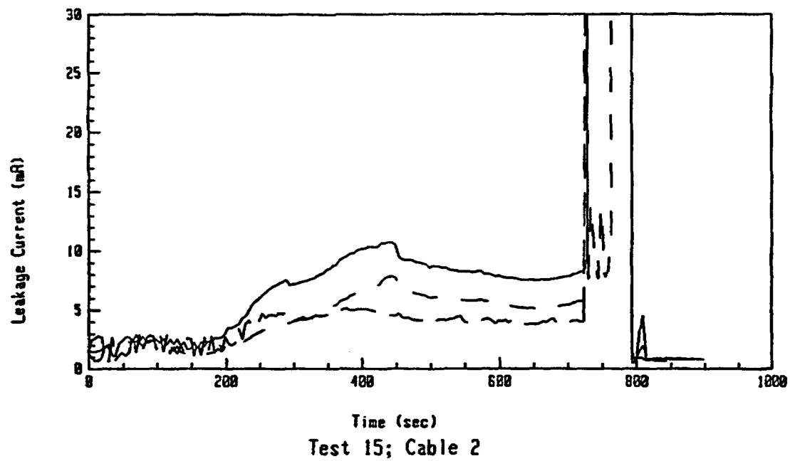
Figure A-12: Leakage Current Data For Test 15 Involving an Aged BIW Cable at an Exposure Temperature of 375°C.
