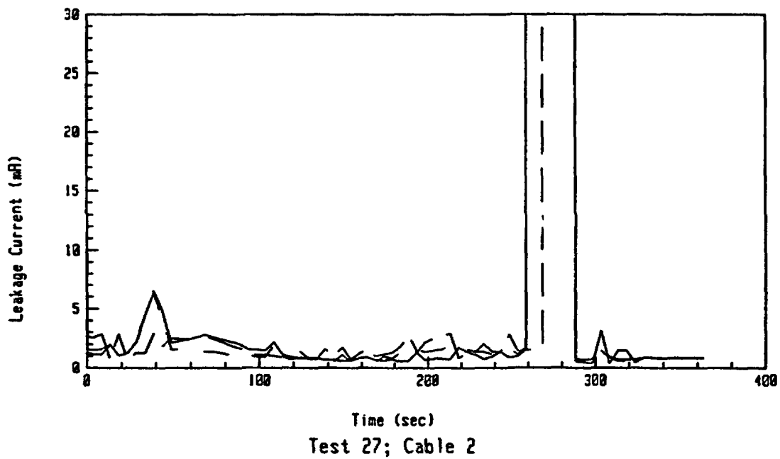
Figure A-24: Leakage Current Data For Test 27 Involving an Unaged BIW Cable at an Exposure Temperature of 425°C.
