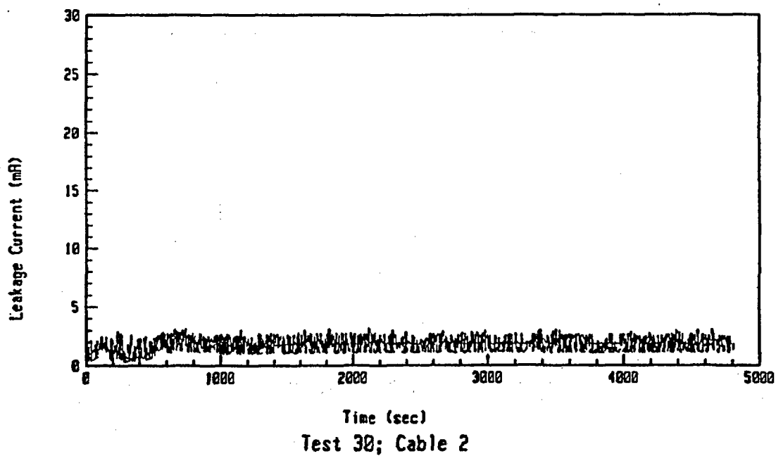
Figure A-27: Leakage Current Data For Test 30 Involving an Unaged BIW Cable at an Exposure Temperature of 365°C.
