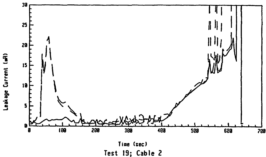
Figure A-16: Leakage Current Data For Test 19 Involving an Unaged Rockbestos Cable at an Exposure Temperature of 350°C.
