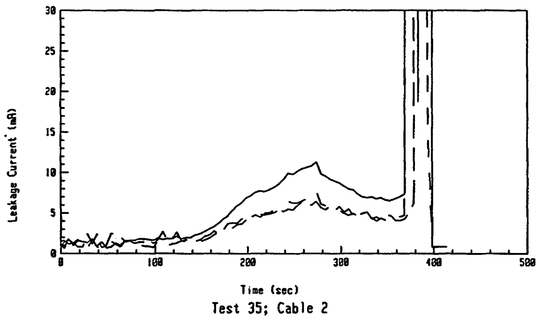
Figure A-32: Leakage Current Data For Test 35 Involving an Aged BIW Cable at an Exposure Temperature of 425°C.
