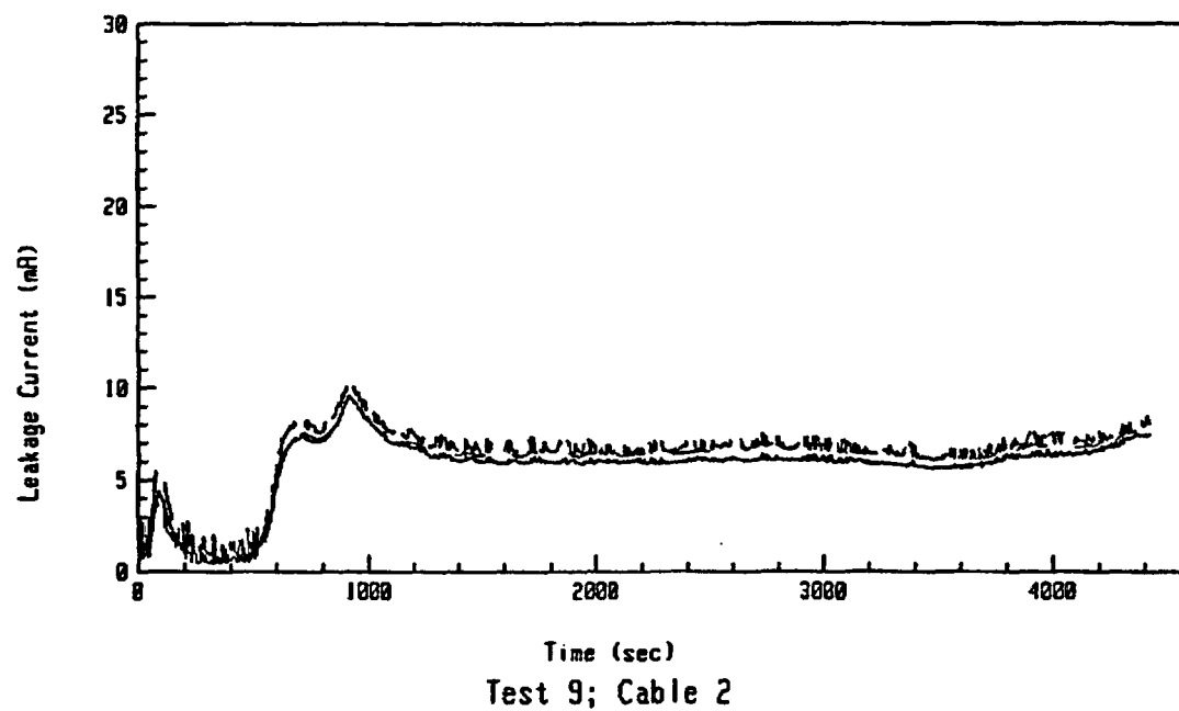
Figure A-6: Leakage Current Data For Test 9 Involving an Unaged Rockbestos Cable at an Exposure Temperature of 325°C.
