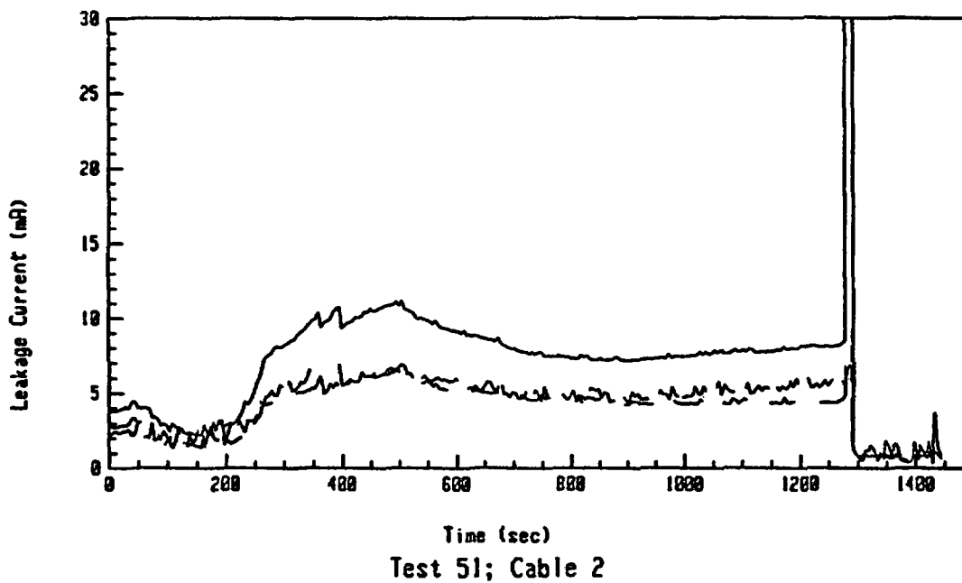
Figure A-48: Leakage Current Data For Test 51 Involving an Aged BIW Cable at an Exposure Temperature of 360°C.
