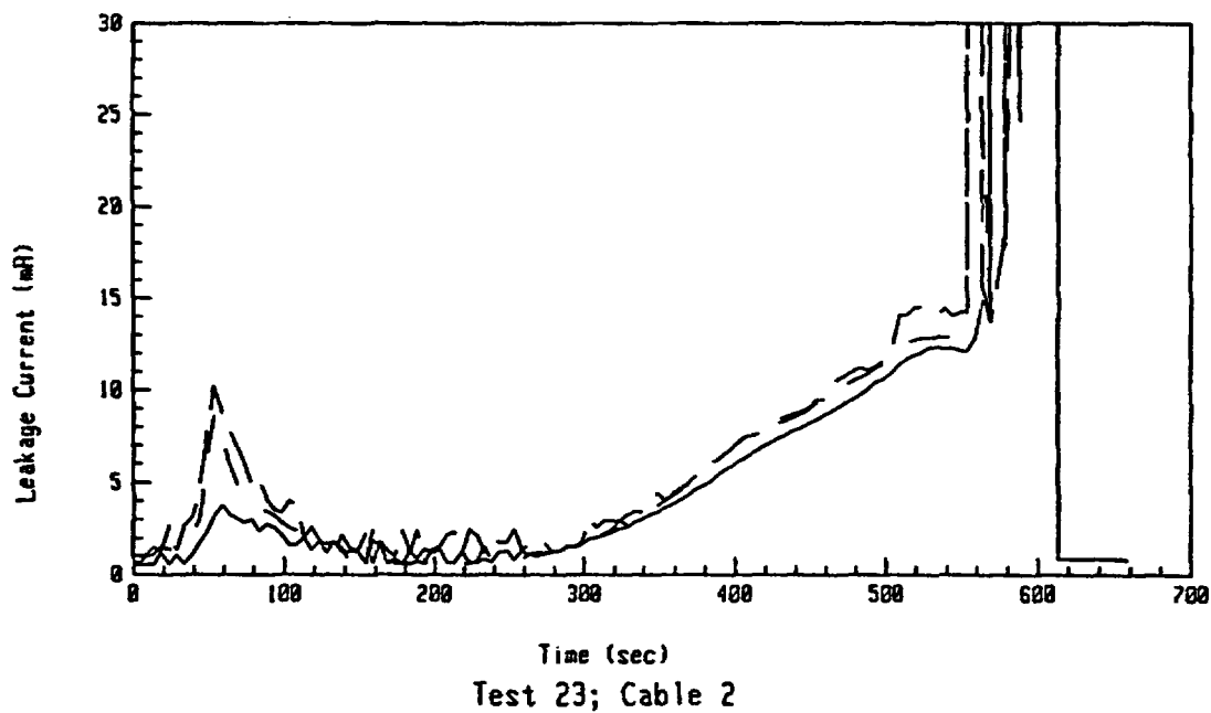
Figure A-20: Leakage Current Data For Test 23 Involving an Aged Rockbestos Cable at an Exposure Temperature of 400°C.
