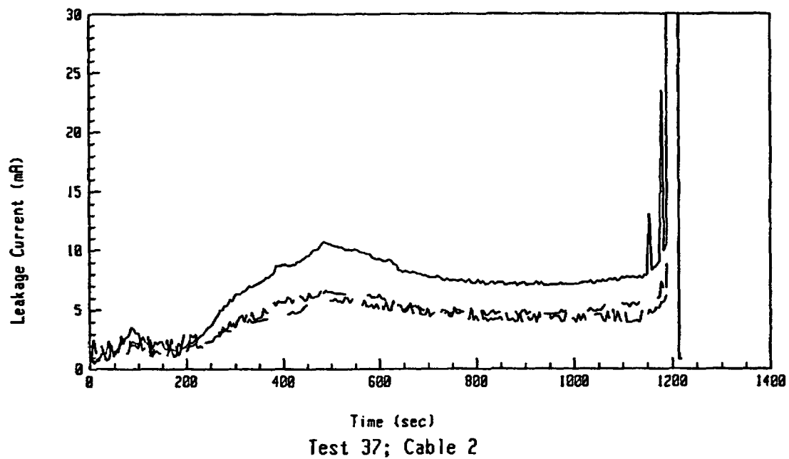
Figure A-34: Leakage Current Data For Test 37 Involving an Aged BIW Cable at an Exposure Temperature of 365°C.
