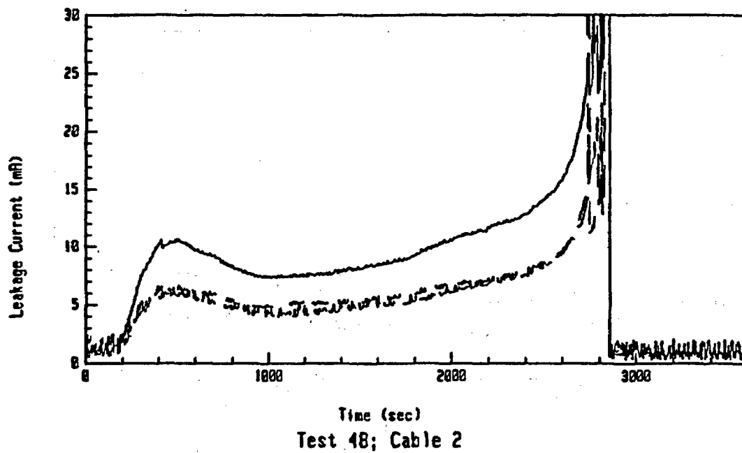
Figure A-45: Leakage Current Data For Test 48 Involving an Aged BIW Cable at an Exposure Temperature of 350°C.
