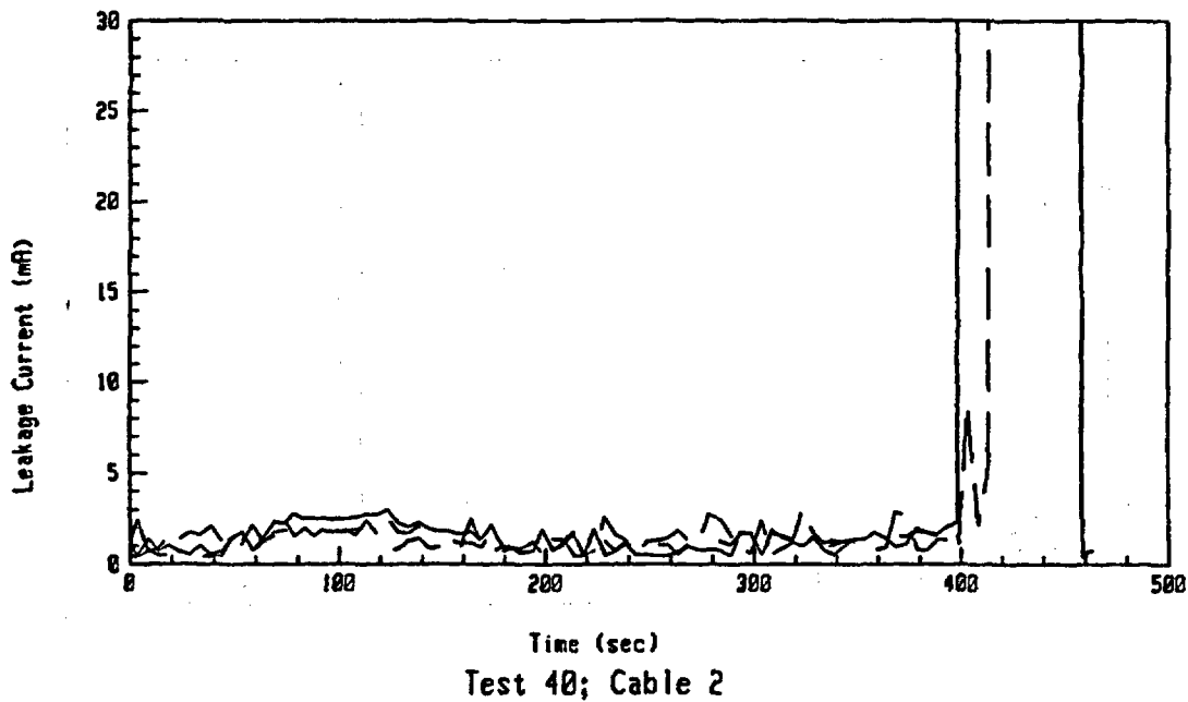
Figure A-37: Leakage Current Data For Test 40 Involving an Unaged BIW Cable at an Exposure Temperature of 400°C.
