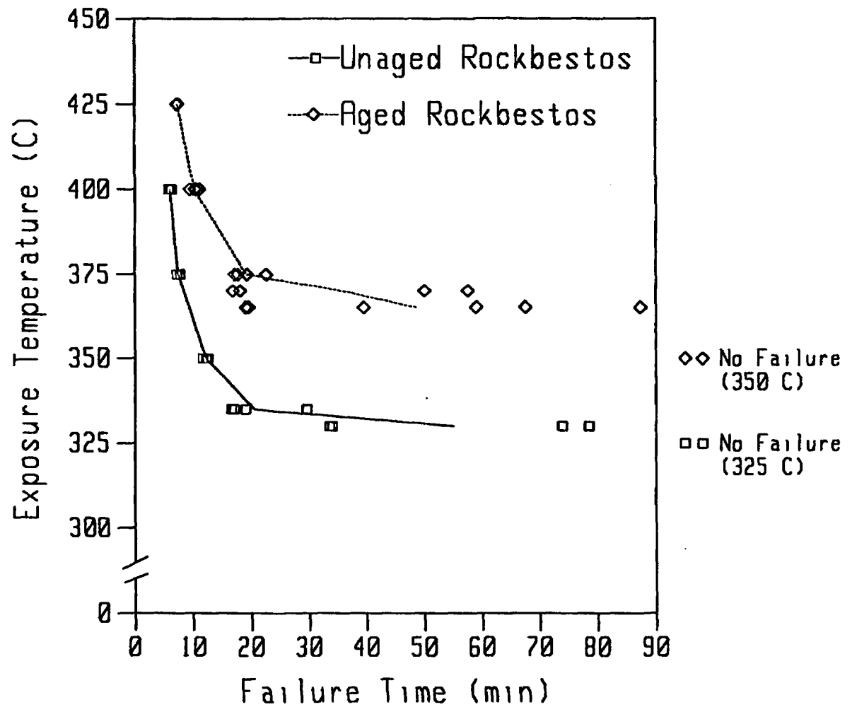
Figure 3.3: Cable Thermal Damage Data for Both the Aged and Unaged Samples of the Rockbestos Firewall III Neoprene/XPE Cables.
