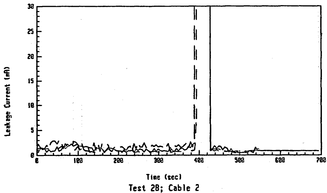
Figure A-25: Leakage Current Data For Test 28 Involving an Unaged BIW Cable at an Exposure Temperature of 400°C.
