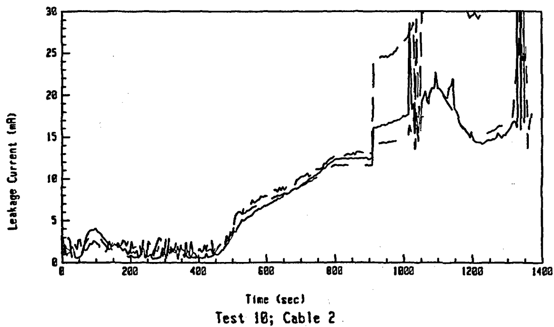
Figure A-7: Leakage Current Data For Test 10 Involving an Unaged Rockbestos Cable at an Exposure Temperature of 335°C.
