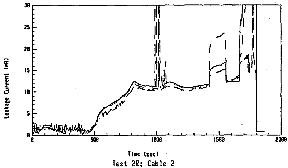
Figure A-17: Leakage Current Data For Test 20 Involving an Unaged Rockbestos Cable at an Exposure Temperature of 335°C.
