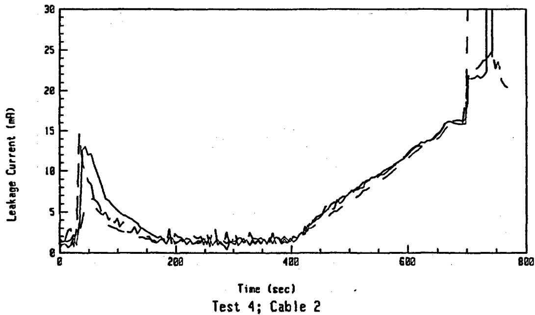
Figure A-1: Leakage Current Data For Test 4 Involving an Unaged Rockbestos Cable at an Exposure Temperature of 350°C.
