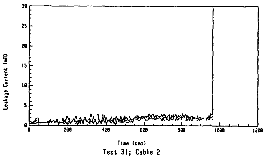
Figure A-28: Leakage Current Data For Test 31 Involving an Unaged BIW Cable at an Exposure Temperature of 370°C.
