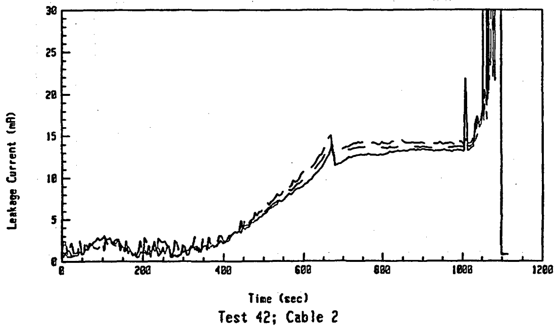
Figure A-39: Leakage Current Data For Test 42 Involving an Aged Rockbestos Cable at an Exposure Temperature of 370°C.
