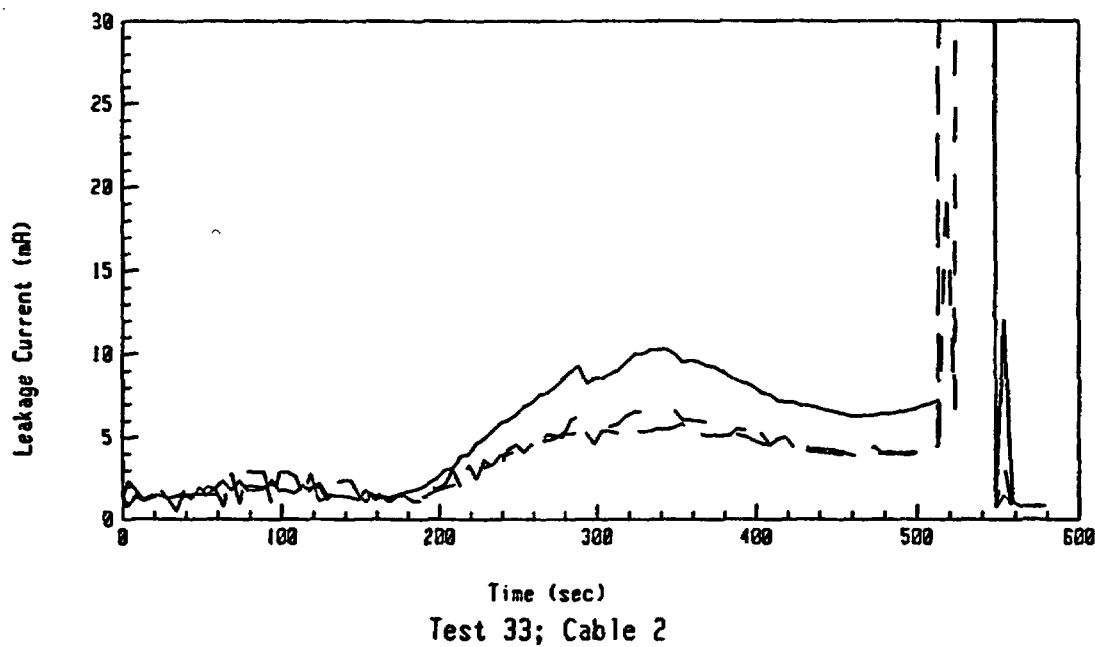
Figure A-30: Leakage Current Data For Test 33 Involving an Aged BIW Cable at an Exposure Temperature of 400°C.
