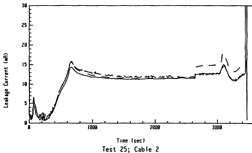
Figure A-22: Leakage Current Data For Test 25 Involving an Aged Rockbestos Cable at an Exposure Temperature of 370°C.
