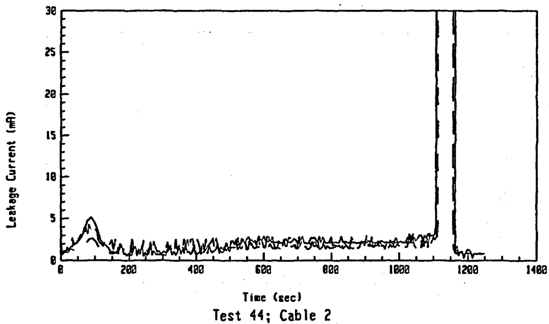
Figure A-41: Leakage Current Data For Test 44 Involving an Unaged BIW Cable at an Exposure Temperature of 370°C.
