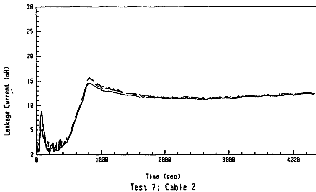
Figure A-4: Leakage Current Data For Test 7 Involving an Aged Rockbestos Cable at an Exposure Temperature of 350°C.
