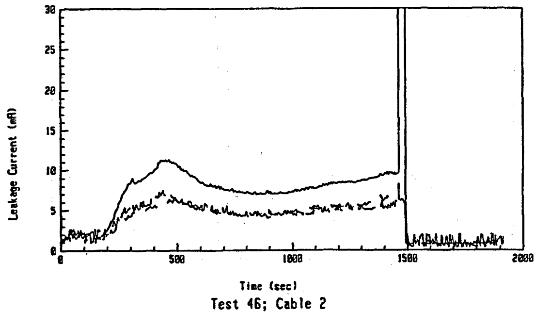
Figure A-43: Leakage Current Data For Test 46 Involving an Aged BIW Cable at an Exposure Temperature of 360°C.
