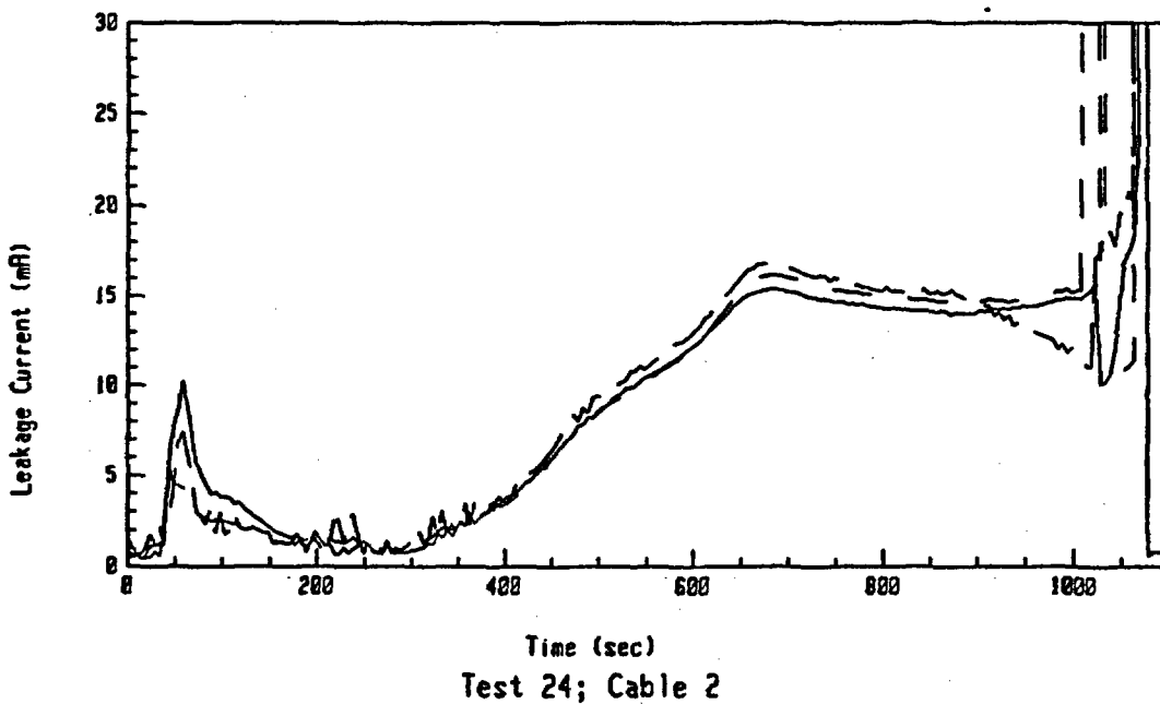
Figure A-21: Leakage Current Data For Test 24 Involving an Aged Rockbestos Cable at an Exposure Temperature of 375°C.
