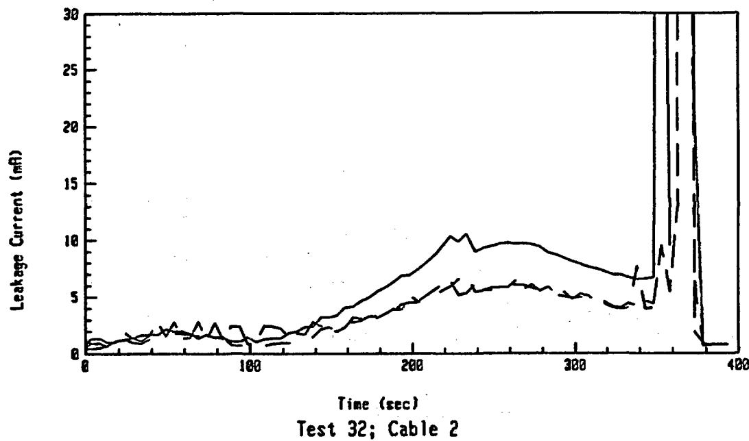
Figure A-29: Leakage Current Data For Test 32 Involving an Aged BIW Cable at an Exposure Temperature of 425°C.
