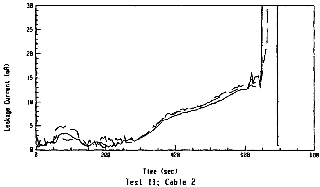
Figure A-8: Leakage Current Data For Test 11 Involving an Aged Rockbestos Cable at an Exposure Temperature of 400°C.
