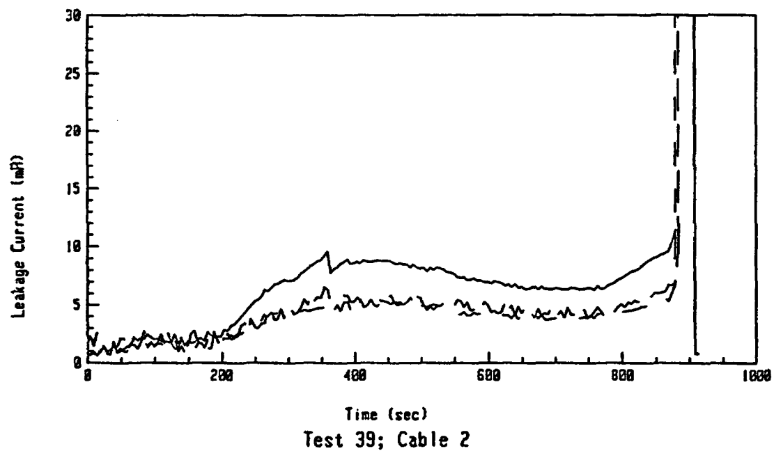
Figure A-36: Leakage Current Data For Test 39 Involving an Aged BIW Cable at an Exposure Temperature of 375°C.
