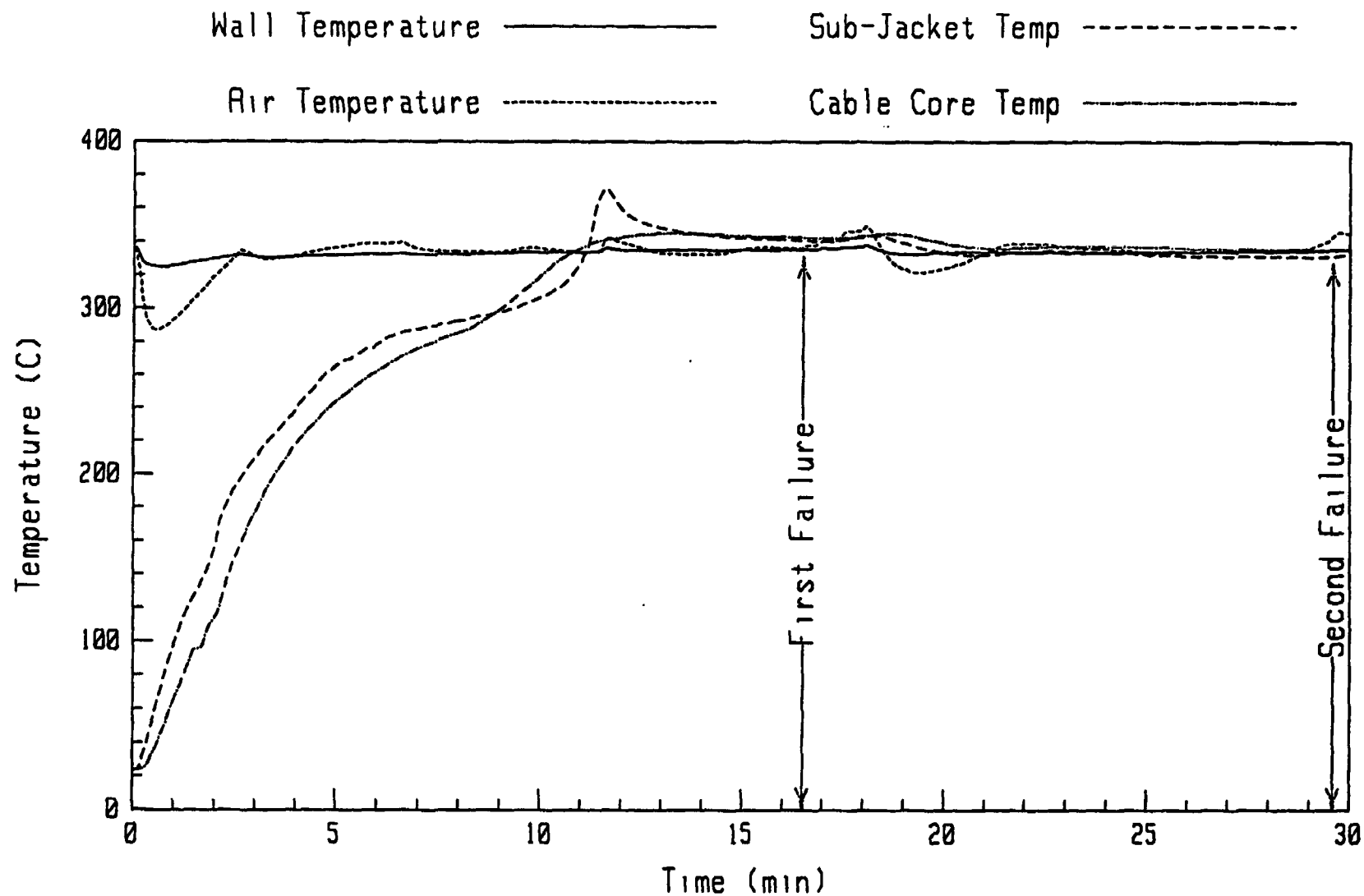
Figure 3.1: Typical Cable Internal Temperature Response for an Unaged Sample of the Rockbestos Cable. This Plot was Taken from Test 20, and Also Illustrates the Consistency of the Exposure Environment. Note that Cable Insertion Occurred at (Time = 0) in this Plot.
