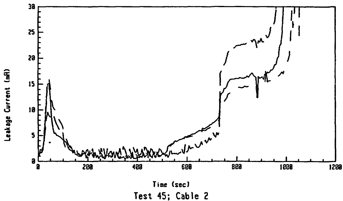
Figure A-42: Leakage Current Data For Test 45 Involving an Unaged Rockbestos Cable at an Exposure Temperature of 330°C.
