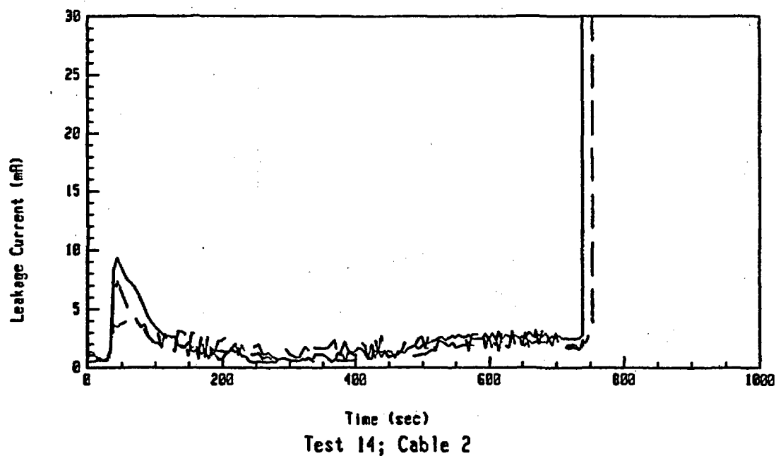
Figure A-11: Leakage Current Data For Test 14 Involving an Unaged BIW Cable at an Exposure Temperature of 375°C.
