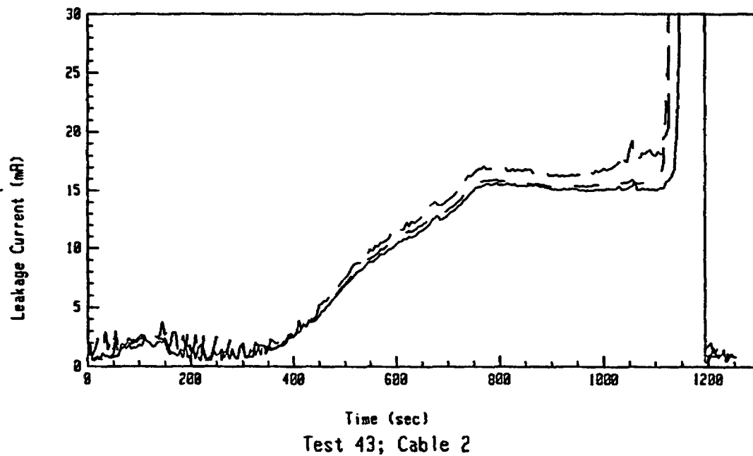
Figure A-40: Leakage Current Data For Test 43 Involving an Aged Rockbestos Cable at an Exposure Temperature of 365°C.
