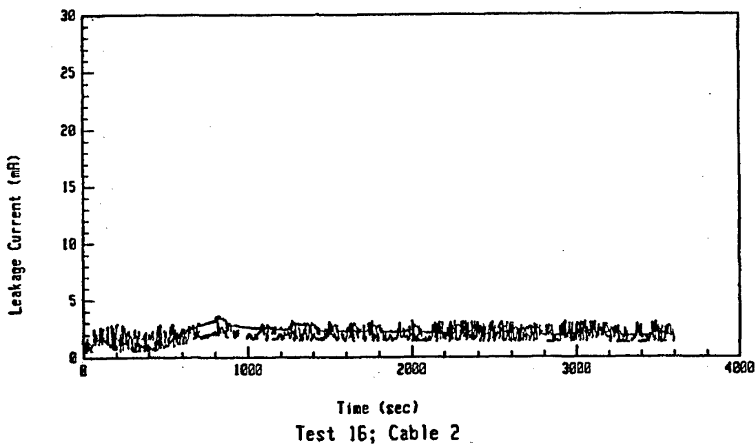
Figure A-13: Leakage Current Data For Test 16 Involving an Unaged BIW Cable at an Exposure Temperature of 350°C.
