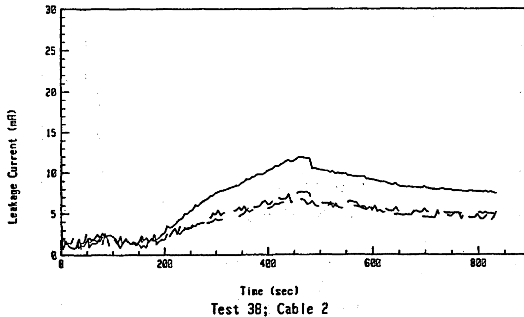
Figure A-35: Leakage Current Data For Test 38 Involving an Aged BIW Cable at an Exposure Temperature of 365°C. Note that a failure in the data logging system occurred prior to the observed cable failures.
