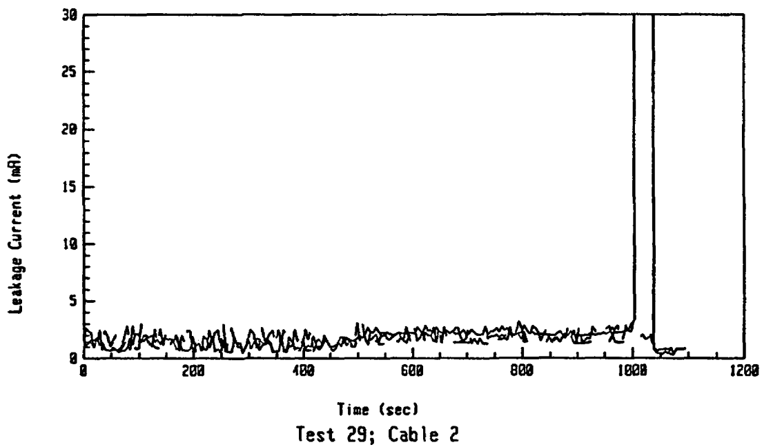
Figure A-26: Leakage Current Data For Test 29 Involving an Unaged BIW Cable at an Exposure Temperature of 375°C.
