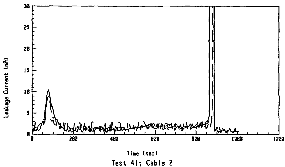
Figure A-38: Leakage Current Data For Test 41 Involving an Unaged BIW Cable at an Exposure Temperature of 375°C.
