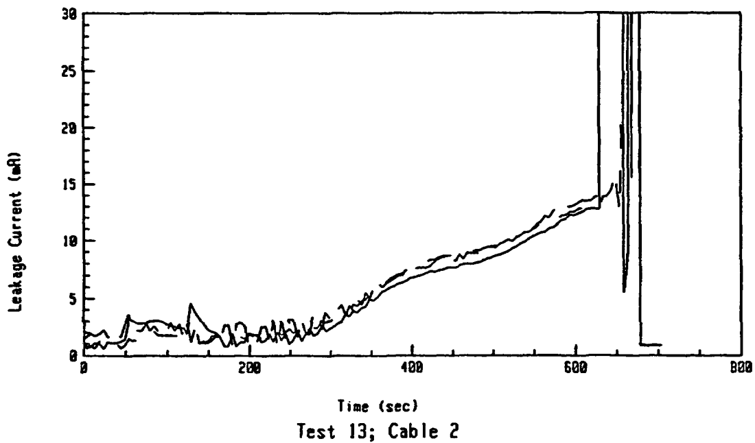
Figure A-10: Leakage Current Data For Test 13 Involving an Aged Rockbestos Cable at an Exposure Temperature of 400°C.
