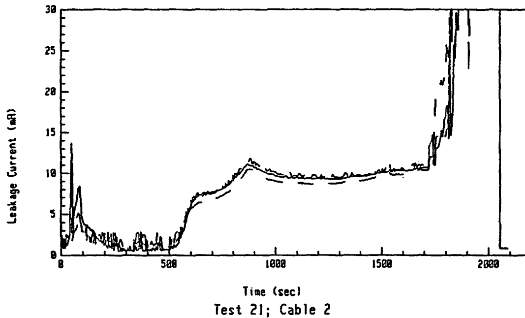
Figure A-18: Leakage Current Data For Test 21 Involving an Unaged Rockbestos Cable at an Exposure Temperature of 330°C.
