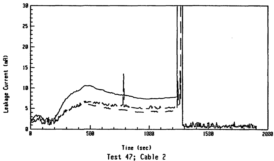
Figure A-44: Leakage Current Data For Test 47 Involving an Aged BIW Cable at an Exposure Temperature of 355°C.
