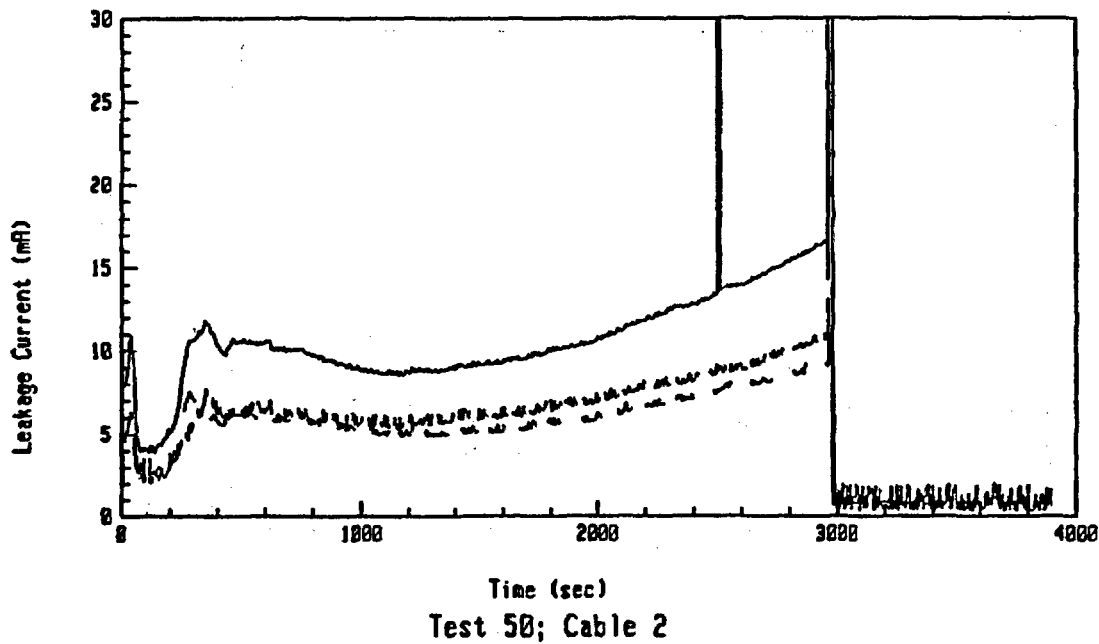
Figure A-47: Leakage Current Data For Test 50 Involving an Aged BIW Cable at an Exposure Temperature of 350°C. Note that a failure in the data logging system occurred prior to the failure of Cable 1.
