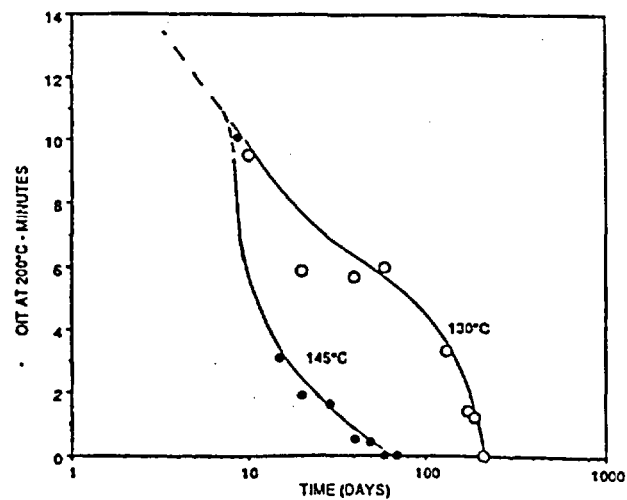
Figure 6.18 OIT at 200°C for EPR (Ref. 6.27) Reproduced with permission from Mr. D.J.R. Dodd, Ontario Hydro Technologies, Canada.
