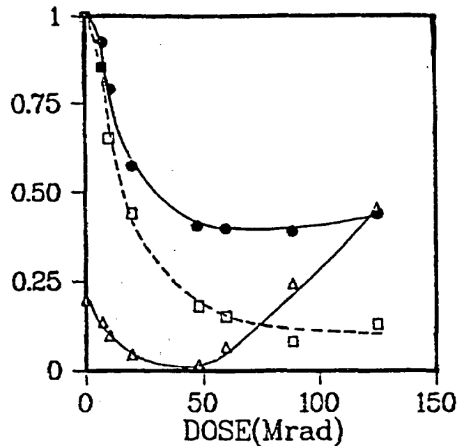
Figure 4.32 Radiation aging of PVC-I at 700 krad/hr (left) and 24 krad/hr (right), 43°C in air. Tensile strength (circles); elongation (squares); nonextractable fraction (triangles) (Ref. 4.64)
