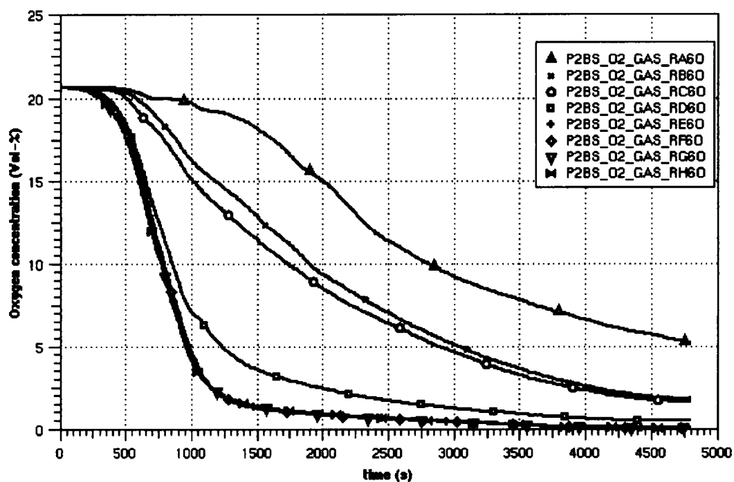
Figure 6-3 Oxygen concentration in the room centre
