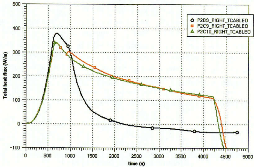
Figure 6-28 Total heat flow into target
