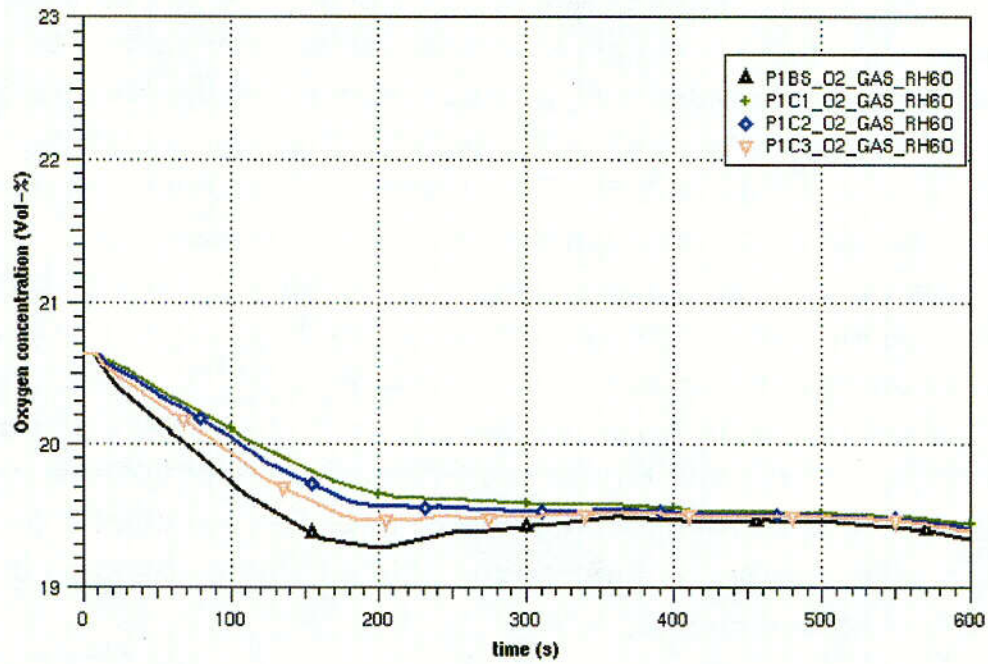
Figure 5-9 Oxygen concentration in the centre of the ceiling (RH6O)
