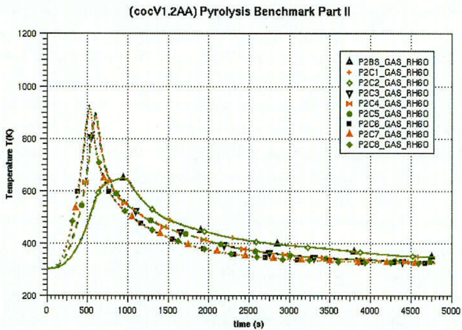
Figure 6-12 Temperatures below the ceiling in the room centre
