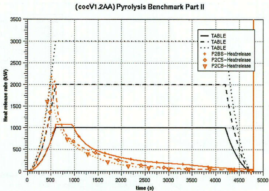
Figure 6-13 Heat release (base case, case5, case8)
