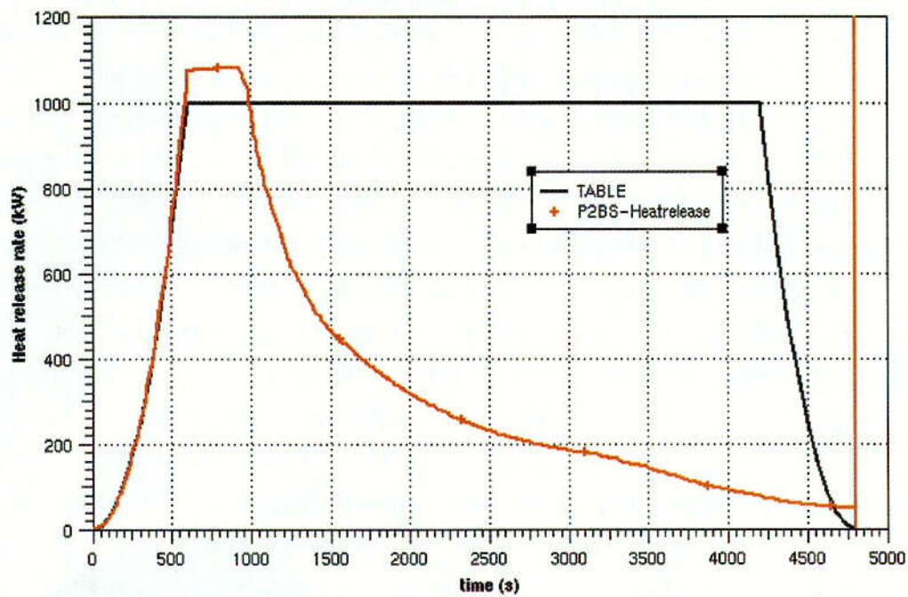
Figure 6-2 Heat release
