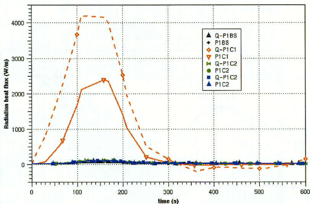
Figure 5-11 Radiation heat flux on the target
