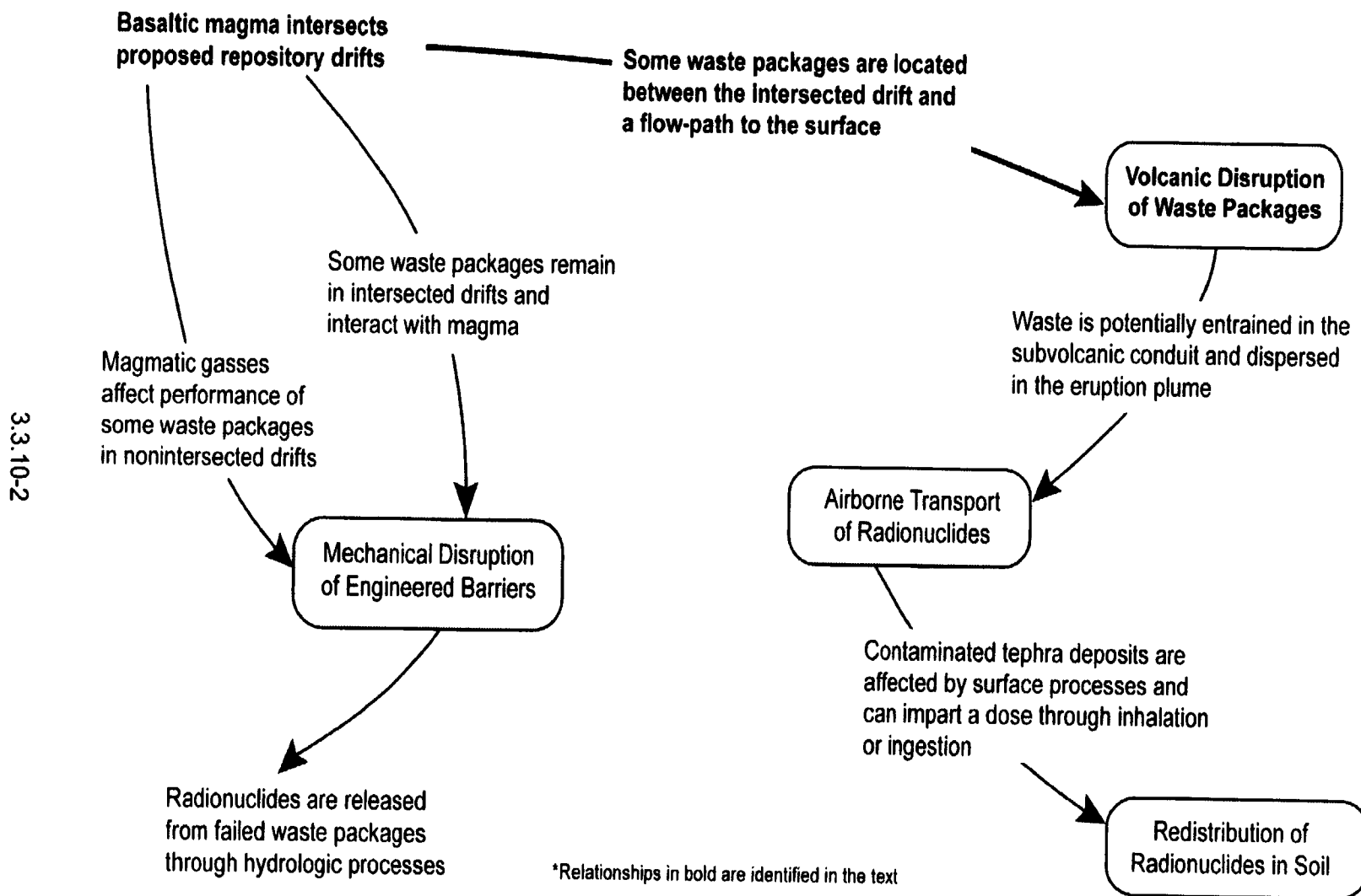
Figure 3.3.10-1. Diagram Illustrating the Relationship Between Volcanic Disruption of Waste Packages and Other Integrated Subissues
