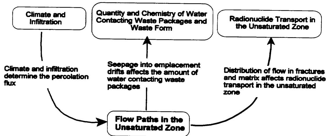
Figure 3.3.6-1. Diagram Illustrating the Relationship Between Flow Paths in the Unsaturated Zone and Other Integrated Subissues
