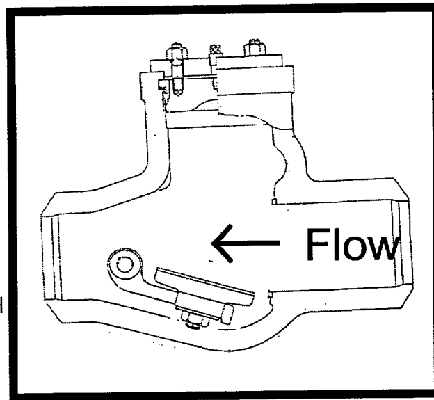
900# Swing Check Valve
