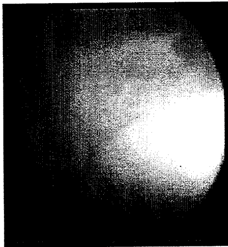
Radiograph of CK-ES3332 (side view) showing disk laying on bottom of valve. The seat side of the disk was facing up and the hinge arm was nearer the outlet port.
