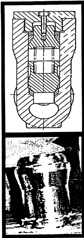
View looking into cylinder / body showing fretting area at outlet port.
