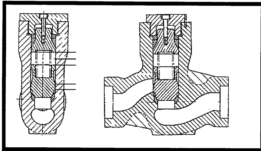
2-inch T-pattern Piston Check Valve
