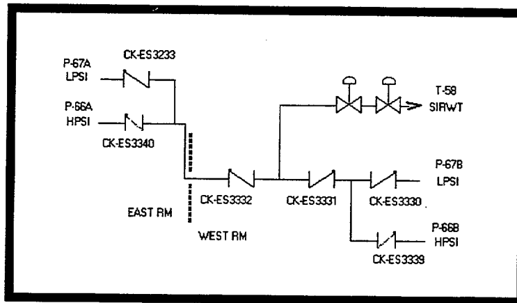
CK-ES3332 System Lineup
