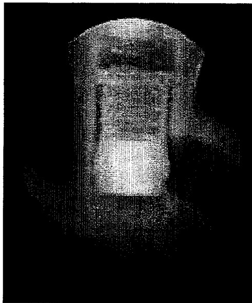
Radiograph of CK-ES3340 showing piston stuck open
