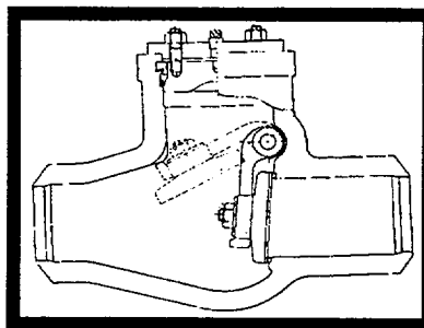
Swing Check Valve
