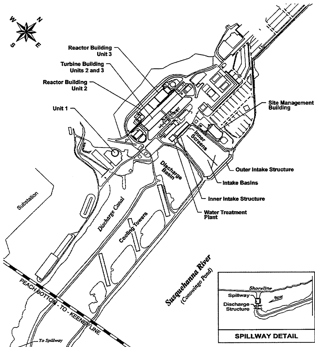
Figure 2-3. Peach Bottom Station Layout
