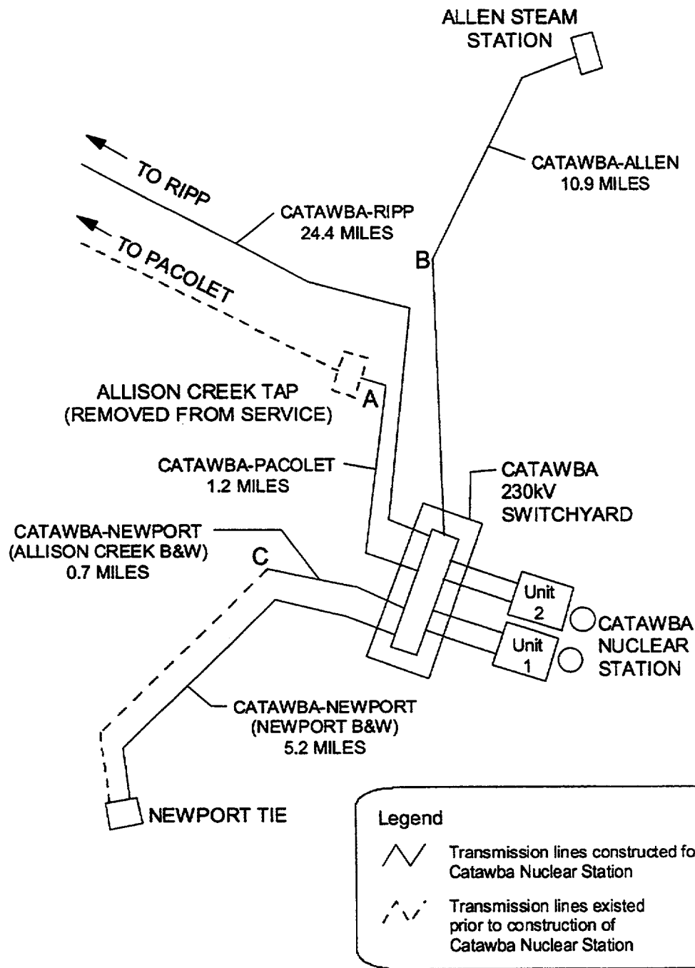
Figure 2-4. Catawba Transmission Lines and Rights-of-Way (Duke 2001a)
