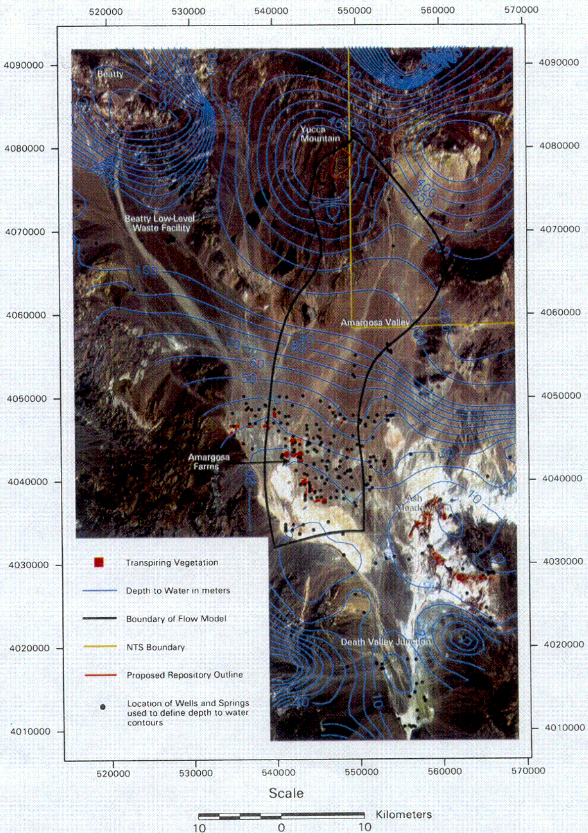
Figure 2-5. Landsat Image of the Yucca Mountain and the Amargosa Desert Region. In the Amargosa Farms area, red circular forms are quarter-section, center-pivot irrigation plots. These contrast with flood-irrigation plots shown as rectangular-shaped forms. Irregular red patches correspond to areas in Ash Meadows containing wetland/riparian vegetation. Blue contour lines showing the depth to the water table are in the equivalent of meters. Thematic sensor data from the Landsat satellite were used to produce the background image. Satellite altitude was approximately 185 kilometers (115 miles).
