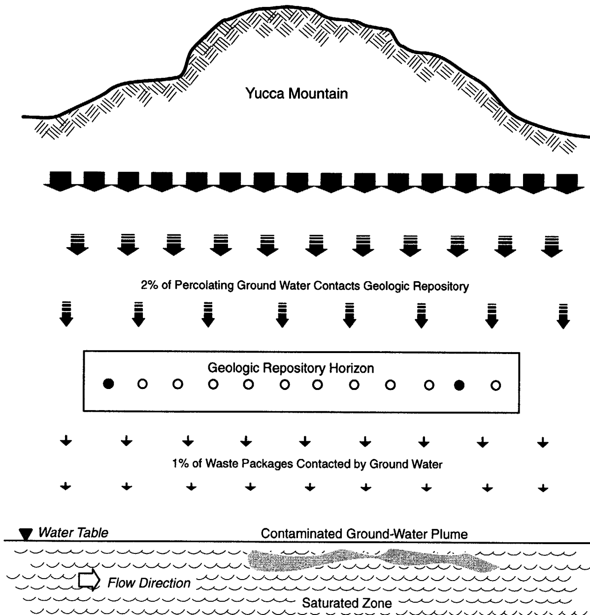
Figure 6-5. Drinking water dose model. Illustration shows ground water percolating through Yucca Mountain, 2 percent of which reaches waste emplacement horizon and contacts 1 percent of the waste package canisters. Subsequently, the radioactive leachate continues to percolate downward until it reaches the water table.
