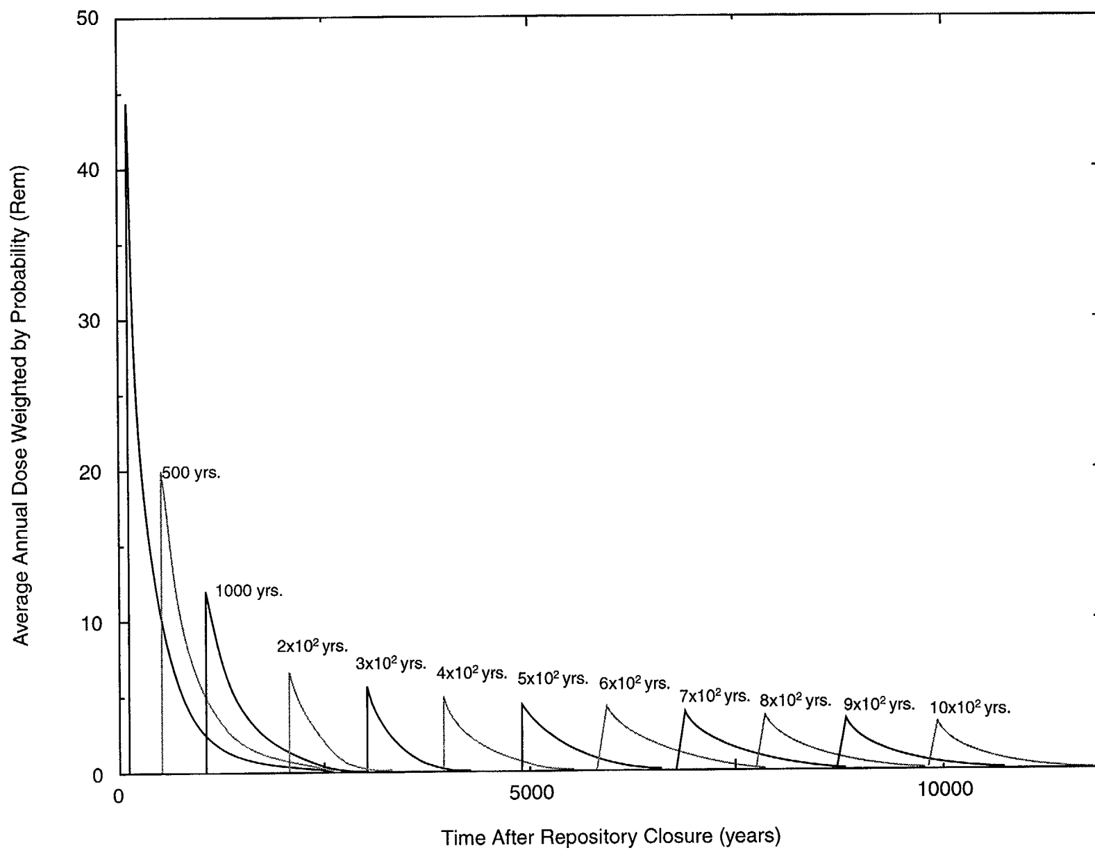
Figure 5-3. Expected annual dose as a function of time from extrusive volcanic events.
