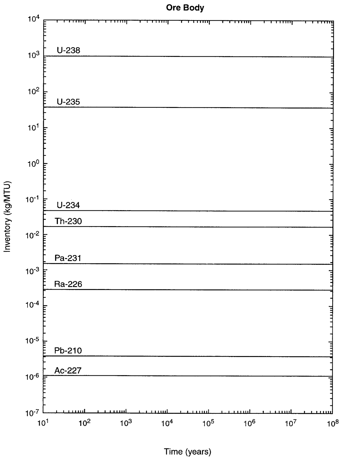
Figure 6-3. Radionuclide inventory of the hypothetical ore body.
