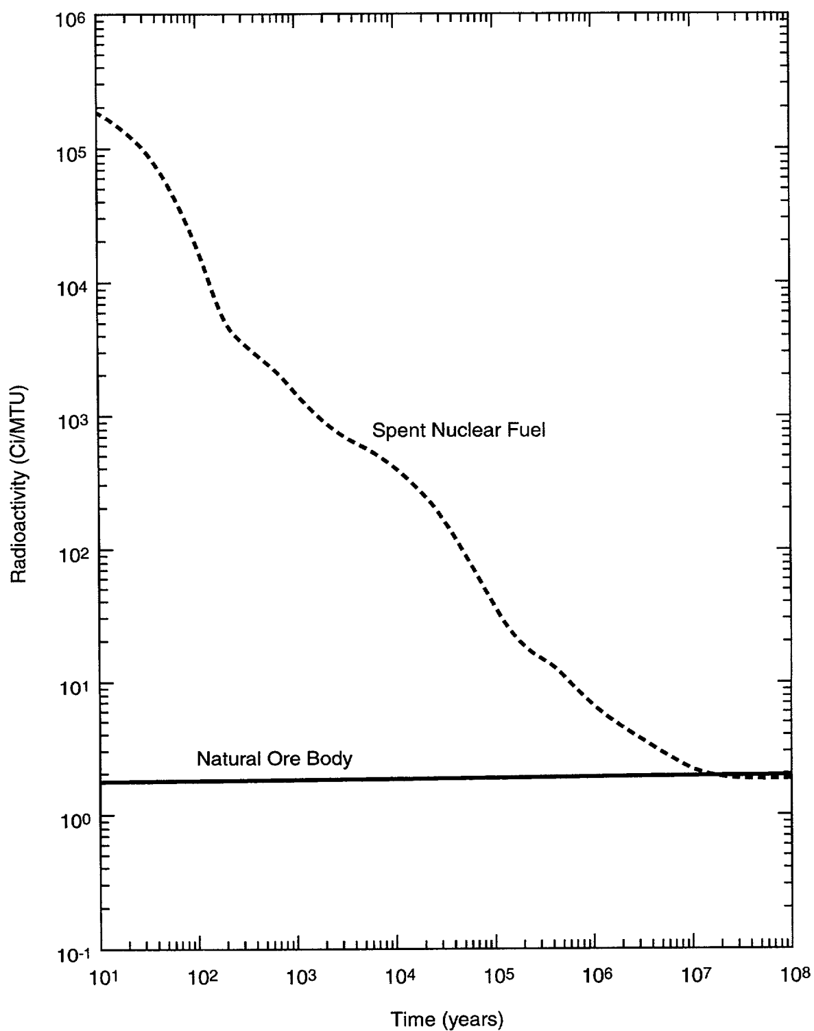
Figure 6-4. Comparison of radioactivity between the spent fuel repository and the hypothetical ore body.
