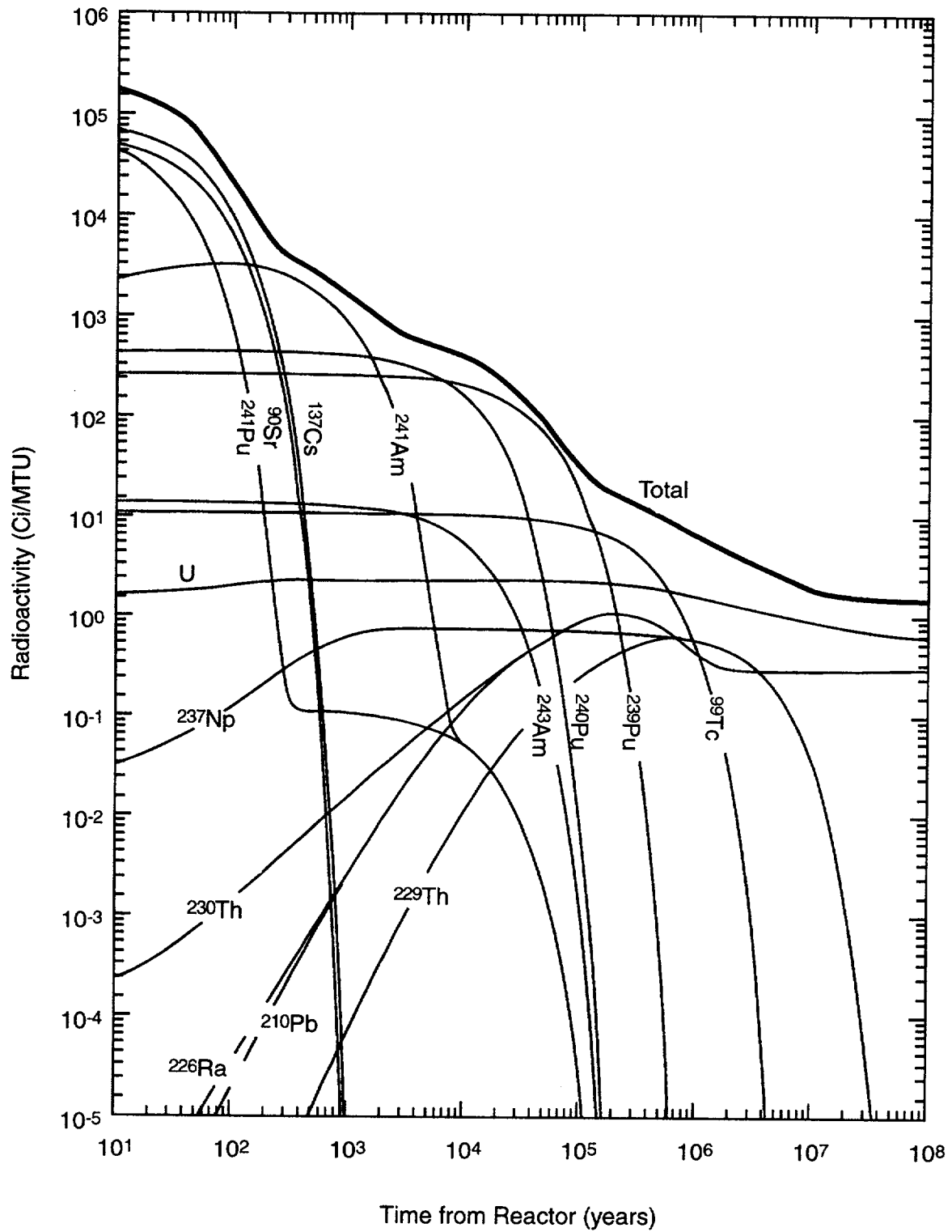
Figure 6-2. Radioactivity of SNF. Inventory based on Lozano et al. (1994).
