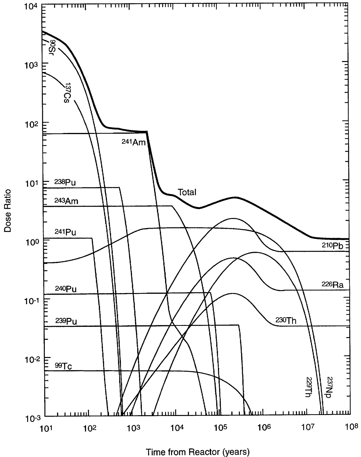
Figure 6-6. Relative radiological hazard of SNF calculated as the ratio of doses from drinking ground water contaminated by the spent fuel repository and by the hypothetical ore body.
