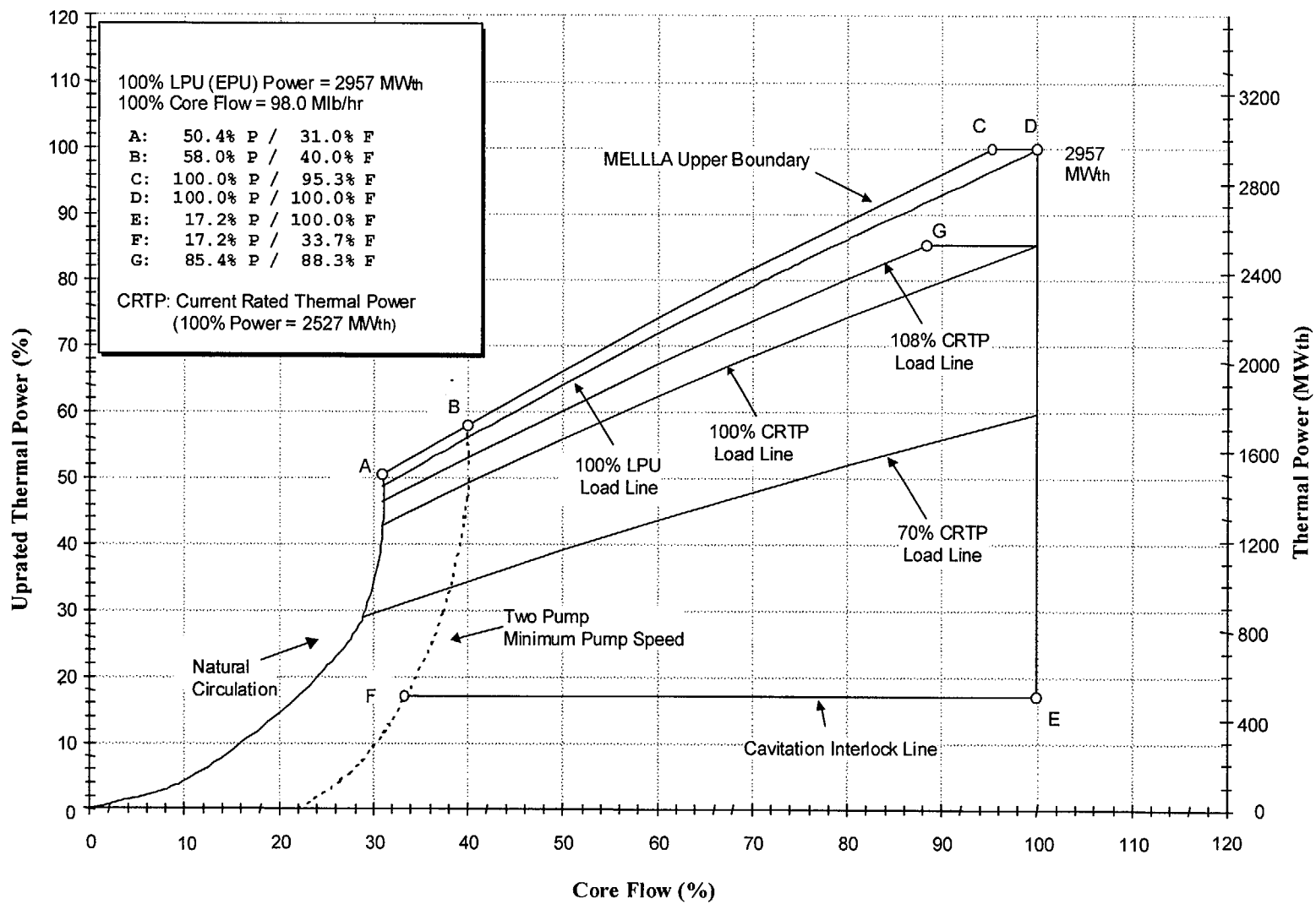
Figure 2-1. Power/Flow Operating Map for EPU
