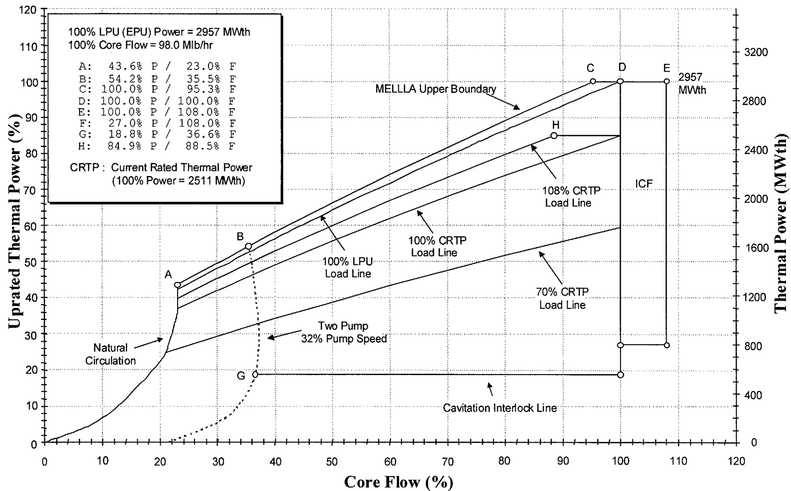
Figure 2-1. Power/Flow Operating Map for EPU
