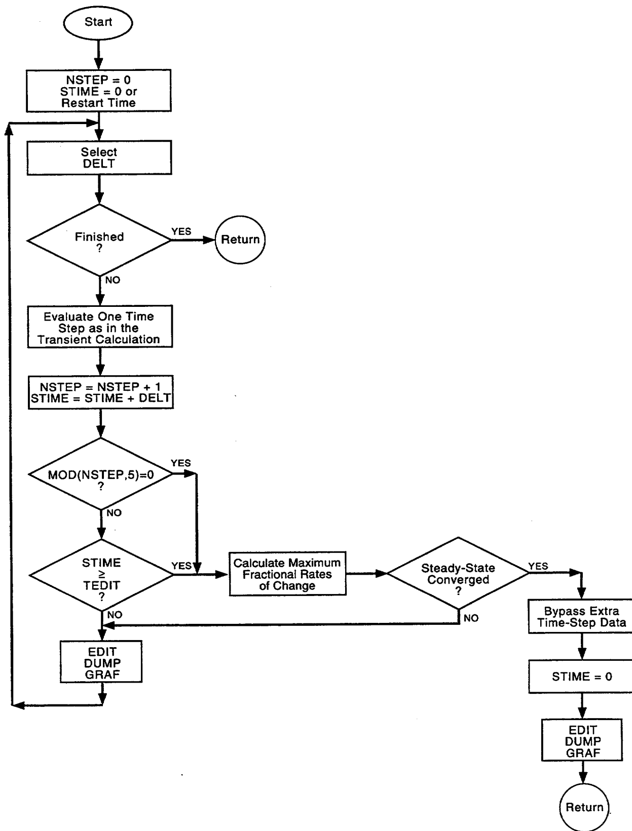
Fig. 2-3. Steady-state-calculation flow diagram.
