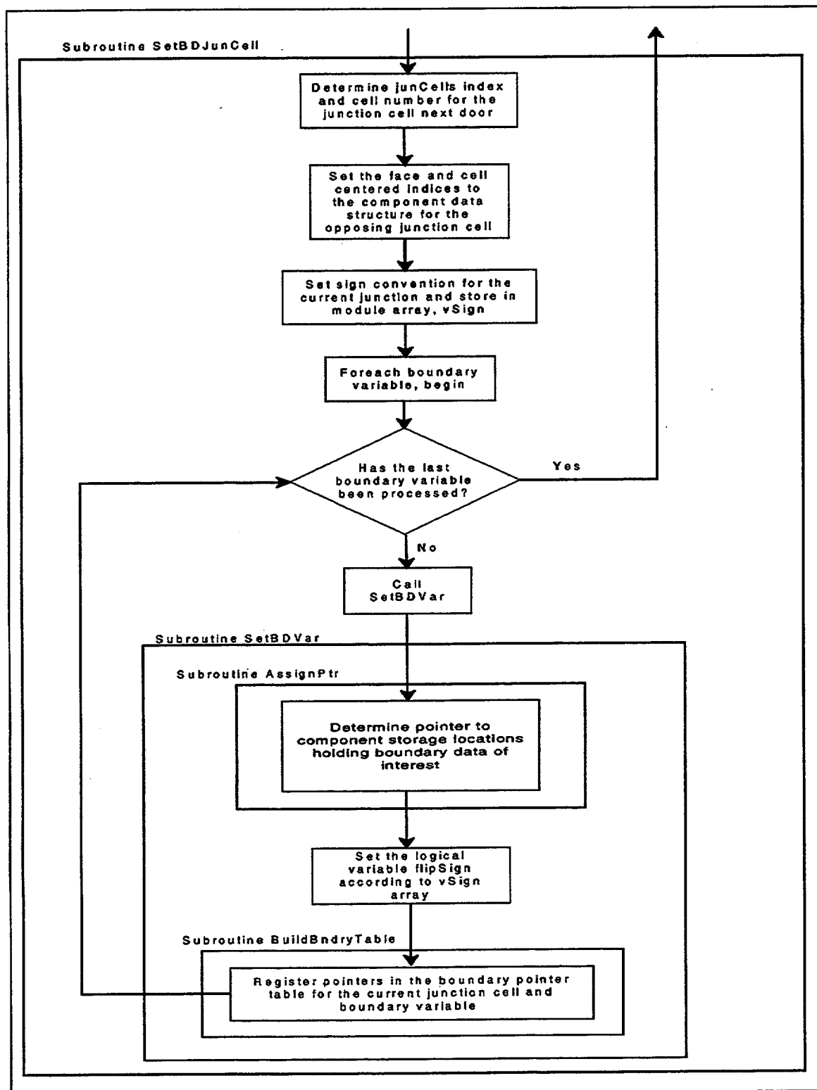
Fig. 3-6. Flow logic for System Service initialization (cont)
