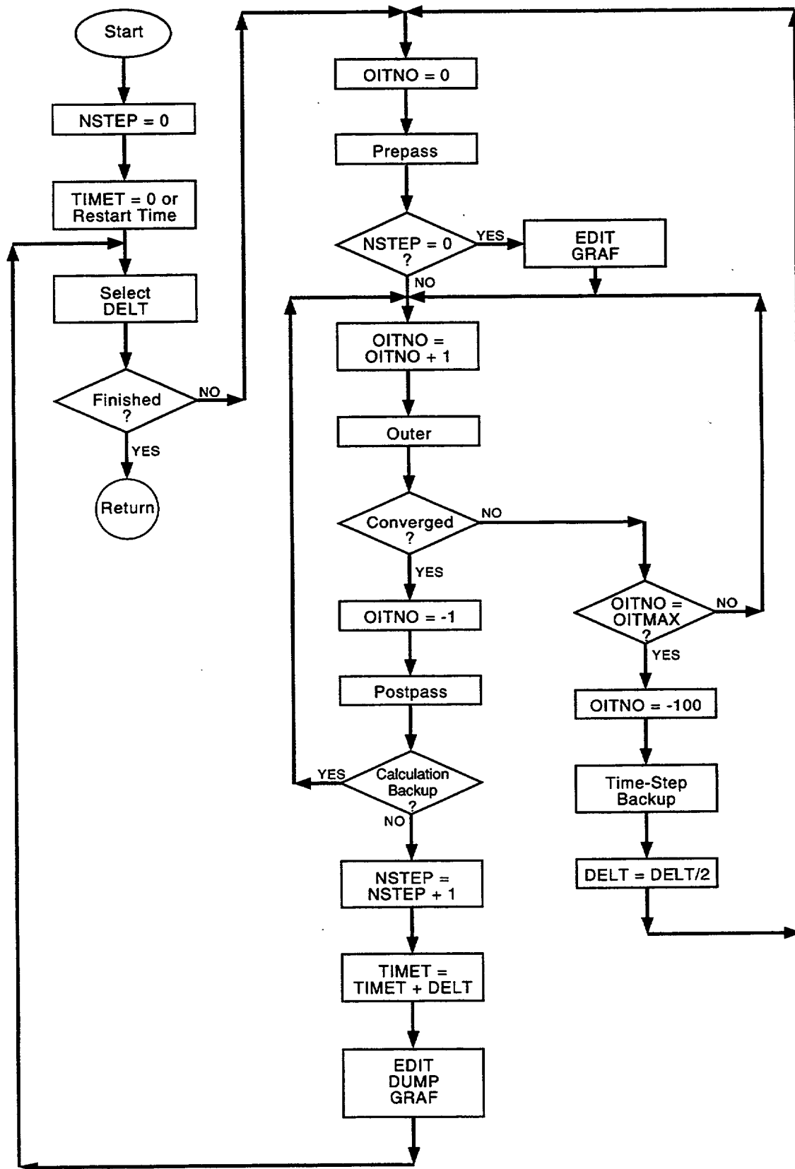
Fig. 2-2. Transient-calculation flow diagram.
