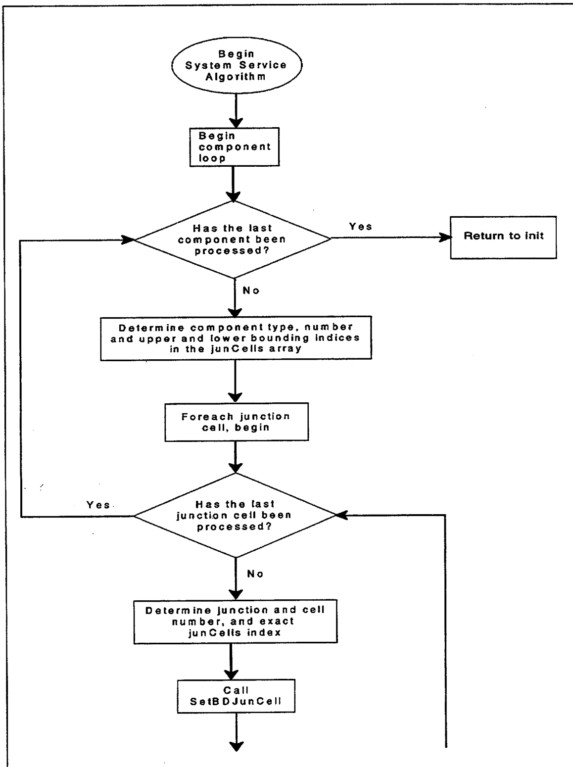
Fig. 3-6. Flow logic for System Service initialization
