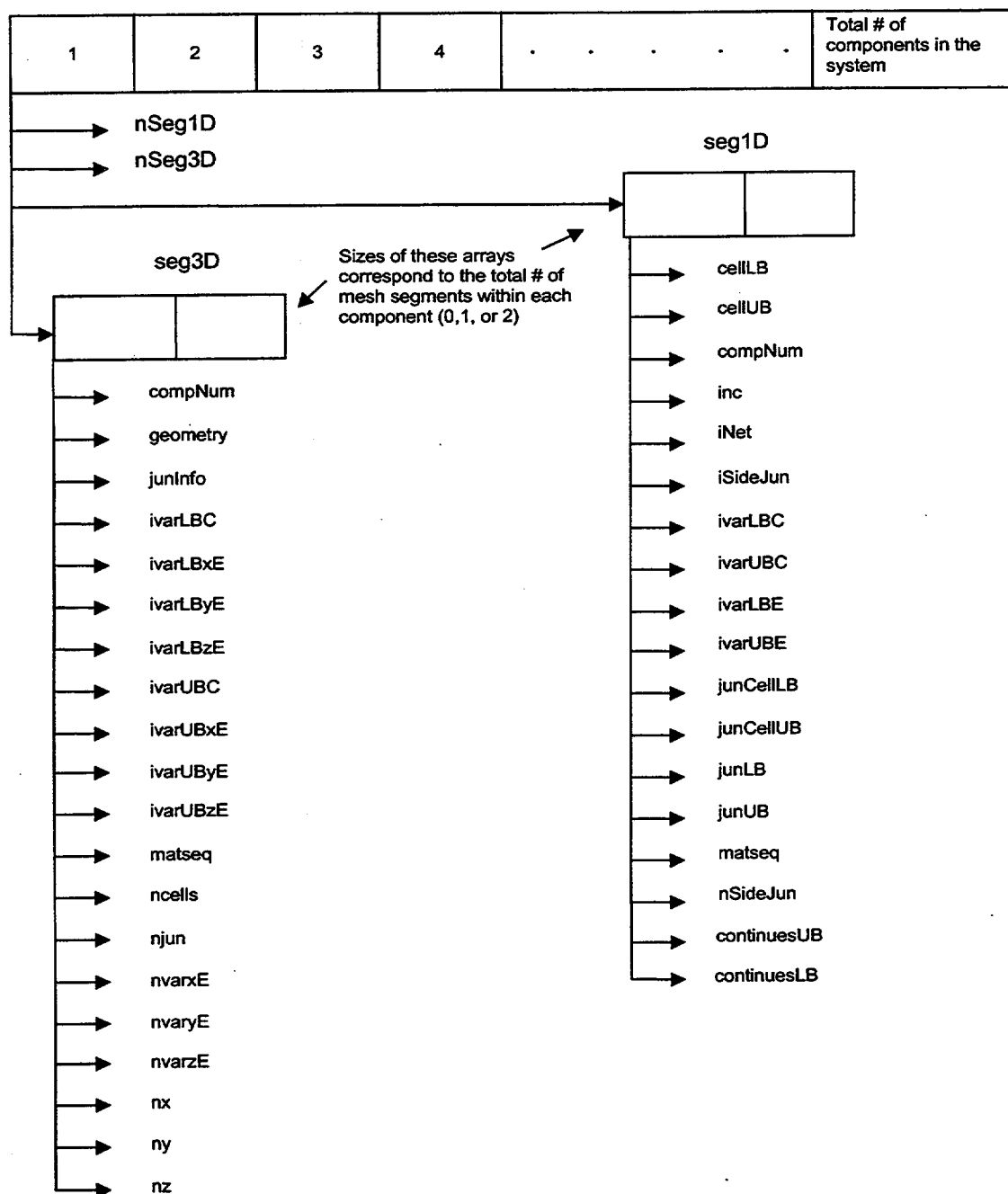
Fig. 3-5. Graphical representation of the compSeg array.
