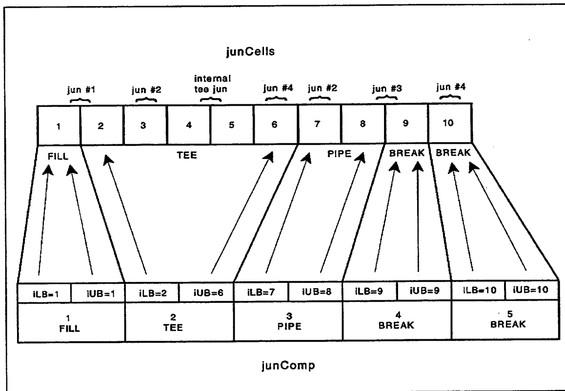
Fig. 3-4. Graphical representation of the coupling between the junCells and junComp arrays for a FILL, TEE, PIPE, BREAK, and BREAK system.
