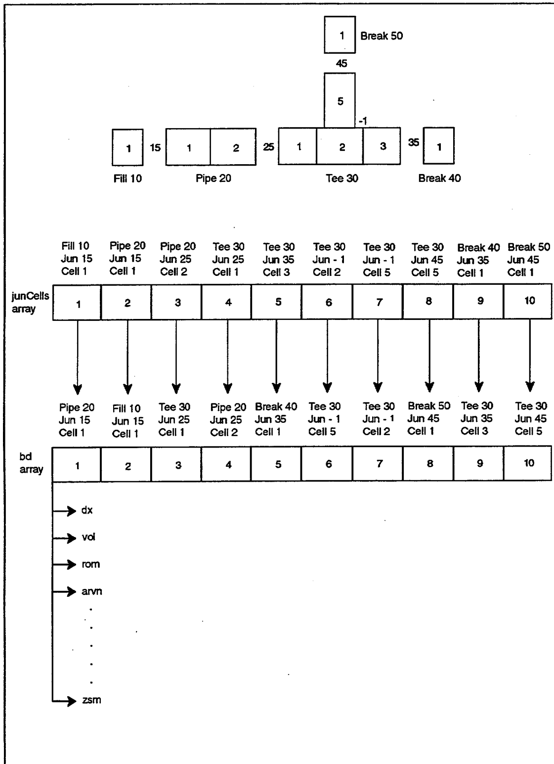
Fig. 3-2. Boundary Array Layout
