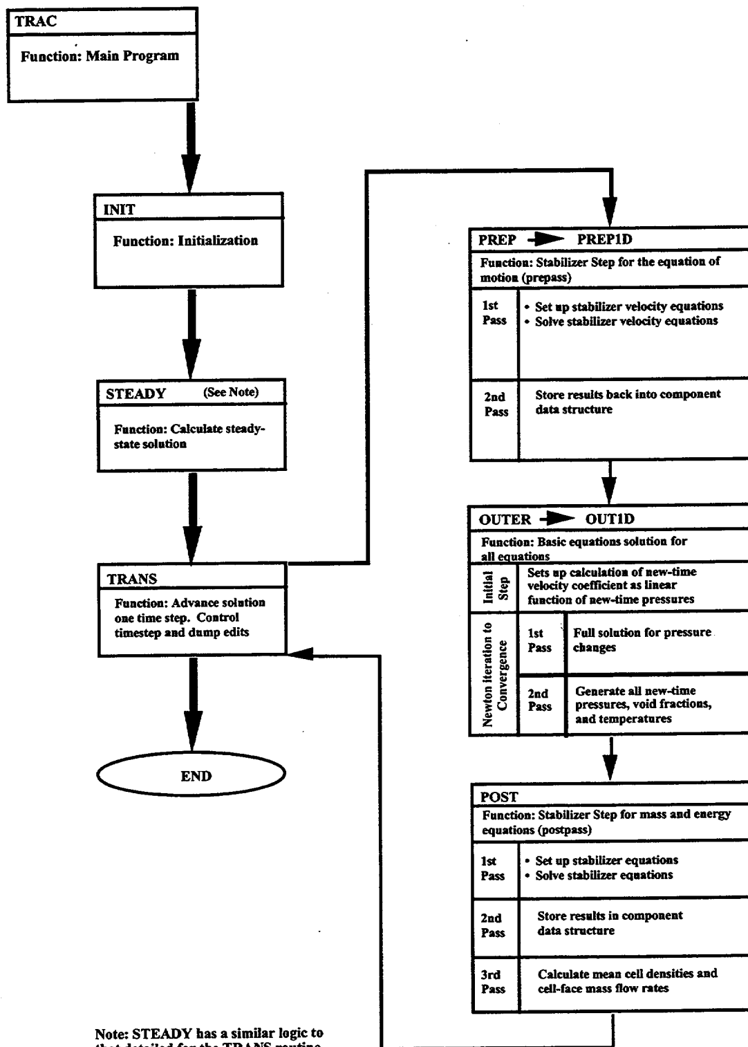
Fig. 2-1. TRAC-M computational flow.
