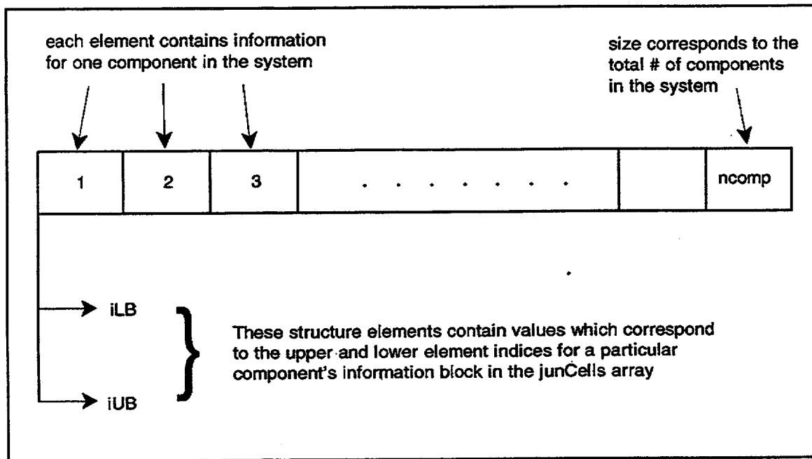
Fig. 3-3. Graphical representation of the junComp array
