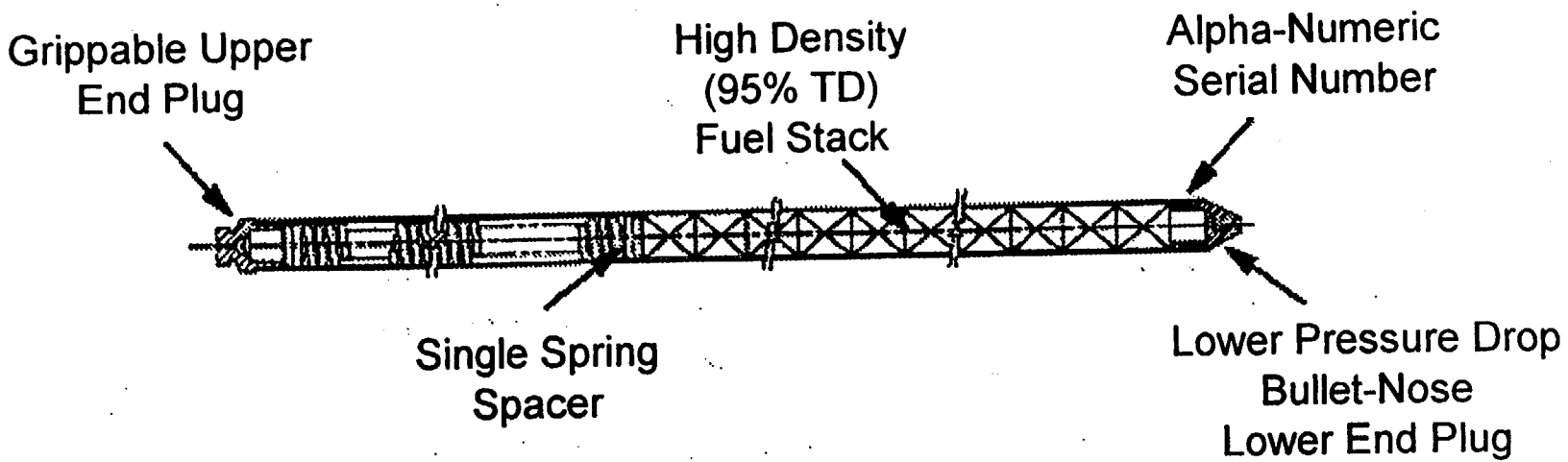
Figure A-6 Mark-BW/MOX1 Fuel Rod Design
