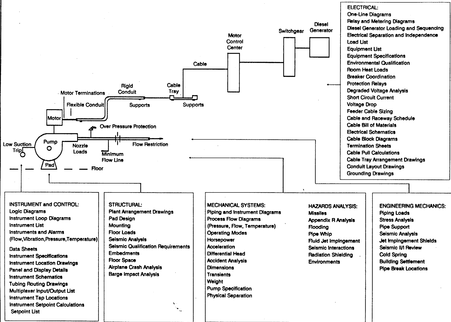
Design Products and Activities for a Typical Pump
